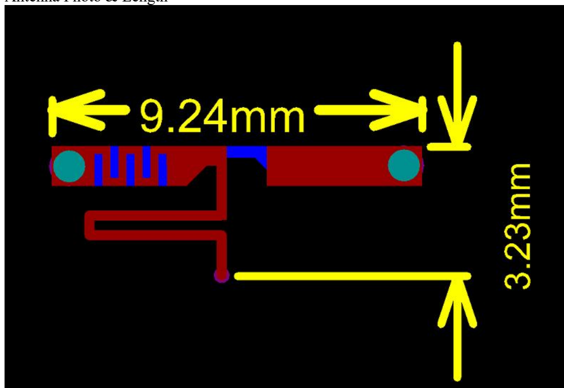
Antenna Photo & Length
