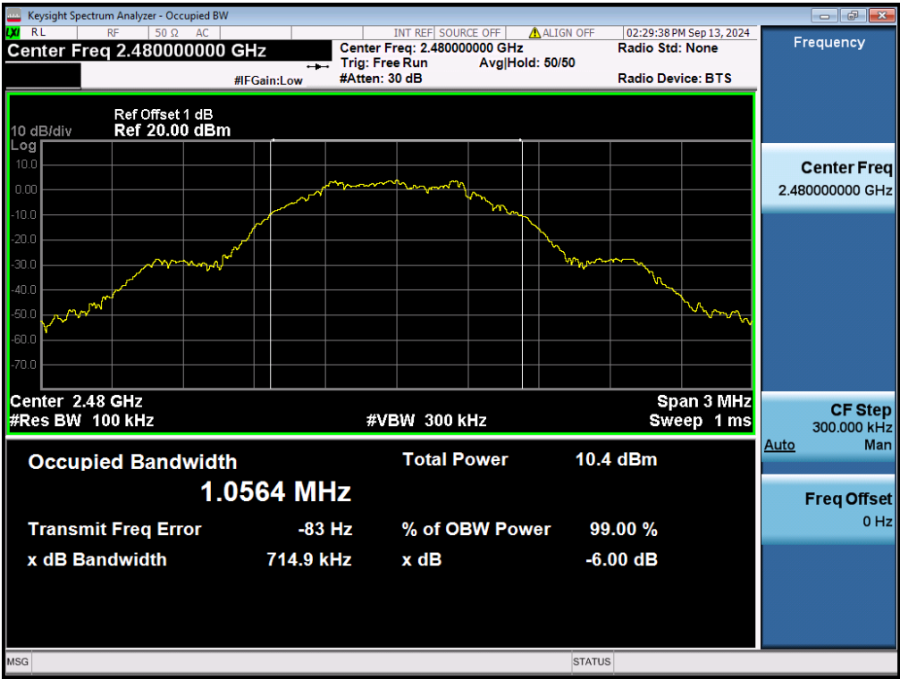
99% Bandwidth, 2480MHz
