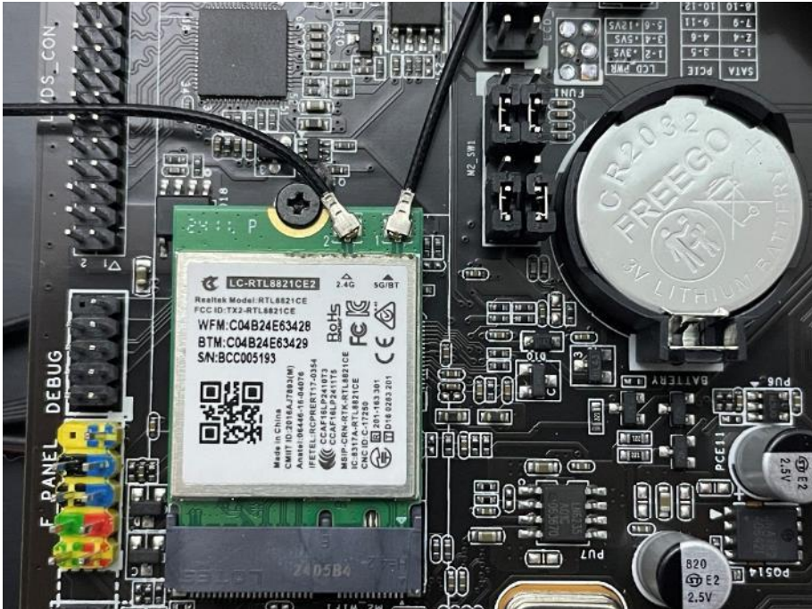
Antenna Interface
