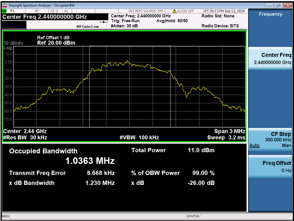
99% Bandwidth, 2440MHz
