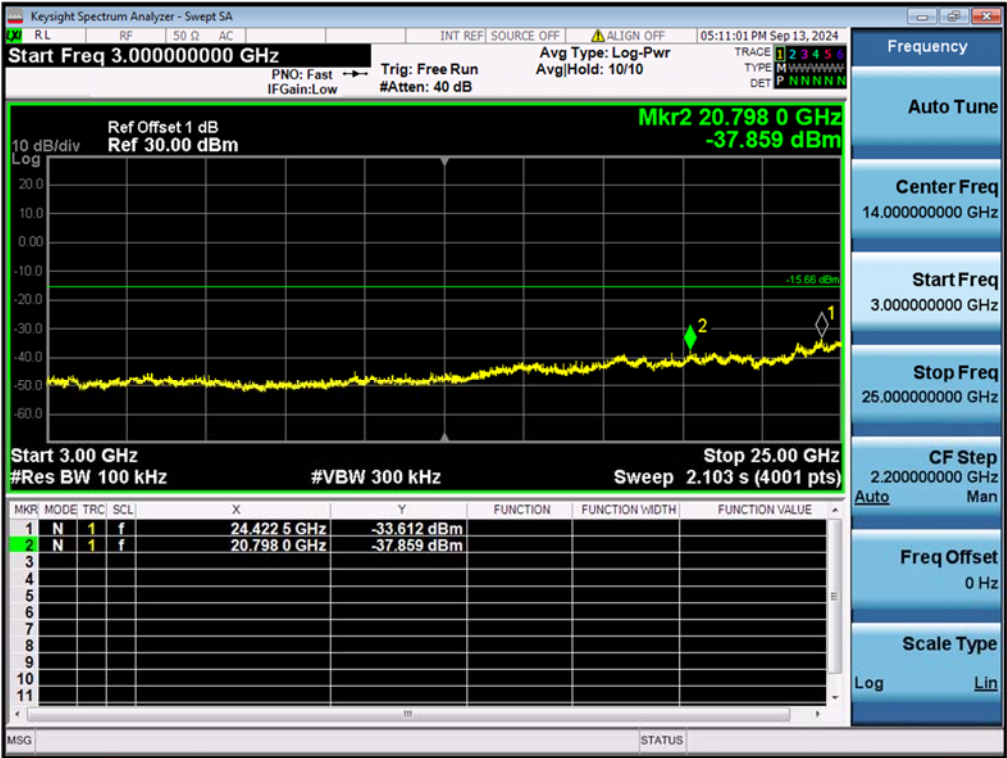
Figure 22: Conducted Spurious Emission & Authorized-band band-edge, 2402MHz, \pi/4 -DQPSK Carrier Level
