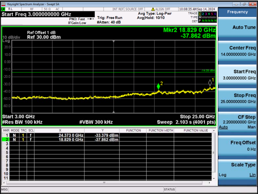
Figure 23: Conducted Spurious Emission & Authorized-band band-edge, 2441MHz, \pi/4 -DQPSK Carrier Level
