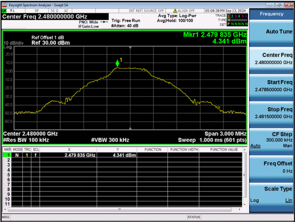
Figure 21: Conducted Spurious Emission & Authorized-band band-edge, 2480MHz, GFSK Carrier Level
