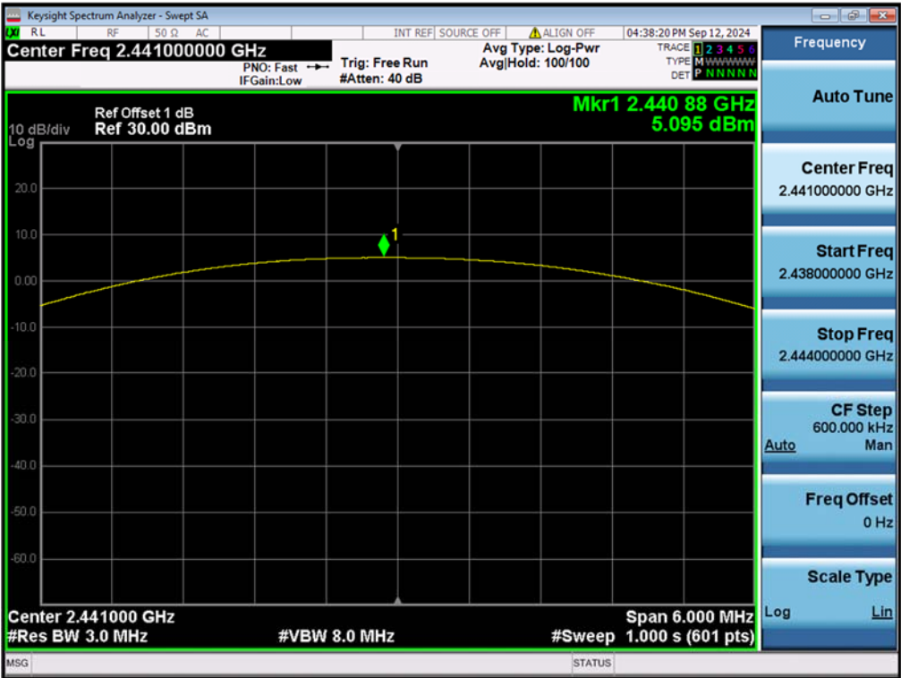
Figure 2: Maximum Peak Output Power, 2441MHz, GFSK
