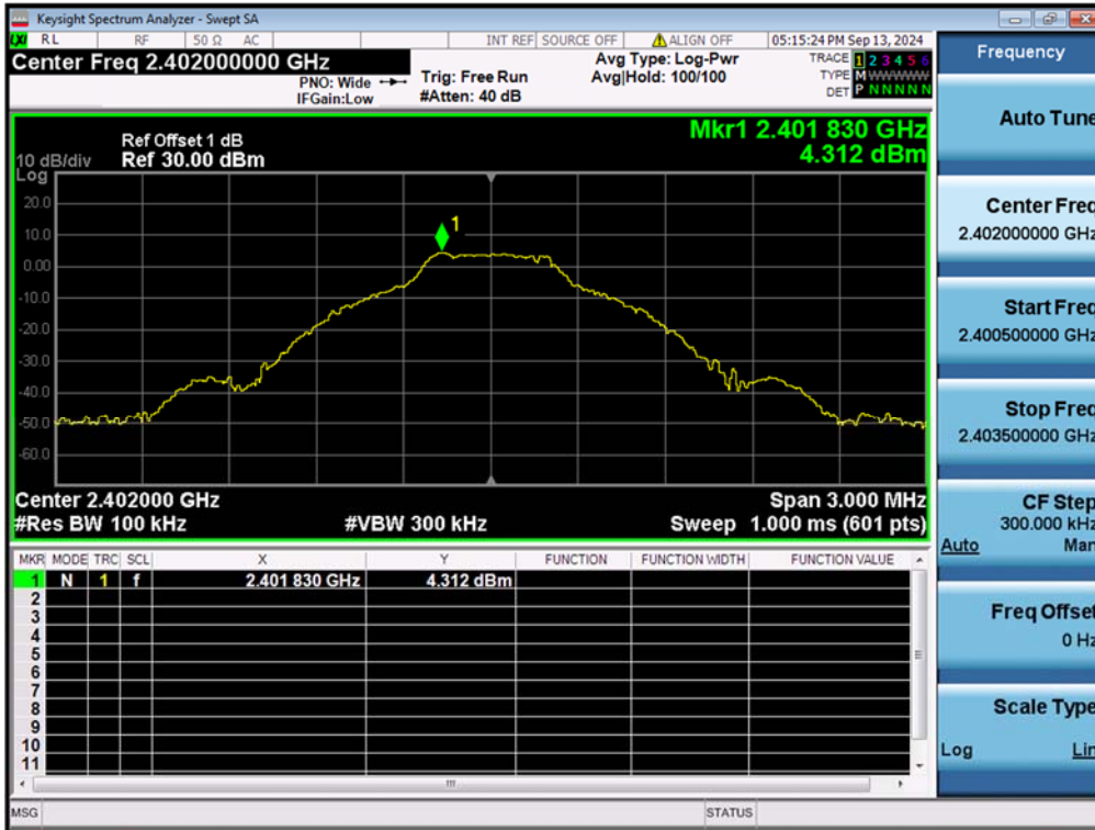
Figure 19: Conducted Spurious Emission & Authorized-band band-edge, 2402MHz, GFSK Carrier Level
