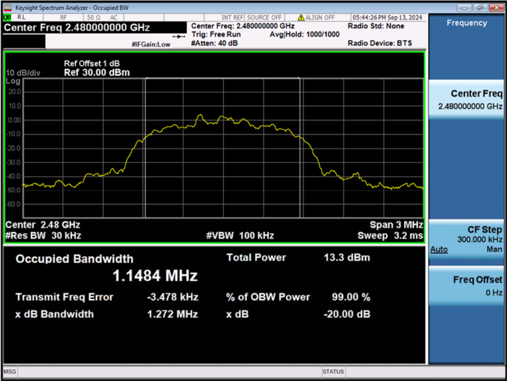
Figure 18: 20dB Bandwidth and 99% Bandwidth, 2480MHz, 8-DPSK
