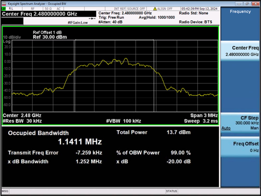
Figure 15: 20dB Bandwidth and 99% Bandwidth, 2480MHz, \pi/4 -DQPSK
