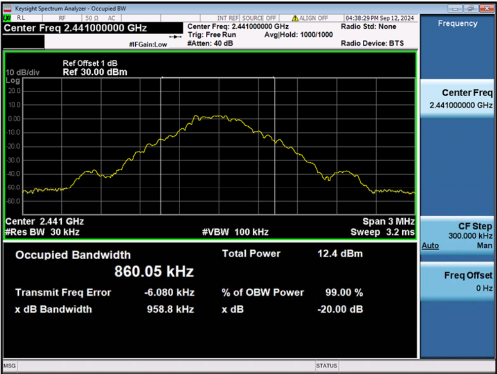
Figure 11: 20dB Bandwidth and 99% Bandwidth, 2441MHz, GFSK
