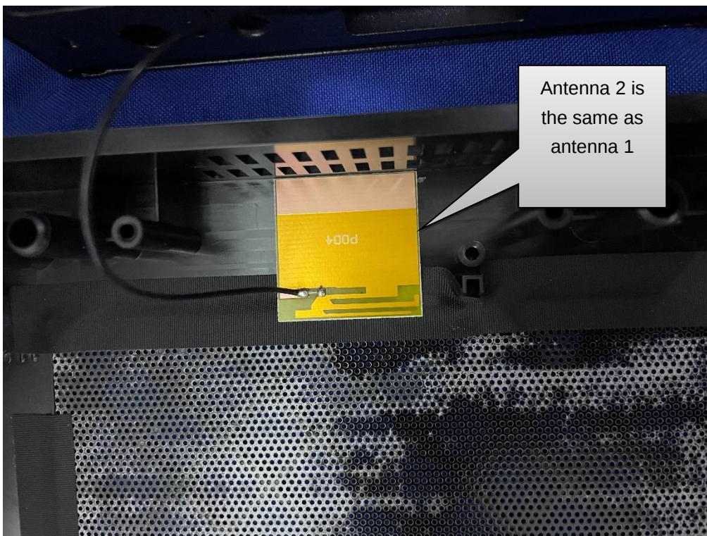
Antenna Interface
