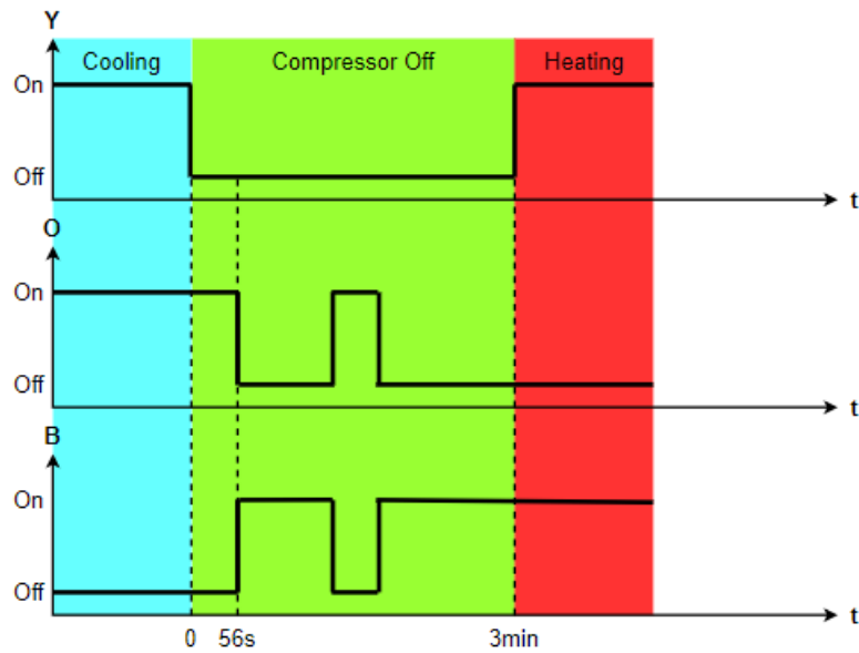
4-Way Valve Changing : Cooling To Heating
