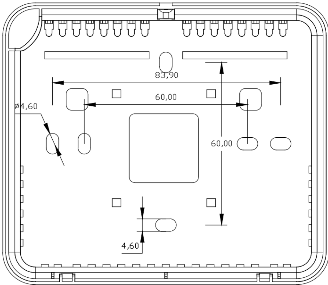
FIGURE 2: MT-5 MOUNTING HOLES DISTANCES AND SIZES(MM).
