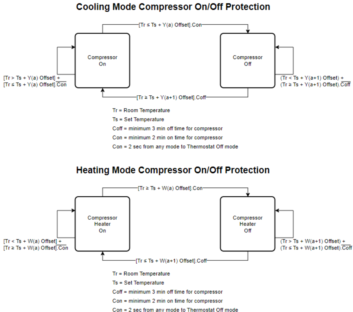
FIGURE 16: COMPRESSOR PROTECTION
