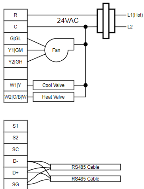
FIGURE 23: FCU APPLICATION AN TYPE AND WIRING
