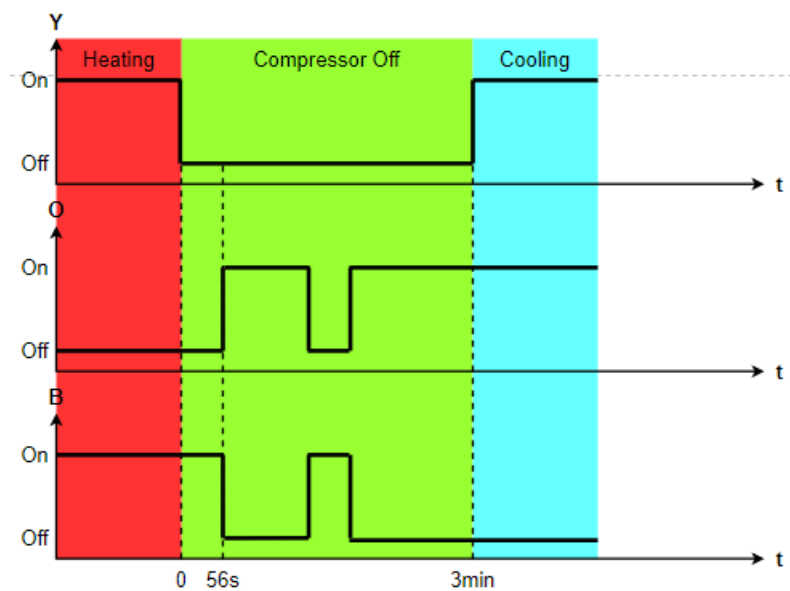
4-Way Valve Changing : Heating To Cooling
