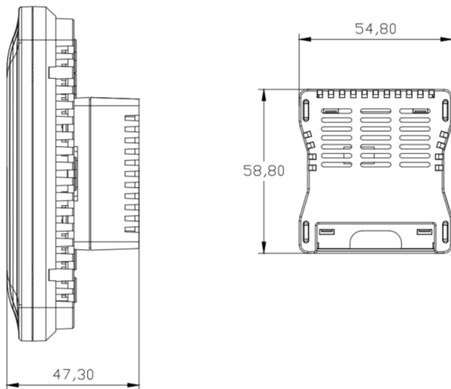
FIGURE 3: MT-5-X/L DIMENSION
