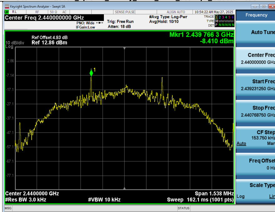
Power Spectral Density NVNT ANT1 500 kbps 2440
