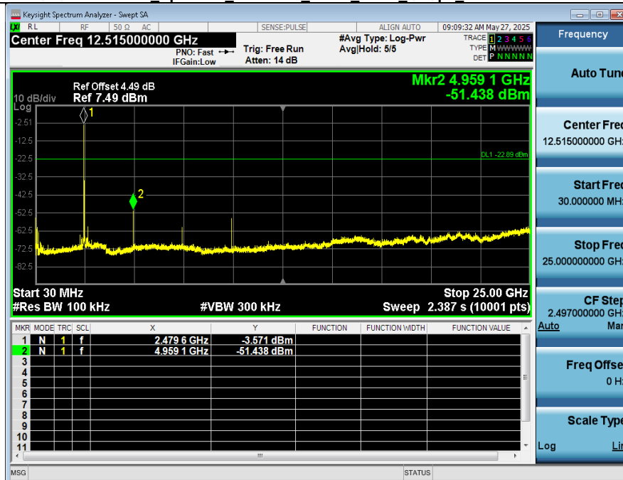
2_Spurious_Emission_NVNT_ANT1_1Mbps_2480
