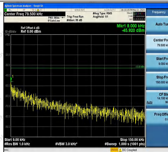
Band5-4182-3-0.009~0.15MHz-PASS
