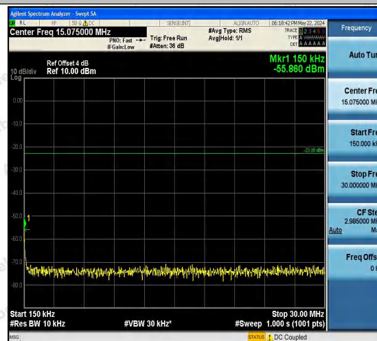
Band5-4182-3-0.15~30MHz-PASS
