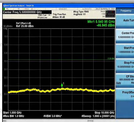
Band5-4182-4-1000~10000MHz-PASS
