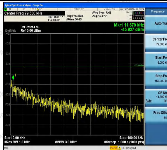
Band5-4132-2-0.009~0.15MHz-PASS
