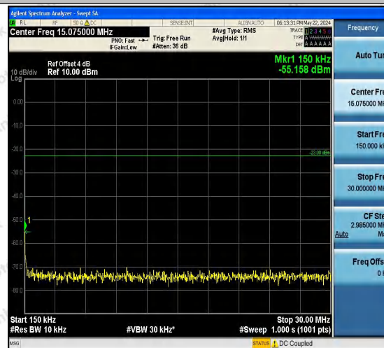
Band5-4132-2-0.15~30MHz-PASS
