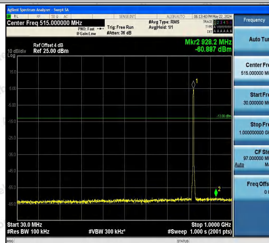
Band5-4132-2-30~1000MHz-PASS
