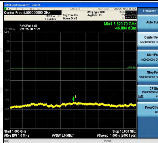
Band5-4132-3-1000~10000MHz-PASS
