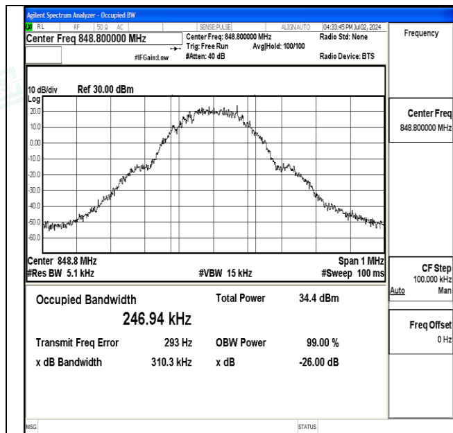
Channel 251 / 848.8 MHz
