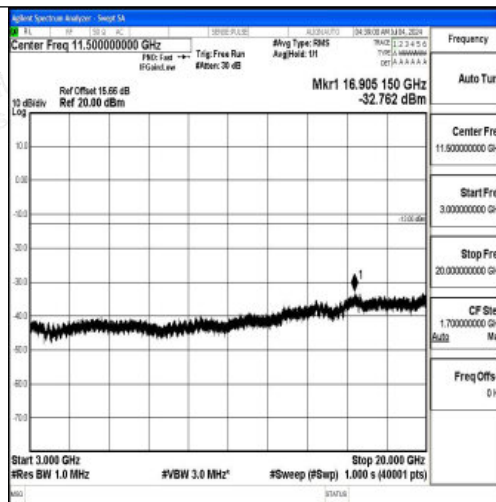
Band66_15MHz_16QAM_132047_1RB#0_3000~20000_3000~20000
