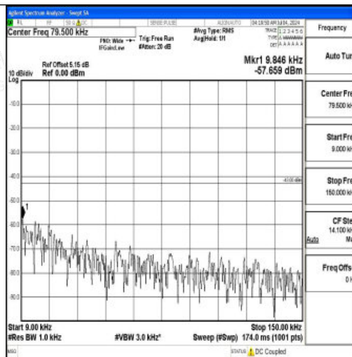
Band66_10MHz_16QAM_132322_1RB#0_0.009~0.15_0.009~0.15
