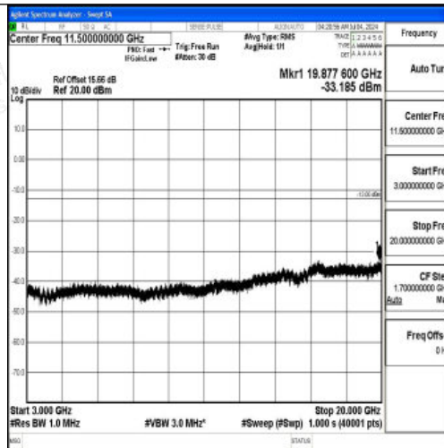
Band66_10MHz_QPSK_132622_1RB#0_3000~20000_3000~20000
