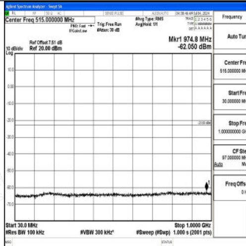
Band66_15MHz_16QAM_132047_1RB#0_30~1000_30~1000
