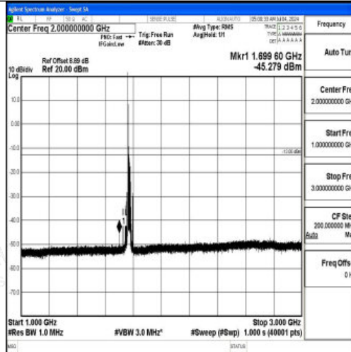
Band66_20MHz_16QAM_132572_1RB#0_1000~3000_1000~3000
