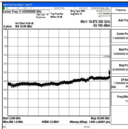
Band66_20MHz_QPSK_132572_1RB#0_3000~20000_3000~20000
