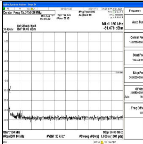
Band66_15MHz_QPSK_132322_1RB#0_0.15~30_0.15~30
