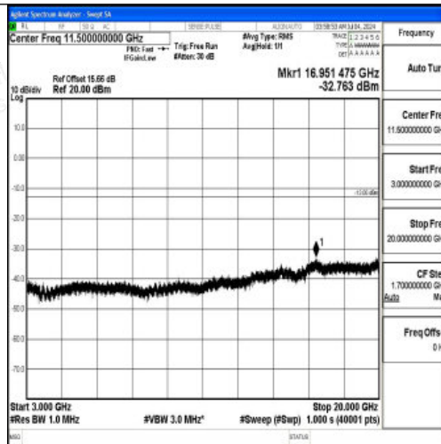
Band66_5MHz_16QAM_131997_1RB#0_3000~20000_3000~20000
