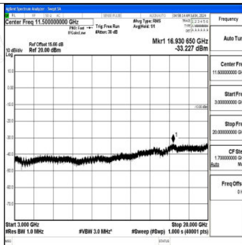
Band66_20MHz_16QAM_132072_1RB#0_3000~20000_3000~20000
