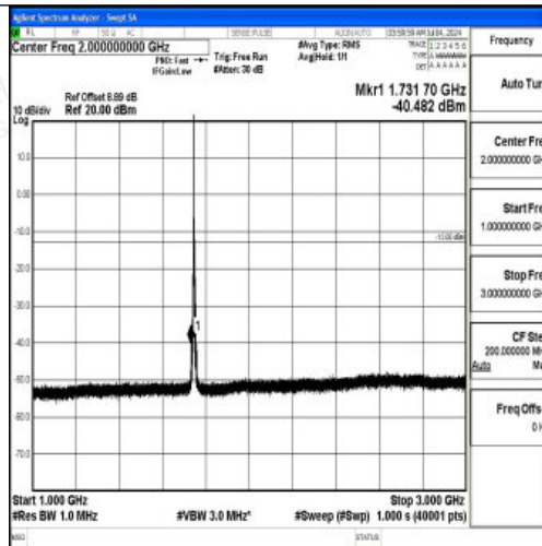
Band66_5MHz_16QAM_132322_1RB#0_1000~3000_1000~3000
