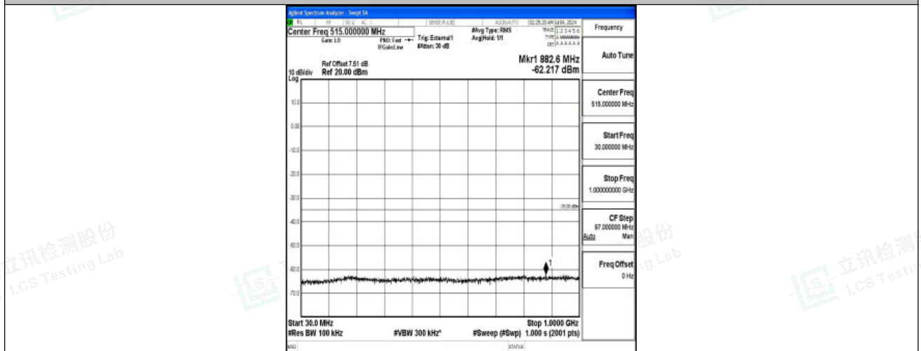
Band41_15MHz_16QAM_41515_1RB#0_30~1000_30~1000
