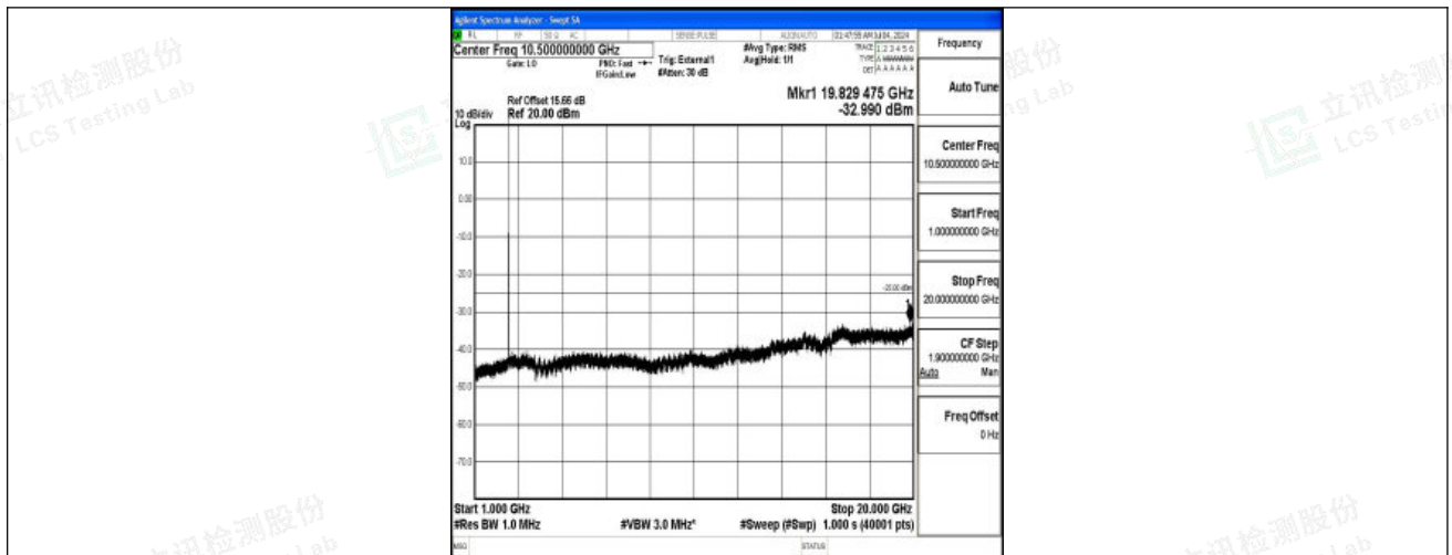
Band41_10MHz_16QAM_39700_1RB#0_1000~20000_1000~20000
