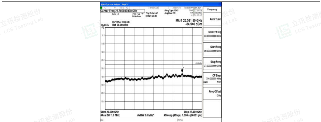
Band41_10MHz_16QAM_41540_1RB#0_20000~27000_20000~27000
