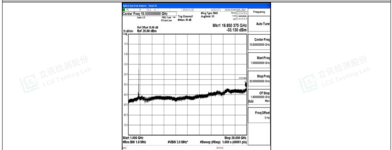
Band41_20MHz_16QAM_41490_1RB#0_1000~20000_1000~20000
