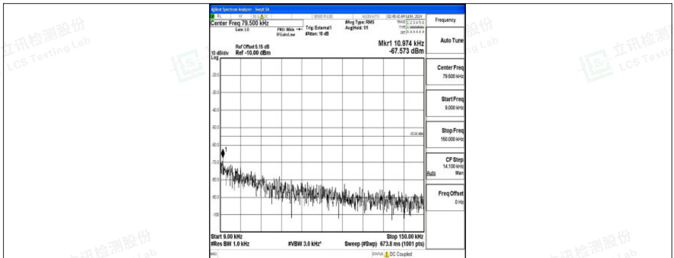
Band41_20MHz_16QAM_39750_1RB#0_0.009~0.15_0.009~0.15
