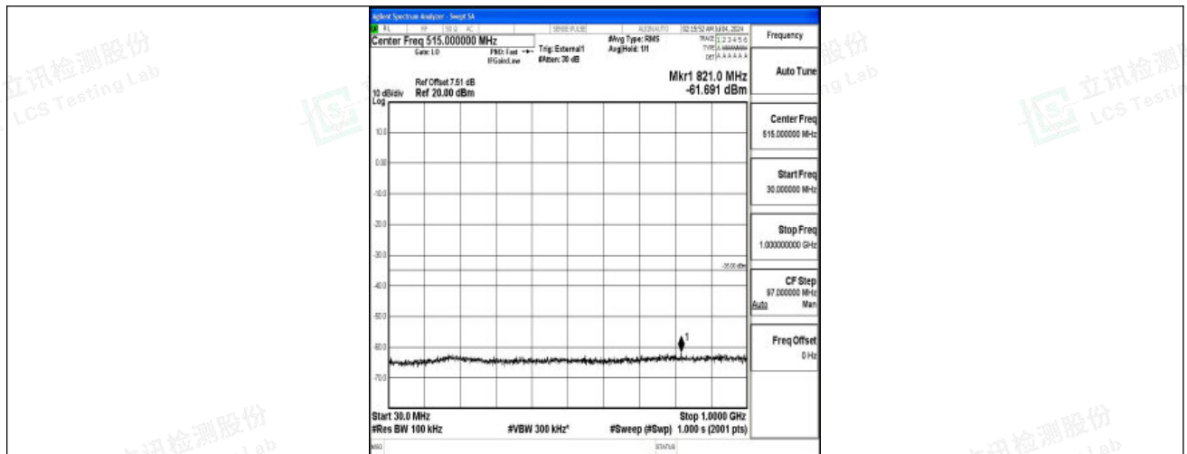
Band41_15MHz_QPSK_39725_1RB#0_30~1000_30~1000
