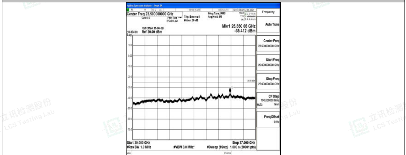
Band41_20MHz_16QAM_39750_1RB#0_20000~27000_20000~27000
