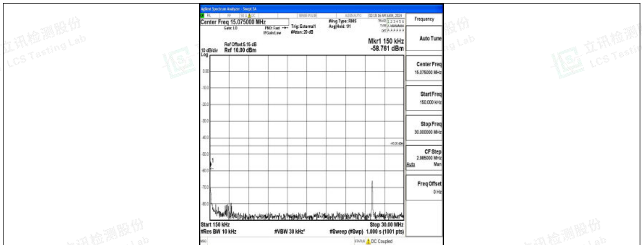
Band41_15MHz_QPSK_40620_1RB#0_0.15~30_0.15~30
