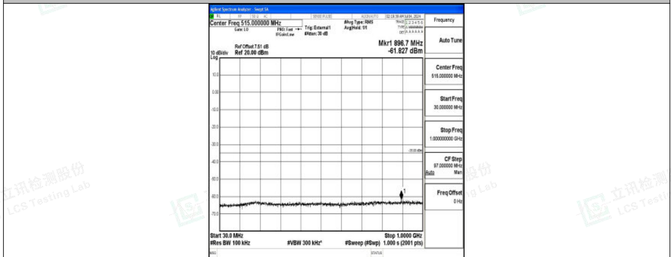
Band41_15MHz_QPSK_40620_1RB#0_30~1000_30~1000
