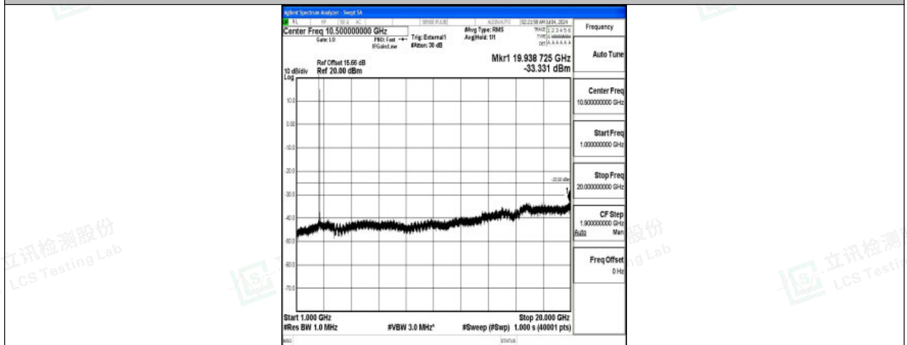
Band41_15MHz_16QAM_40620_1RB#0_1000~20000_1000~20000
