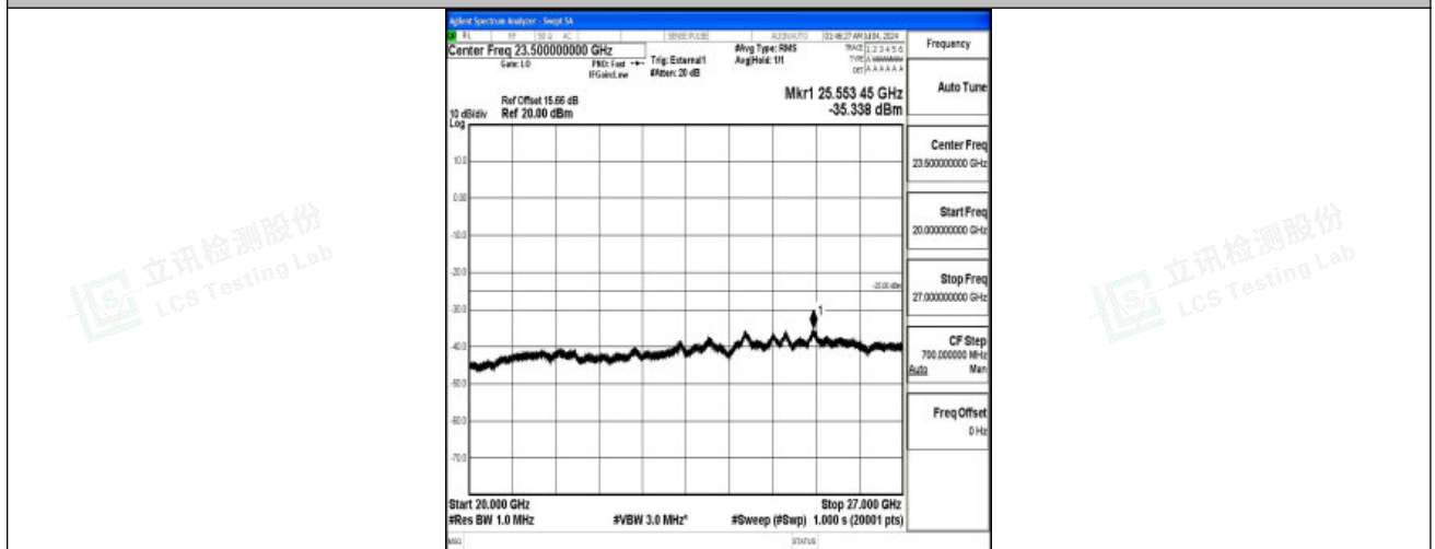
Band41_10MHz_QPSK_39700_1RB#0_20000~27000_20000~27000
