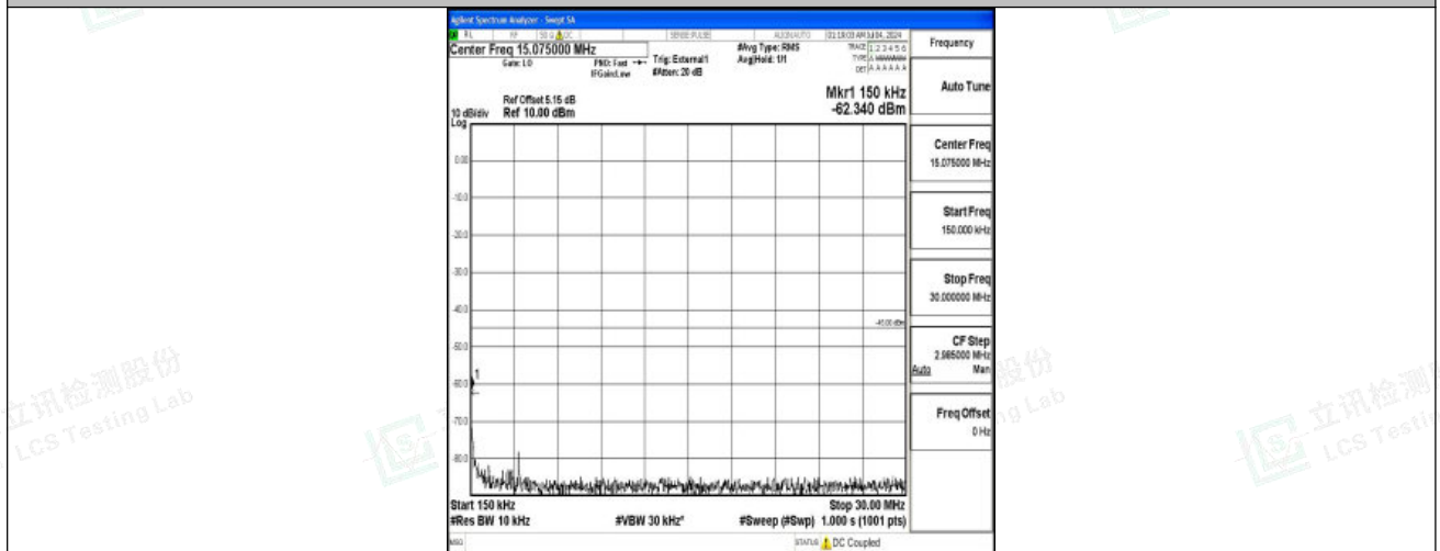
Band41_5MHz_QPSK_41565_1RB#0_0.15~30_0.15~30
