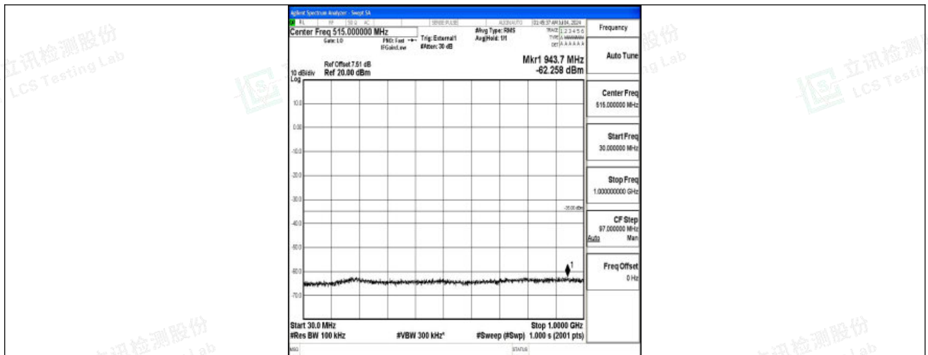
Band41_10MHz_QPSK_39700_1RB#0_30~1000_30~1000
