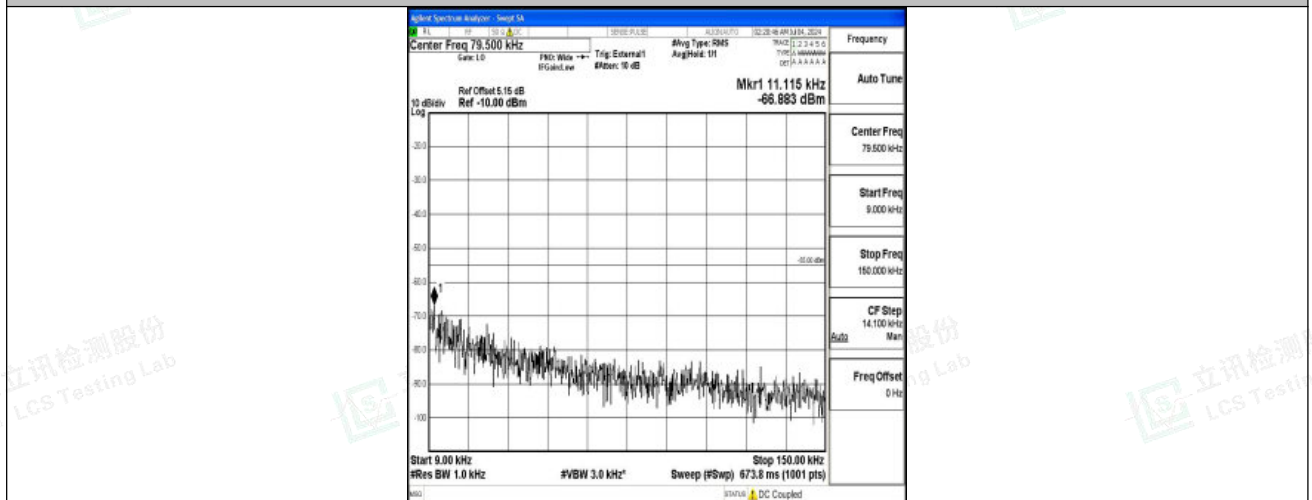
Band41_15MHz_16QAM_40620_1RB#0_0.009~0.15_0.009~0.15
