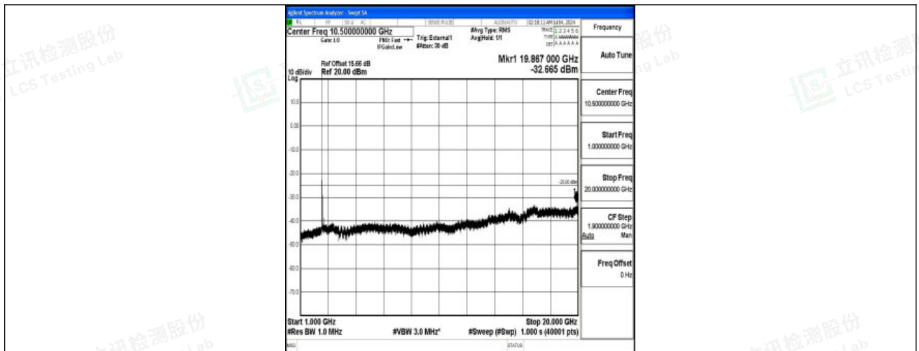
Band41_15MHz_16QAM_39725_1RB#0_1000~20000_1000~20000
