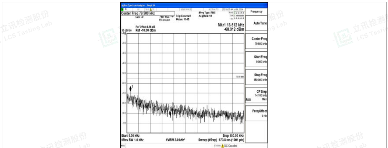
Band41_20MHz_QPSK_41490_1RB#0_0.009~0.15_0.009~0.15
