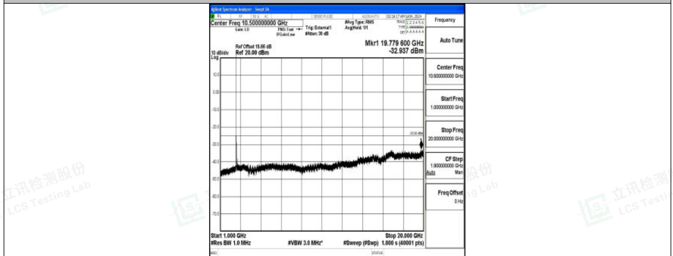
Band41_15MHz_QPSK_39725_1RB#0_1000~20000_1000~20000
