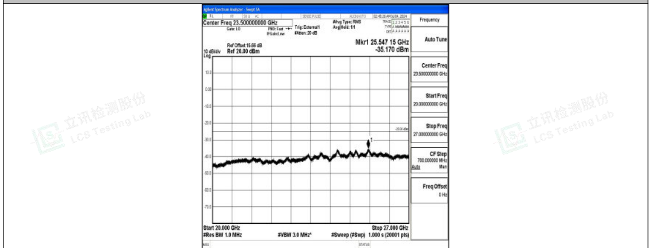
Band41_20MHz_QPSK_39750_1RB#0_20000~27000_20000~27000
