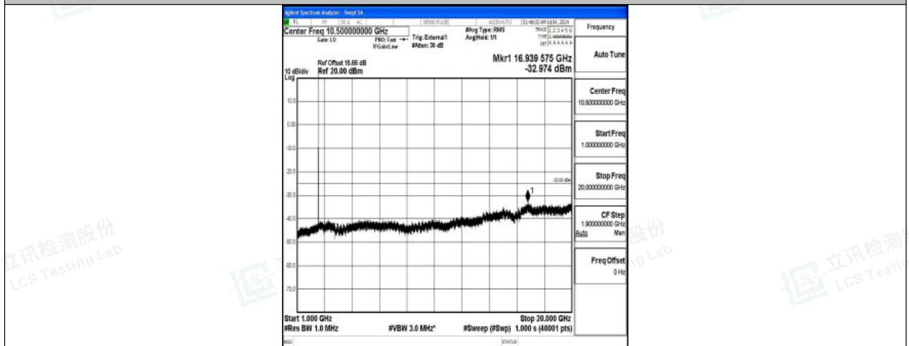
Band41_10MHz_QPSK_39700_1RB#0_1000~20000_1000~20000
