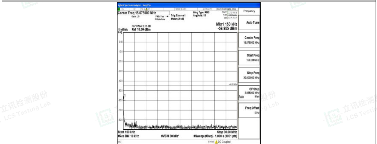
Band41_10MHz_16QAM_39700_1RB#0_0.15~30_0.15~30
