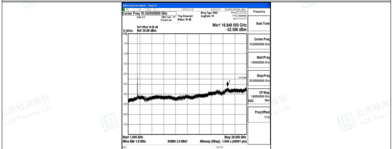
Band41_20MHz_QPSK_39750_1RB#0_1000~20000_1000~20000
