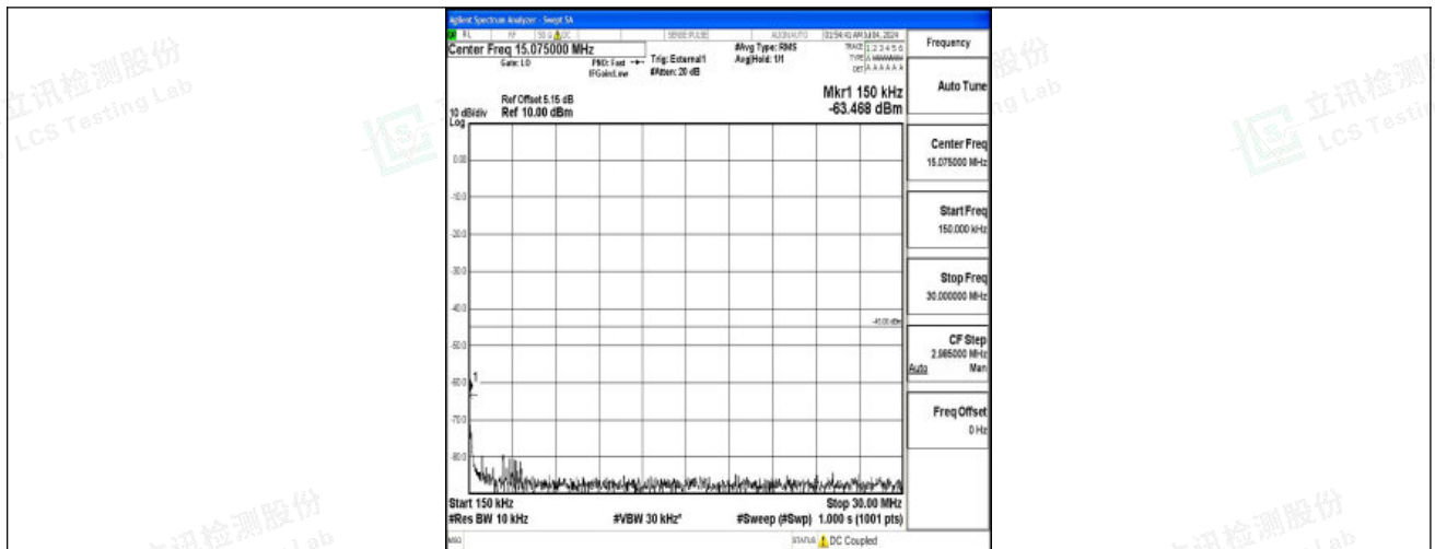
Band41_10MHz_16QAM_41540_1RB#0_0.15~30_0.15~30
