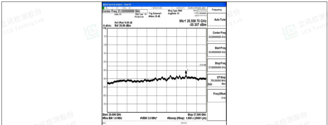
Band41_20MHz_QPSK_40620_1RB#0_20000~27000_20000~27000
