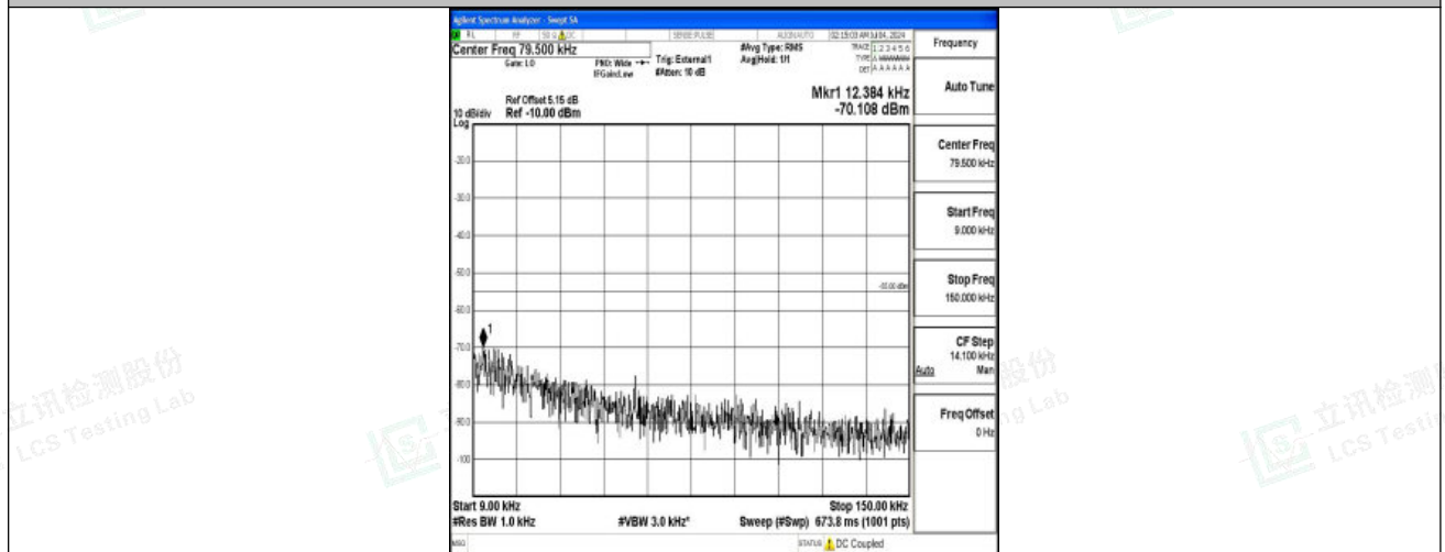
Band41_15MHz_QPSK_39725_1RB#0_0.009~0.15_0.009~0.15
