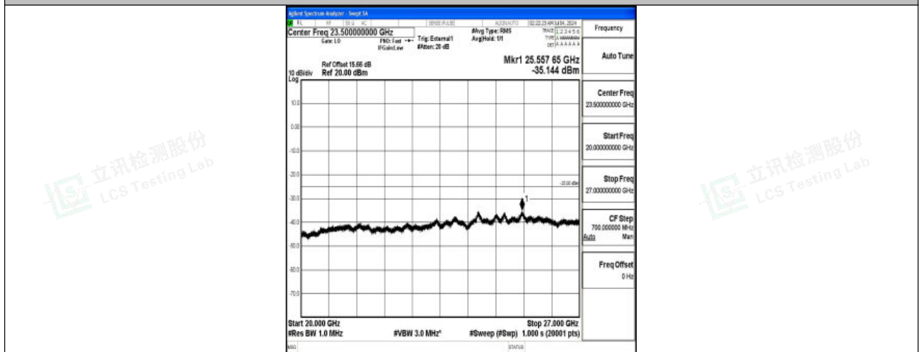
Band41_15MHz_16QAM_40620_1RB#0_20000~27000_20000~27000
