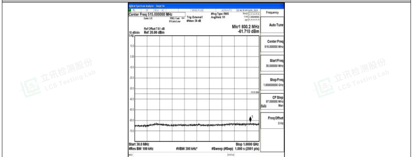
Band41_20MHz_16QAM_39750_1RB#0_30~1000_30~1000
