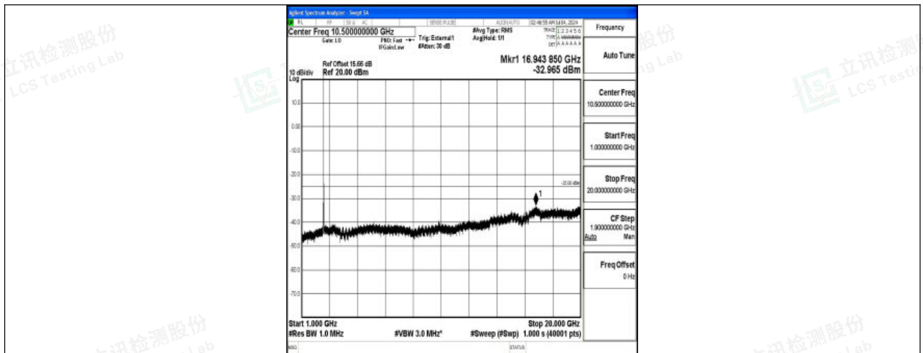
Band41_20MHz_16QAM_39750_1RB#0_1000~20000_1000~20000
