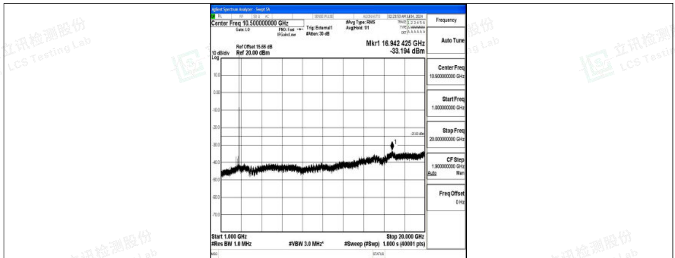
Band41_15MHz_QPSK_41515_1RB#0_1000~20000_1000~20000
