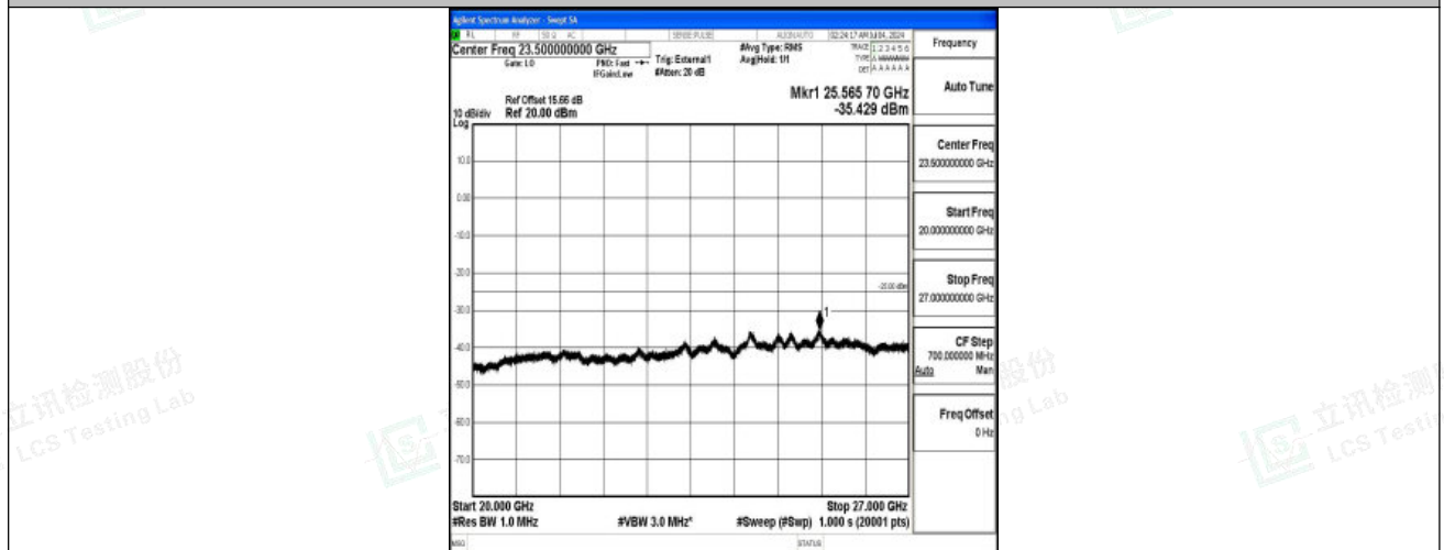
Band41_15MHz_QPSK_41515_1RB#0_20000~27000_20000~27000
