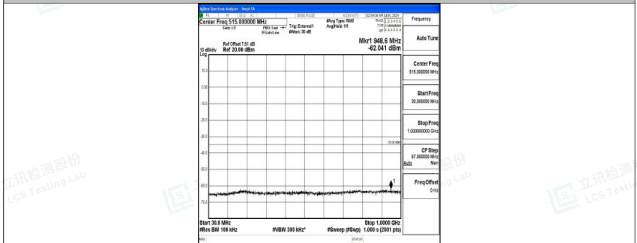
Band41_20MHz_16QAM_41490_1RB#0_30~1000_30~1000
