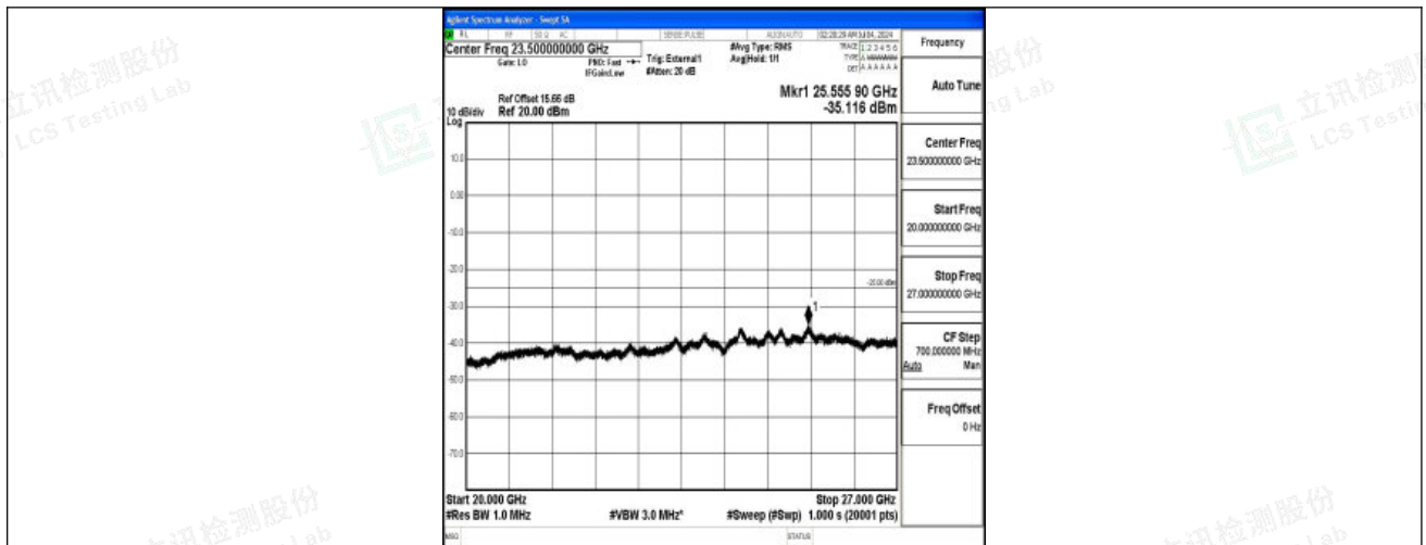
Band41_15MHz_QPSK_40620_1RB#0_20000~27000_20000~27000
