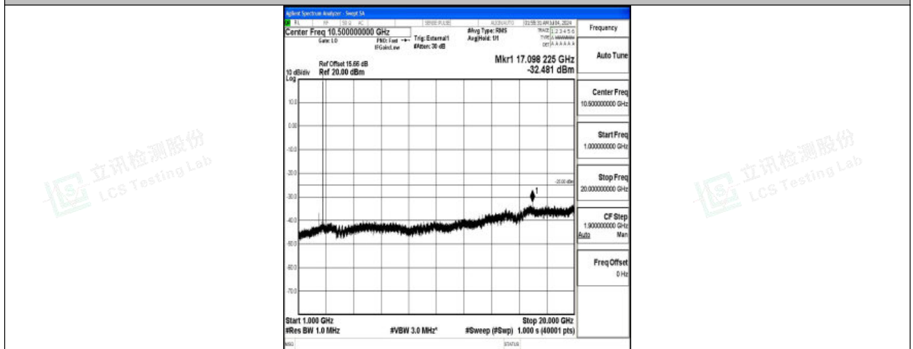
Band41_10MHz_16QAM_41540_1RB#0_1000~20000_1000~20000
