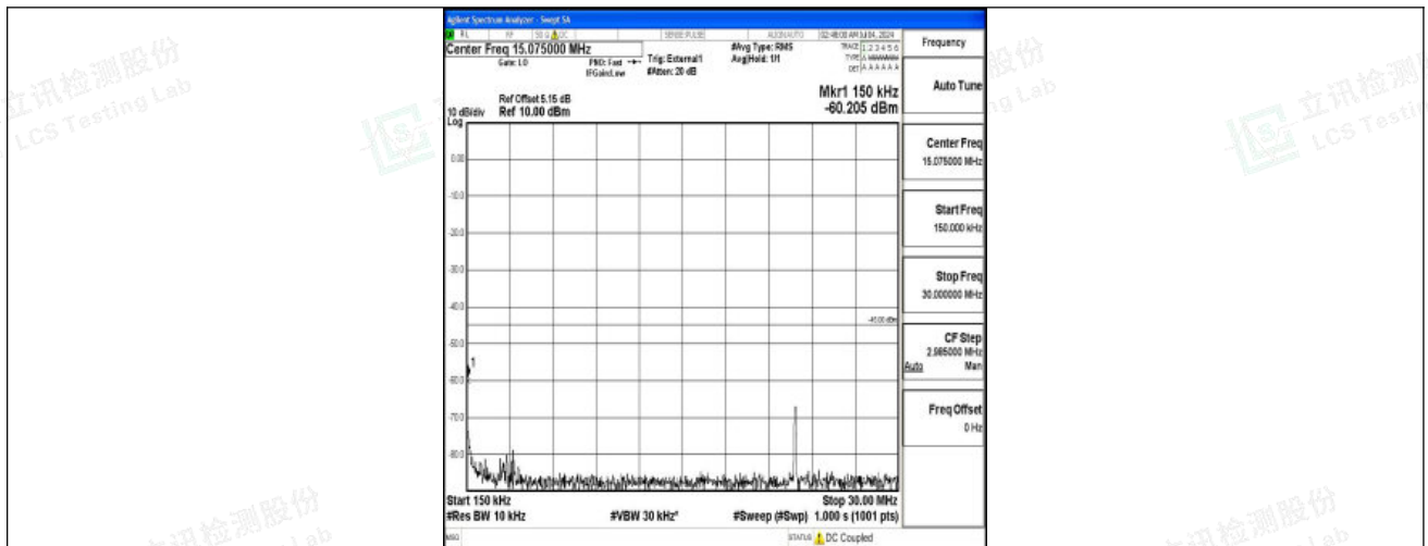
Band41_20MHz_QPSK_40620_1RB#0_0.15~30_0.15~30
