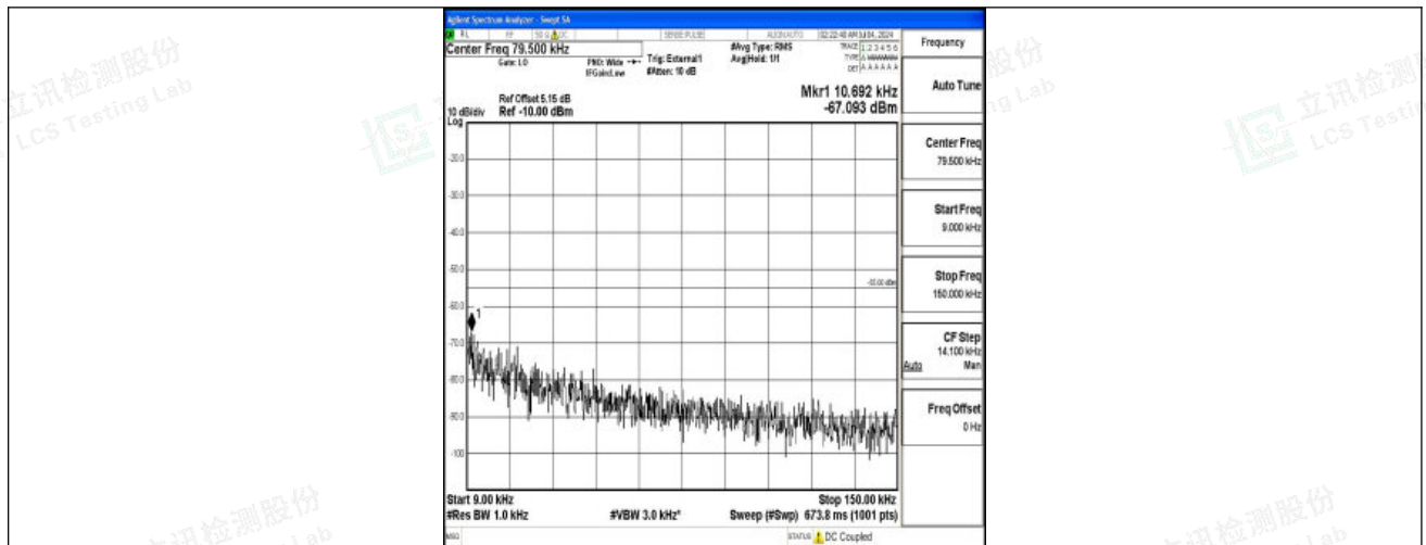
Band41_15MHz_QPSK_41515_1RB#0_0.009~0.15_0.009~0.15
