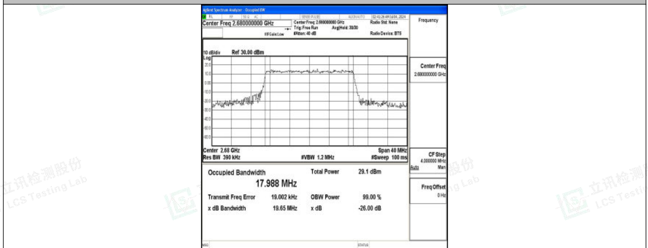
Band41-20MHz-QPSK-41490-100RB#0-PASS
