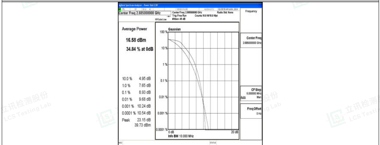
Band41-10MHz-QPSK-41540-50RB#0-PASS
