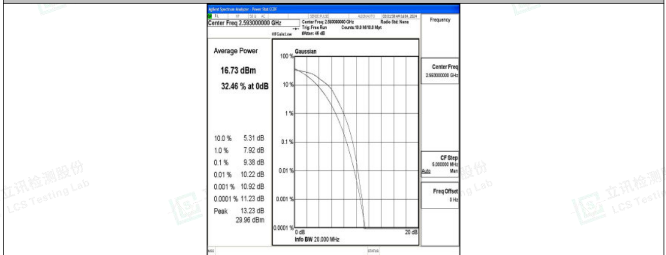
Band41-20MHz-16QAM-40620-100RB#0-PASS
