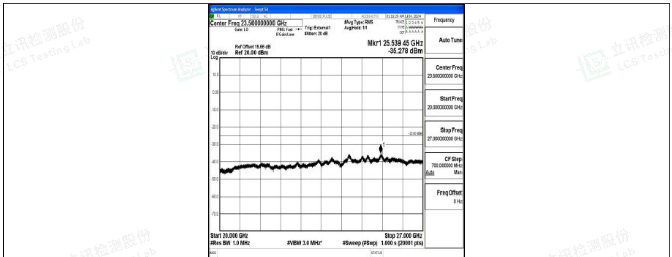
Band41_5MHz_QPSK_40620_1RB#0_20000~27000_20000~27000
