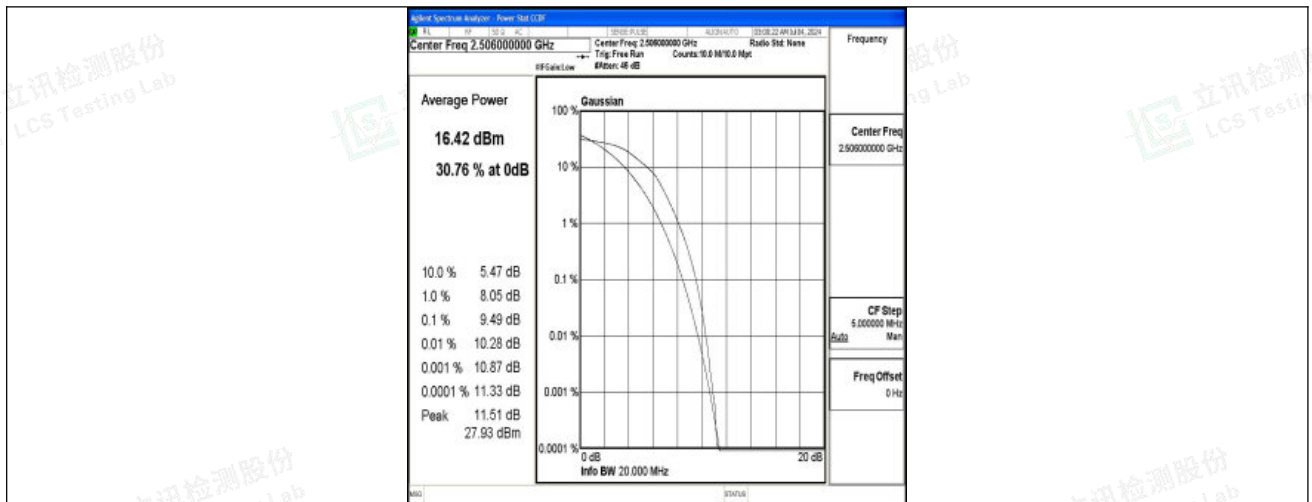
Band41-20MHz-16QAM-39750-100RB#0-PASS
