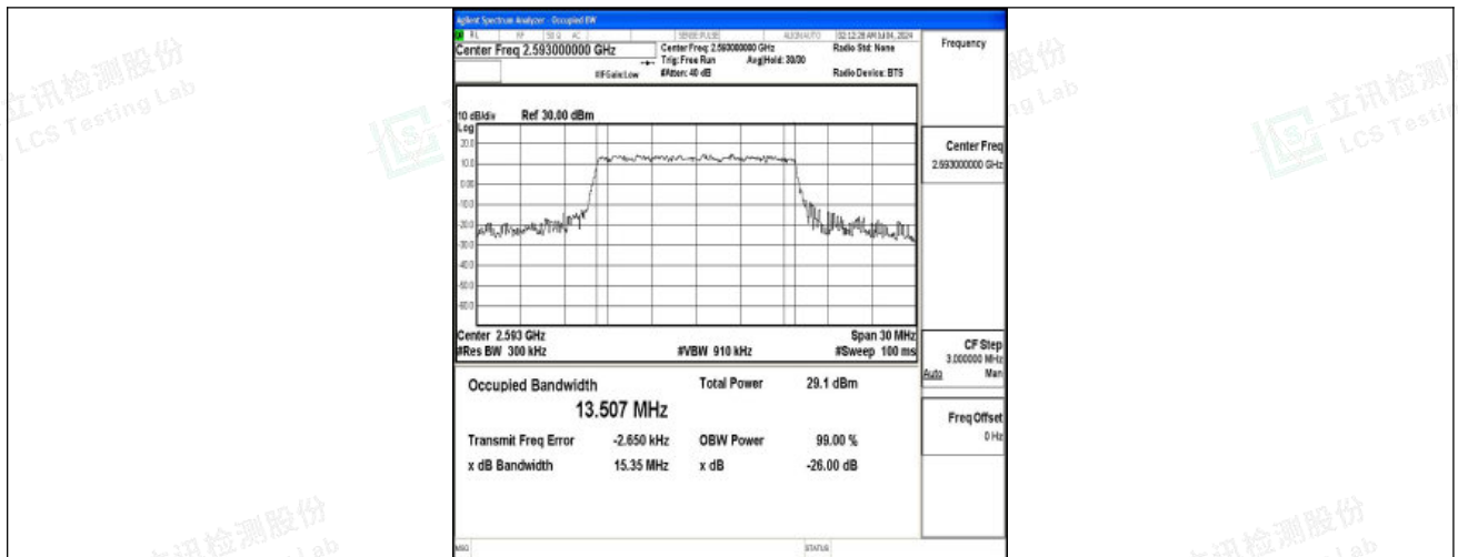
Band41-15MHz-16QAM-40620-75RB#0-PASS
