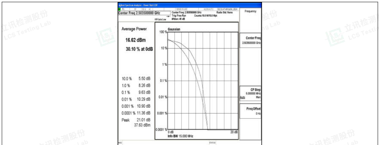
Band41-15MHz-16QAM-39725-75RB#0-PASS
