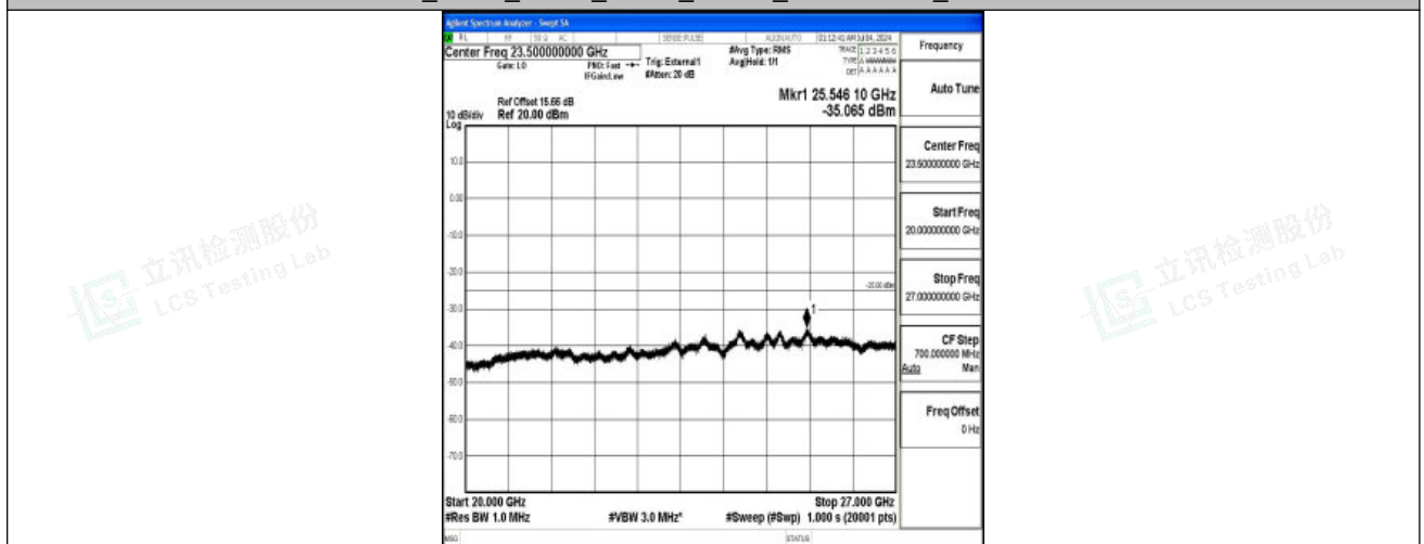
Band41_5MHz_QPSK_39675_1RB#0_20000~27000_20000~27000
