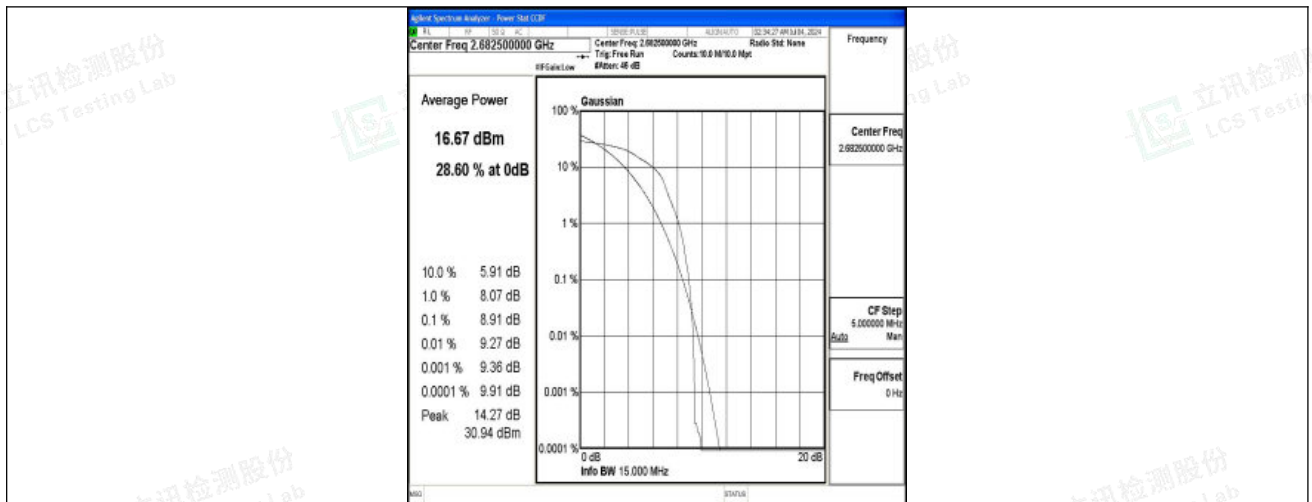
Band41-15MHz-16QAM-41515-1RB#0-PASS
