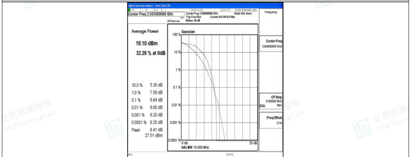
Band41-15MHz-QPSK-40620-1RB#0-PASS
