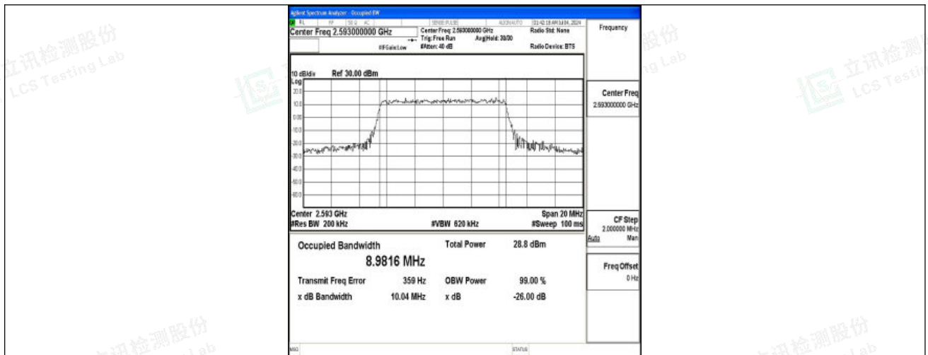
Band41-10MHz-16QAM-40620-50RB#0-PASS
