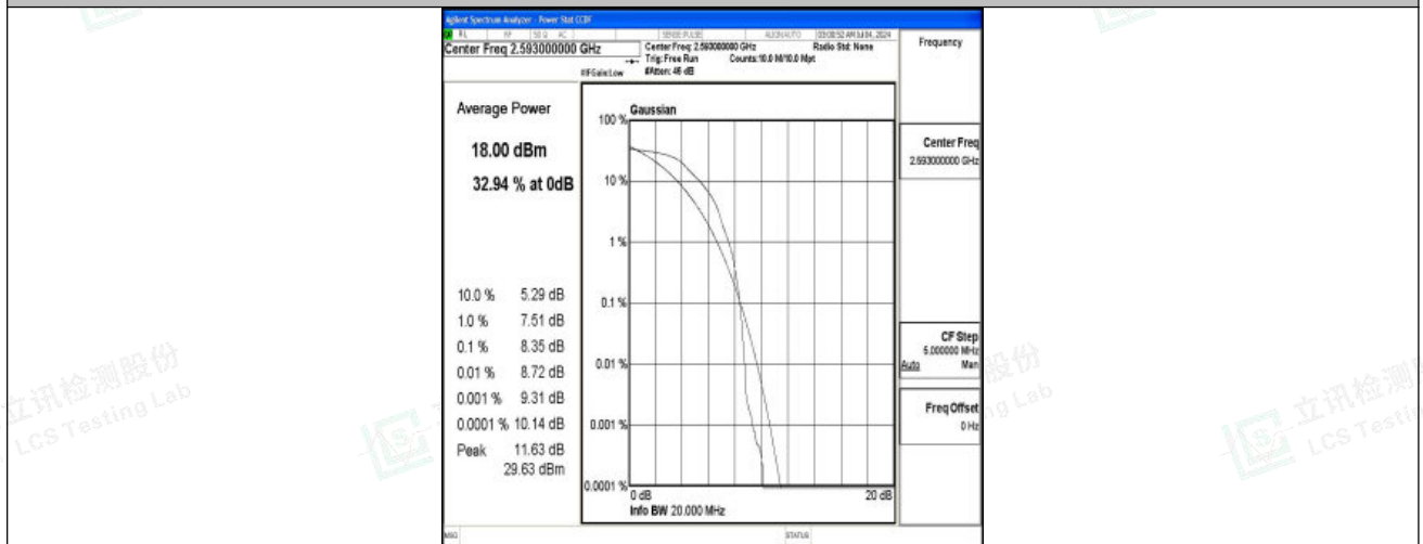
Band41-20MHz-QPSK-40620-1RB#0-PASS
