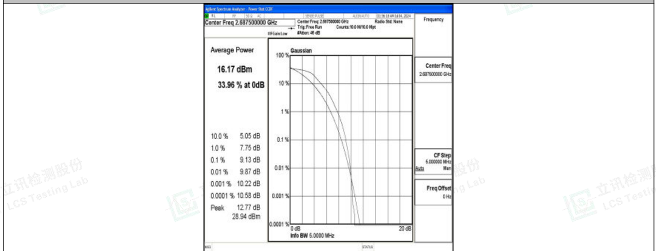
Band41-5MHz-QPSK-41565-25RB#0-PASS
