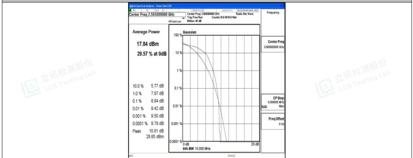
Band41-10MHz-16QAM-40620-1RB#0-PASS
