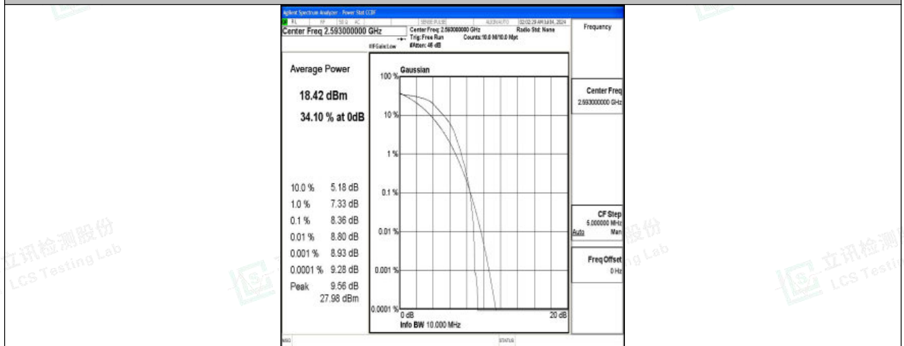
Band41-10MHz-QPSK-40620-1RB#0-PASS
