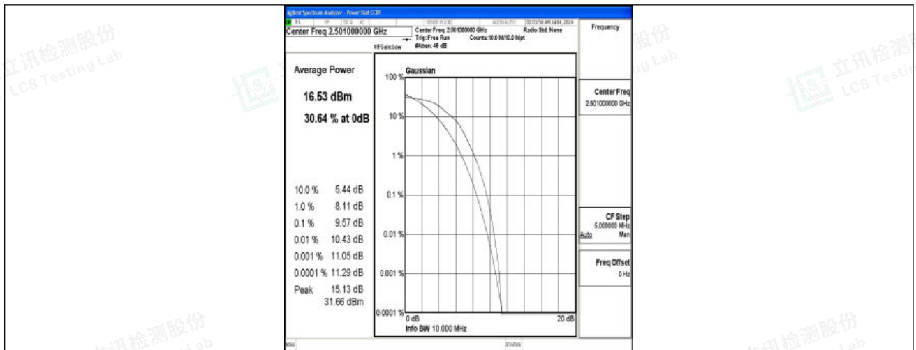
Band41-10MHz-16QAM-39700-50RB#0-PASS
