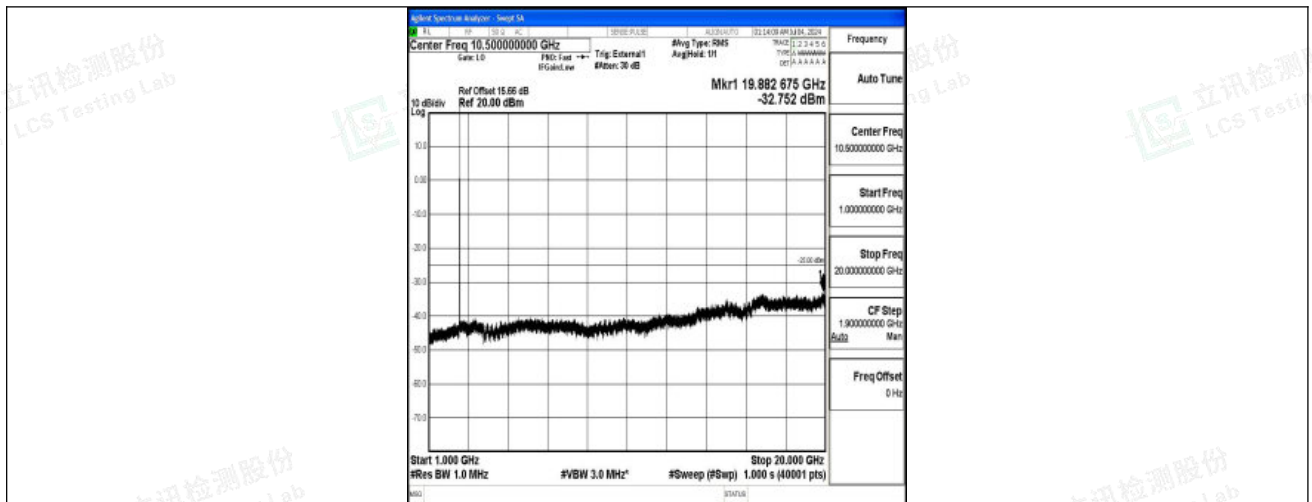
Band41_5MHz_16QAM_39675_1RB#0_1000~20000_1000~20000
