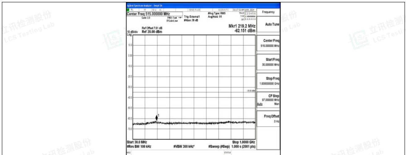
Band41_5MHz_16QAM_40620_1RB#0_30~1000_30~1000
