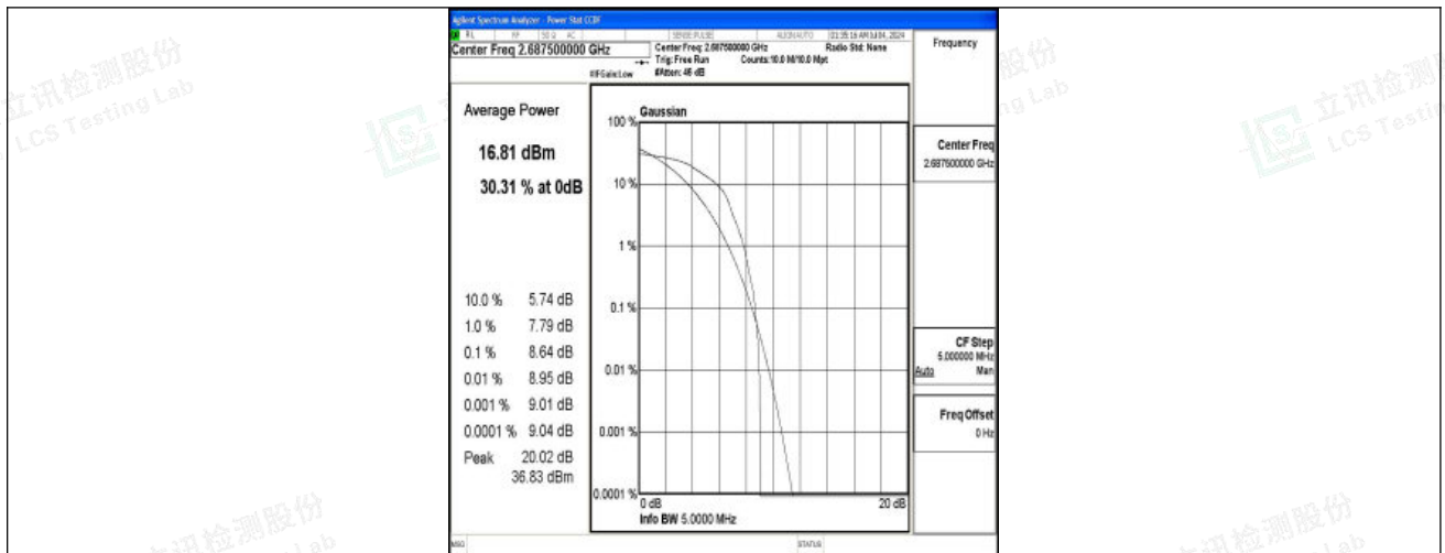
Band41-5MHz-16QAM-41565-1RB#0-PASS
