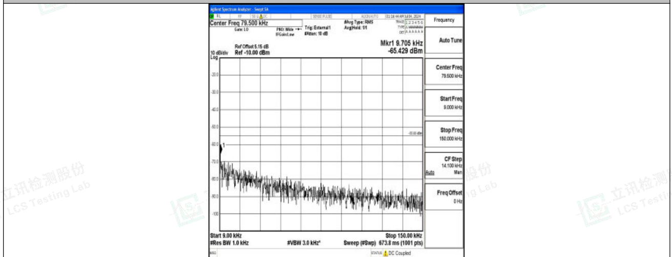
Band41_5MHz_16QAM_40620_1RB#0_0.009~0.15_0.009~0.15
