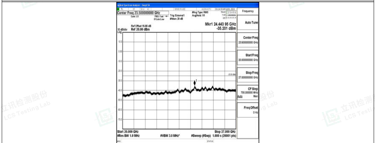
Band41_5MHz_16QAM_39675_1RB#0_20000~27000_20000~27000
