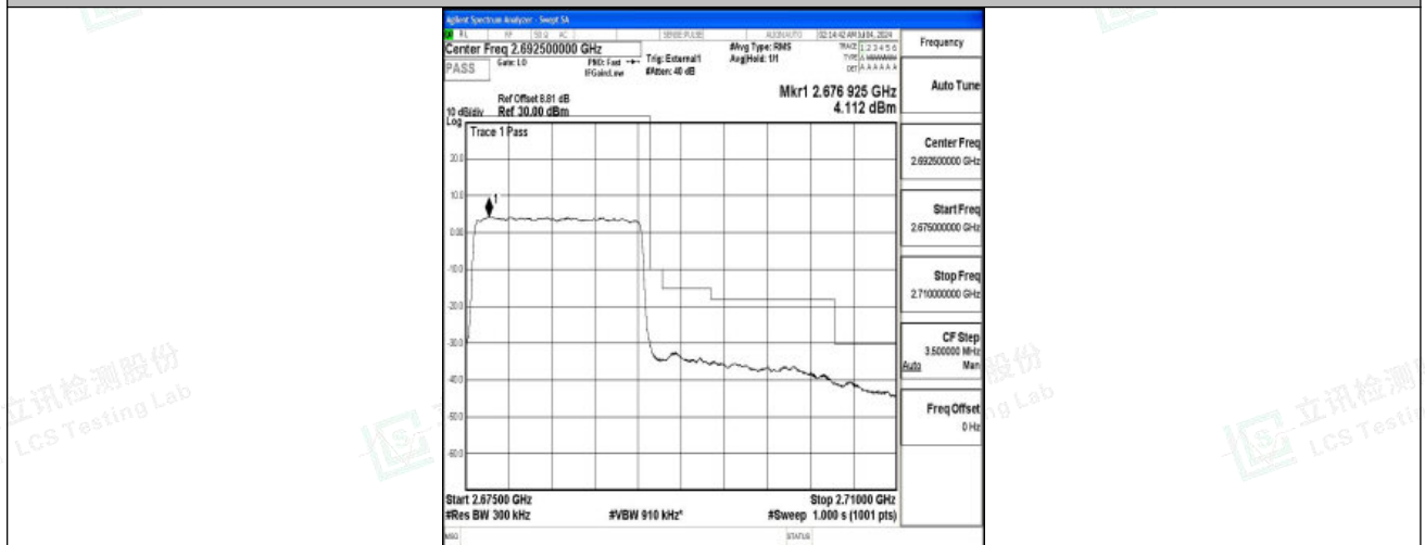
Band41_15MHz_16QAM_41515_75RB#0
