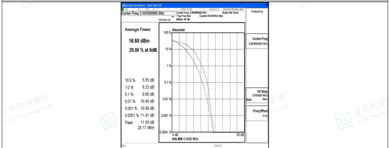
Band41-5MHz-16QAM-40620-25RB#0-PASS
