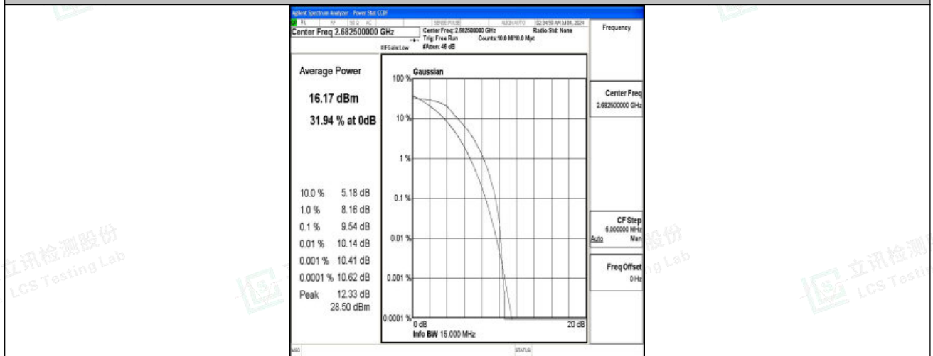
Band41-15MHz-QPSK-41515-75RB#0-PASS
