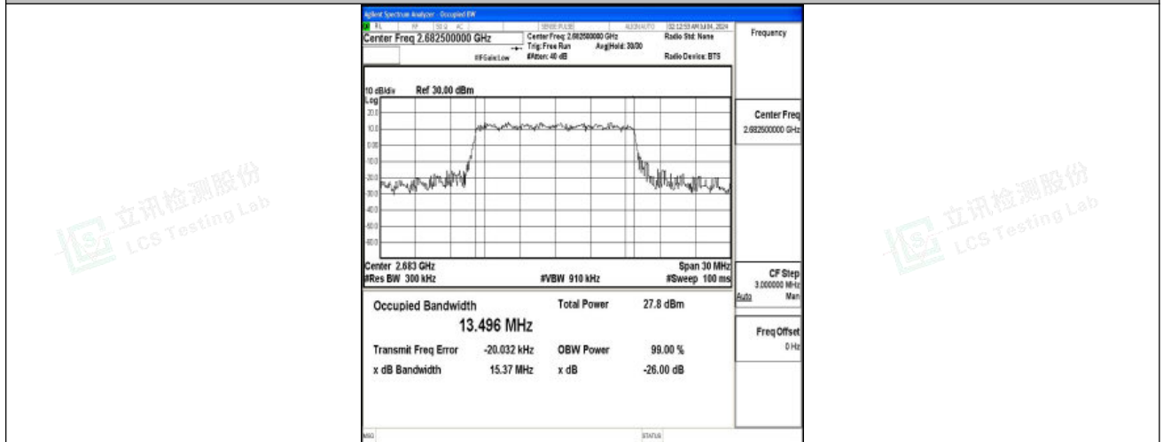
Band41-15MHz-16QAM-41515-75RB#0-PASS
