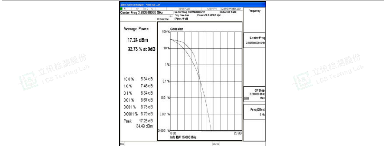
Band41-15MHz-QPSK-41515-1RB#0-PASS
