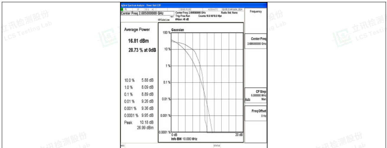
Band41-10MHz-16QAM-41540-1RB#0-PASS
