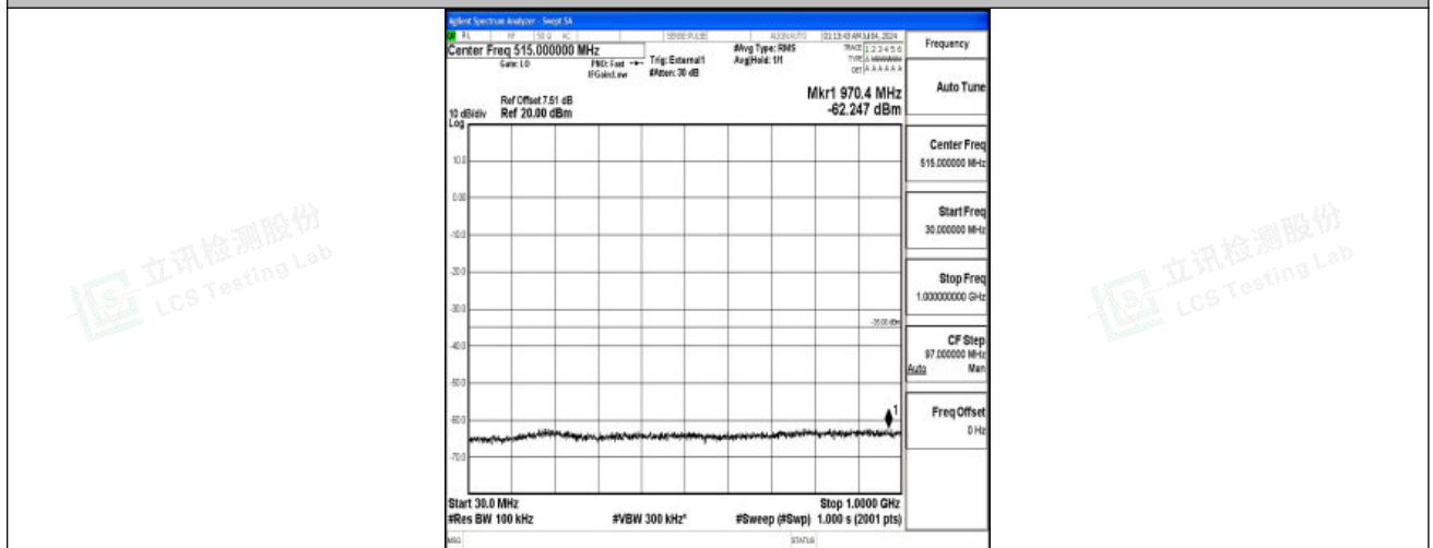
Band41_5MHz_16QAM_39675_1RB#0_30~1000_30~1000
