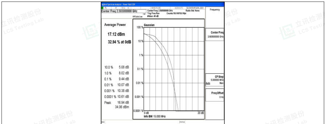
Band41-15MHz-QPSK-40620-75RB#0-PASS
