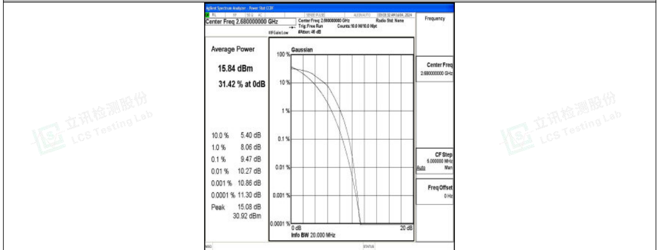
Band41-20MHz-16QAM-41490-100RB#0-PASS
