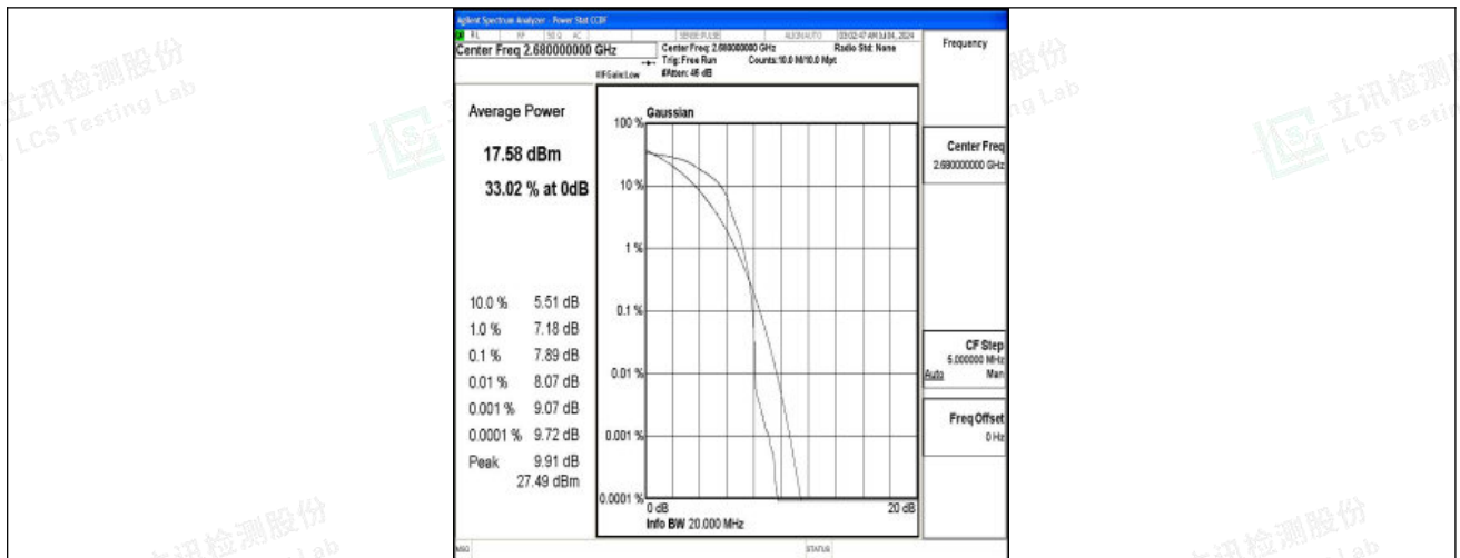
Band41-20MHz-16QAM-41490-1RB#0-PASS
