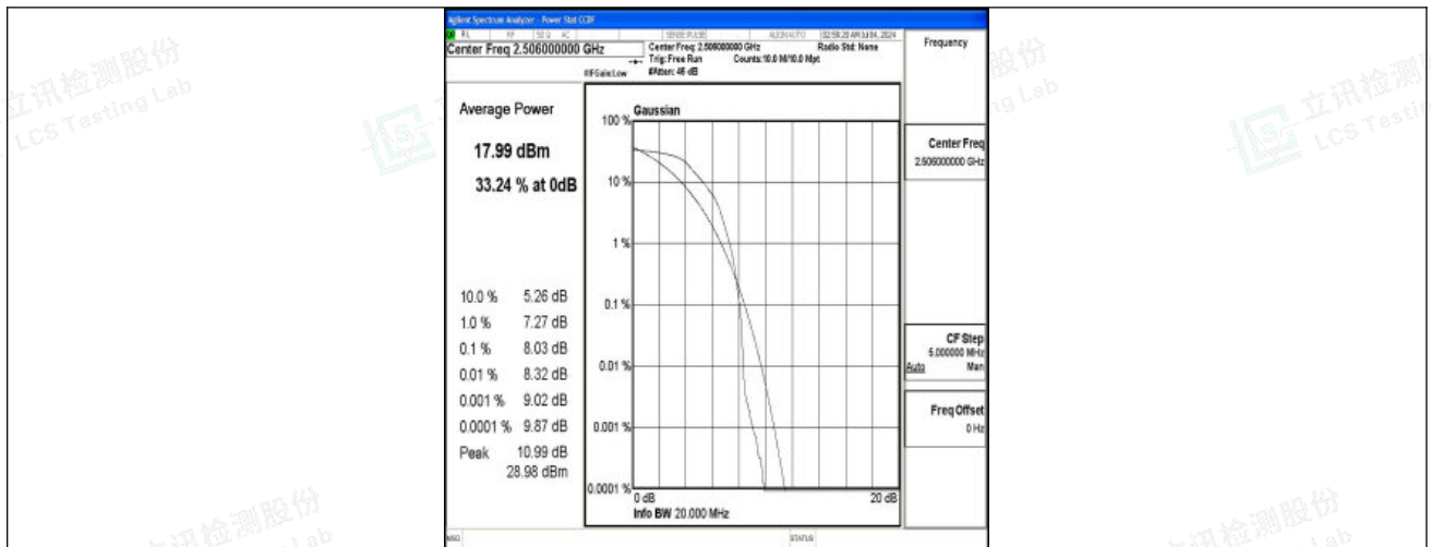
Band41-20MHz-QPSK-39750-1RB#0-PASS
