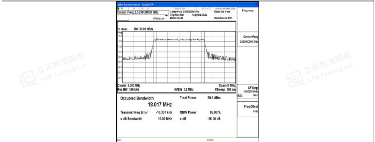
Band41-20MHz-QPSK-40620-100RB#0-PASS
