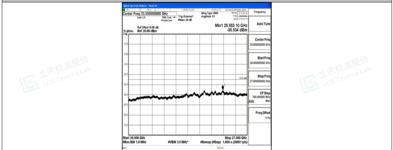
Band41_5MHz_16QAM_40620_1RB#0_20000~27000_20000~27000
