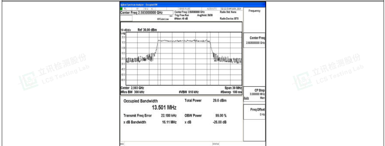
Band41-15MHz-QPSK-40620-75RB#0-PASS
