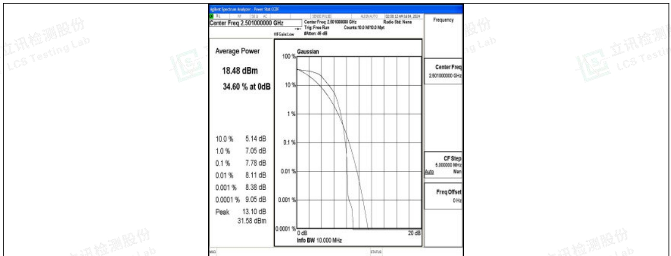
Band41-10MHz-QPSK-39700-1RB#0-PASS
