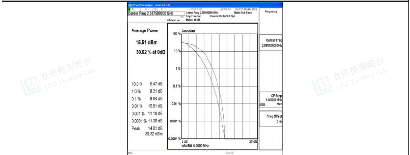
Band41-5MHz-16QAM-41565-25RB#0-PASS
