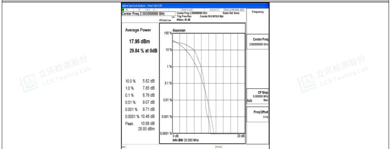
Band41-20MHz-16QAM-40620-1RB#0-PASS
