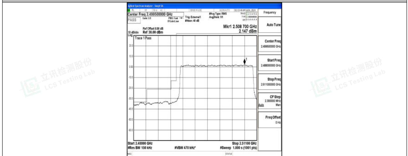
Band41_15MHz_16QAM_39725_75RB#0
