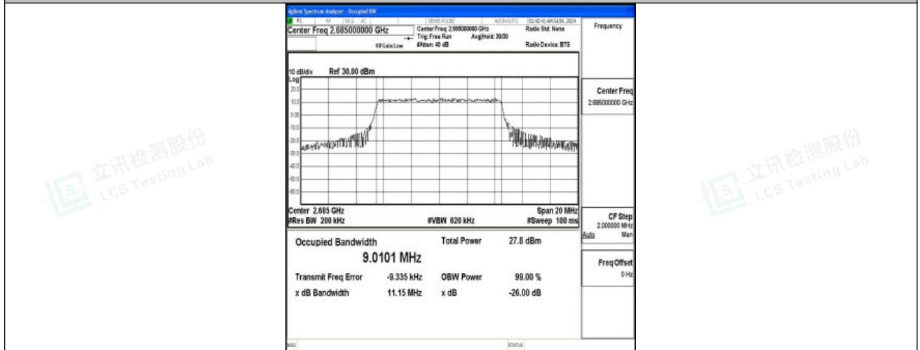
Band41-10MHz-16QAM-41540-50RB#0-PASS
