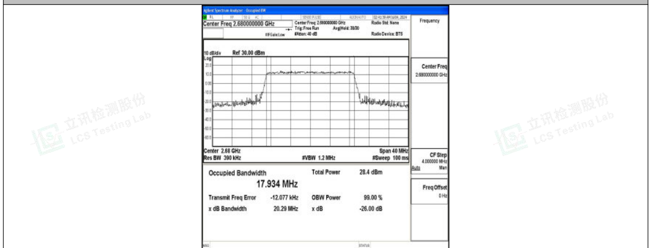
Band41-20MHz-16QAM-41490-100RB#0-PASS
