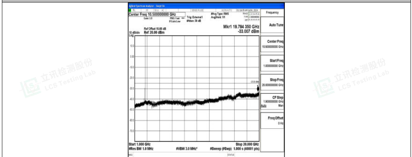
Band41_5MHz_QPSK_40620_1RB#0_1000~20000_1000~20000
