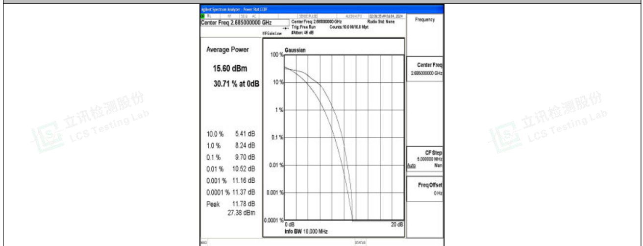
Band41-10MHz-16QAM-41540-50RB#0-PASS
