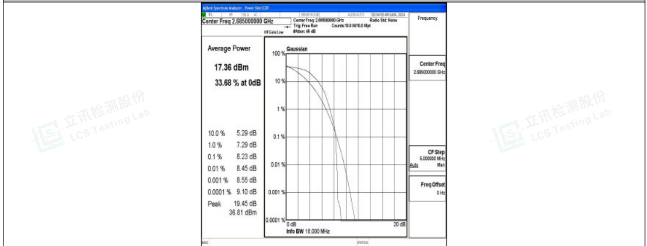
Band41-10MHz-QPSK-41540-1RB#0-PASS
