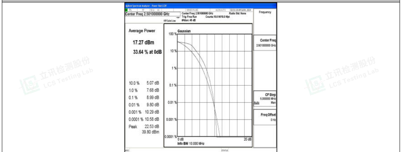
Band41-10MHz-QPSK-39700-50RB#0-PASS
