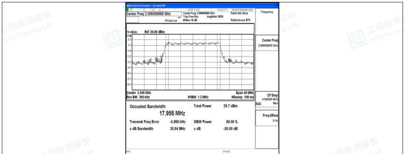
Band41-20MHz-QPSK-39750-100RB#0-PASS
