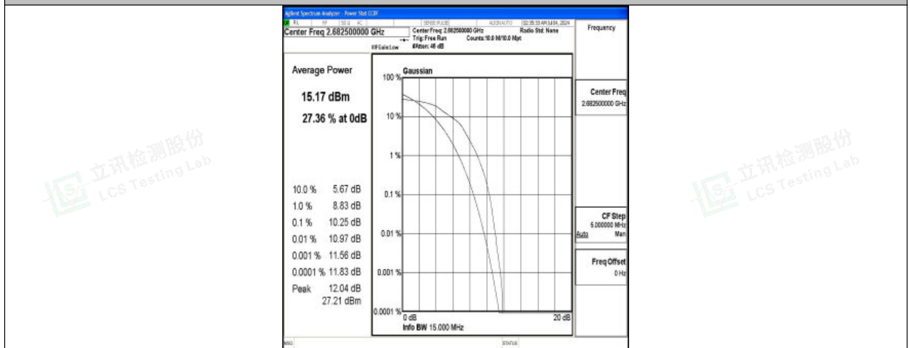
Band41-15MHz-16QAM-41515-75RB#0-PASS
