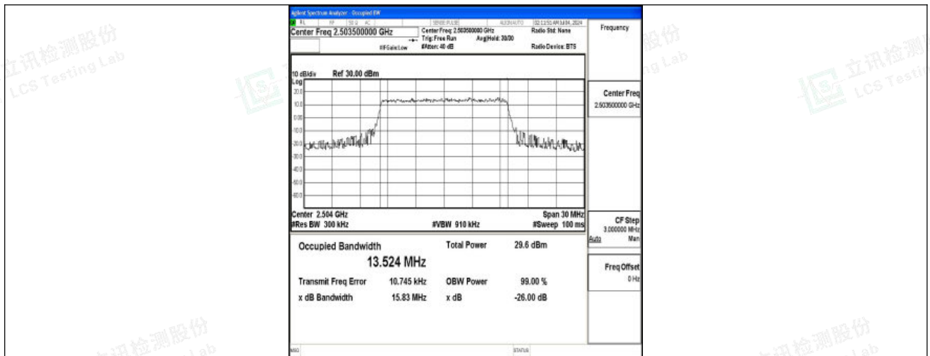
Band41-15MHz-QPSK-39725-75RB#0-PASS
