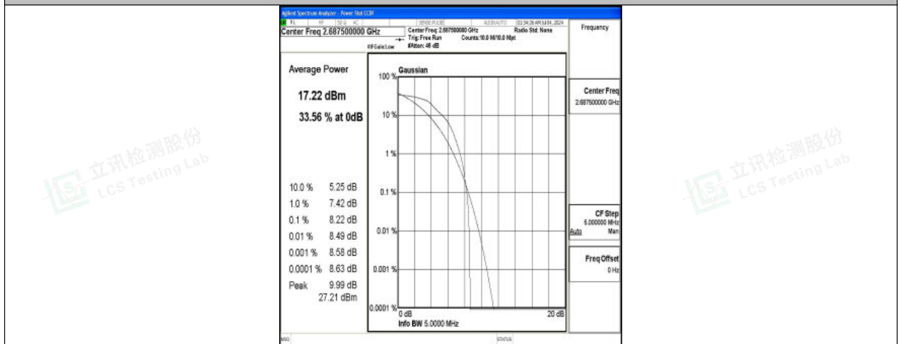
Band41-5MHz-QPSK-41565-1RB#0-PASS
