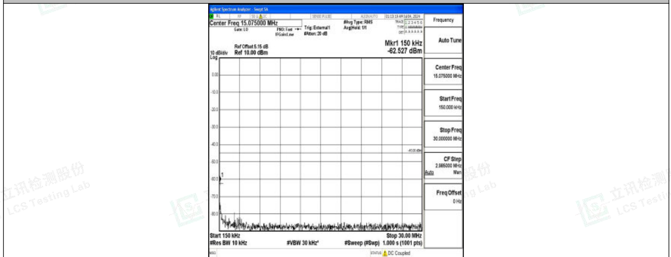
Band41_5MHz_16QAM_39675_1RB#0_0.15~30_0.15~30
