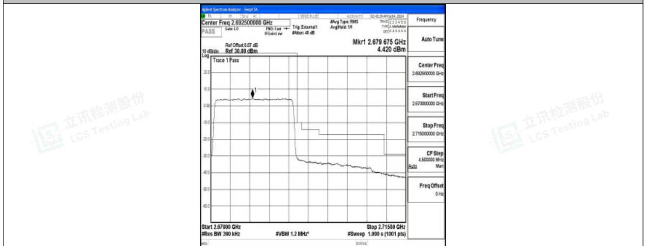
Band41_20MHz_16QAM_41490_100RB#0
