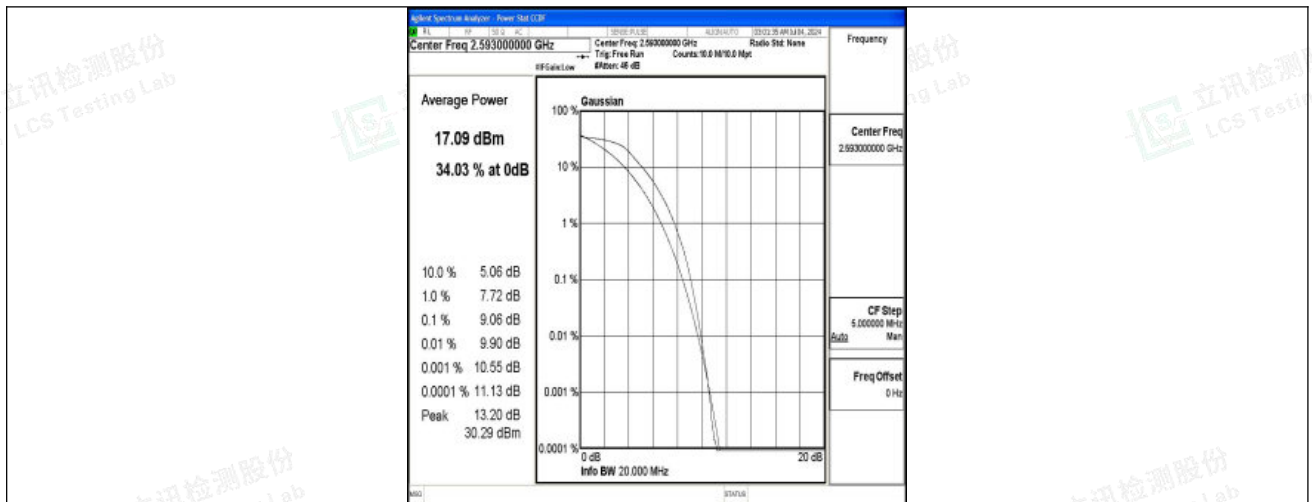
Band41-20MHz-QPSK-40620-100RB#0-PASS
