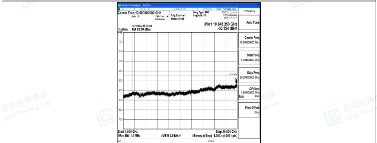
Band41_5MHz_QPSK_39675_1RB#0_1000~20000_1000~20000
