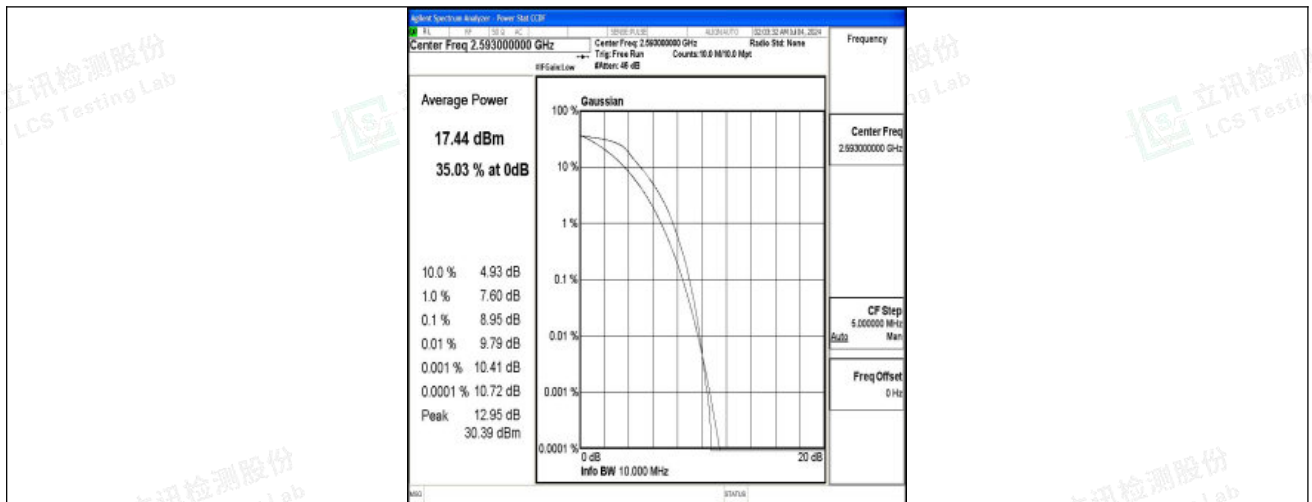
Band41-10MHz-QPSK-40620-50RB#0-PASS
