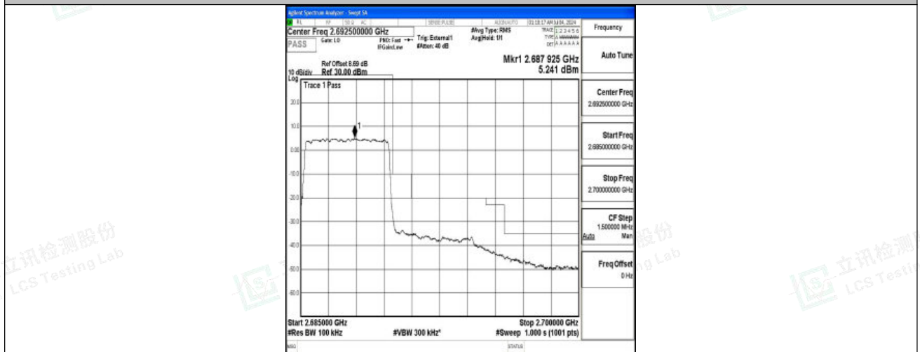
Band41_5MHz_QPSK_41565_25RB#0
