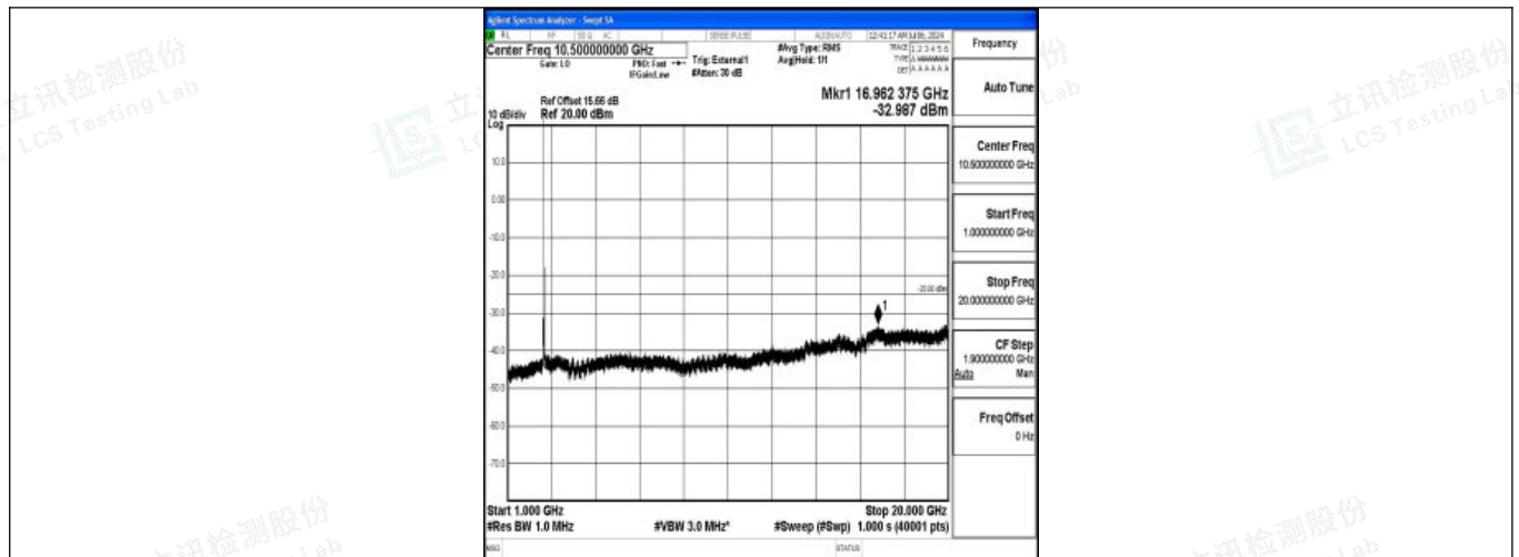
Band38_20MHz_16QAM_37850_1RB#0_1000~20000_1000~20000
