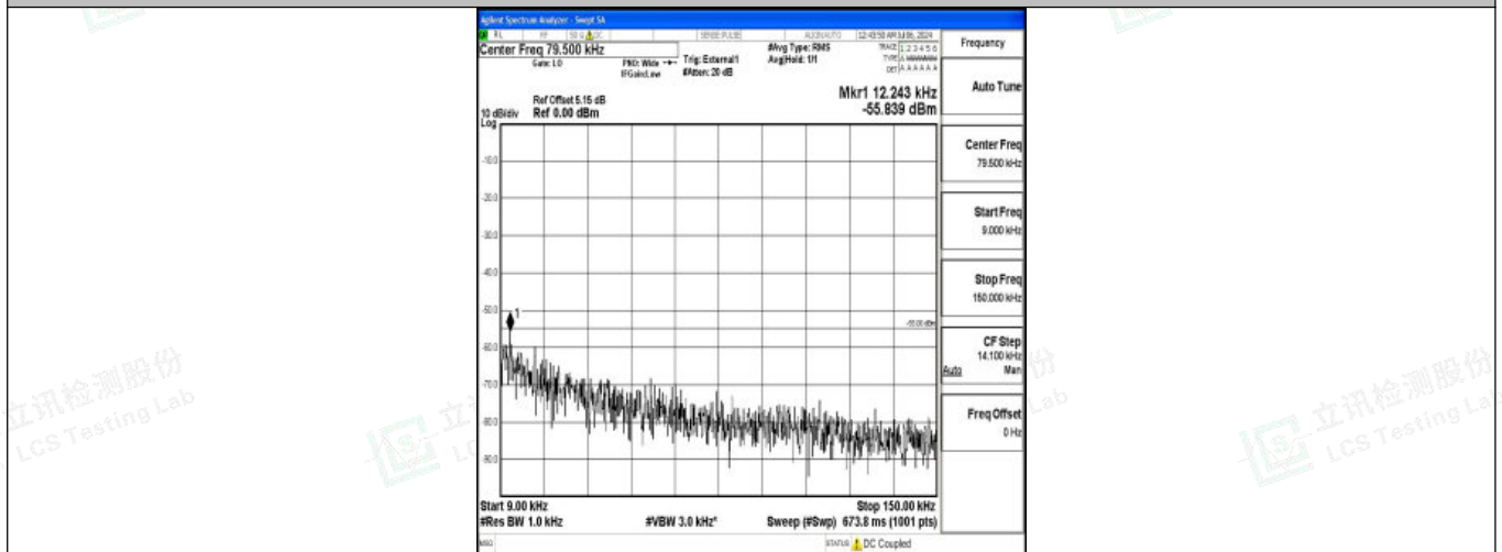
Band38_20MHz_16QAM_38000_1RB#0_0.009~0.15_0.009~0.15
