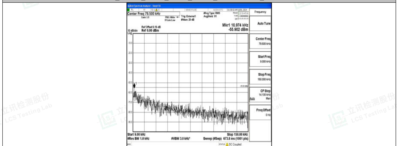
Band38_15MHz_16QAM_38000_1RB#0_0.009~0.15_0.009~0.15
