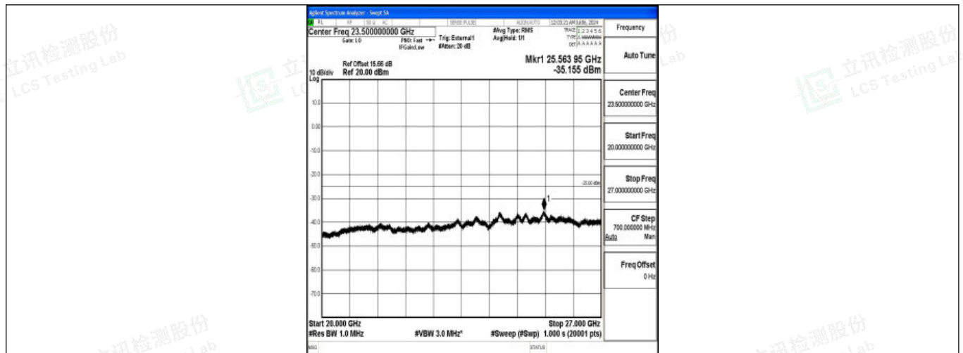
Band38_10MHz_16QAM_38200_1RB#0_20000~27000_20000~27000
