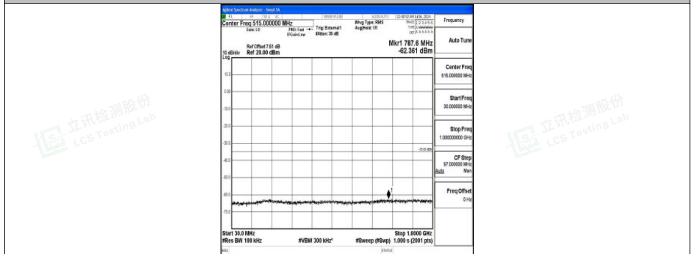
Band38_20MHz_16QAM_37850_1RB#0_30~1000_30~1000
