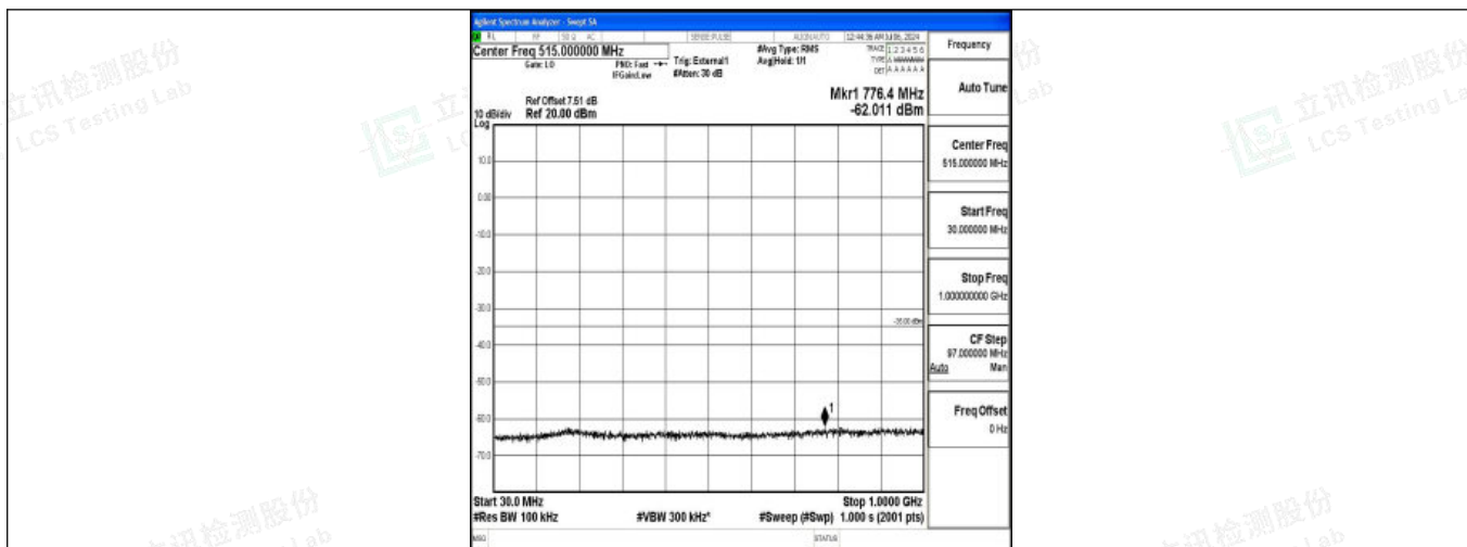
Band38_20MHz_16QAM_38000_1RB#0_30~1000_30~1000
