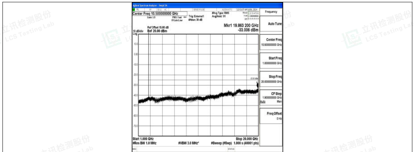
Band38_10MHz_QPSK_38200_1RB#0_1000~20000_1000~20000
