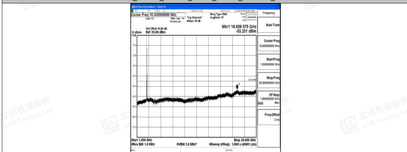
Band38_20MHz_16QAM_38000_1RB#0_1000~20000_1000~20000
