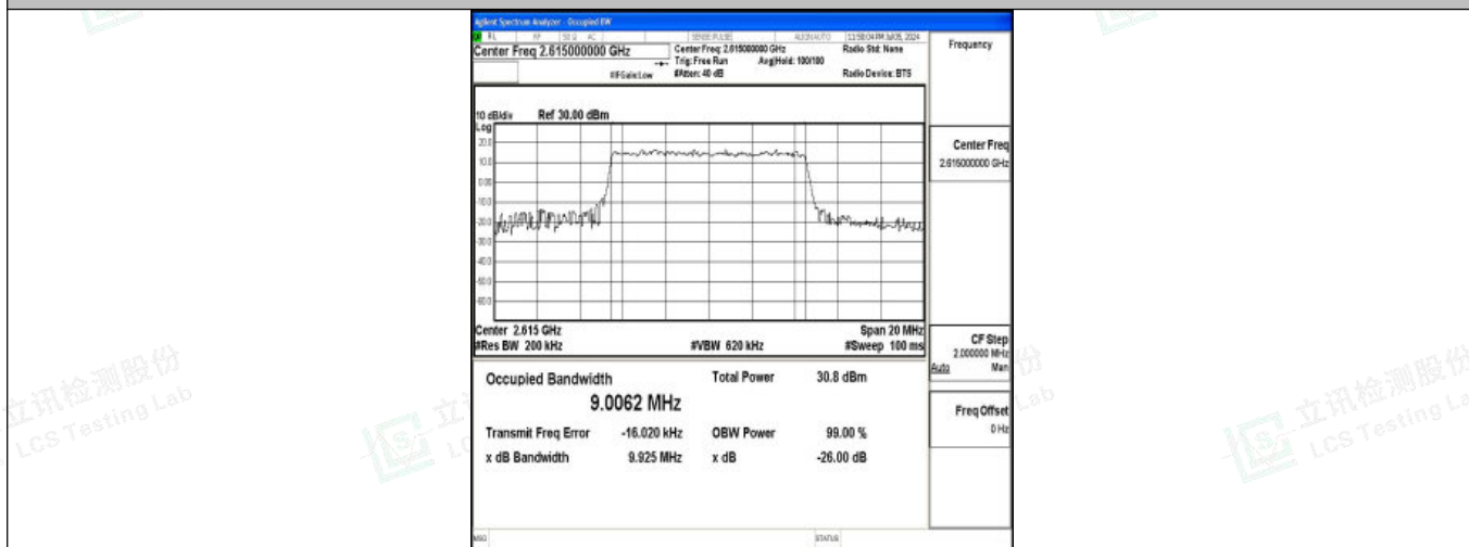
Band38-10MHz-QPSK-38200-50RB#0-PASS
