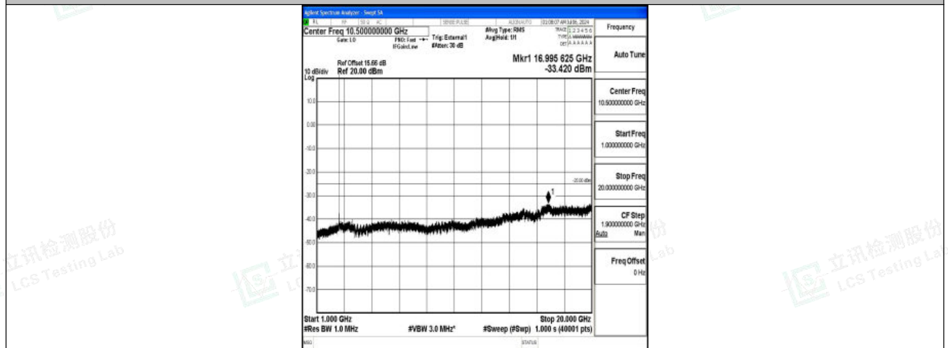
Band38_5MHz_QPSK_37775_1RB#0_1000~20000_1000~20000
