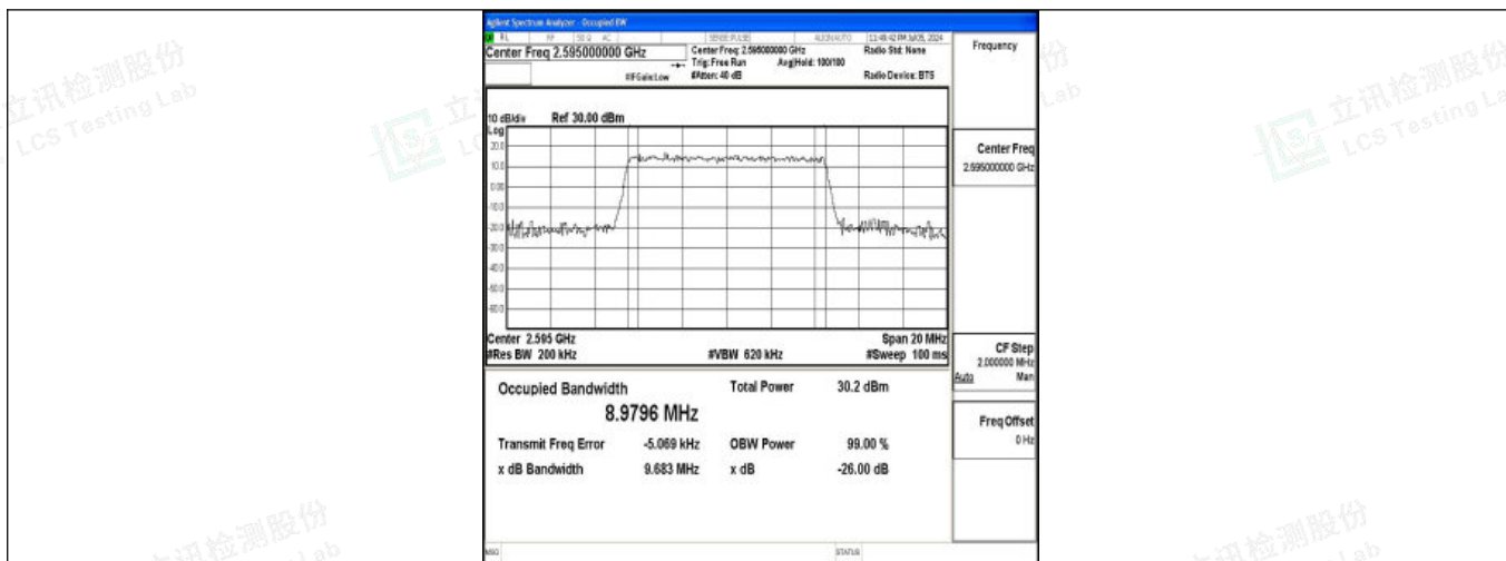
Band38-10MHz-16QAM-38000-50RB#0-PASS
