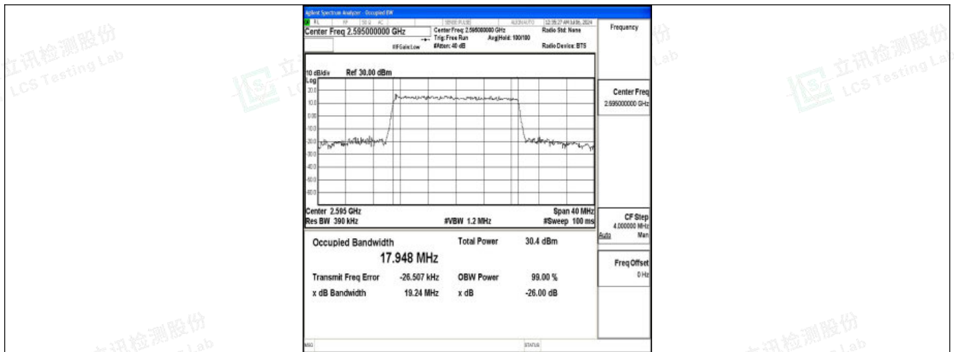
Band38-20MHz-16QAM-38000-100RB#0-PASS
