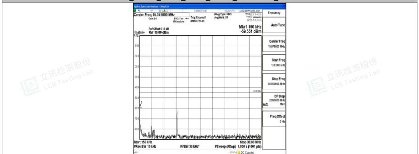
Band38_10MHz_QPSK_37800_1RB#0_0.15~30_0.15~30
