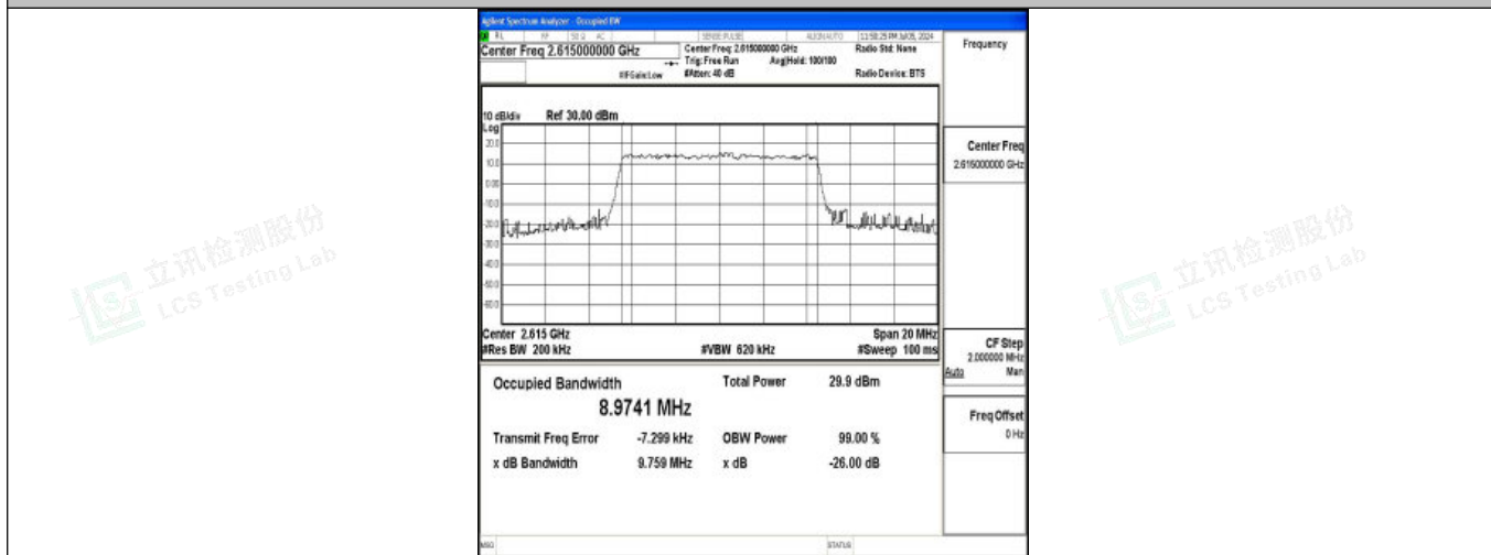
Band38-10MHz-16QAM-38200-50RB#0-PASS
