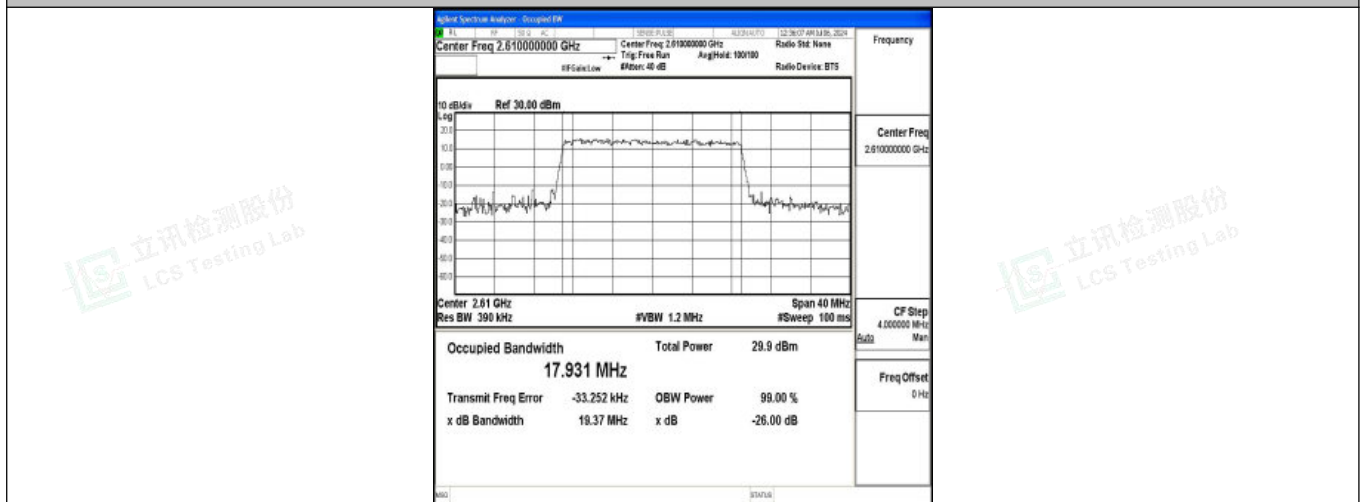
Band38-20MHz-16QAM-38150-100RB#0-PASS
