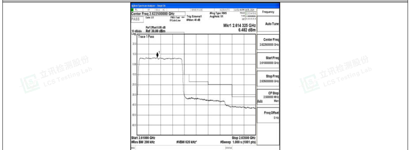
Band38_10MHz_QPSK_38200_50RB#0
