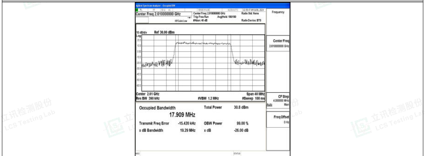
Band38-20MHz-QPSK-38150-100RB#0-PASS
