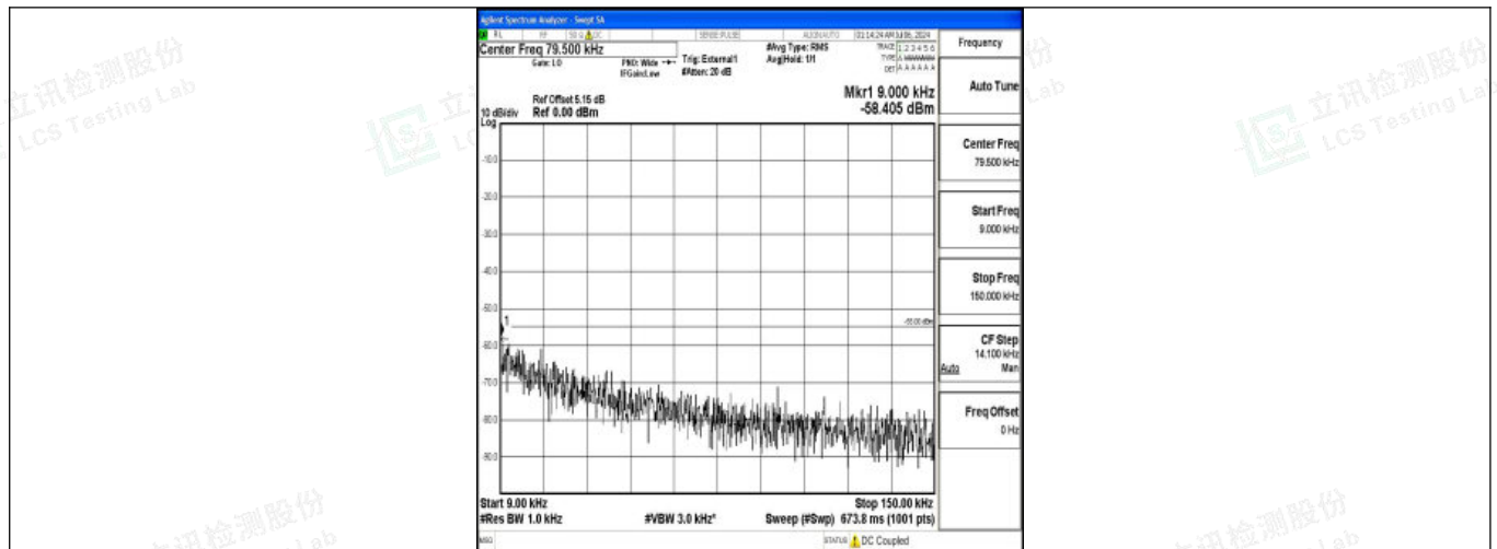
Band38_5MHz_QPSK_38225_1RB#0_0.009~0.15_0.009~0.15
