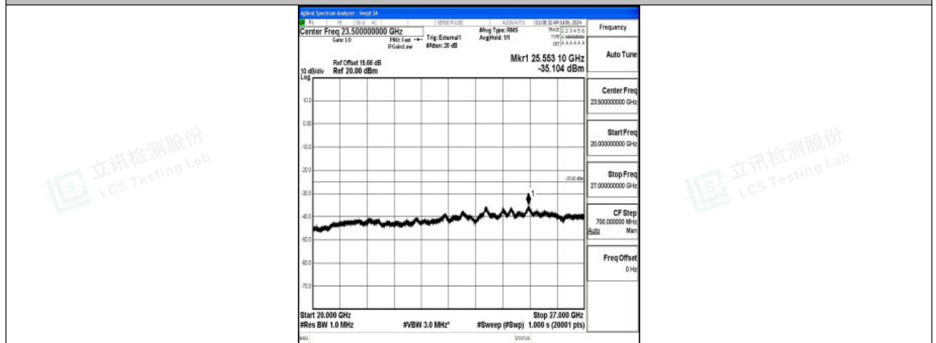
Band38_5MHz_QPSK_37775_1RB#0_20000~27000_20000~27000
