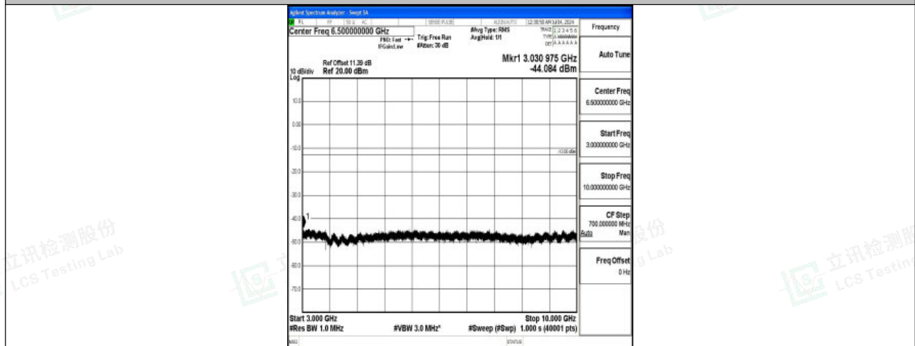
Band26_10MHz_16QAM_26915_1RB#0_3000~10000_3000~10000
