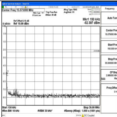
Band26_5MHz_16QAM_27015_1RB#0_0.15~30_0.15~30
