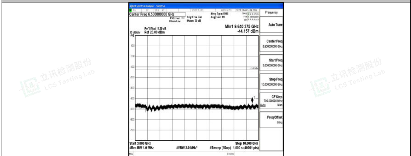
Band26_10MHz_QPSK_26915_1RB#0_3000~10000_3000~10000
