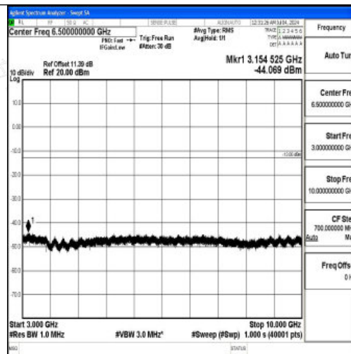
Band26_10MHz_QPSK_26990_1RB#0_3000~10000_3000~10000
