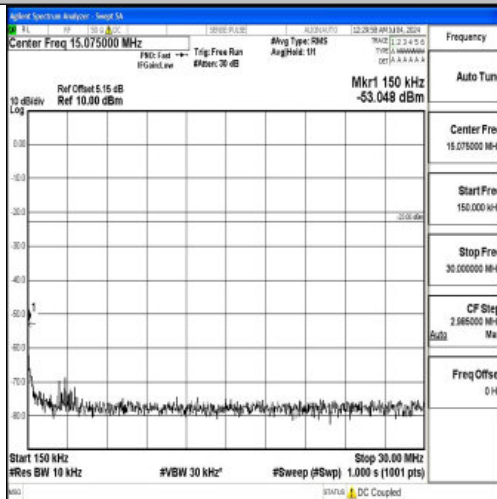
Band26_10MHz_QPSK_26915_1RB#0_0.15~30_0.15~30
