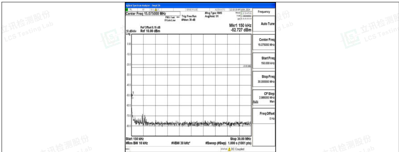
Band26_5MHz_QPSK_27015_1RB#0_0.15~30_0.15~30
