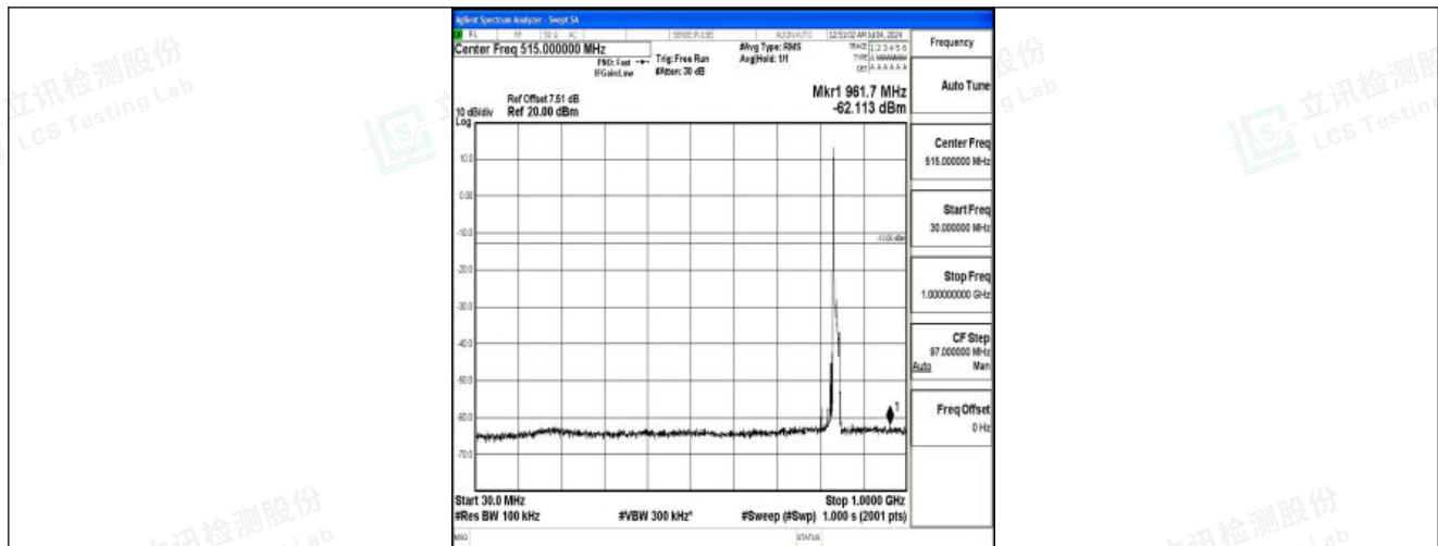
Band26_15MHz_16QAM_26965_1RB#0_30~1000_30~1000
