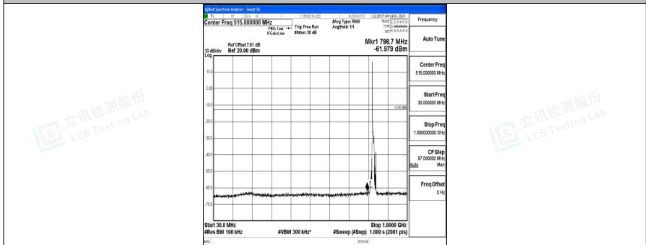
Band26_10MHz_QPSK_26840_1RB#0_30~1000_30~1000
