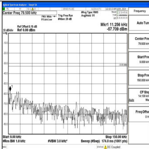
Band26_5MHz_QPSK_27015_1RB#0_0.009~0.15_0.009~0.15
