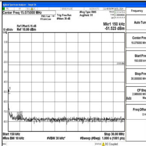
Band26_3MHz_16QAM_27025_1RB#0_0.15~30_0.15~30
