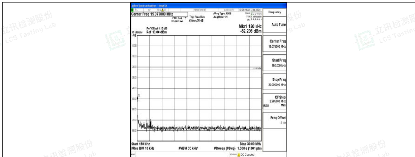
Band26_10MHz_16QAM_26840_1RB#0_0.15~30_0.15~30
