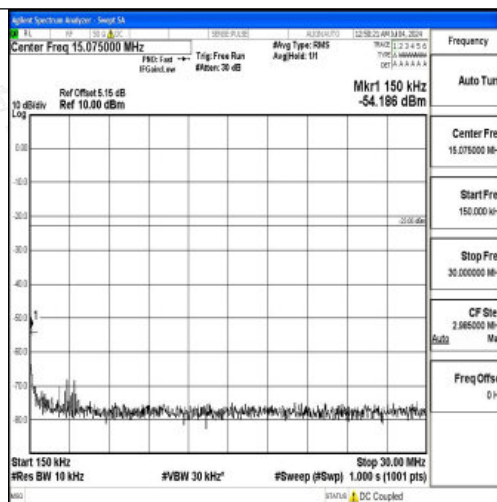
Band26_15MHz_QPSK_26965_1RB#0_0.15~30_0.15~30
