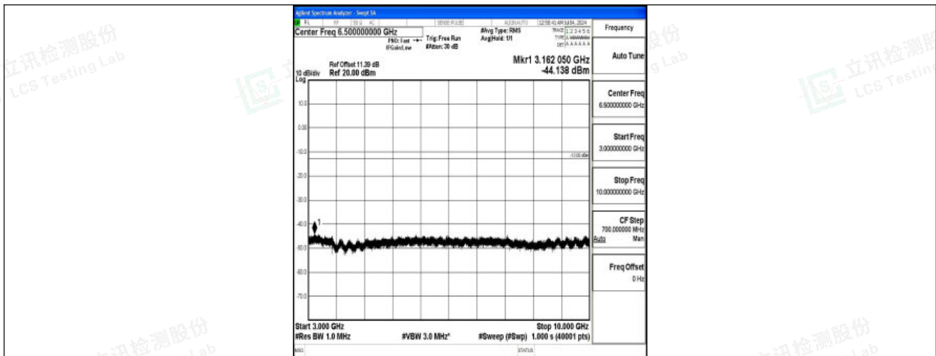
Band26_15MHz_QPSK_26965_1RB#0_3000~10000_3000~10000
