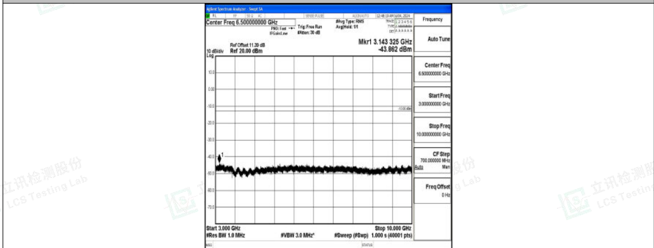
Band26_15MHz_QPSK_26865_1RB#0_3000~10000_3000~10000
