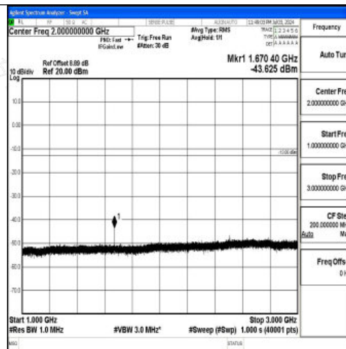
Band26_3MHz_16QAM_26915_1RB#0_1000~3000_1000~3000
