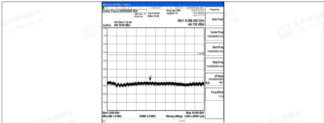
Band26_5MHz_16QAM_26815_1RB#0_3000~10000_3000~10000
