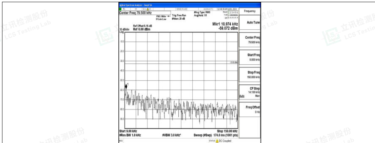
Band26_15MHz_16QAM_26915_1RB#0_0.009~0.15_0.009~0.15
