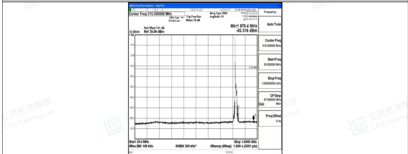
Band26_15MHz_16QAM_26865_1RB#0_30~1000_30~1000
