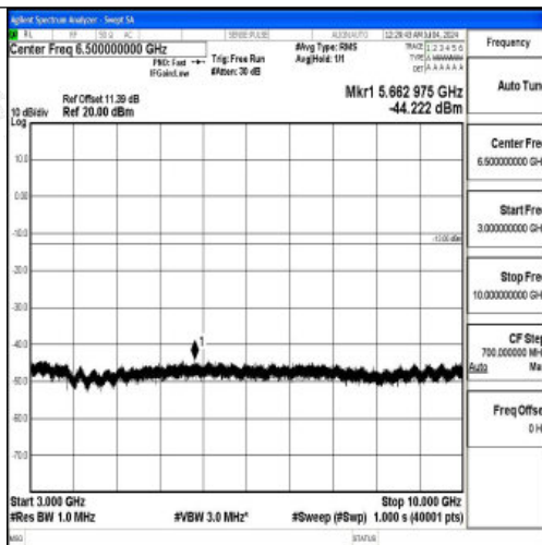
Band26_10MHz_16QAM_26840_1RB#0_3000~10000_3000~10000
