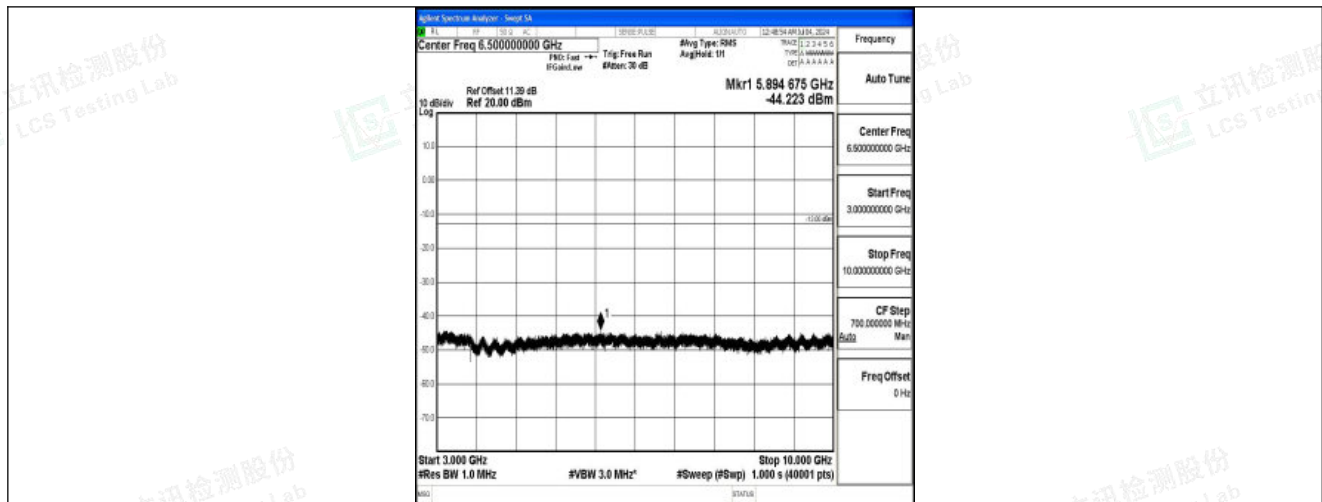
Band26_15MHz_16QAM_26865_1RB#0_3000~10000_3000~10000
