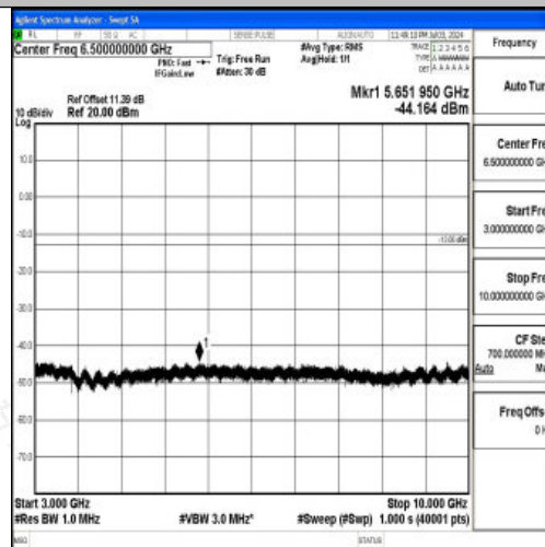
Band26_3MHz_16QAM_26915_1RB#0_3000~10000_3000~10000
