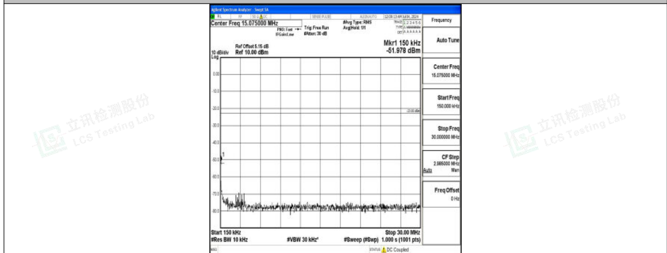
Band26_5MHz_QPSK_26915_1RB#0_0.15~30_0.15~30
