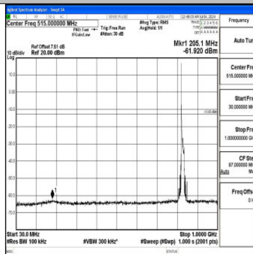
Band26_15MHz_QPSK_26865_1RB#0_30~1000_30~1000
