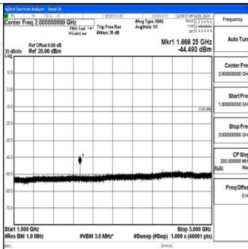
Band26_5MHz_16QAM_26915_1RB#0_1000~3000_1000~3000
