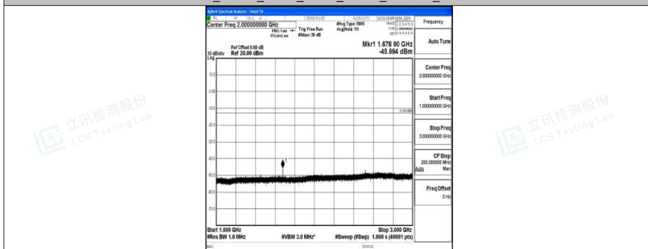
Band26_10MHz_QPSK_26990_1RB#0_1000~3000_1000~3000
