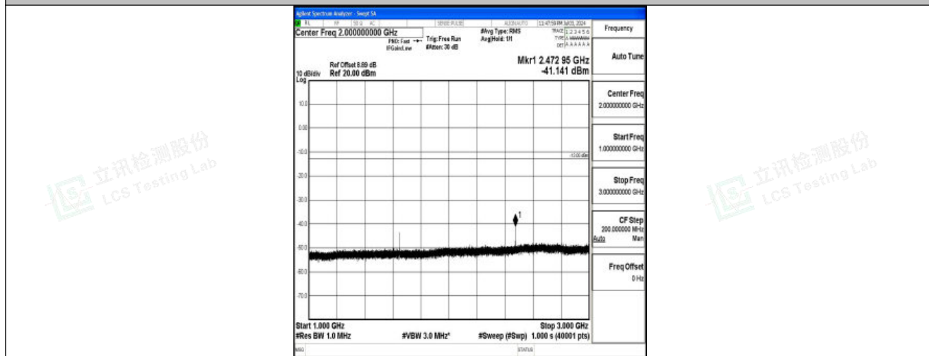
Band26_3MHz_16QAM_26805_1RB#0_1000~3000_1000~3000
