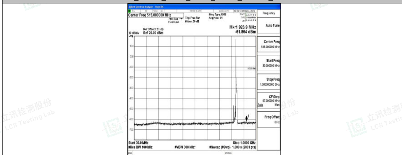
Band26_10MHz_QPSK_26990_1RB#0_30~1000_30~1000
