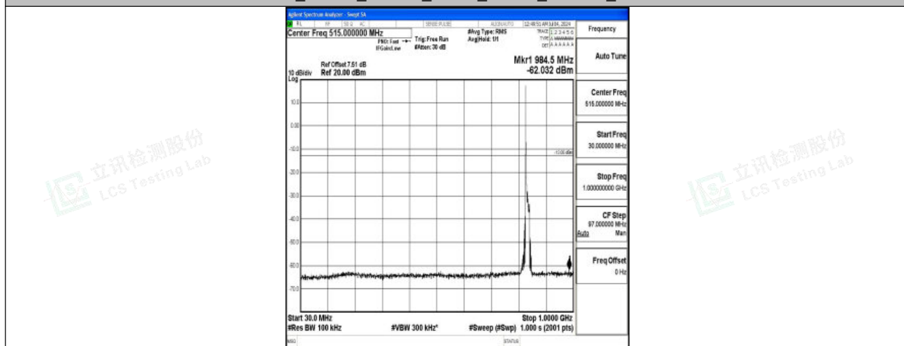
Band26_15MHz_16QAM_26915_1RB#0_30~1000_30~1000
