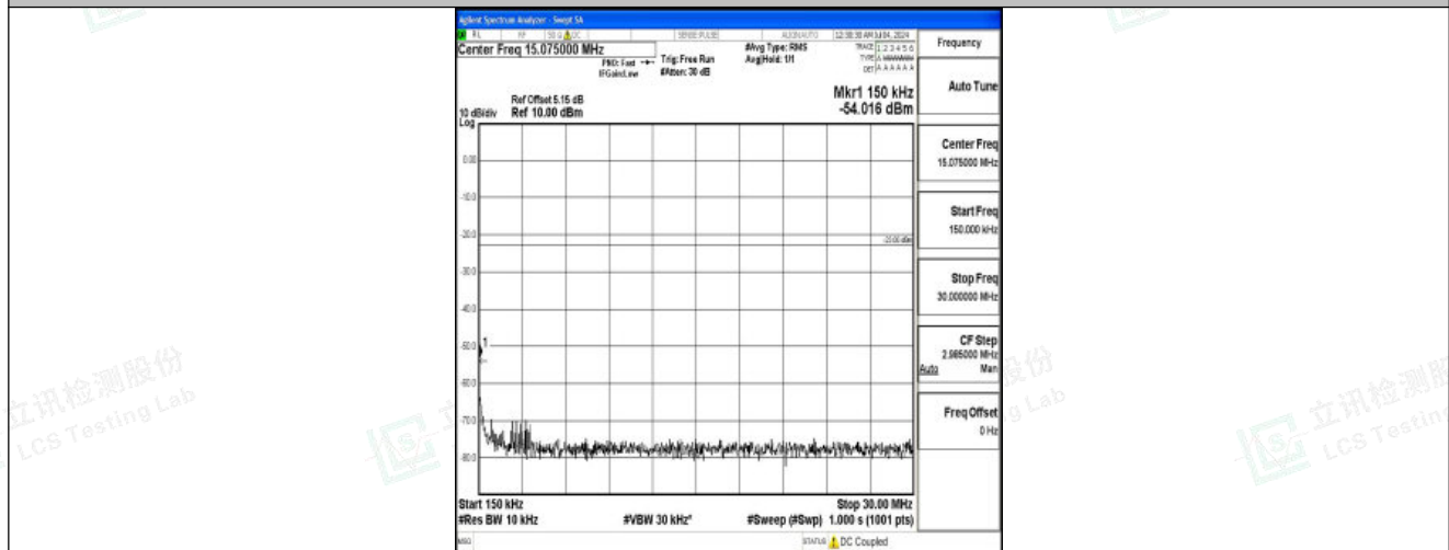
Band26_10MHz_16QAM_26915_1RB#0_0.15~30_0.15~30
