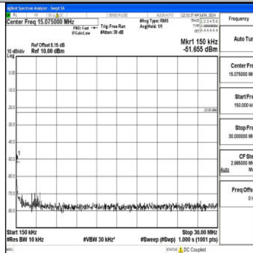
Band26_10MHz_16QAM_26990_1RB#0_0.15~30_0.15~30
