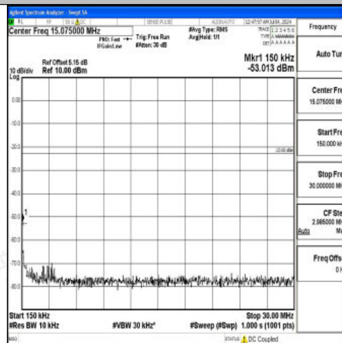
Band26_15MHz_QPSK_26865_1RB#0_0.15~30_0.15~30
