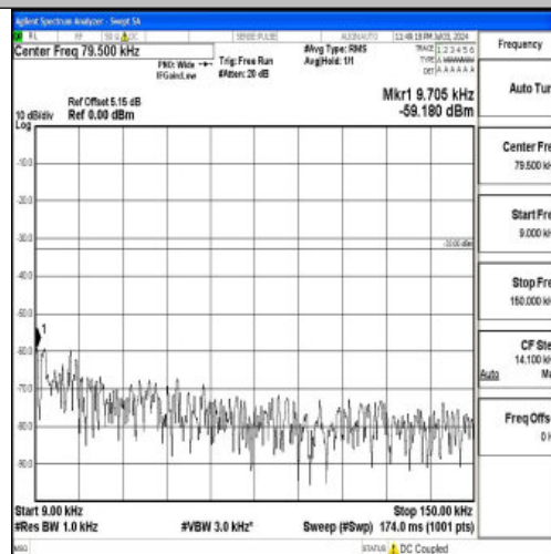
Band26_3MHz_QPSK_27025_1RB#0_0.009~0.15_0.009~0.15
