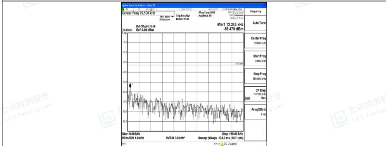
Band26_5MHz_QPSK_26915_1RB#0_0.009~0.15_0.009~0.15
