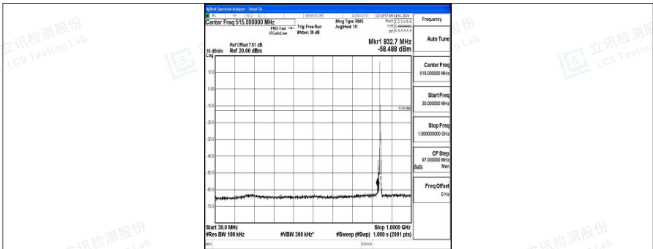
Band26_5MHz_16QAM_27015_1RB#0_30~1000_30~1000
