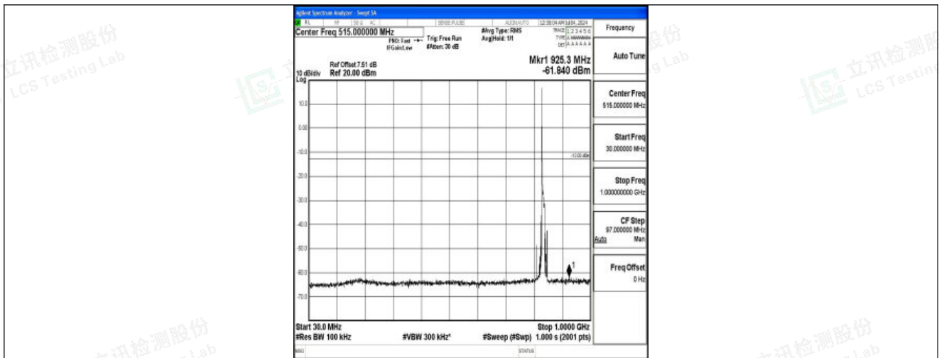
Band26_10MHz_QPSK_26915_1RB#0_30~1000_30~1000
