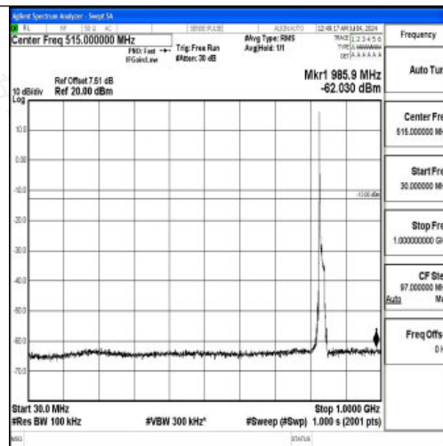
Band26_15MHz_QPSK_26915_1RB#0_30~1000_30~1000
