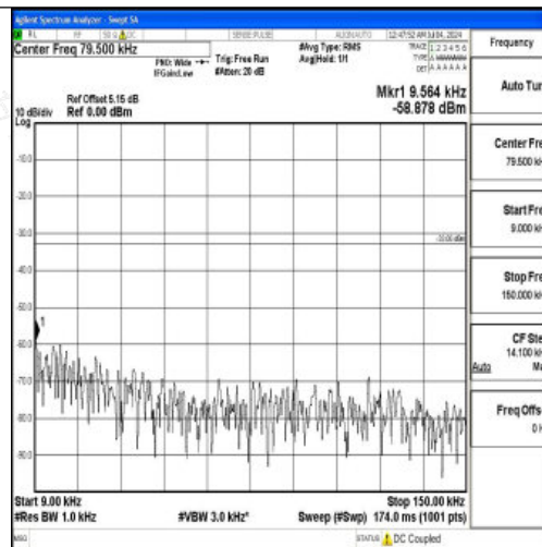
Band26_15MHz_QPSK_26865_1RB#0_0.009~0.15_0.009~0.15
