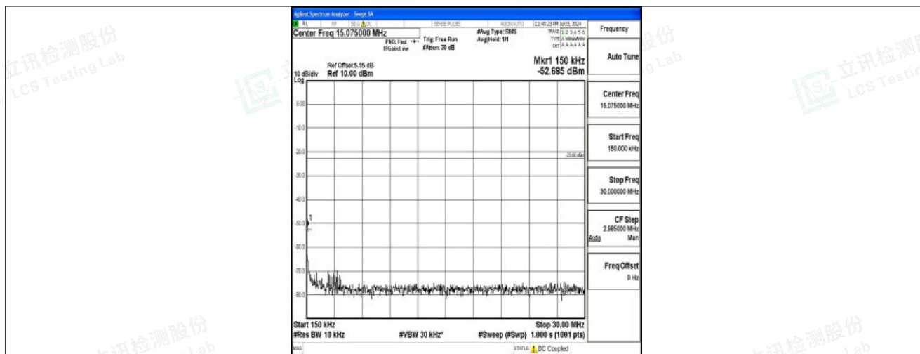
Band26_3MHz_QPSK_27025_1RB#0_0.15~30_0.15~30
