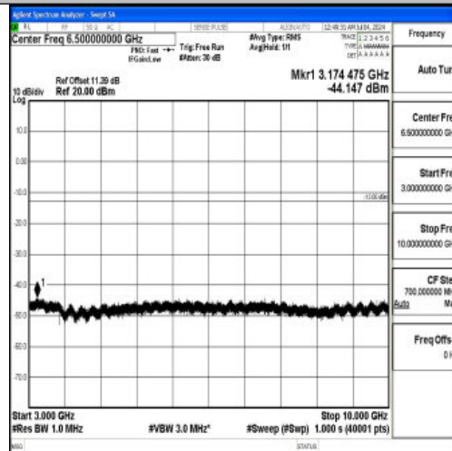
Band26_15MHz_QPSK_26915_1RB#0_3000~10000_3000~10000
