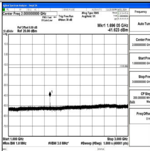
Band26_1.4MHz_16QAM_27033_1RB#0_1000~3000_1000~3000
