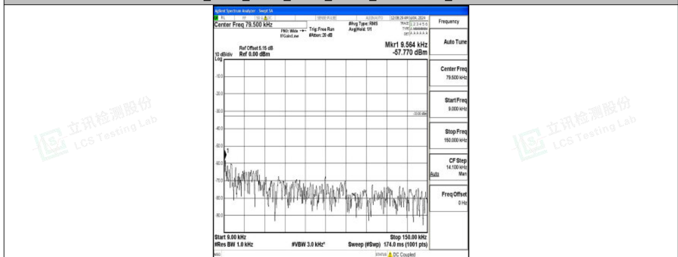
Band26_5MHz_16QAM_26815_1RB#0_0.009~0.15_0.009~0.15
