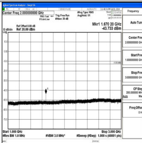
Band26_3MHz_QPSK_26915_1RB#0_1000~3000_1000~3000
