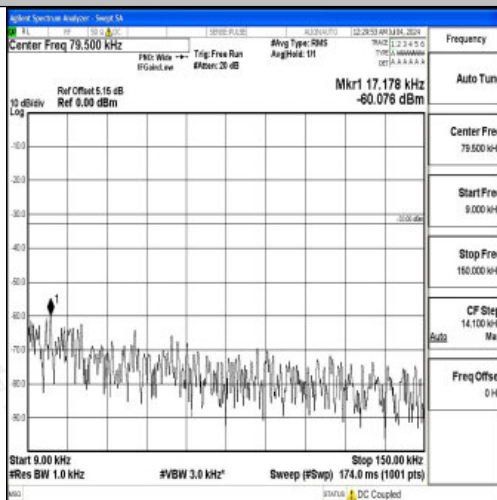
Band26_10MHz_QPSK_26915_1RB#0_0.009~0.15_0.009~0.15
