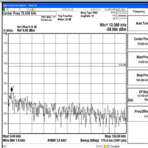
Band26_3MHz_16QAM_27025_1RB#0_0.009~0.15_0.009~0.15
