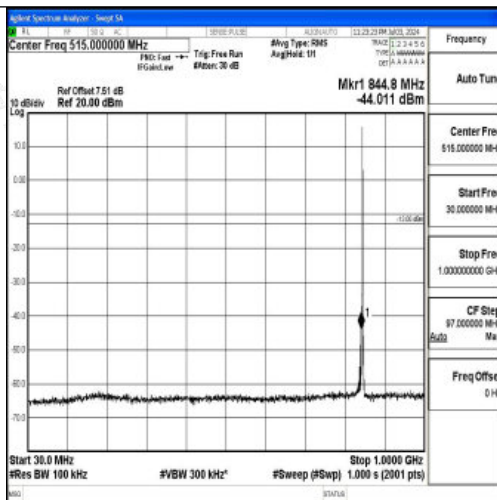
Band26_1.4MHz_16QAM_27033_1RB#0_30~1000_30~1000
