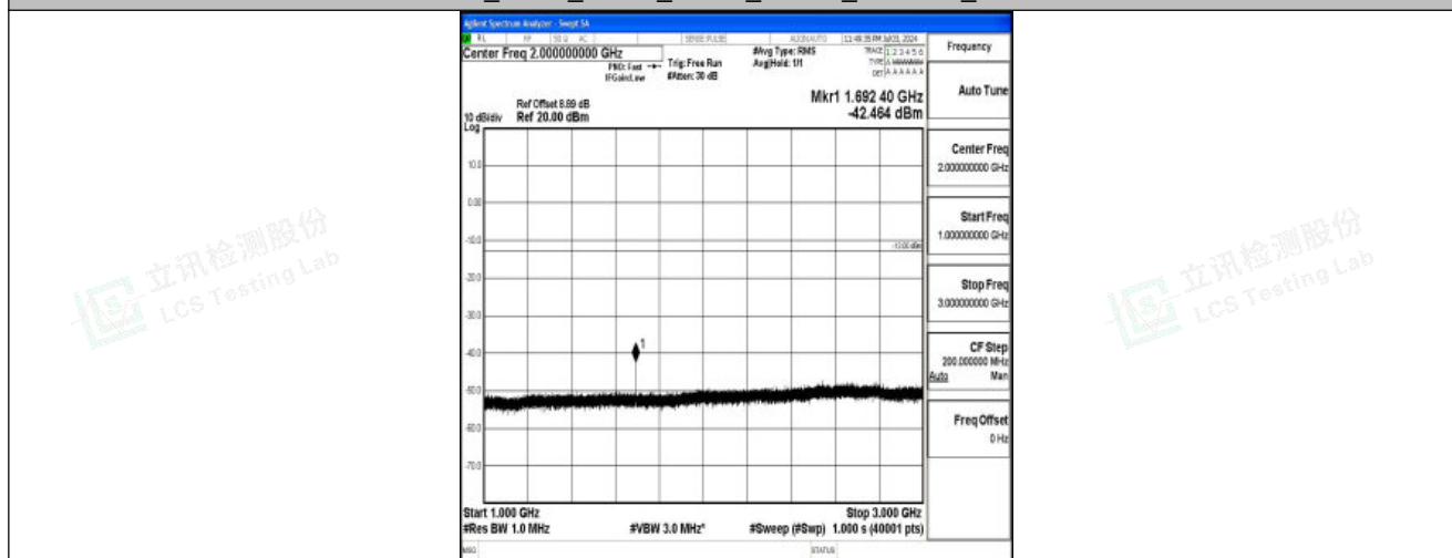
Band26_3MHz_QPSK_27025_1RB#0_1000~3000_1000~3000
