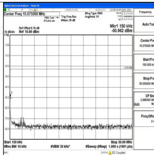
Band26_5MHz_16QAM_26815_1RB#0_0.15~30_0.15~30
