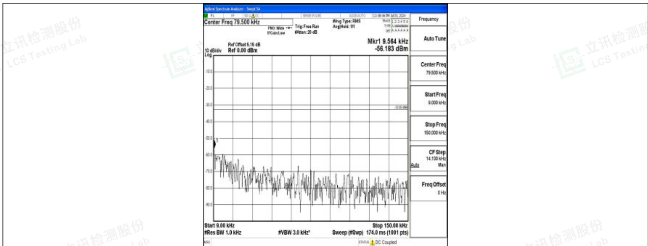
Band26_3MHz_16QAM_26915_1RB#0_0.009~0.15_0.009~0.15
