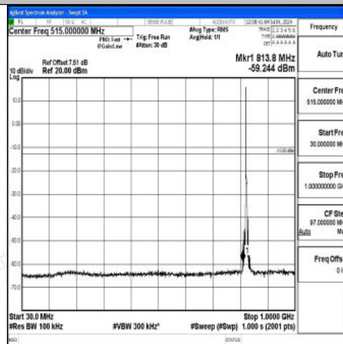
Band26_5MHz_16QAM_26815_1RB#0_30~1000_30~1000
