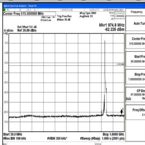
Band26_15MHz_QPSK_26965_1RB#0_30~1000_30~1000
