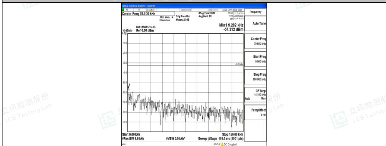
Band26_1.4MHz_16QAM_27033_1RB#0_0.009~0.15_0.009~0.15
