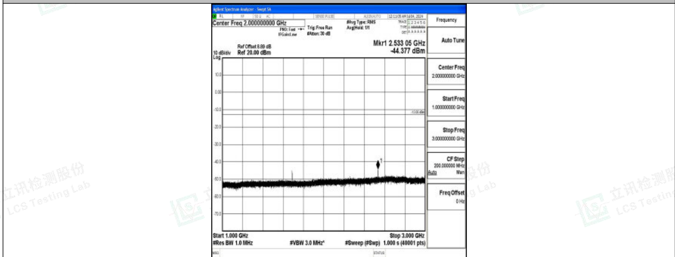
Band26_5MHz_16QAM_27015_1RB#0_1000~3000_1000~3000
