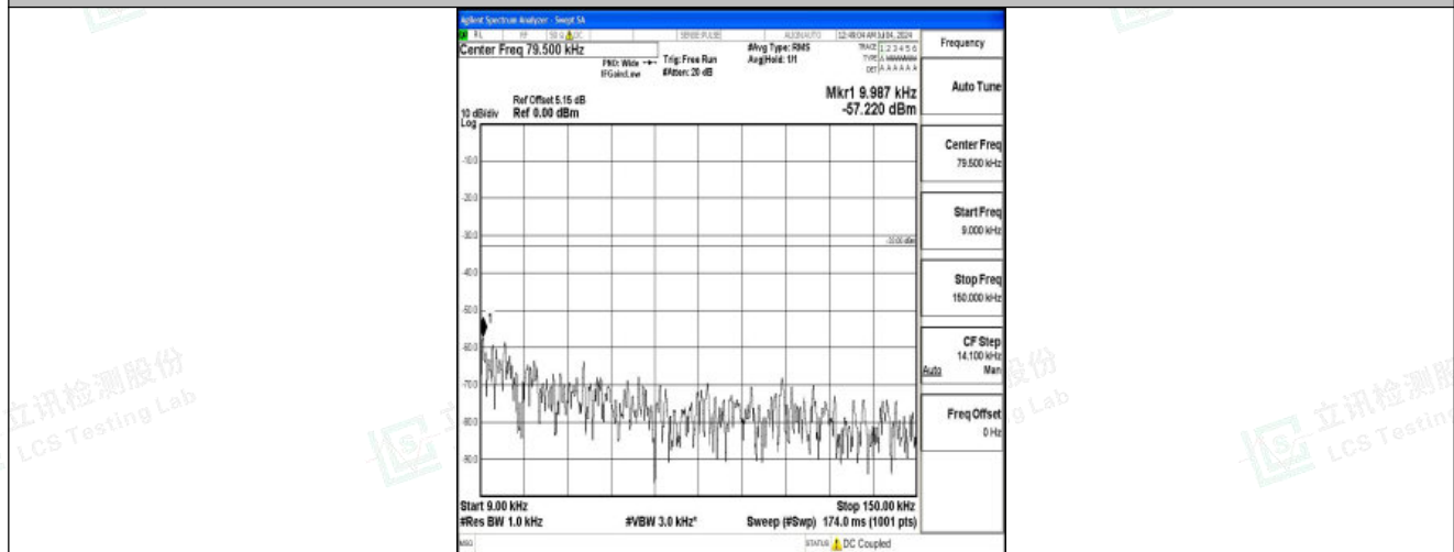
Band26_15MHz_QPSK_26915_1RB#0_0.009~0.15_0.009~0.15
