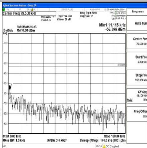
Band26_5MHz_16QAM_27015_1RB#0_0.009~0.15_0.009~0.15
