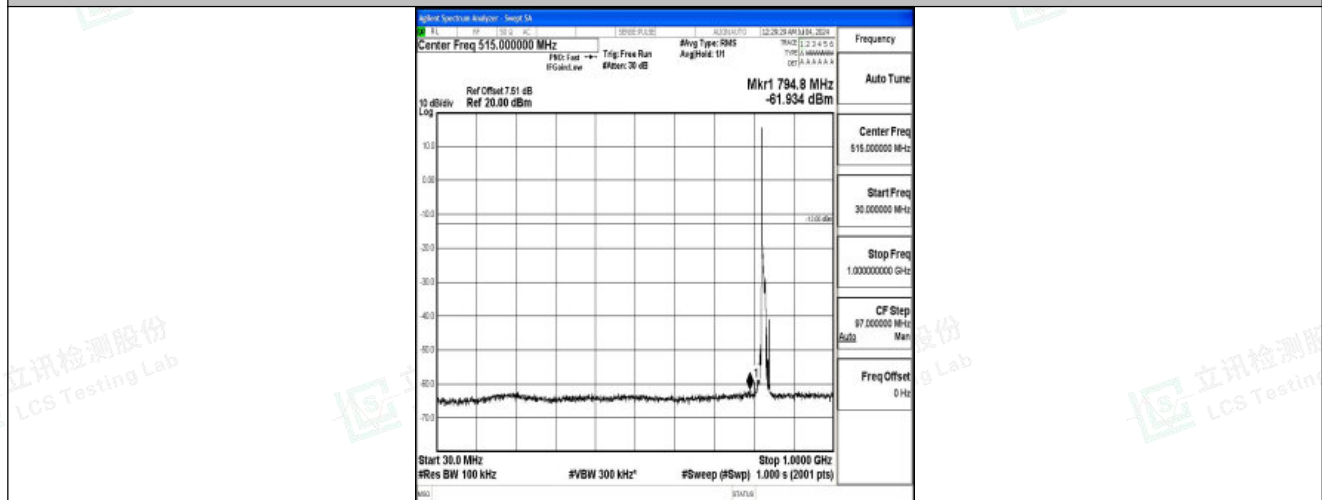
Band26_10MHz_16QAM_26840_1RB#0_30~1000_30~1000
