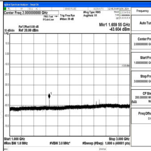
Band26_15MHz_QPSK_26915_1RB#0_1000~3000_1000~3000
