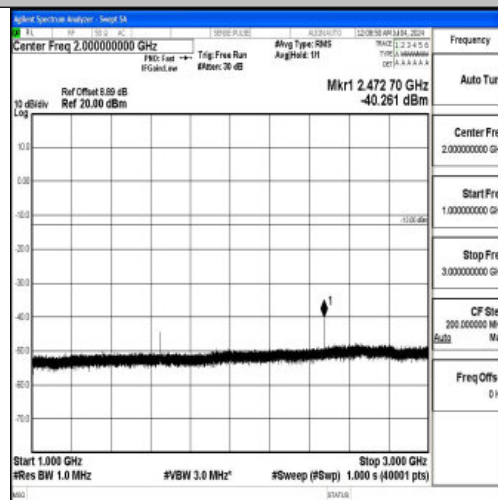
Band26_5MHz_16QAM_26815_1RB#0_1000~3000_1000~3000
