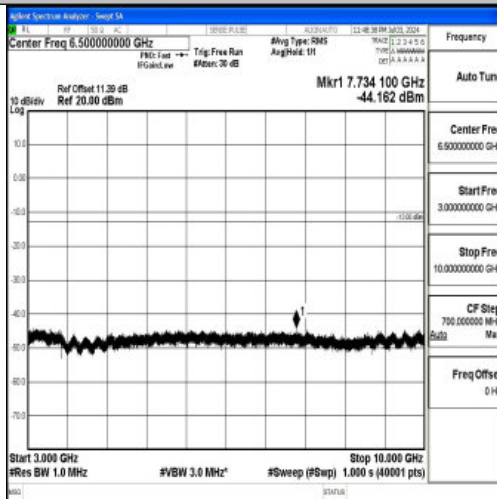
Band26_3MHz_QPSK_26915_1RB#0_3000~10000_3000~10000
