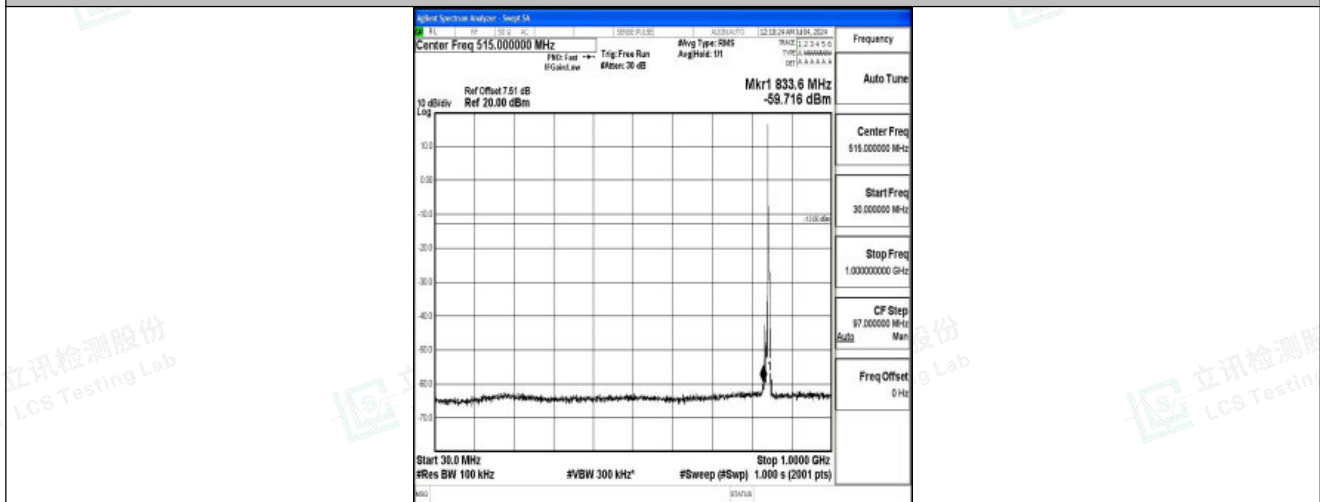
Band26_5MHz_QPSK_27015_1RB#0_30~1000_30~1000
