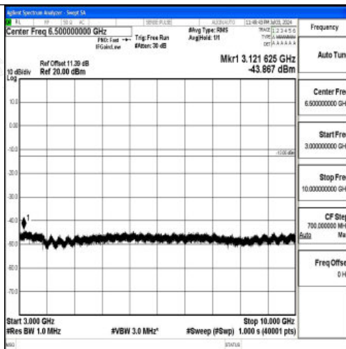
Band26_3MHz_QPSK_27025_1RB#0_3000~10000_3000~10000
