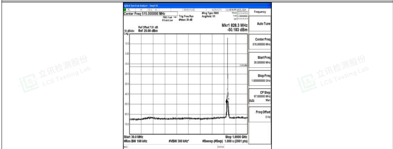
Band26_3MHz_16QAM_26915_1RB#0_30~1000_30~1000
