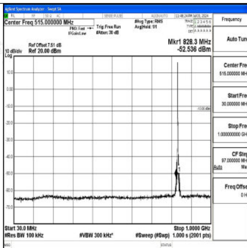
Band26_3MHz_QPSK_26915_1RB#0_30~1000_30~1000
