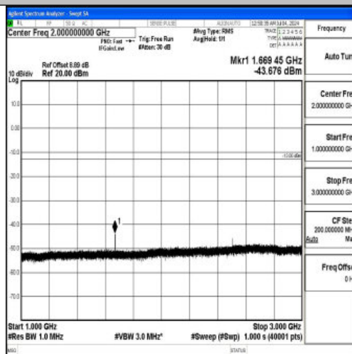
Band26_15MHz_QPSK_26965_1RB#0_1000~3000_1000~3000
