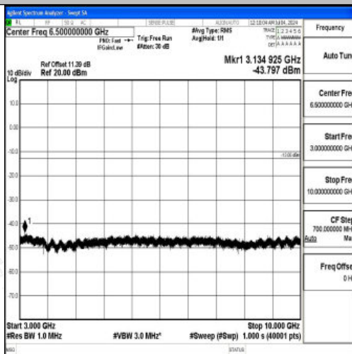
Band26_5MHz_16QAM_26915_1RB#0_3000~10000_3000~10000
