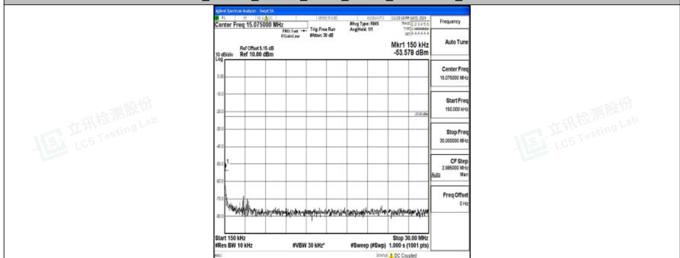
Band26_1.4MHz_16QAM_27033_1RB#0_0.15~30_0.15~30
