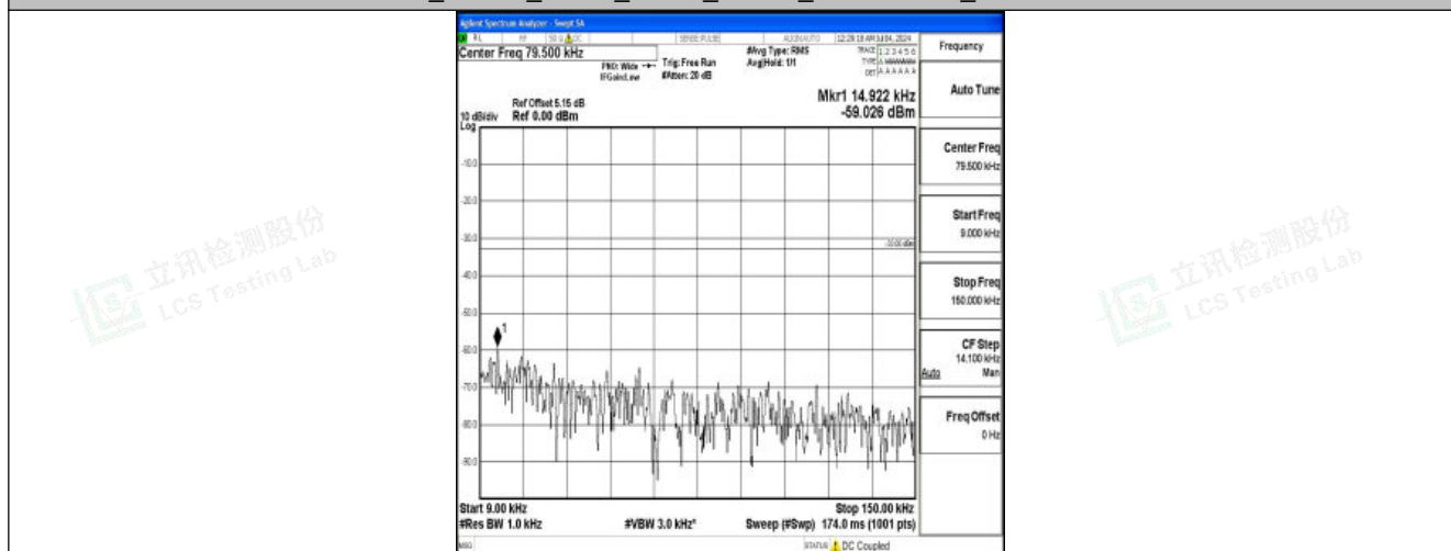
Band26_10MHz_16QAM_26840_1RB#0_0.009~0.15_0.009~0.15
