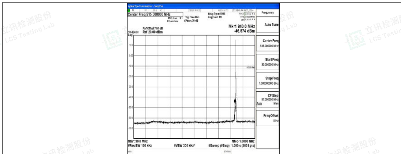
Band26_3MHz_16QAM_27025_1RB#0_30~1000_30~1000
