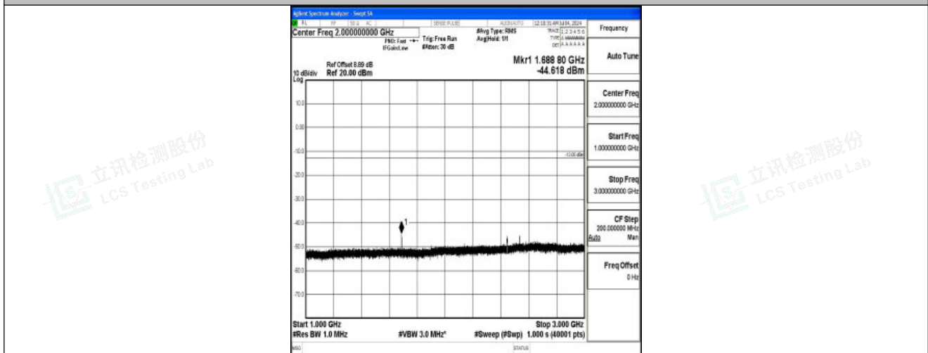
Band26_5MHz_QPSK_27015_1RB#0_1000~3000_1000~3000
