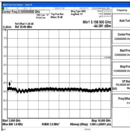
Band26_5MHz_QPSK_27015_1RB#0_3000~10000_3000~10000
