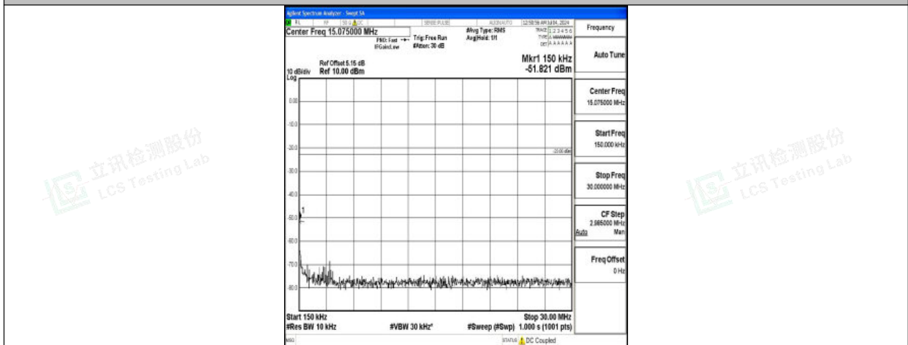
Band26_15MHz_16QAM_26965_1RB#0_0.15~30_0.15~30
