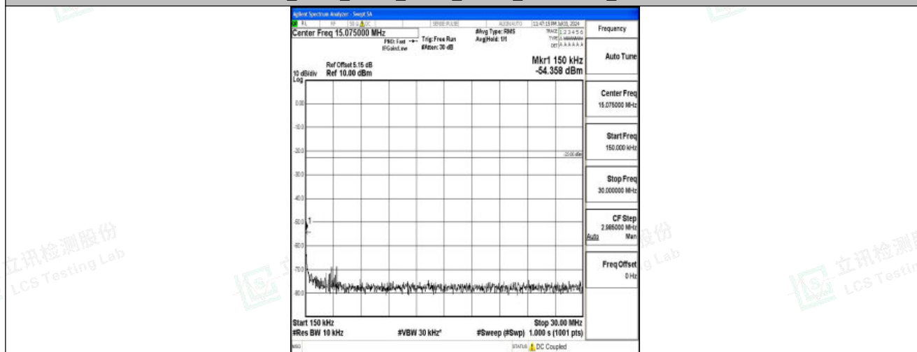
Band26_3MHz_QPSK_26805_1RB#0_0.15~30_0.15~30
