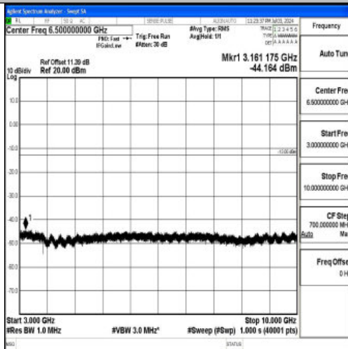
Band26_1.4MHz_16QAM_27033_1RB#0_3000~10000_3000~10000
