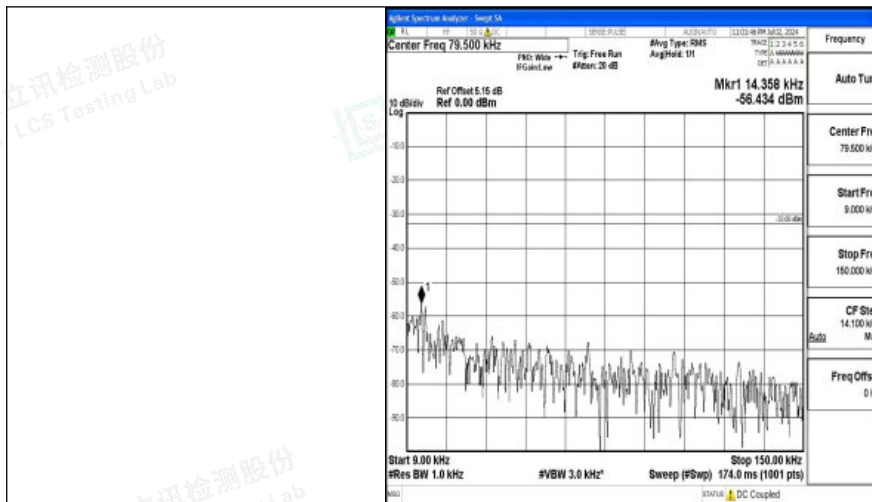
Band26_5MHz_16QAM_26740_1RB#0_0.009~0.15_0.009~0.15
