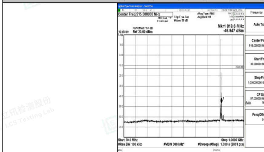
Band26_1.4MHz_16QAM_26697_1RB#0_30~1000_30~1000
