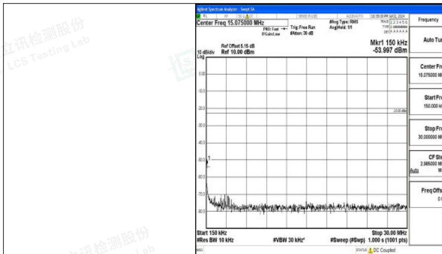
Band26_3MHz_QPSK_26775_1RB#0_0.15~30_0.15~30
