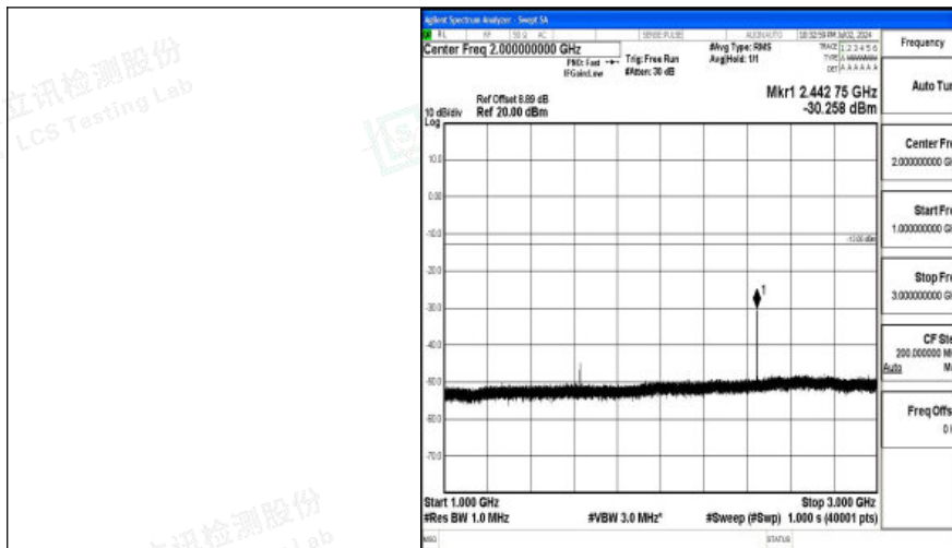
Band26_3MHz_QPSK_26705_1RB#0_1000~3000_1000~3000
