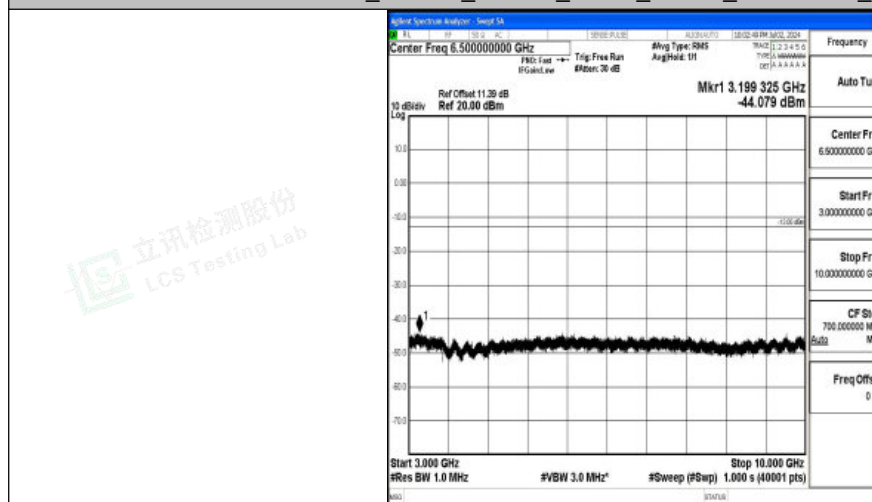
Band26_1.4MHz_16QAM_26783_1RB#0_3000~10000_3000~10000
