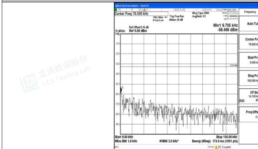
Band26_10MHz_16QAM_26740_1RB#0_0.009~0.15_0.009~0.15
