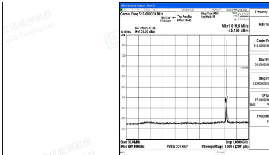
Band26_1.4MHz_16QAM_26783_1RB#0_30~1000_30~1000
