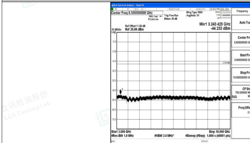
Band26_3MHz_QPSK_26705_1RB#0_3000~10000_3000~10000
