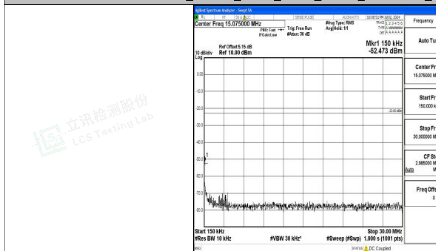
Band26_1.4MHz_QPSK_26740_1RB#0_0.15~30_0.15~30
