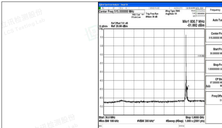
Band26_3MHz_16QAM_26775_1RB#0_30~1000_30~1000
