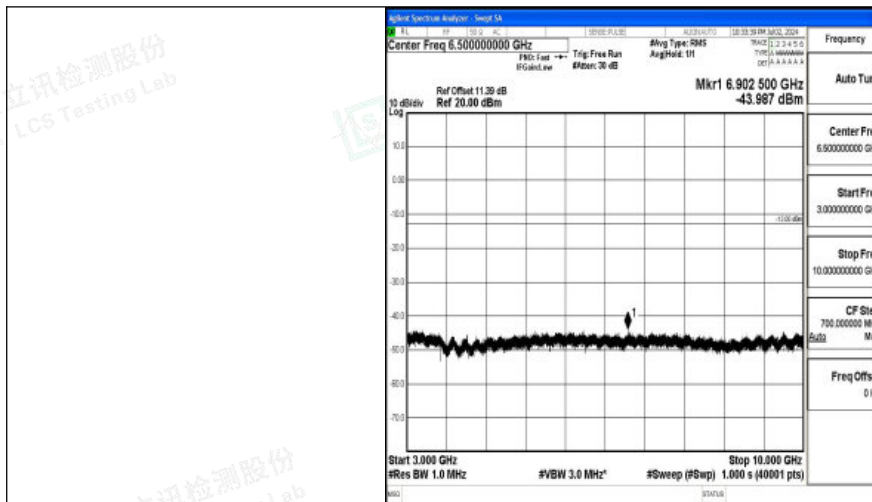
Band26_3MHz_16QAM_26705_1RB#0_3000~10000_3000~10000
