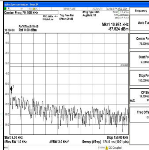
Band26_5MHz_QPSK_26740_1RB#0_0.009~0.15_0.009~0.15
