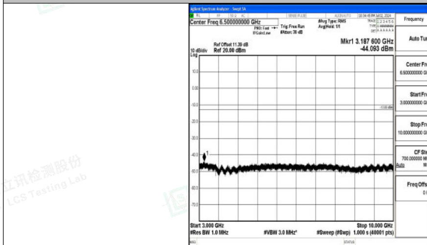
Band26_3MHz_16QAM_26740_1RB#0_3000~10000_3000~10000
