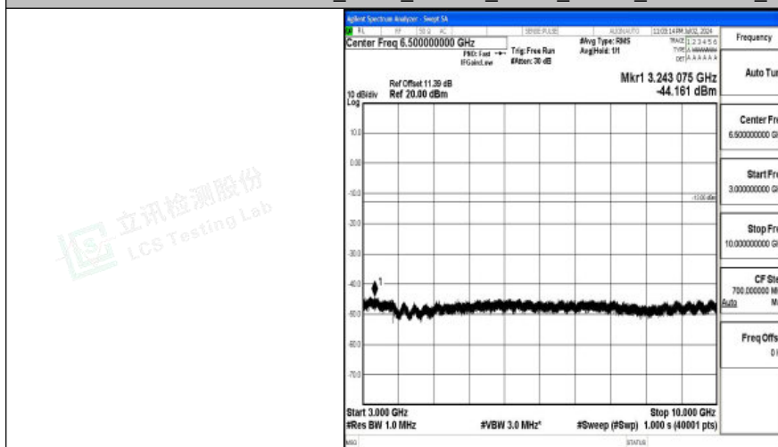
Band26_5MHz_16QAM_26765_1RB#0_3000~10000_3000~10000
