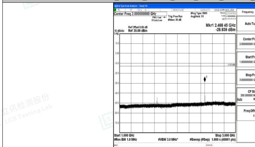
Band26_1.4MHz_16QAM_26783_1RB#0_1000~3000_1000~3000
