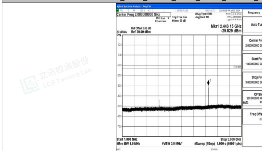
Band26_5MHz_16QAM_26715_1RB#0_1000~3000_1000~3000
