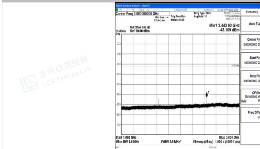
Band26_10MHz_16QAM_26740_1RB#0_1000~3000_1000~3000
