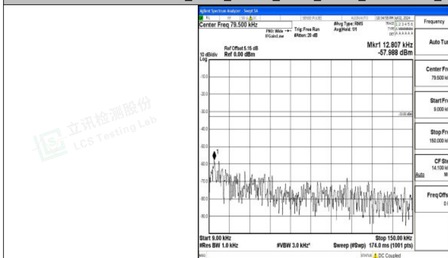
Band26_3MHz_QPSK_26775_1RB#0_0.009~0.15_0.009~0.15
