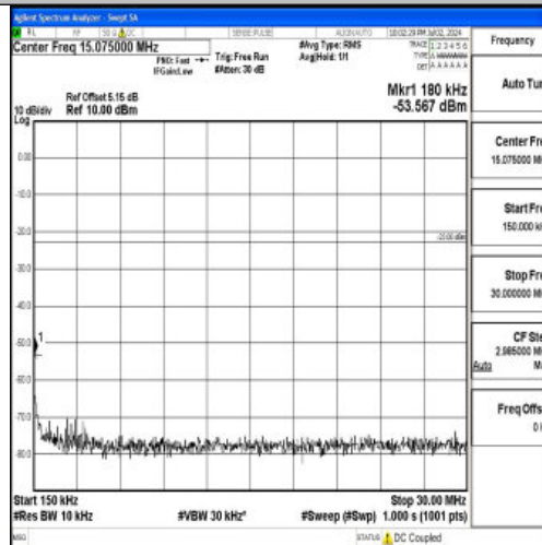
Band26_1.4MHz_16QAM_26783_1RB#0_0.15~30_0.15~30
