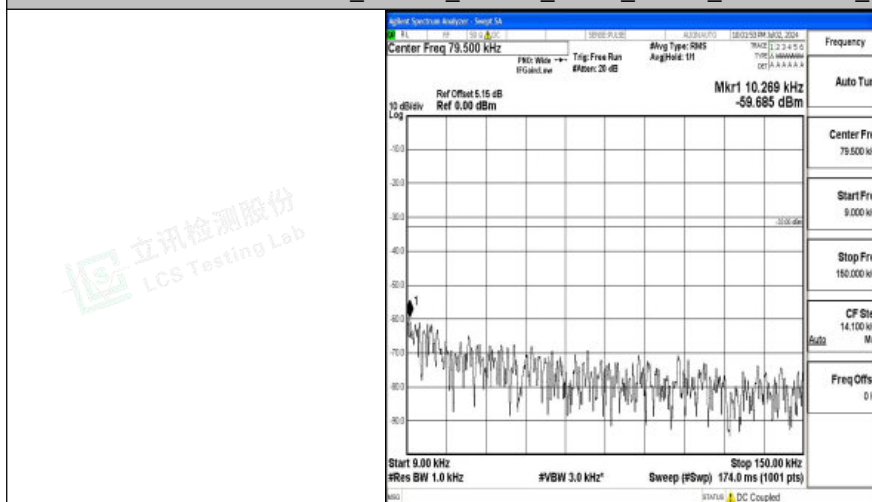
Band26_1.4MHz_QPSK_26783_1RB#0_0.009~0.15_0.009~0.15
