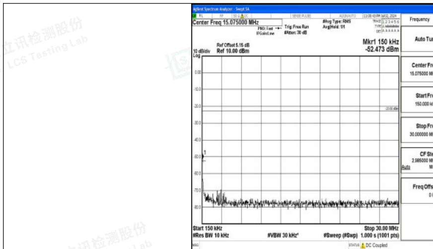
Band26_5MHz_16QAM_26715_1RB#0_0.15~30_0.15~30
