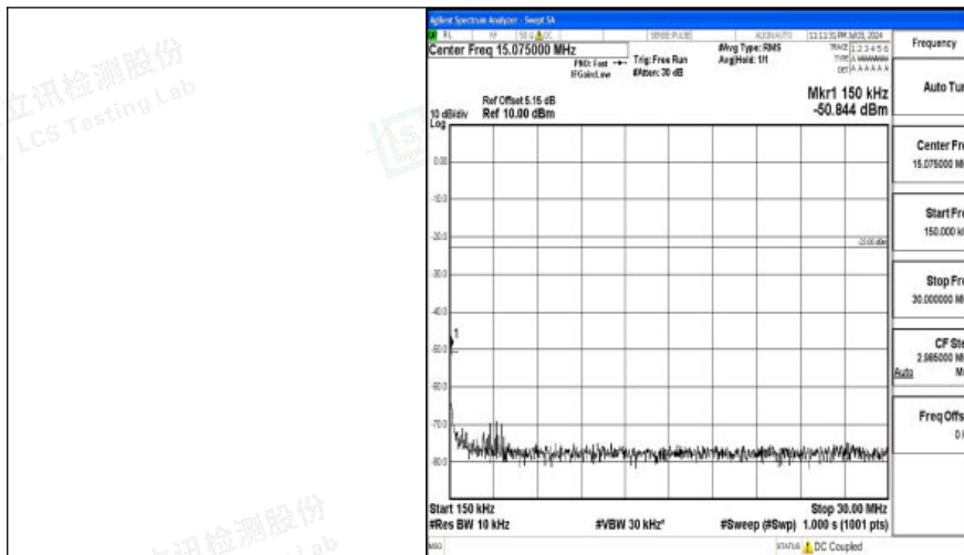
Band26_10MHz_16QAM_26740_1RB#0_0.15~30_0.15~30
