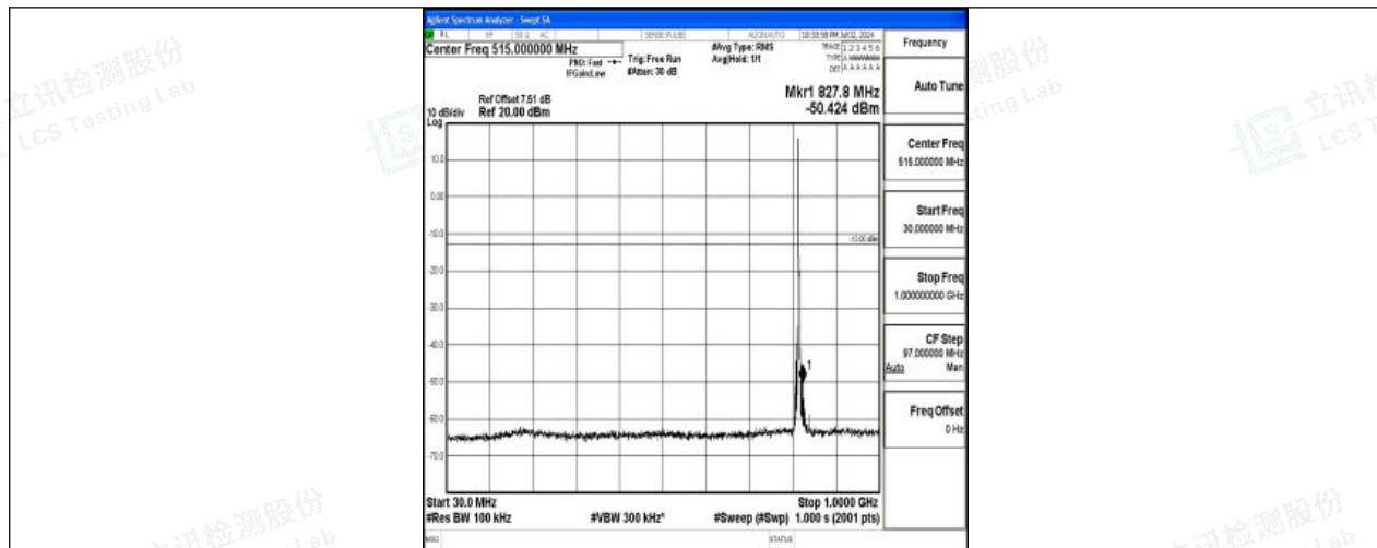
Band26_3MHz_QPSK_26740_1RB#0_30~1000_30~1000
