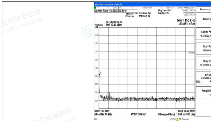
Band26_1.4MHz_16QAM_26697_1RB#0_0.15~30_0.15~30
