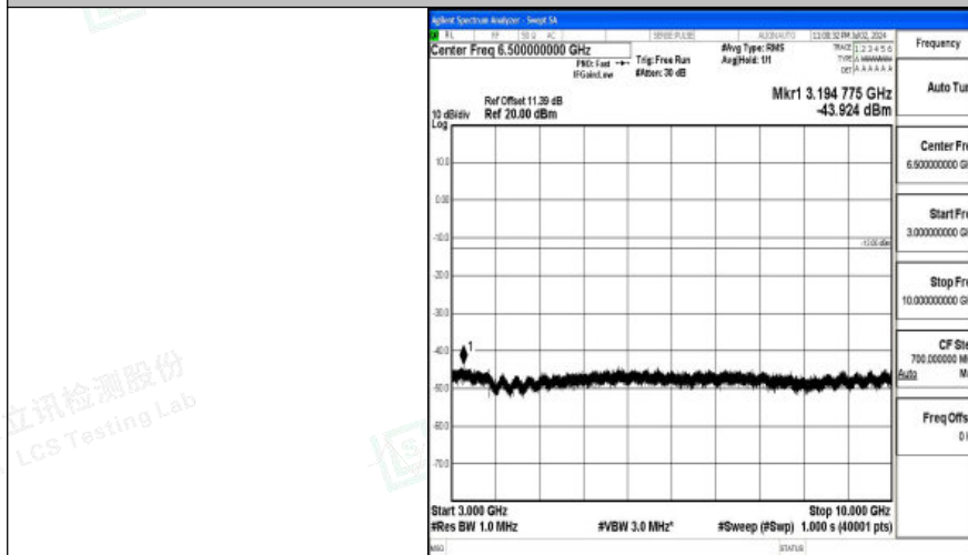
Band26_5MHz_QPSK_26715_1RB#0_3000~10000_3000~10000
