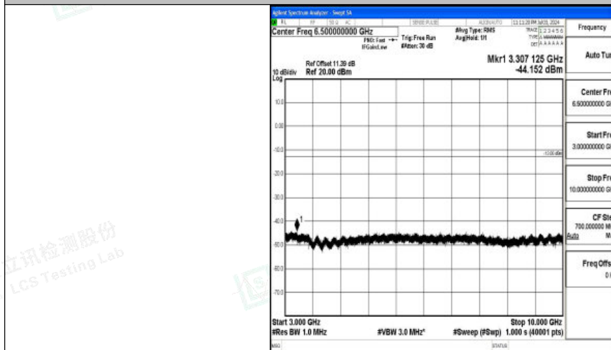
Band26_10MHz_QPSK_26740_1RB#0_3000~10000_3000~10000
