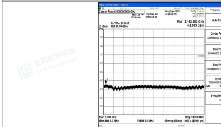
Band26_5MHz_QPSK_26740_1RB#0_3000~10000_3000~10000
