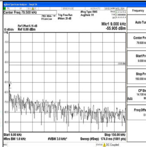
Band26_1.4MHz_16QAM_26783_1RB#0_0.009~0.15_0.009~0.15
