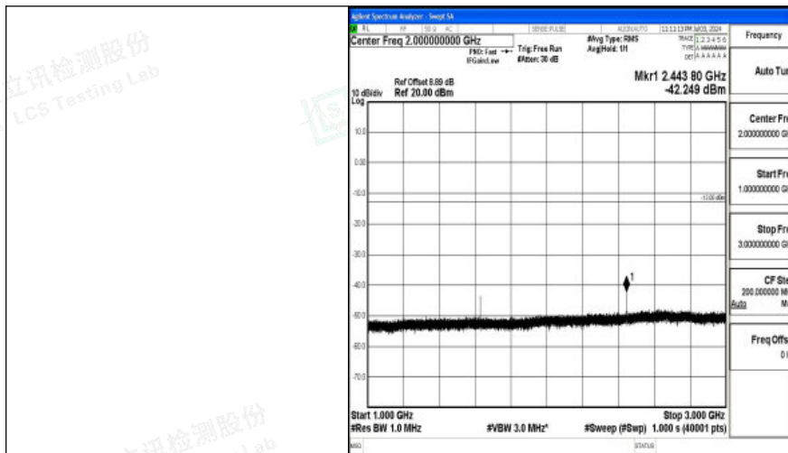
Band26_10MHz_QPSK_26740_1RB#0_1000~3000_1000~3000
