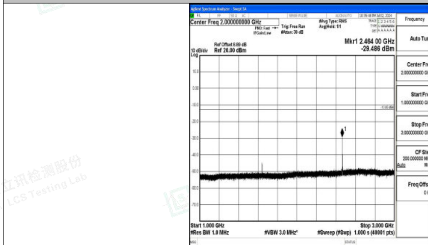
Band26_3MHz_16QAM_26775_1RB#0_1000~3000_1000~3000
