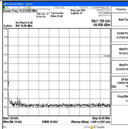
Band26_5MHz_16QAM_26740_1RB#0_0.15~30_0.15~30
