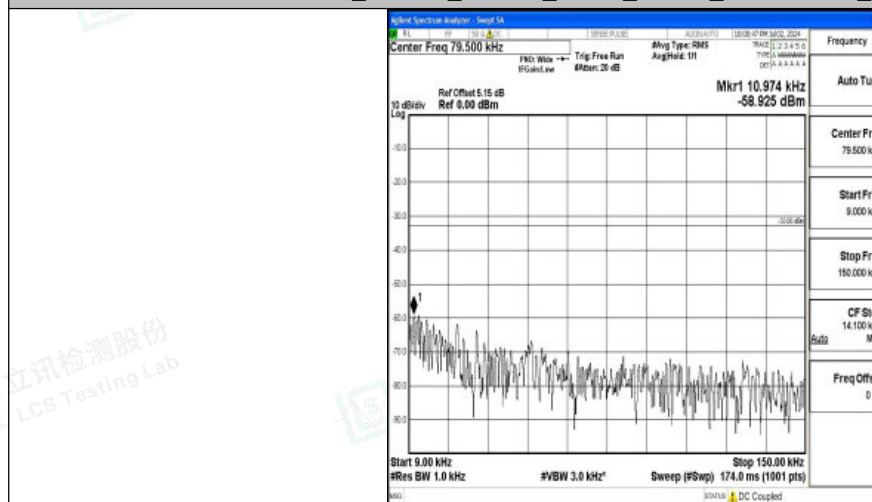
Band26_1.4MHz_QPSK_26740_1RB#0_0.009~0.15_0.009~0.15
