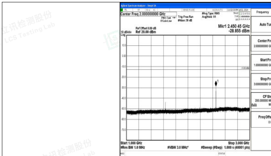
Band26_5MHz_16QAM_26740_1RB#0_1000~3000_1000~3000
