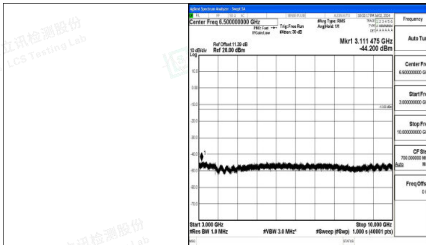
Band26_1.4MHz_QPSK_26783_1RB#0_3000~10000_3000~10000
