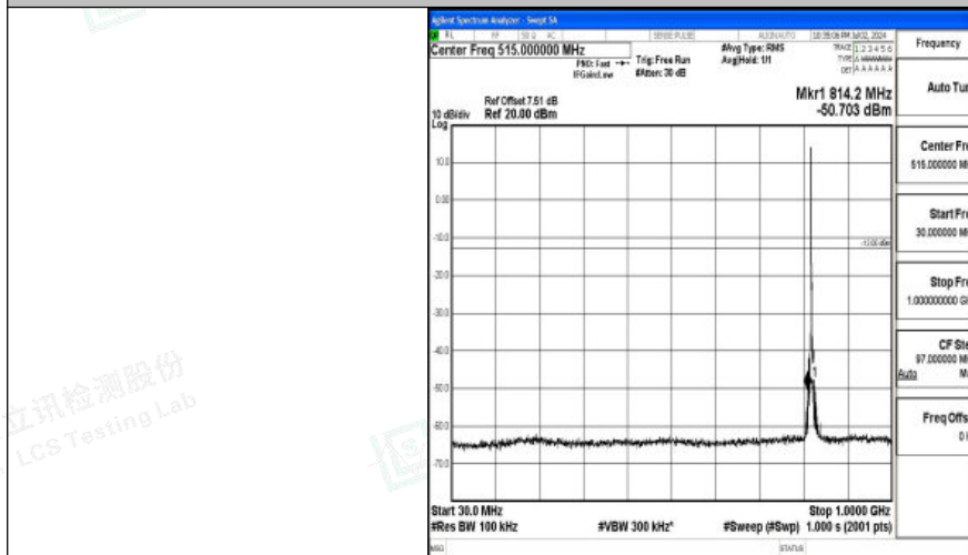
Band26_3MHz_QPSK_26775_1RB#0_30~1000_30~1000
