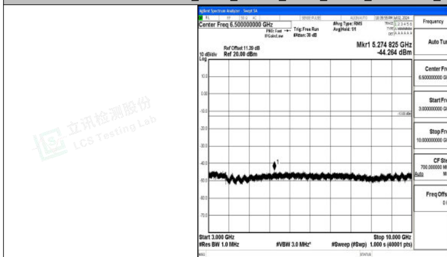
Band26_3MHz_16QAM_26775_1RB#0_3000~10000_3000~10000
