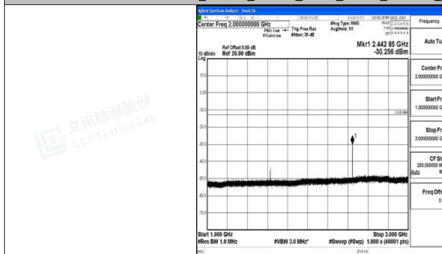
Band26_1.4MHz_16QAM_26697_1RB#0_1000~3000_1000~3000
