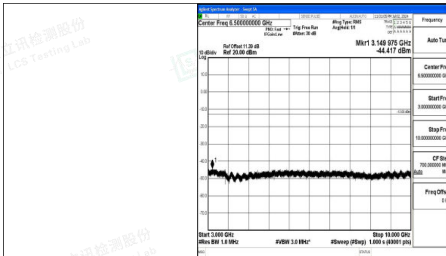
Band26_5MHz_16QAM_26715_1RB#0_3000~10000_3000~10000
