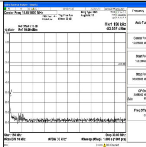
Band26_5MHz_QPSK_26740_1RB#0_0.15~30_0.15~30
