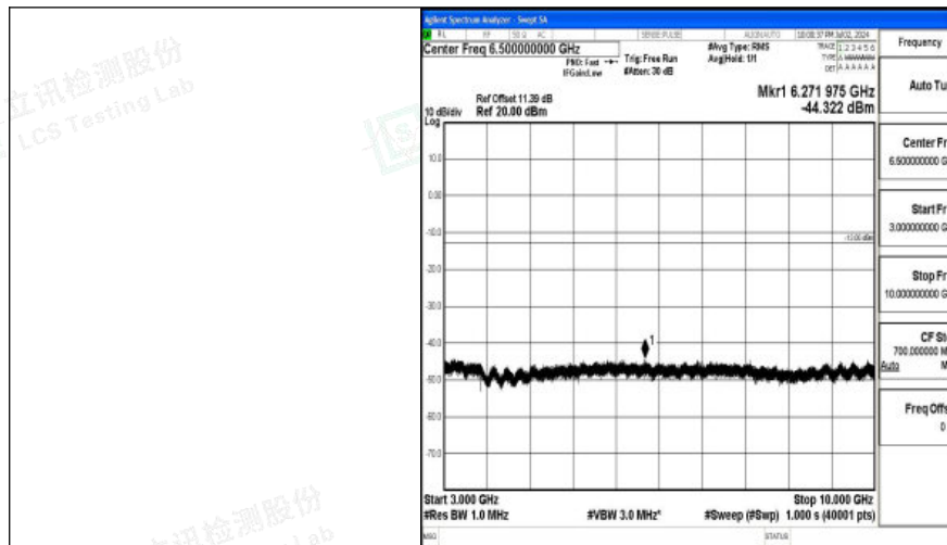
Band26_1.4MHz_16QAM_26697_1RB#0_3000~10000_3000~10000
