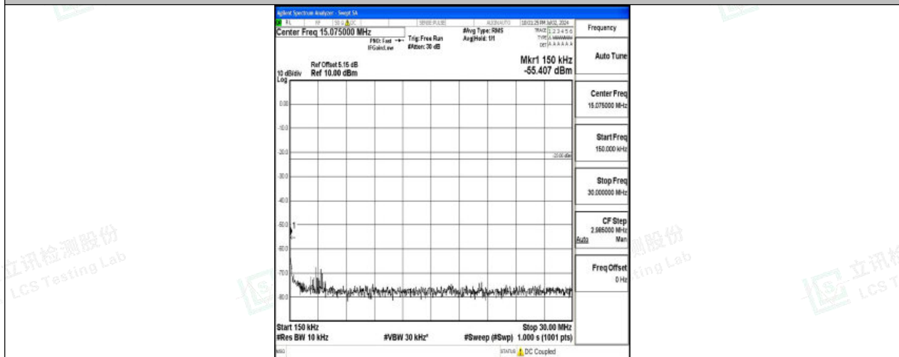
Band26_1.4MHz_16QAM_26740_1RB#0_0.15~30_0.15~30
