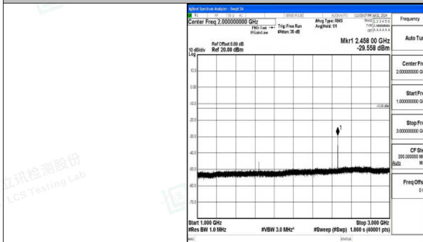
Band26_5MHz_16QAM_26765_1RB#0_1000~3000_1000~3000
