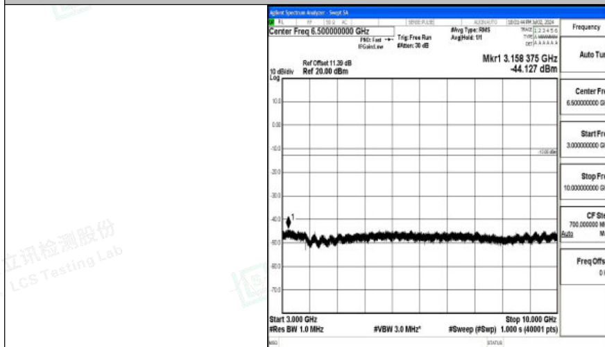
Band26_1.4MHz_16QAM_26740_1RB#0_3000~10000_3000~10000
