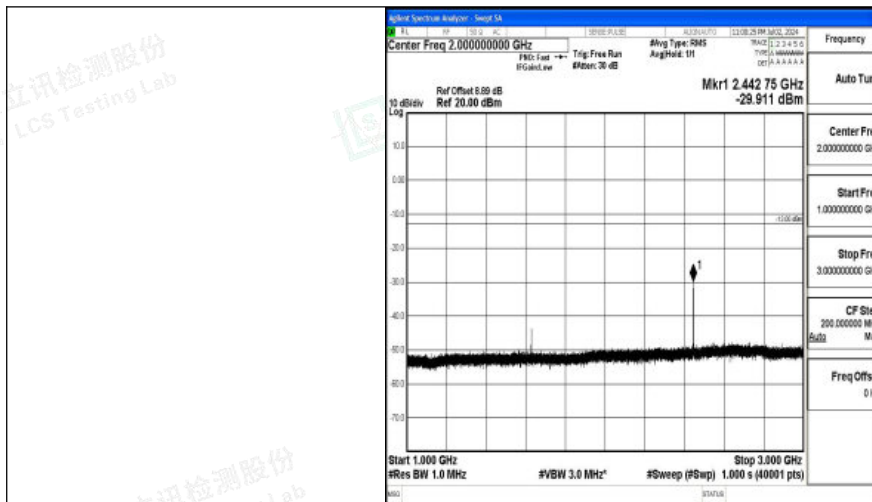
Band26_5MHz_QPSK_26715_1RB#0_1000~3000_1000~3000
