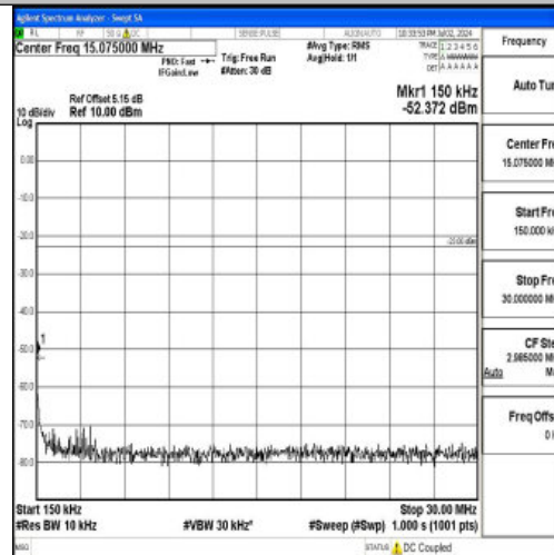
Band26_3MHz_QPSK_26740_1RB#0_0.15~30_0.15~30
