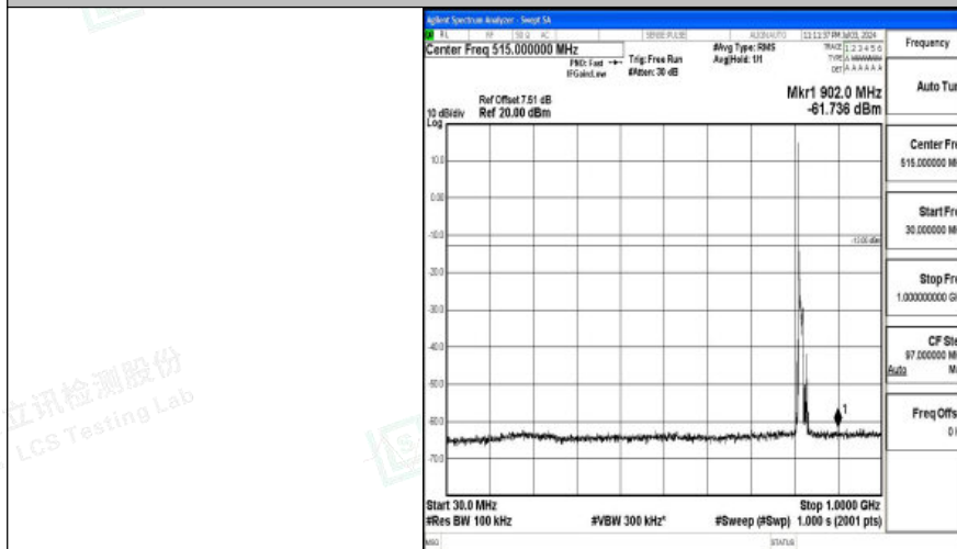
Band26_10MHz_16QAM_26740_1RB#0_30~1000_30~1000
