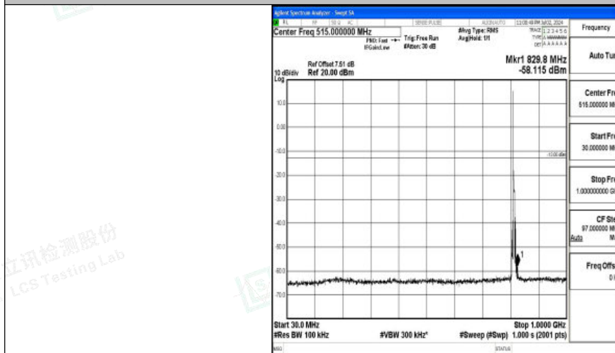
Band26_5MHz_16QAM_26715_1RB#0_30~1000_30~1000
