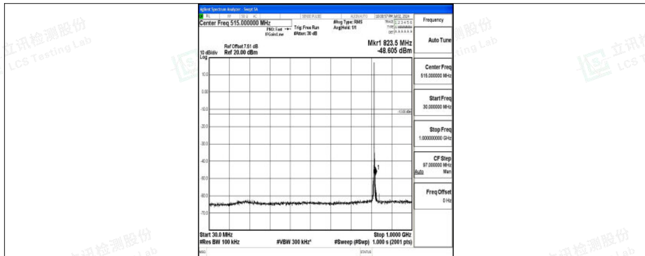
Band26_1.4MHz_QPSK_26740_1RB#0_30~1000_30~1000
