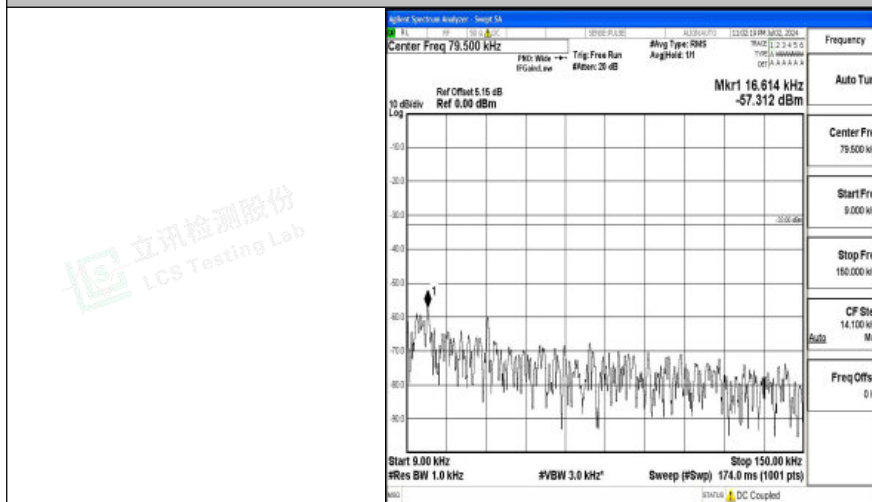
Band26_5MHz_QPSK_26765_1RB#0_0.009~0.15_0.009~0.15
