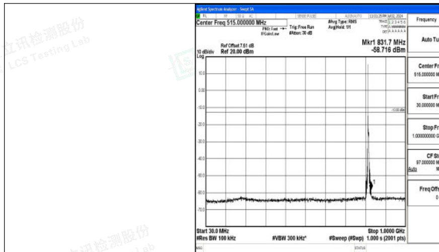
Band26_5MHz_QPSK_26740_1RB#0_30~1000_30~1000
