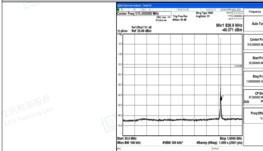
Band26_1.4MHz_QPSK_26783_1RB#0_30~1000_30~1000
