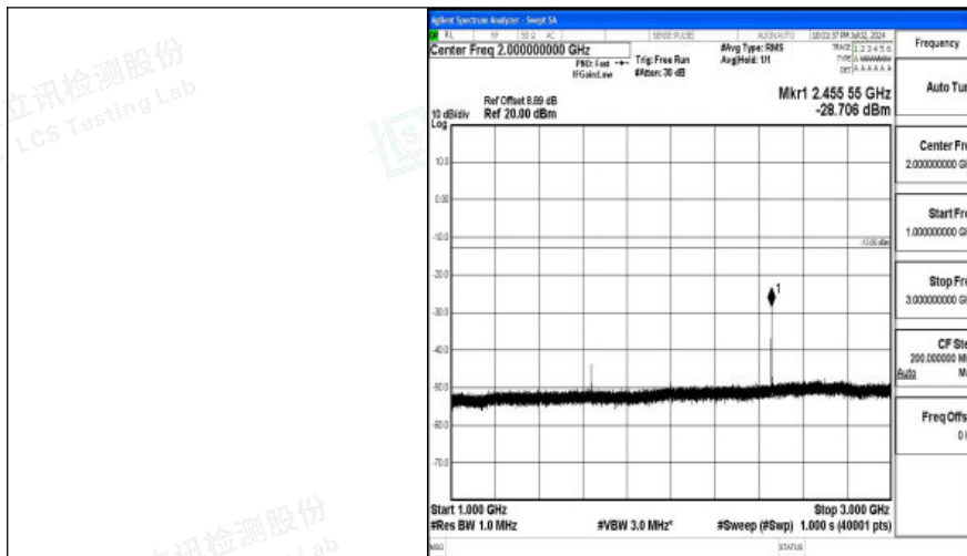
Band26_1.4MHz_16QAM_26740_1RB#0_1000~3000_1000~3000
