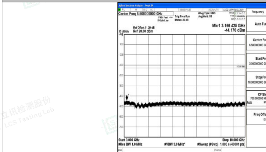
Band26_5MHz_16QAM_26740_1RB#0_3000~10000_3000~10000
