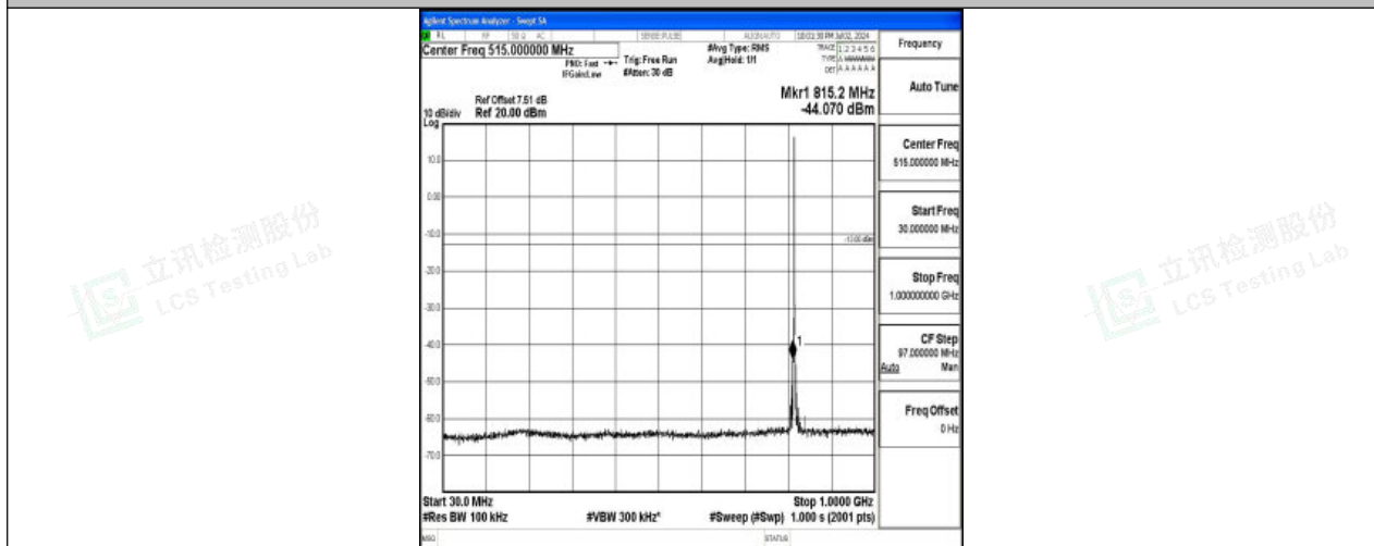
Band26_1.4MHz_16QAM_26740_1RB#0_30~1000_30~1000
