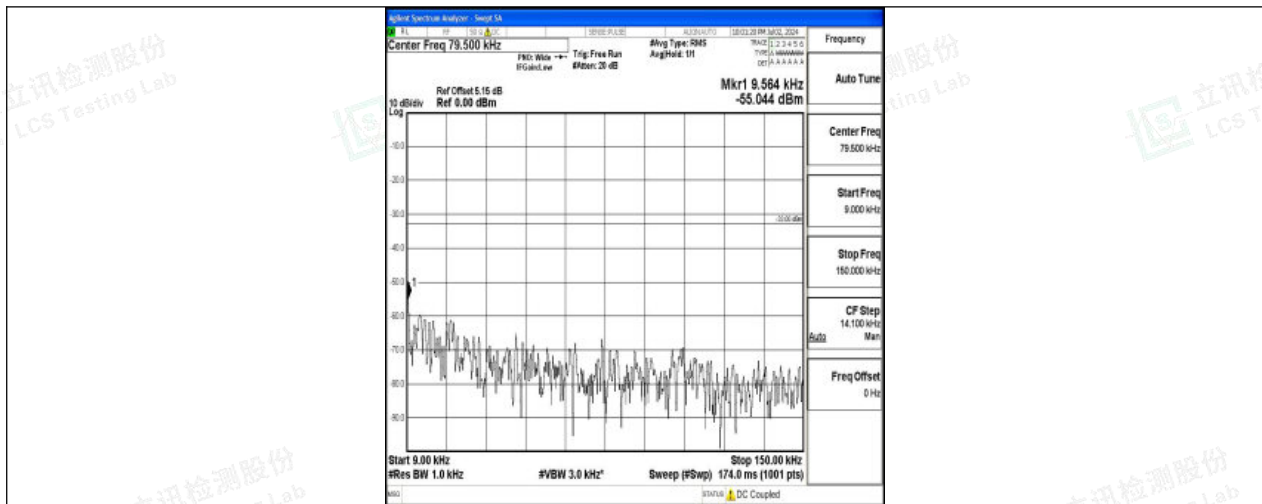
Band26_1.4MHz_16QAM_26740_1RB#0_0.009~0.15_0.009~0.15
