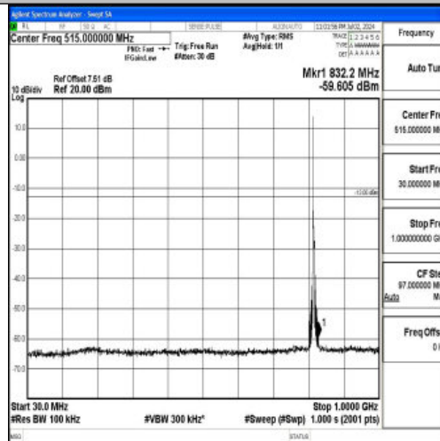
Band26_5MHz_16QAM_26740_1RB#0_30~1000_30~1000
