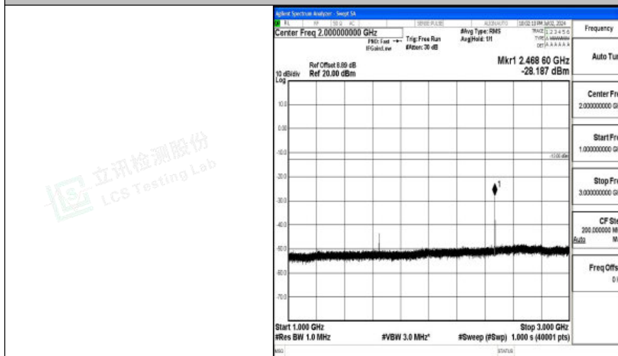
Band26_1.4MHz_QPSK_26783_1RB#0_1000~3000_1000~3000
