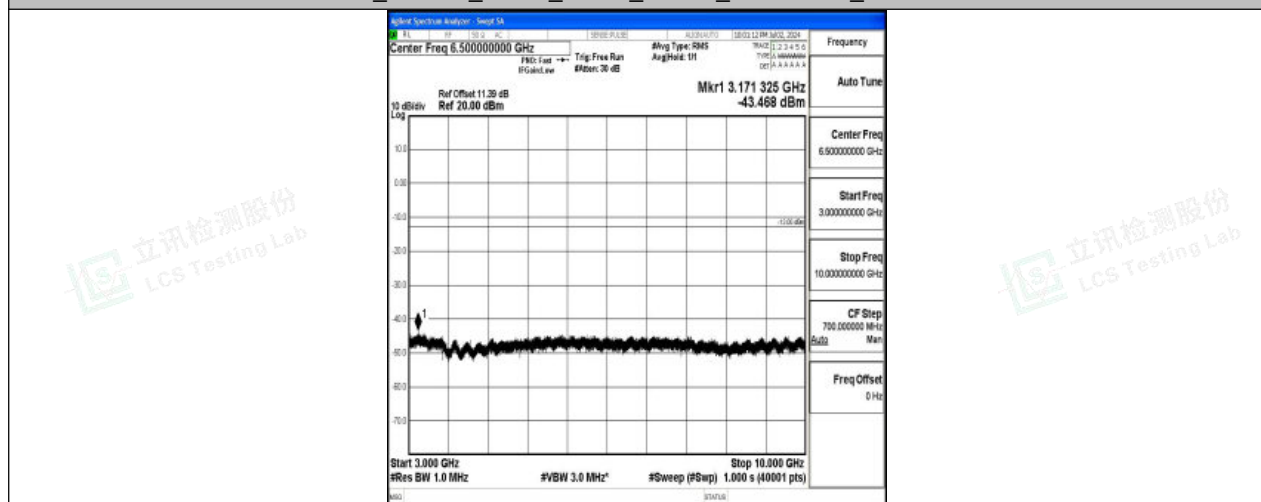
Band26_1.4MHz_QPSK_26740_1RB#0_3000~10000_3000~10000
