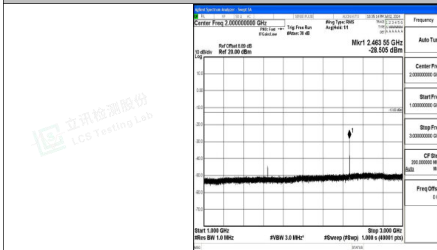
Band26_3MHz_QPSK_26775_1RB#0_1000~3000_1000~3000
