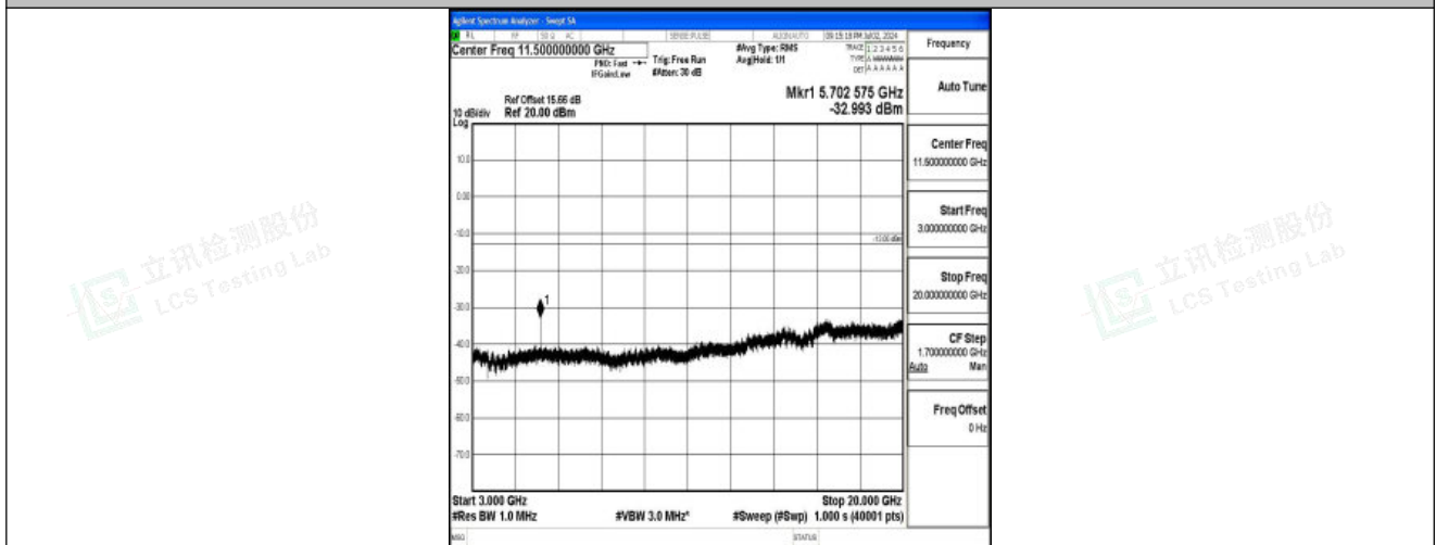
Band25_15MHz_16QAM_26615_1RB#0_3000~20000_3000~20000
