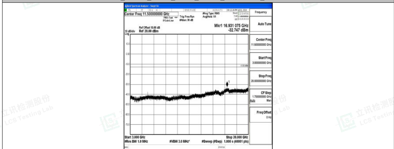
Band25_15MHz_QPSK_26115_1RB#0_3000~20000_3000~20000
