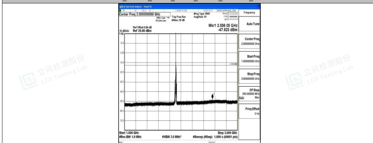
Band25_10MHz_QPSK_26640_1RB#0_1000~3000_1000~3000
