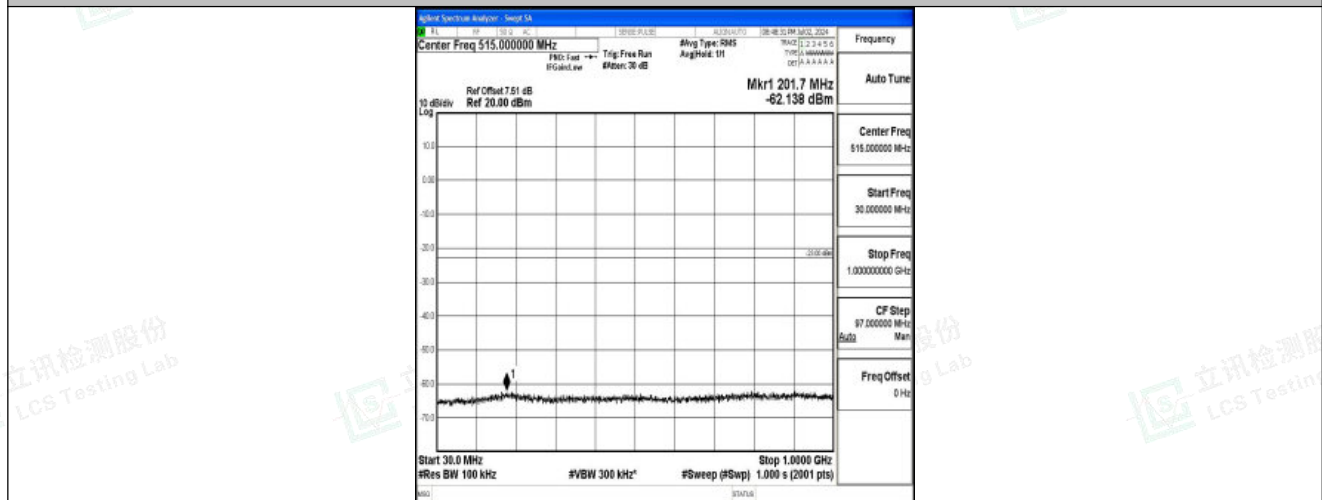
Band25_10MHz_16QAM_26090_1RB#0_30~1000_30~1000
