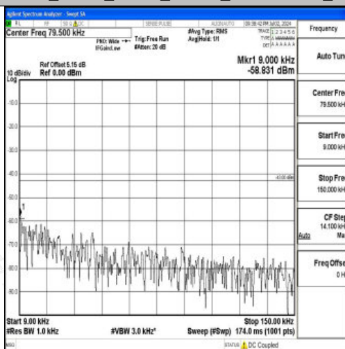
Band25_20MHz_16QAM_26590_1RB#0_0.009~0.15_0.009~0.15
