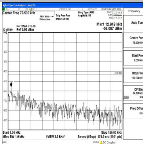
Band25_10MHz_QPSK_26365_1RB#0_0.009~0.15_0.009~0.15
