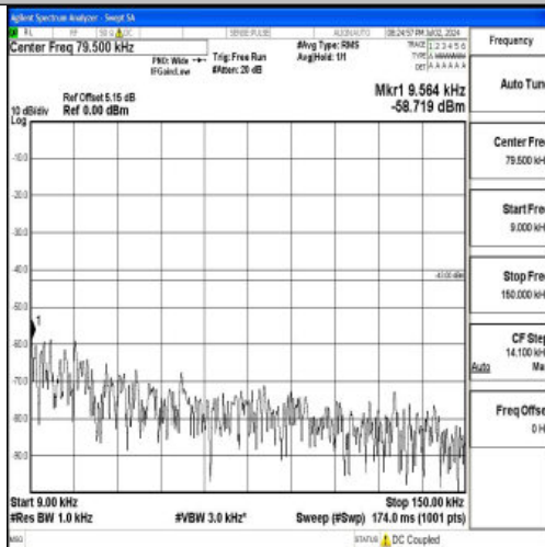
Band25_5MHz_QPSK_26665_1RB#0_0.009~0.15_0.009~0.15
