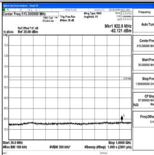
Band25_20MHz_QPSK_26590_1RB#0_30~1000_30~1000
