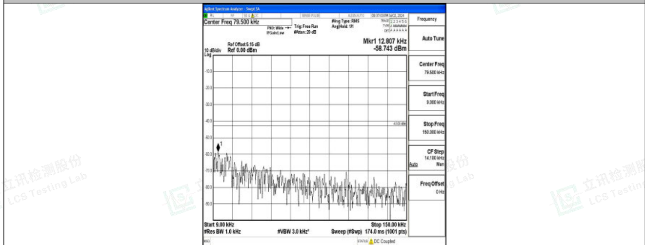
Band25_20MHz_QPSK_26365_1RB#0_0.009~0.15_0.009~0.15
