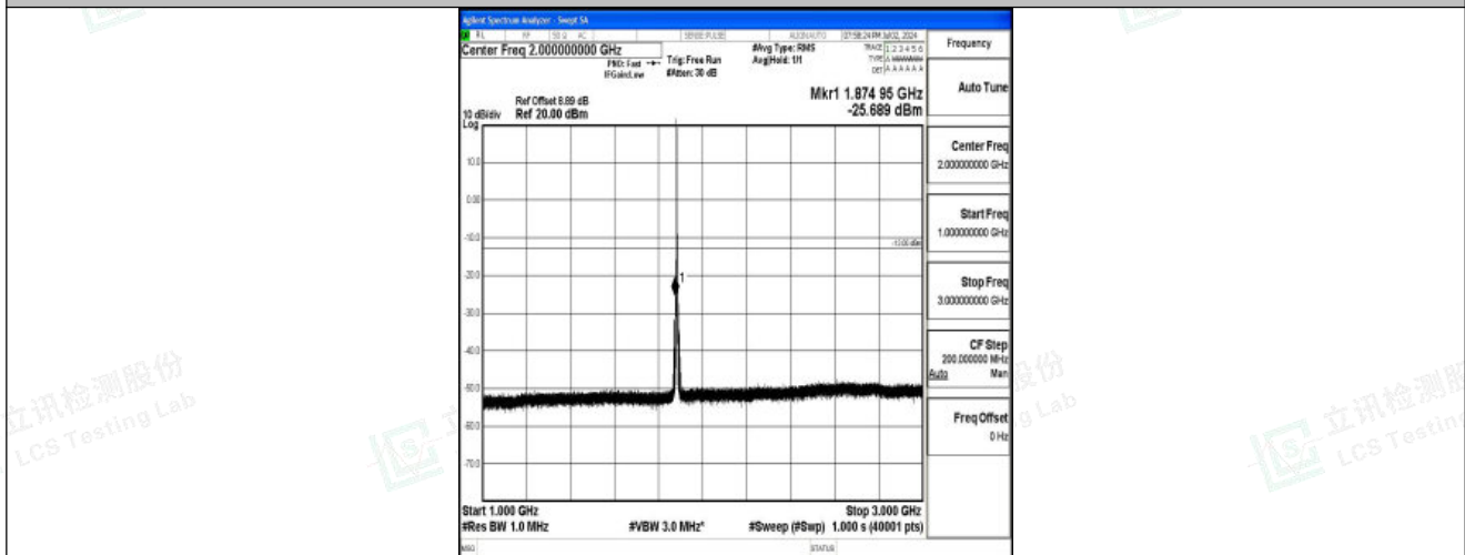
Band25_3MHz_QPSK_26365_1RB#0_1000~3000_1000~3000
