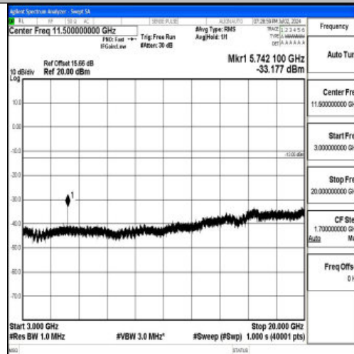
Band25_1.4MHz_16QAM_26683_1RB#0_3000~20000_3000~20000
