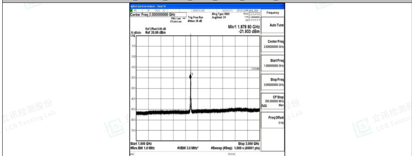
Band25_1.4MHz_QPSK_26365_1RB#0_1000~3000_1000~3000
