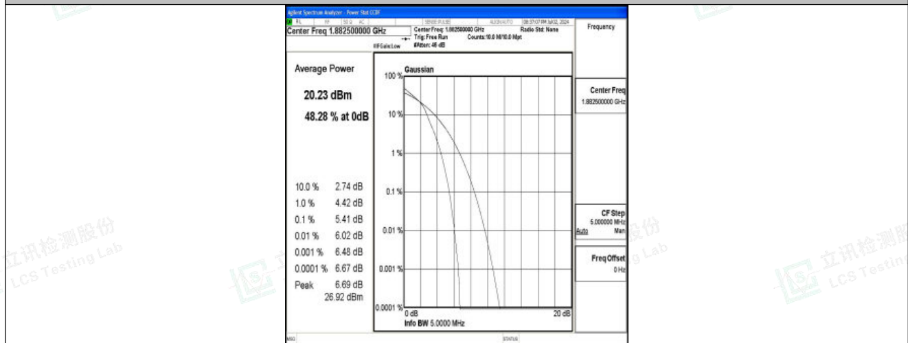
Band25-5MHz-16QAM-26365-25RB#0-PASS
