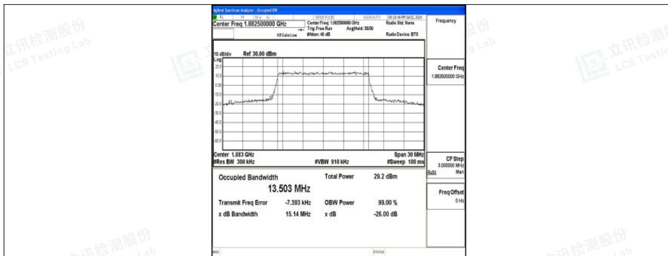
Band25-15MHz-16QAM-26365-75RB#0-PASS
