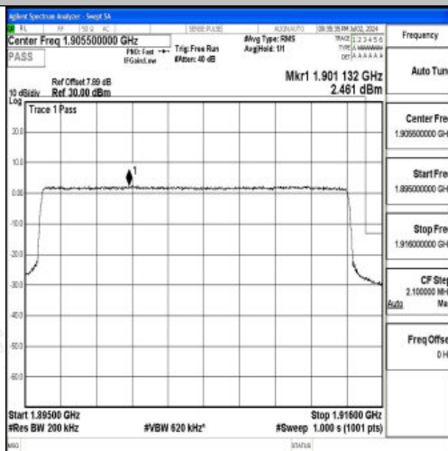
Band25_20MHz_QPSK_26590_100RB#0
