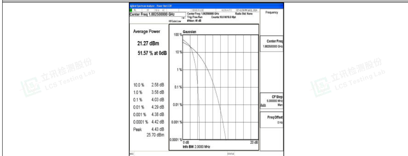
Band25-1.4MHz-16QAM-26365-1RB#0-PASS
