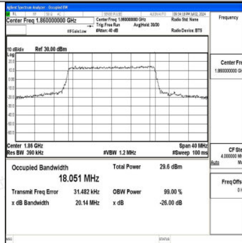
Band25-20MHz-16QAM-26140-100RB#0-PASS
