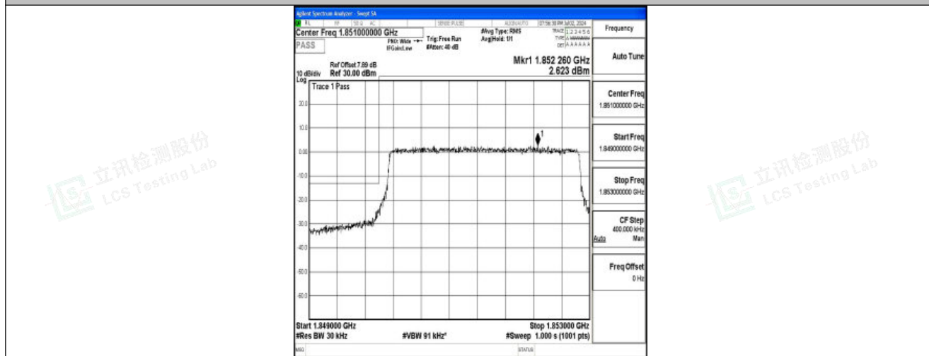
Band25_3MHz_16QAM_26055_15RB#0
