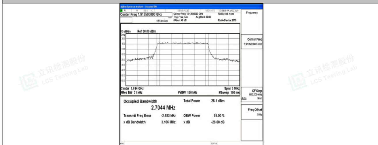
Band25-3MHz-16QAM-26675-15RB#0-PASS
