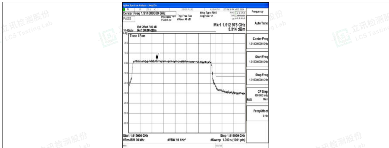
Band25_3MHz_QPSK_26675_15RB#0
