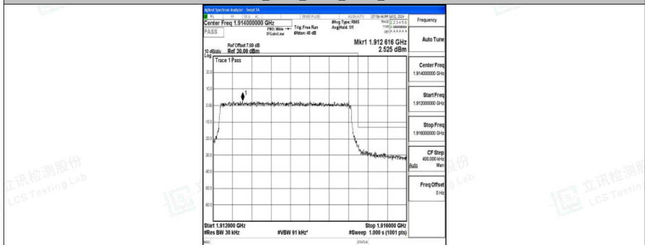
Band25_3MHz_16QAM_26675_15RB#0
