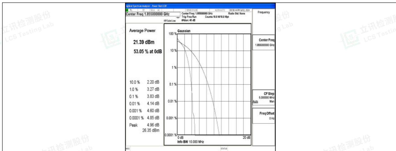
Band25-10MHz-QPSK-26090-1RB#0-PASS
