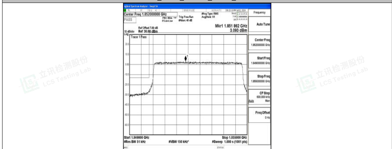
Band25_5MHz_QPSK_26065_25RB#0
