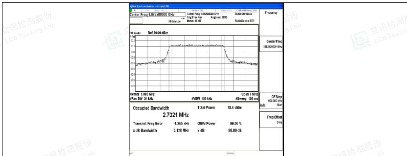
Band25-3MHz-16QAM-26365-15RB#0-PASS
