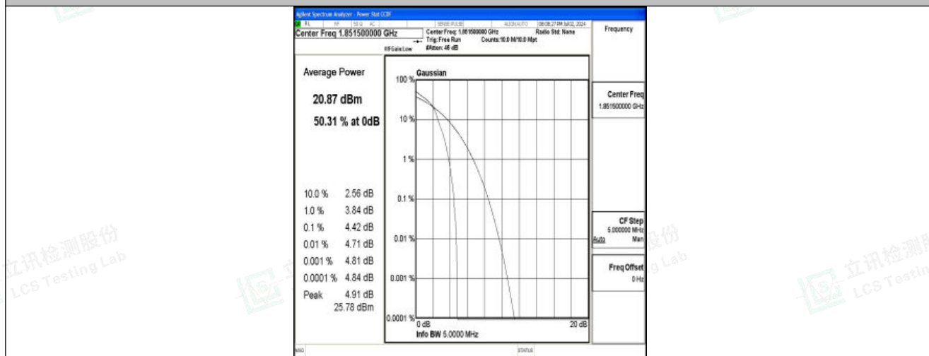
Band25-3MHz-16QAM-26055-1RB#0-PASS
