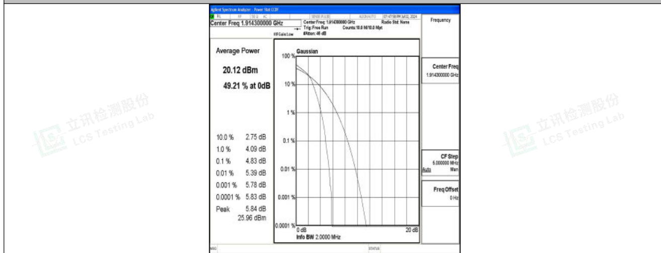
Band25-1.4MHz-16QAM-26683-6RB#0-PASS
