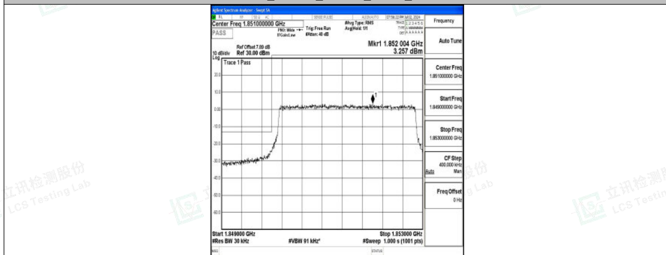
Band25_3MHz_QPSK_26055_15RB#0
