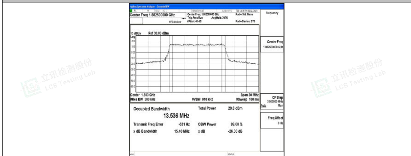
Band25-15MHz-QPSK-26365-75RB#0-PASS
