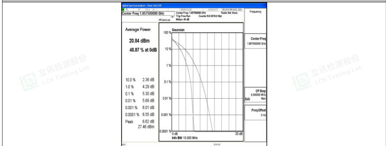
Band25-15MHz-QPSK-26115-75RB#0-PASS
