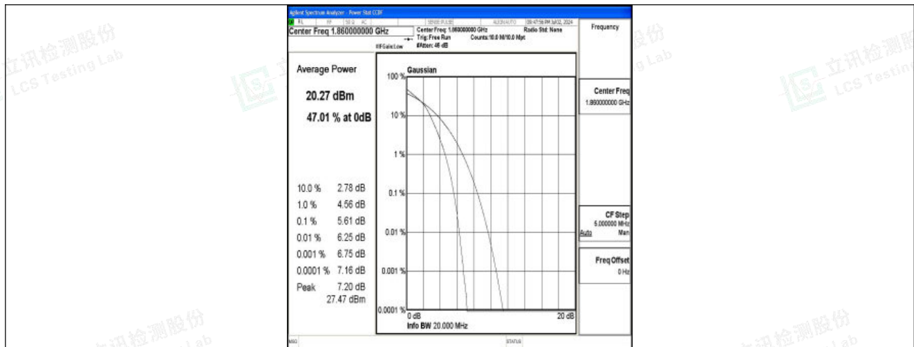
Band25-20MHz-16QAM-26140-100RB#0-PASS
