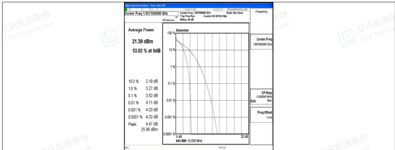
Band25-15MHz-QPSK-26115-1RB#0-PASS
