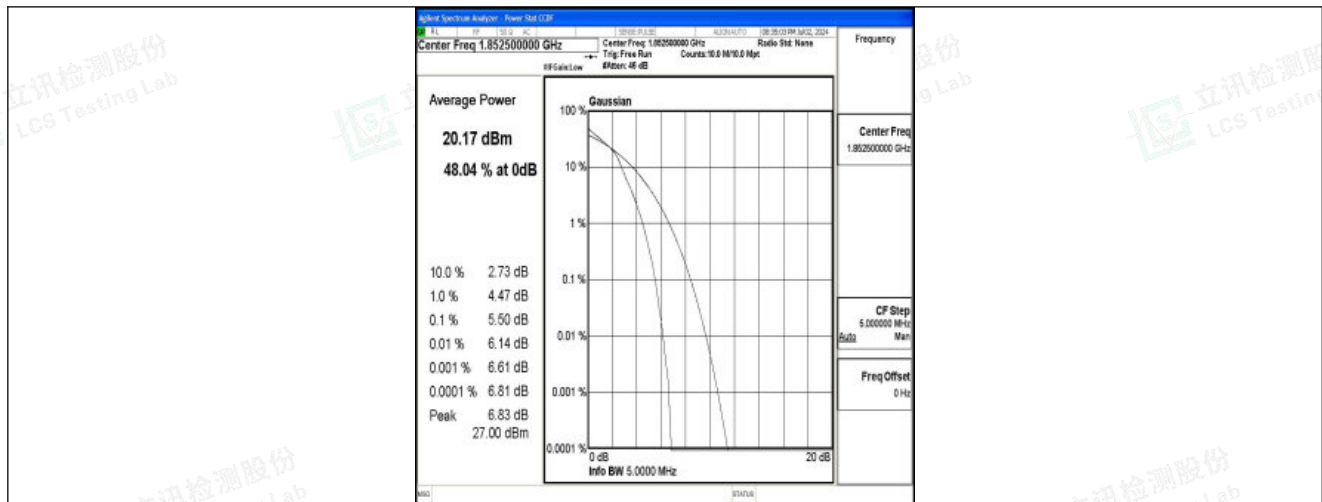
Band25-5MHz-16QAM-26065-25RB#0-PASS
