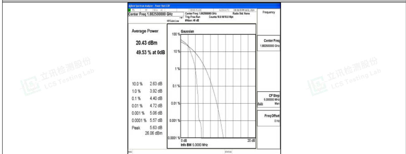
Band25-5MHz-16QAM-26365-1RB#0-PASS
