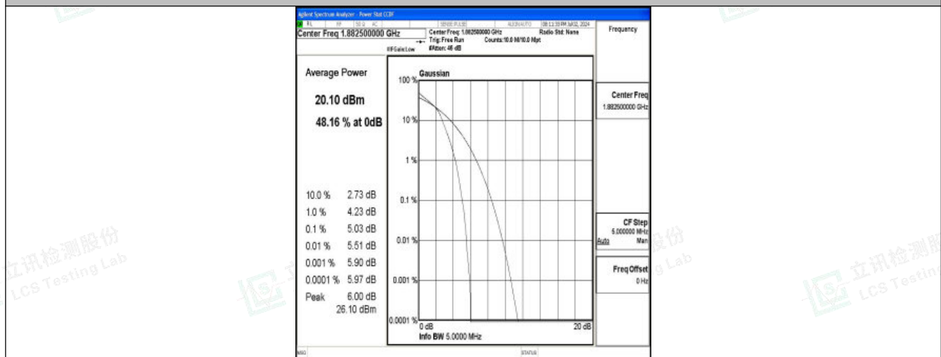
Band25-3MHz-16QAM-26365-15RB#0-PASS
