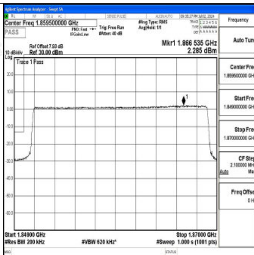
Band25_20MHz_16QAM_26140_100RB#0
