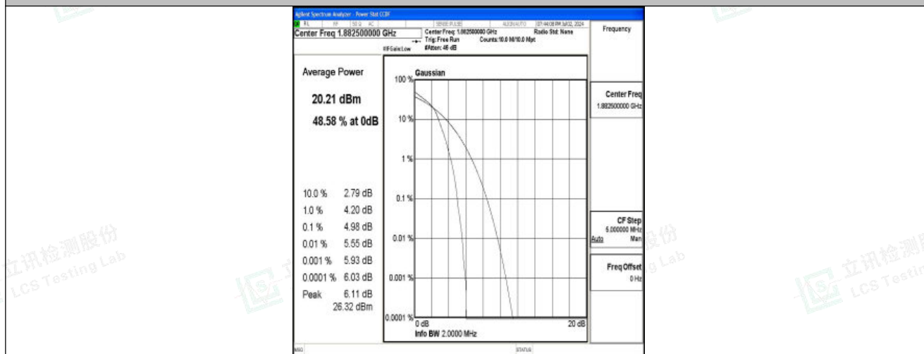
Band25-1.4MHz-16QAM-26365-6RB#0-PASS
