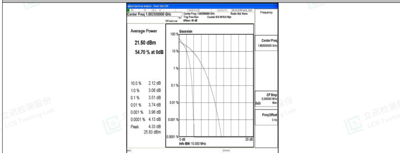
Band25-15MHz-QPSK-26365-1RB#0-PASS
