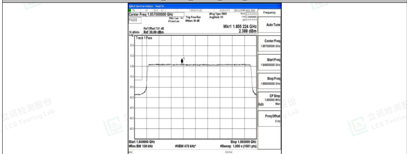
Band25_15MHz_QPSK_26115_75RB#0
