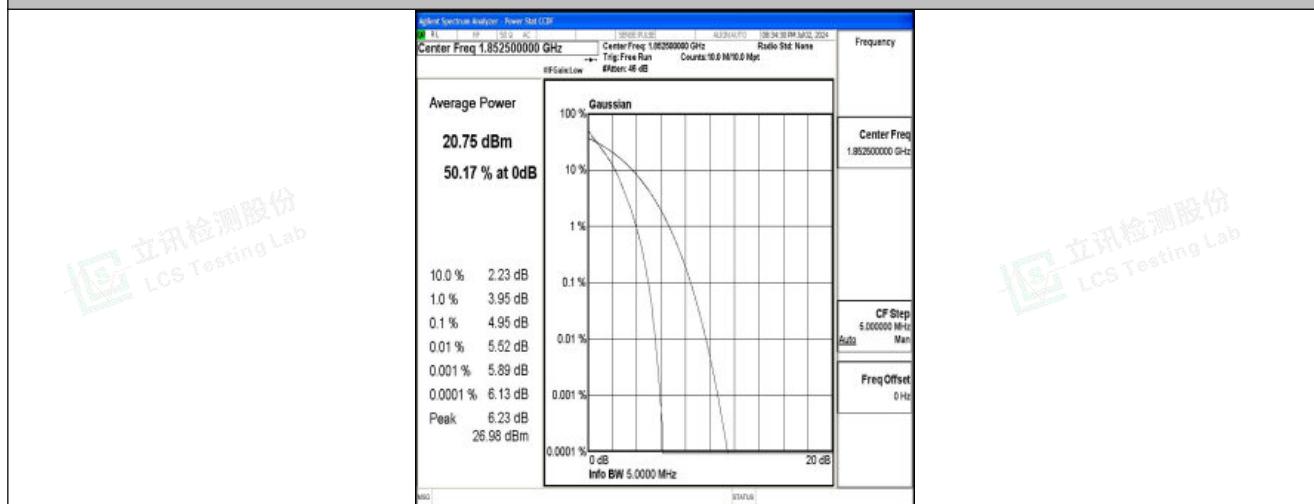
Band25-5MHz-QPSK-26065-25RB#0-PASS
