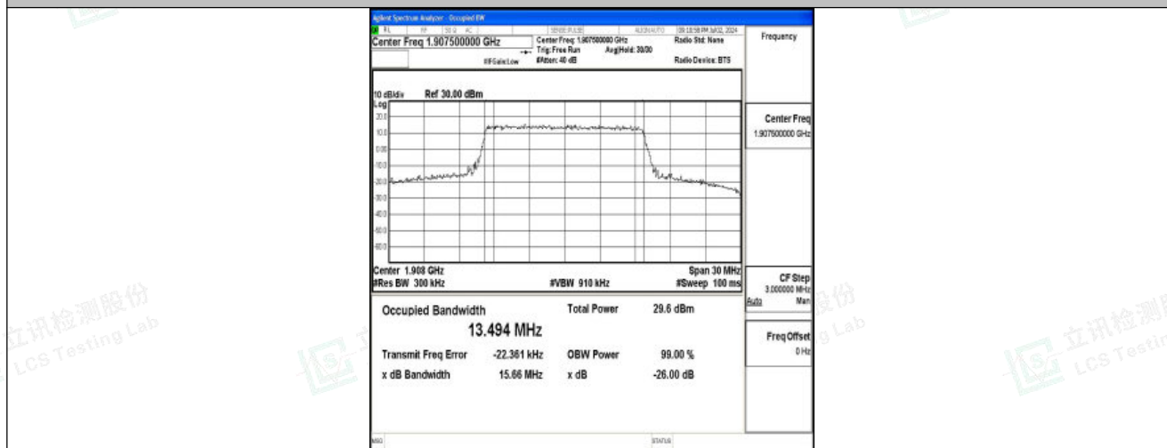
Band25-15MHz-QPSK-26615-75RB#0-PASS
