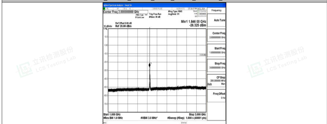
Band25_1.4MHz_16QAM_26047_1RB#0_1000~3000_1000~3000
