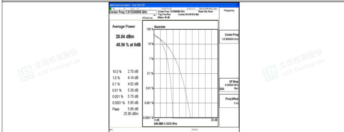
Band25-3MHz-16QAM-26675-15RB#0-PASS
