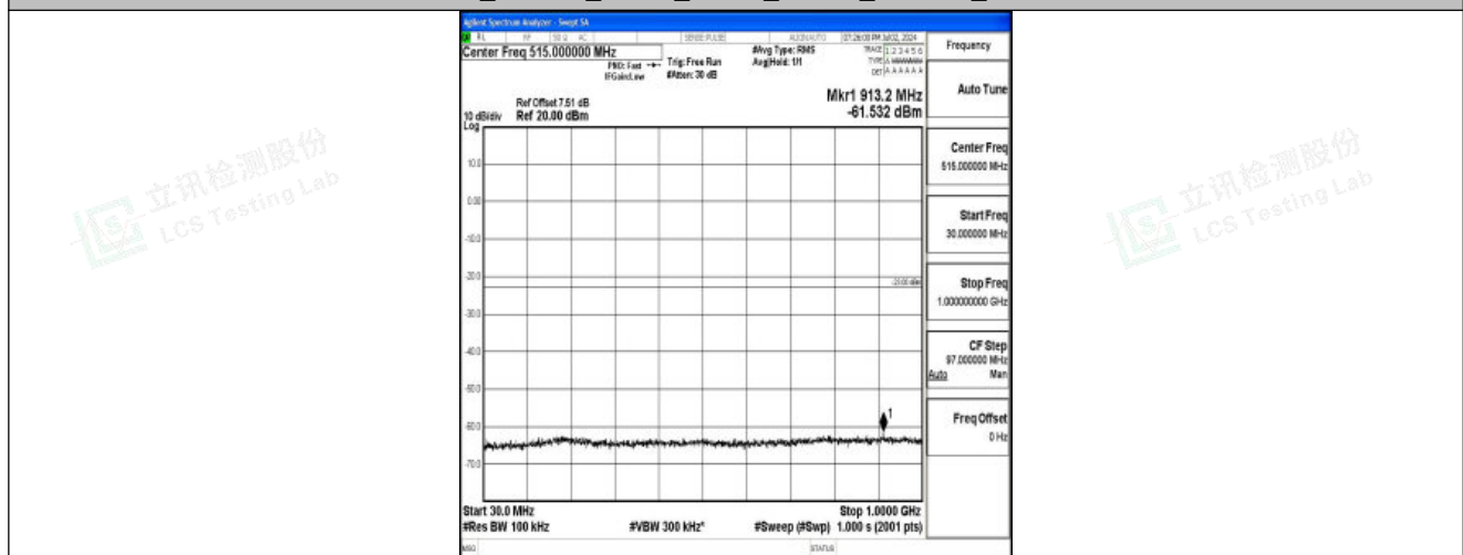
Band25_1.4MHz_QPSK_26047_1RB#0_30~1000_30~1000
