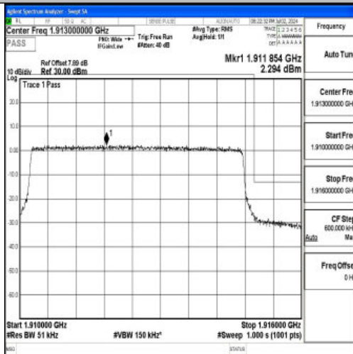
Band25_5MHz_16QAM_26665_25RB#0
