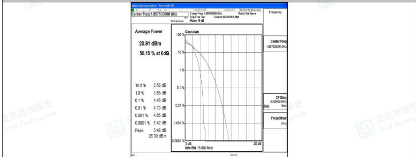
Band25-15MHz-16QAM-26115-1RB#0-PASS
