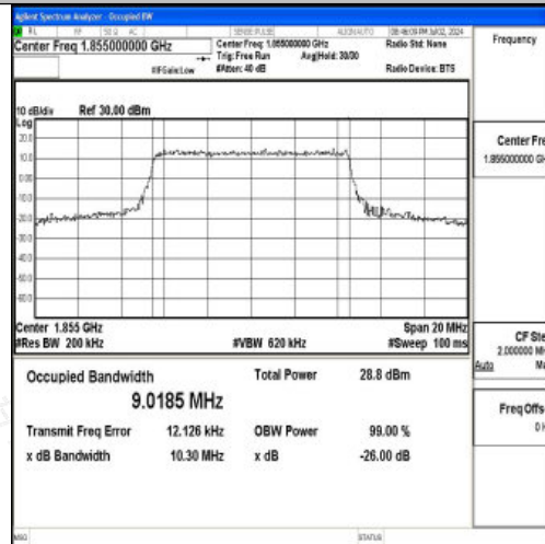
Band25-10MHz-16QAM-26090-50RB#0-PASS
