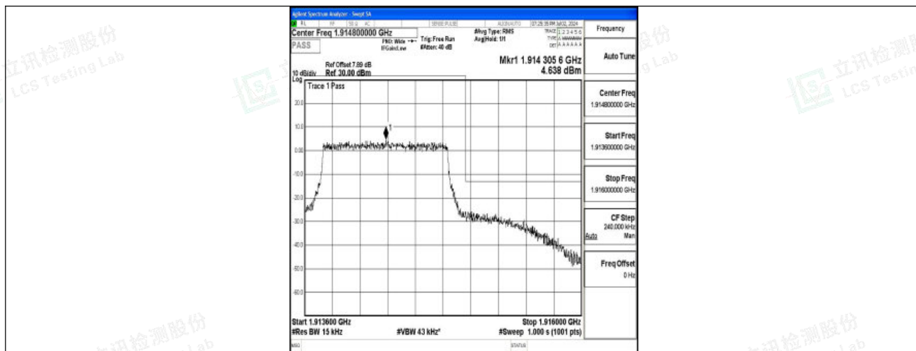
Band25_1.4MHz_16QAM_26683_6RB#0
