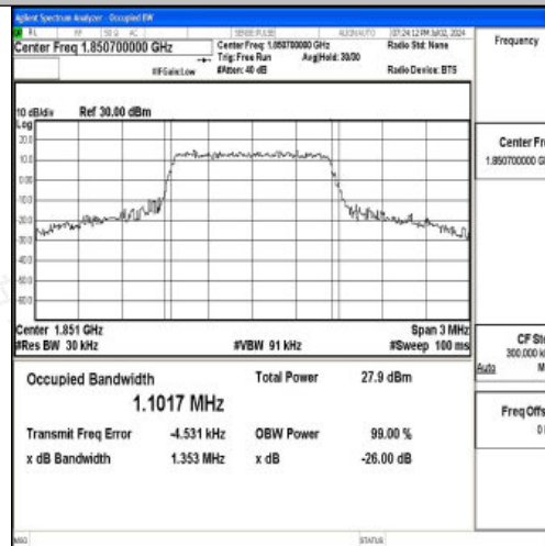
Band25-1.4MHz-16QAM-26047-6RB#0-PASS
