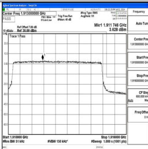
Band25_5MHz_QPSK_26665_25RB#0
