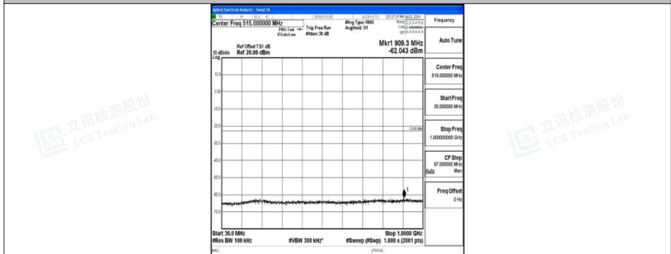
Band25_1.4MHz_16QAM_26365_1RB#0_30~1000_30~1000
