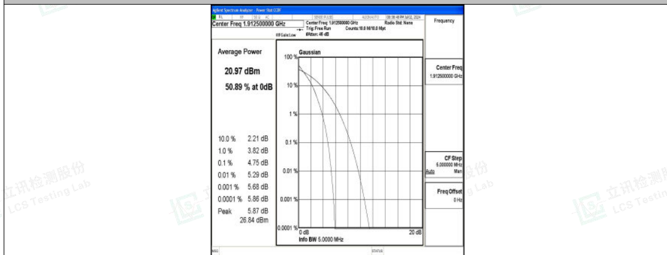
Band25-5MHz-QPSK-26665-25RB#0-PASS
