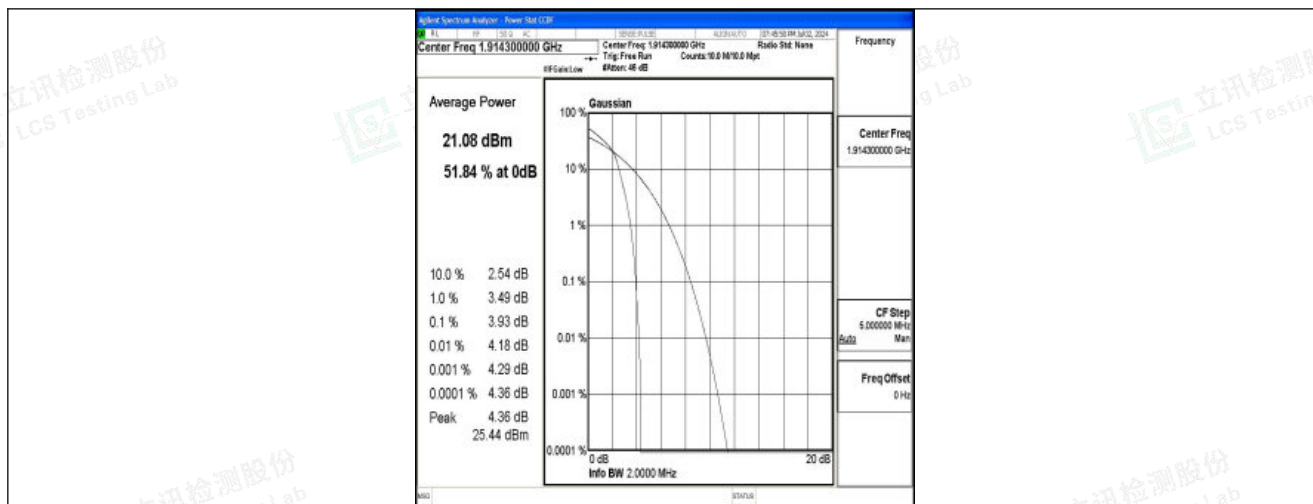
Band25-1.4MHz-16QAM-26683-1RB#0-PASS
