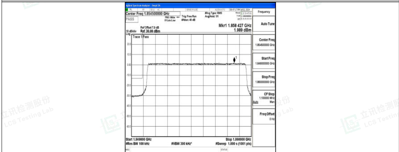
Band25_10MHz_16QAM_26090_50RB#0
