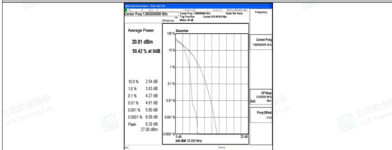
Band25-20MHz-16QAM-26140-1RB#0-PASS
