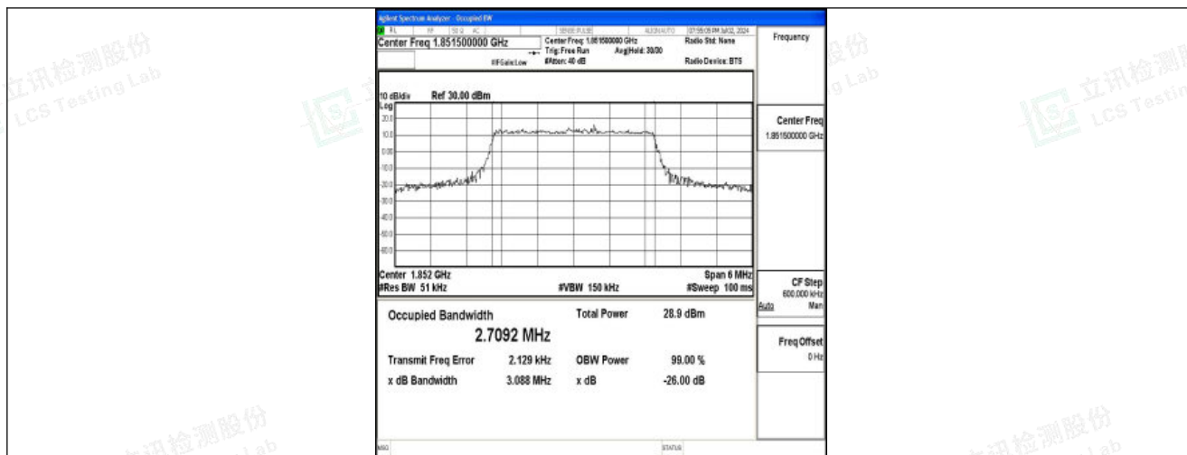
Band25-3MHz-QPSK-26055-15RB#0-PASS
