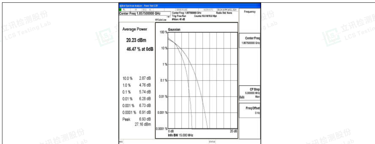
Band25-15MHz-16QAM-26115-75RB#0-PASS
