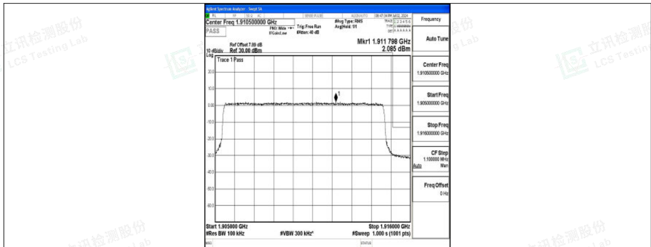
Band25_10MHz_16QAM_26640_50RB#0
