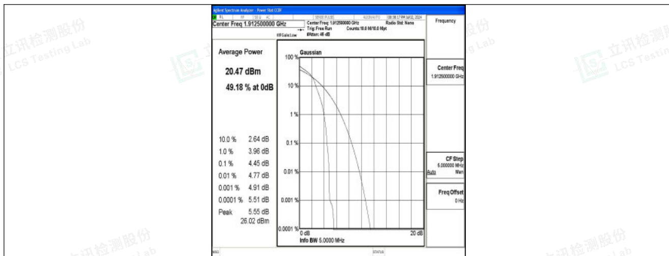
Band25-5MHz-16QAM-26665-1RB#0-PASS
