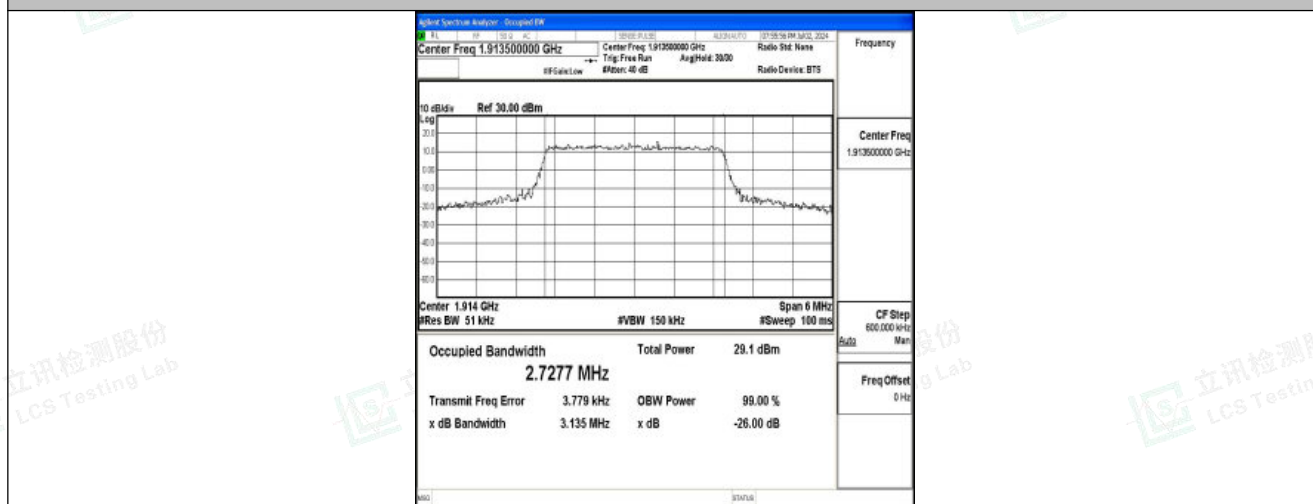
Band25-3MHz-QPSK-26675-15RB#0-PASS
