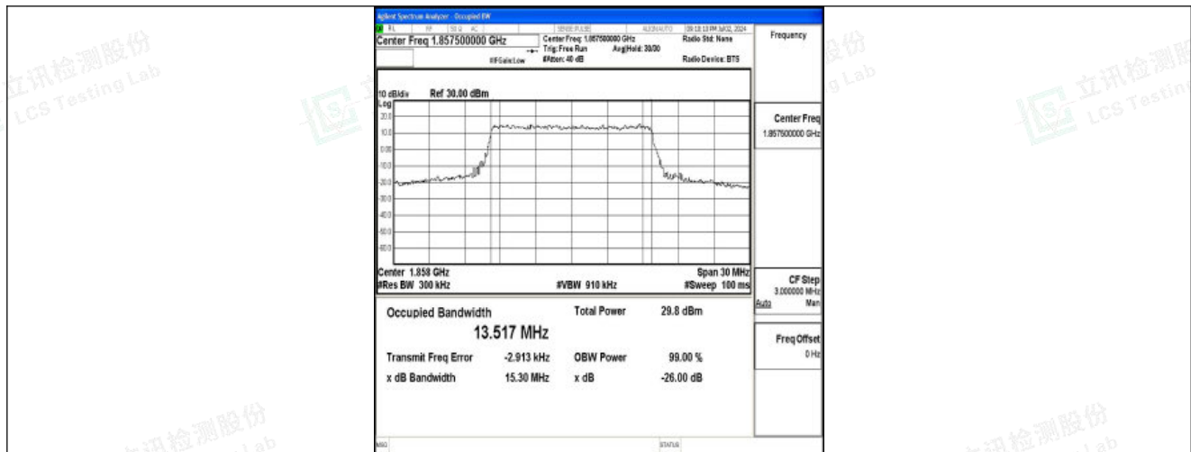
Band25-15MHz-QPSK-26115-75RB#0-PASS
