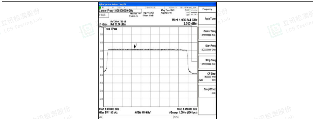
Band25_15MHz_QPSK_26615_75RB#0
