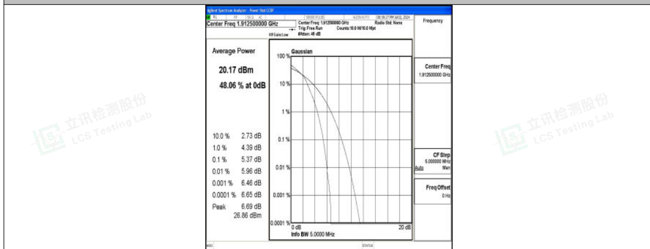
Band25-5MHz-16QAM-26665-25RB#0-PASS
