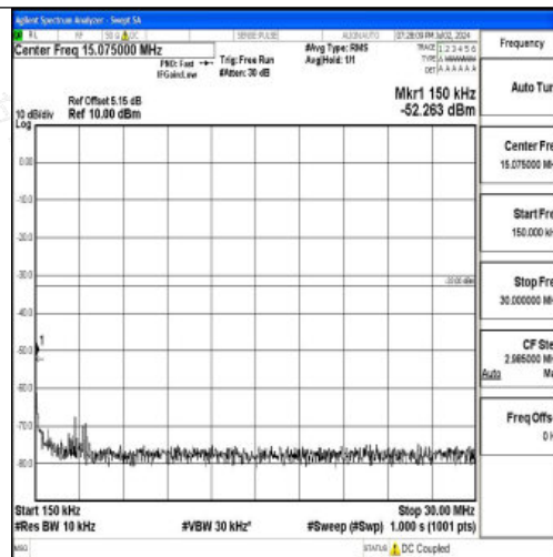
Band25_1.4MHz_QPSK_26683_1RB#0_0.15~30_0.15~30
