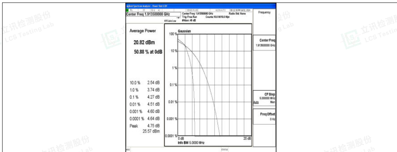
Band25-3MHz-16QAM-26675-1RB#0-PASS
