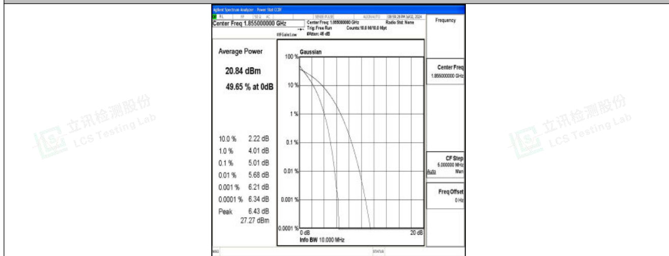
Band25-10MHz-QPSK-26090-50RB#0-PASS
