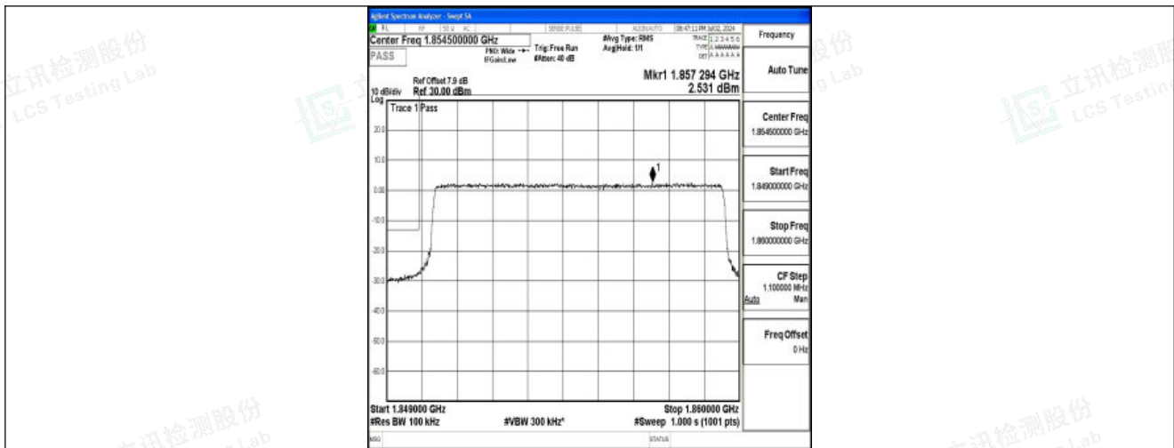
Band25_10MHz_QPSK_26090_50RB#0
