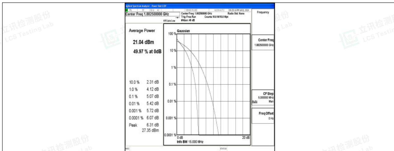
Band25-15MHz-QPSK-26365-75RB#0-PASS
