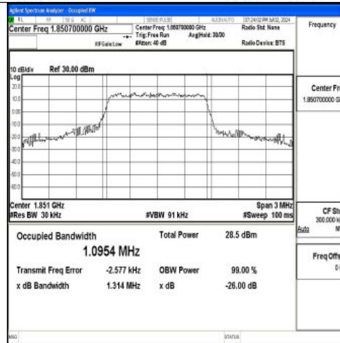
Band25-1.4MHz-QPSK-26047-6RB#0-PASS
