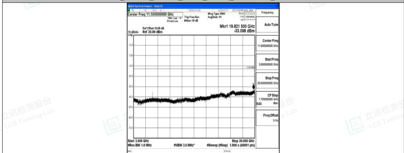
Band25_1.4MHz_16QAM_26365_1RB#0_3000~20000_3000~20000
