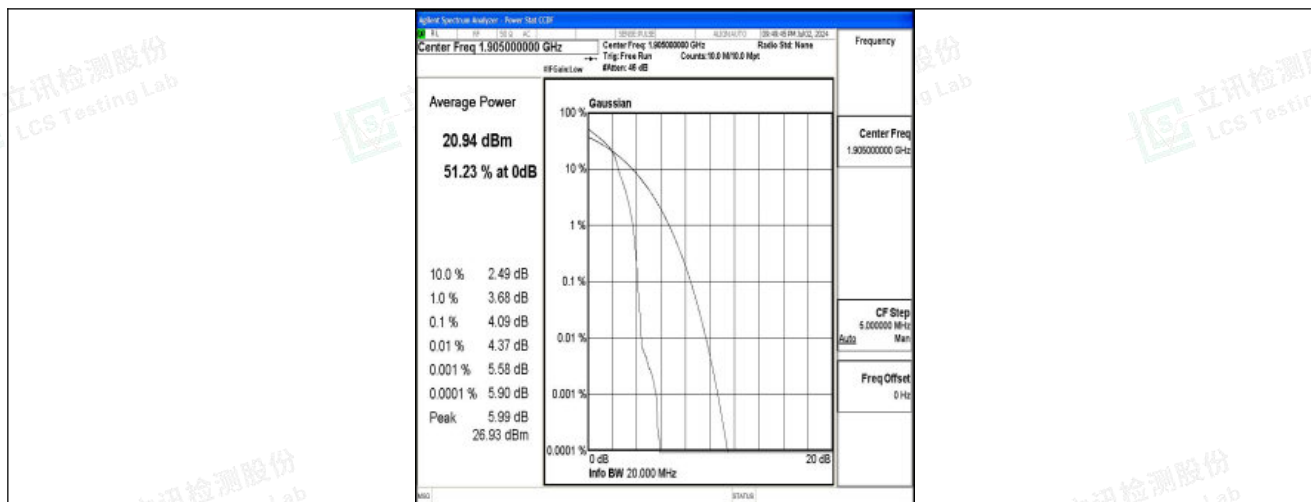
Band25-20MHz-16QAM-26590-1RB#0-PASS
