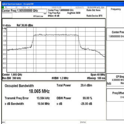
Band25-20MHz-16QAM-26590-100RB#0-PASS
