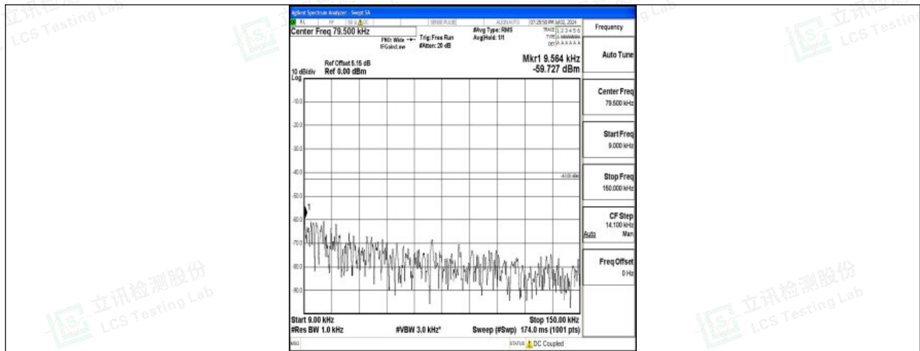
Band25_1.4MHz_QPSK_26047_1RB#0_0.009~0.15_0.009~0.15
