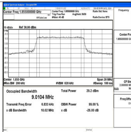
Band25-10MHz-QPSK-26090-50RB#0-PASS
