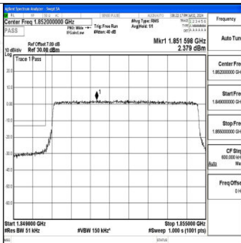
Band25_5MHz_16QAM_26065_25RB#0
