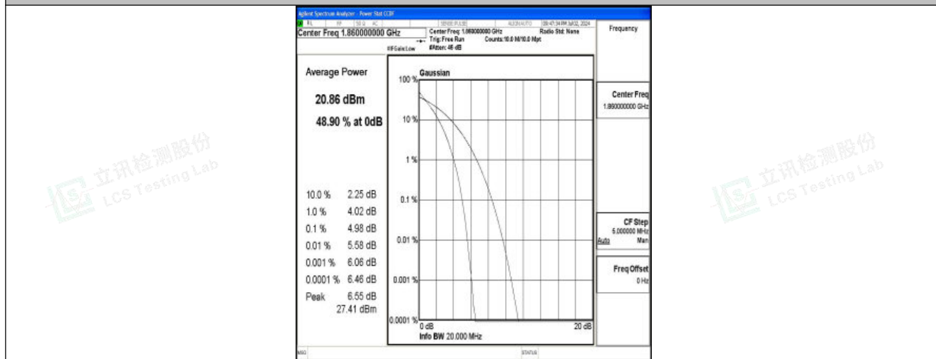
Band25-20MHz-QPSK-26140-100RB#0-PASS
