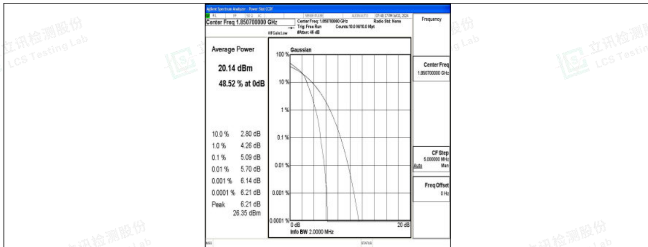
Band25-1.4MHz-16QAM-26047-6RB#0-PASS
