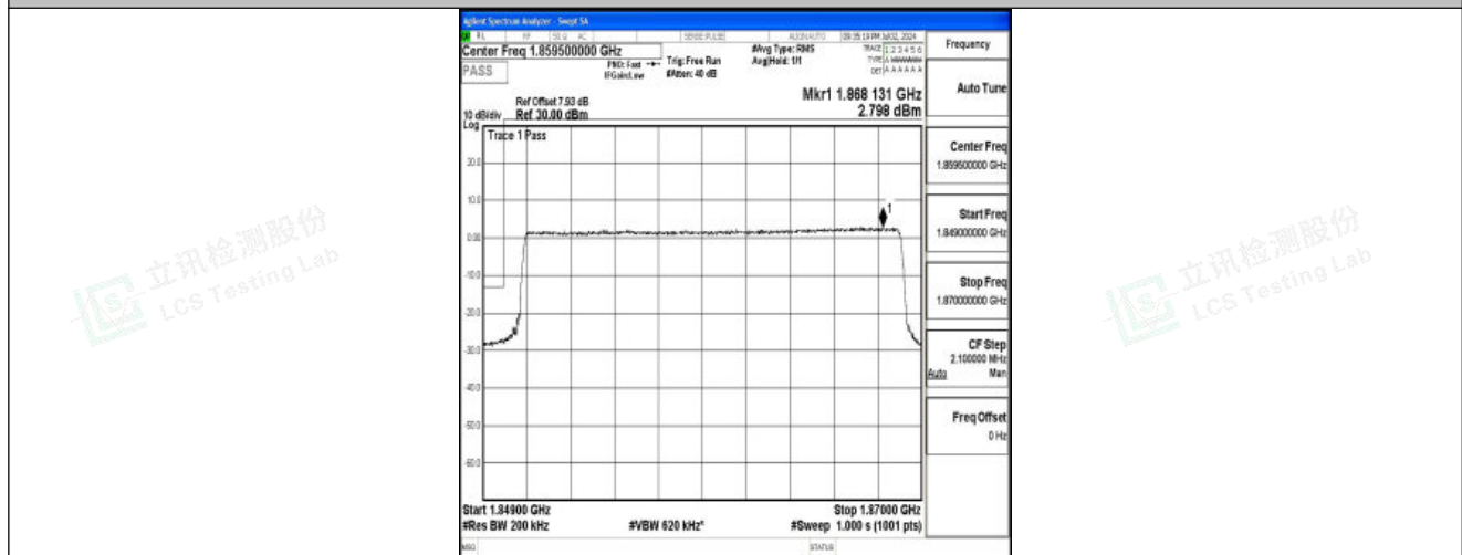
Band25_20MHz_QPSK_26140_100RB#0
