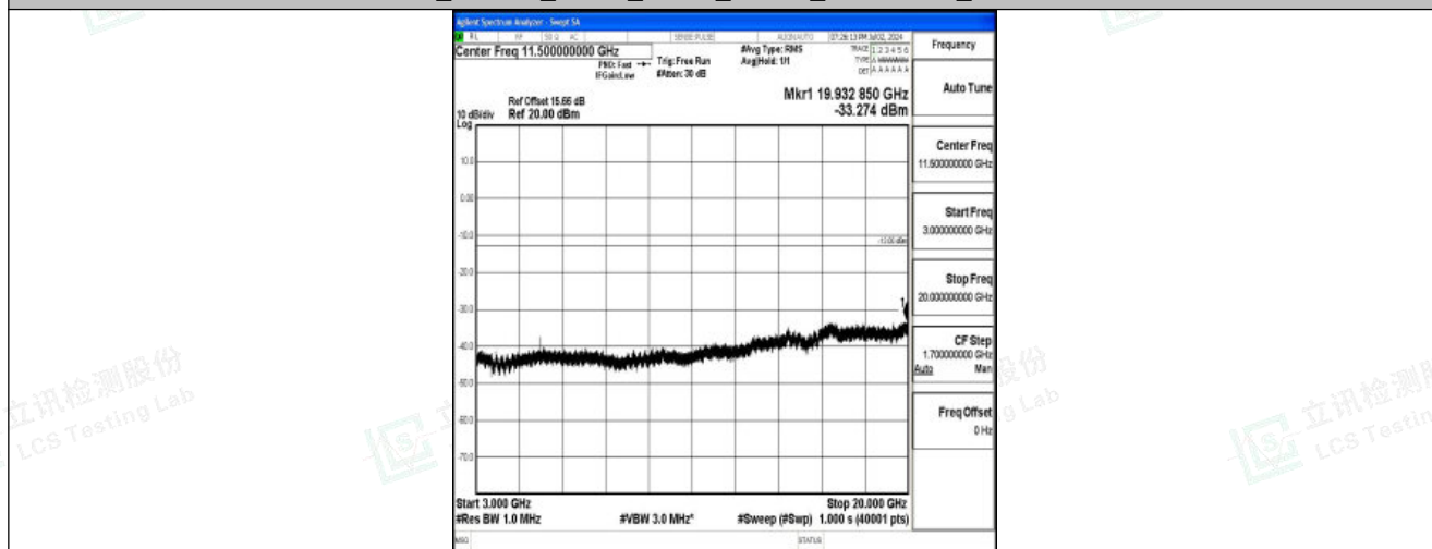
Band25_1.4MHz_QPSK_26047_1RB#0_3000~20000_3000~20000
