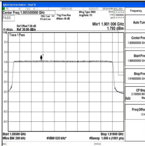
Band25_20MHz_16QAM_26590_100RB#0
