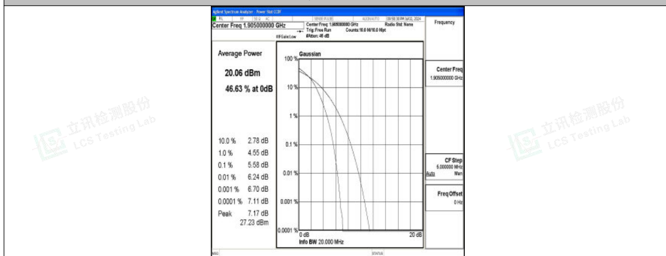
Band25-20MHz-16QAM-26590-100RB#0-PASS
