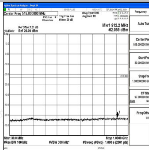
Band25_1.4MHz_QPSK_26683_1RB#0_30~1000_30~1000
