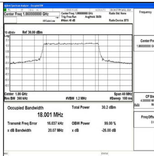
Band25-20MHz-QPSK-26140-100RB#0-PASS
