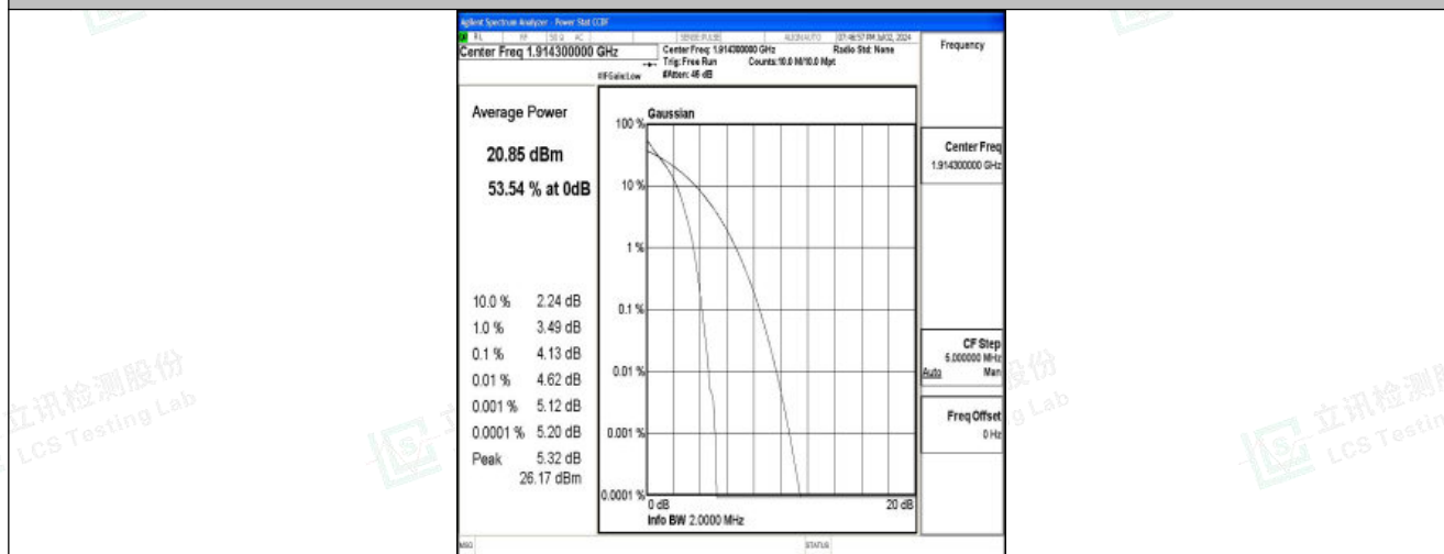
Band25-1.4MHz-QPSK-26683-6RB#0-PASS
