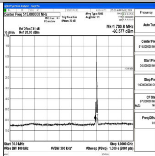
Band12_5MHz_QPSK_23155_1RB#0_30~1000_30~1000
