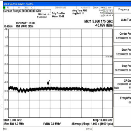
Band12_1.4MHz_QPSK_23173_1RB#0_3000~10000_3000~10000
