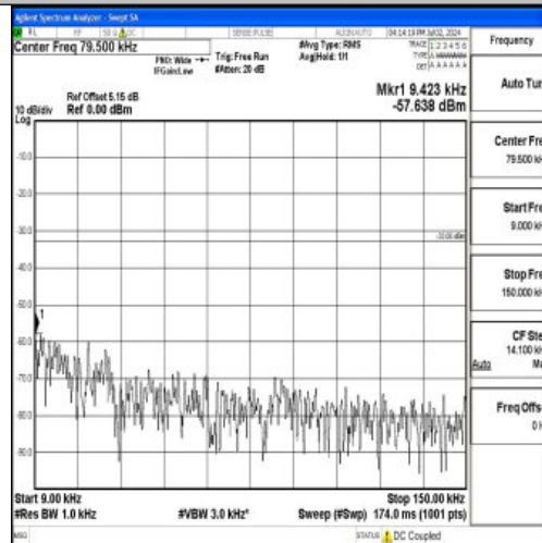
Band12_1.4MHz_16QAM_23173_1RB#0_0.009~0.15_0.009~0.15
