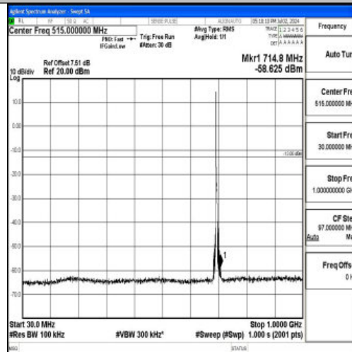
Band12_5MHz_16QAM_23035_1RB#0_30~1000_30~1000
