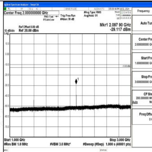
Band12_5MHz_QPSK_23035_1RB#0_1000~3000_1000~3000
