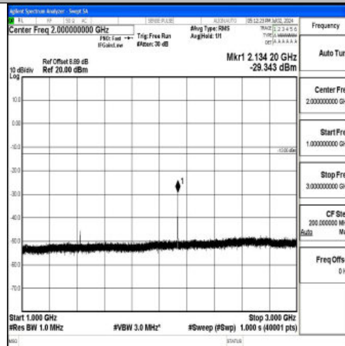
Band12_5MHz_16QAM_23155_1RB#0_1000~3000_1000~3000
