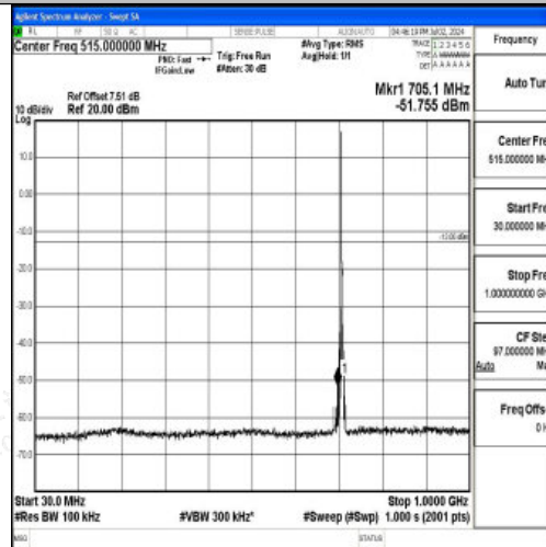
Band12_3MHz_16QAM_23165_1RB#0_30~1000_30~1000
