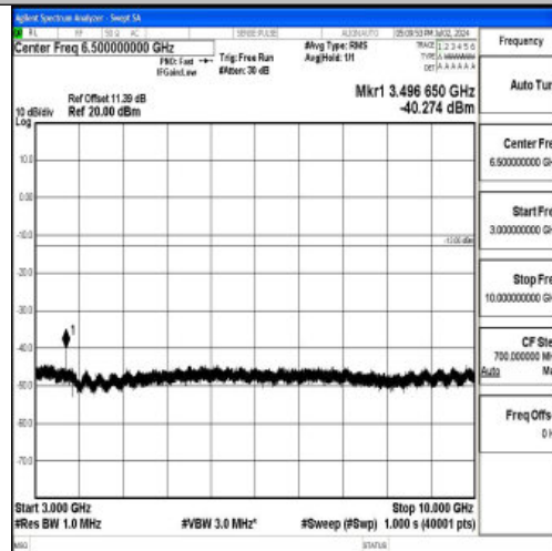
Band12_5MHz_QPSK_23035_1RB#0_3000~10000_3000~10000
