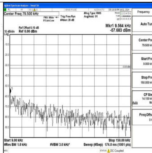
Band12_5MHz_16QAM_23035_1RB#0_0.009~0.15_0.009~0.15
