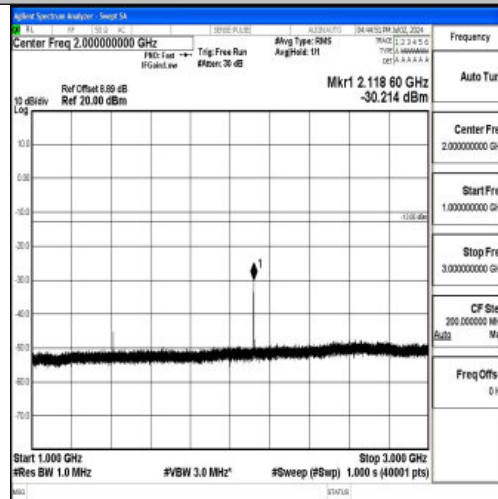
Band12_3MHz_QPSK_23095_1RB#0_1000~3000_1000~3000
