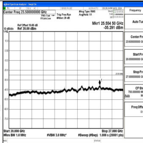
Band7_15MHz_QPSK_21375_1RB#0_20000~27000_20000~27000
