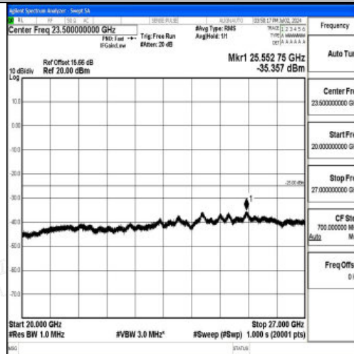
Band7_20MHz_16QAM_20850_1RB#0_20000~27000_20000~27000
