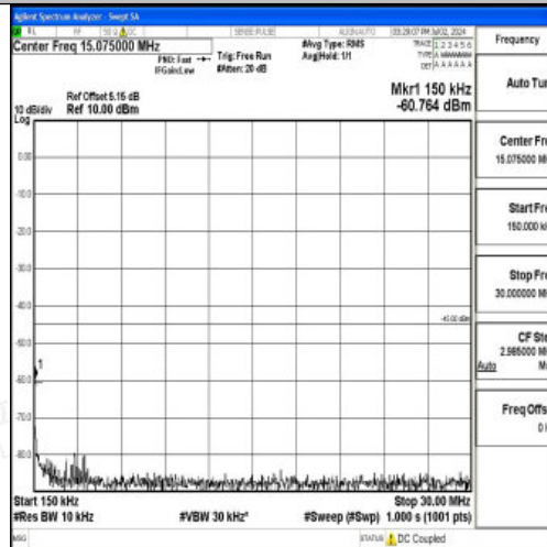
Band7_15MHz_QPSK_21375_1RB#0_0.15~30_0.15~30
