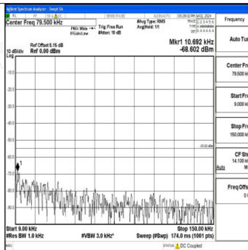
Band7_15MHz_QPSK_21375_1RB#0_0.009~0.15_0.009~0.15
