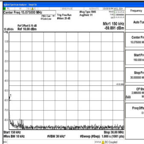
Band7_10MHz_16QAM_21100_1RB#0_0.15~30_0.15~30
