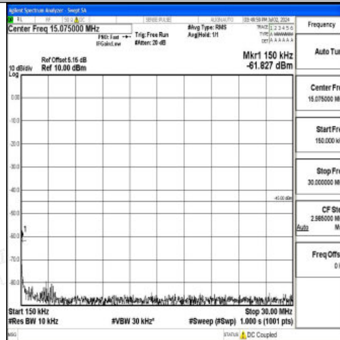
Band7_20MHz_16QAM_20850_1RB#0_0.15~30_0.15~30
