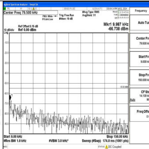
Band7_10MHz_QPSK_20800_1RB#0_0.009~0.15_0.009~0.15
