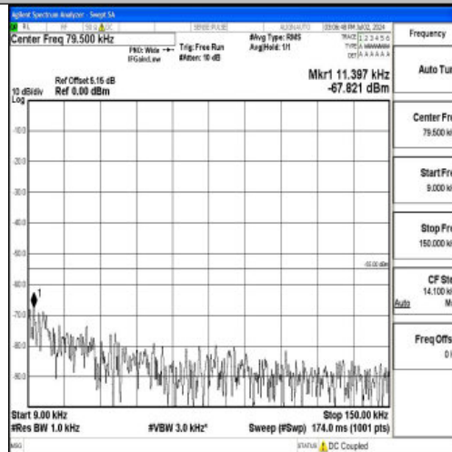
Band7_10MHz_16QAM_21400_1RB#0_0.009~0.15_0.009~0.15
