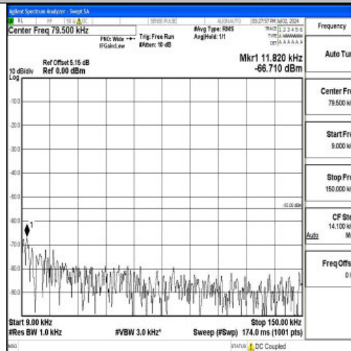
Band7_15MHz_QPSK_21100_1RB#0_0.009~0.15_0.009~0.15
