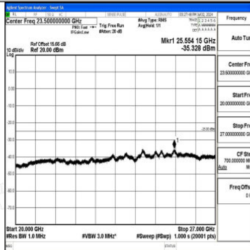
Band7_15MHz_16QAM_20825_1RB#0_20000~27000_20000~27000
