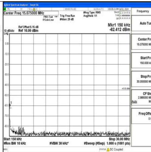
Band7_10MHz_QPSK_21100_1RB#0_0.15~30_0.15~30
