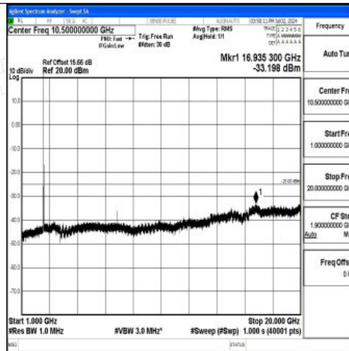
Band7_20MHz_16QAM_20850_1RB#0_1000~20000_1000~20000
