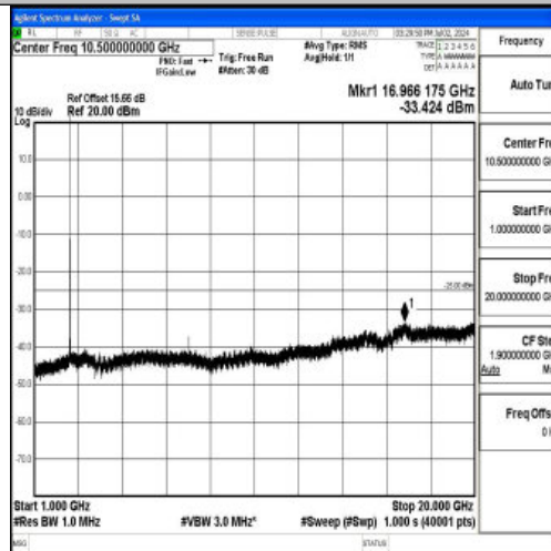
Band7_15MHz_16QAM_21375_1RB#0_1000~20000_1000~20000
