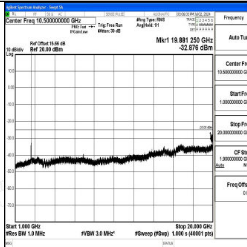
Band7_10MHz_16QAM_21100_1RB#0_1000~20000_1000~20000
