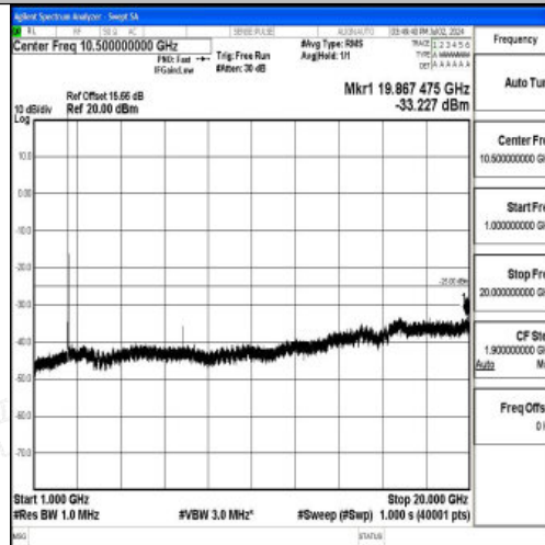
Band7_20MHz_QPSK_20850_1RB#0_1000~20000_1000~20000
