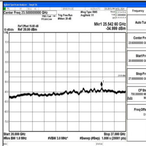
Band7_15MHz_16QAM_21100_1RB#0_20000~27000_20000~27000
