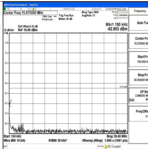
Band7_15MHz_QPSK_21100_1RB#0_0.15~30_0.15~30
