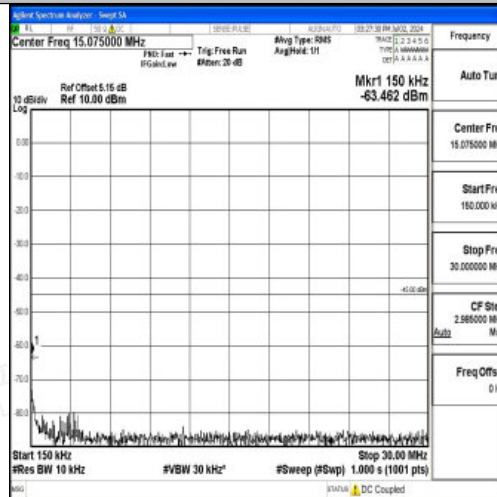
Band7_15MHz_16QAM_20825_1RB#0_0.15~30_0.15~30
