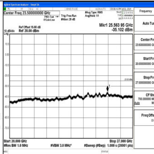
Band7_10MHz_QPSK_21400_1RB#0_20000~27000_20000~27000
