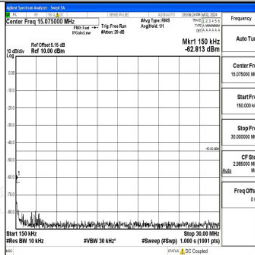
Band7_10MHz_QPSK_21400_1RB#0_0.15~30_0.15~30
