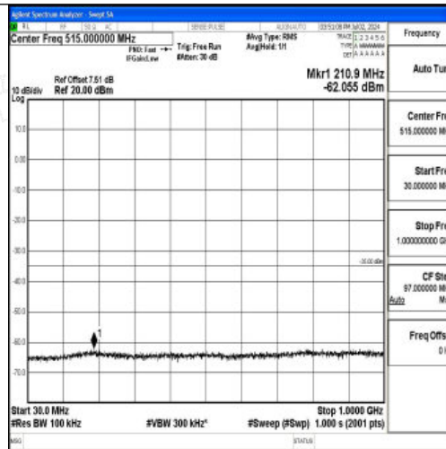
Band7_20MHz_16QAM_21100_1RB#0_30~1000_30~1000
