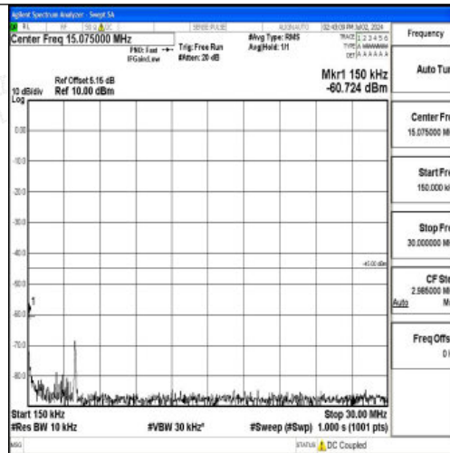
Band7_5MHz_16QAM_21425_1RB#0_0.15~30_0.15~30
