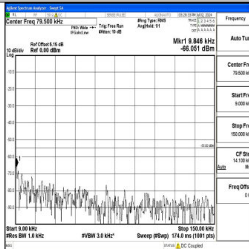
Band7_15MHz_16QAM_21375_1RB#0_0.009~0.15_0.009~0.15
