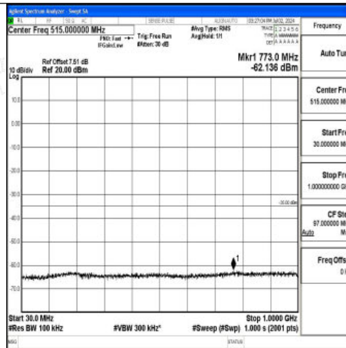
Band7_15MHz_QPSK_20825_1RB#0_30~1000_30~1000
