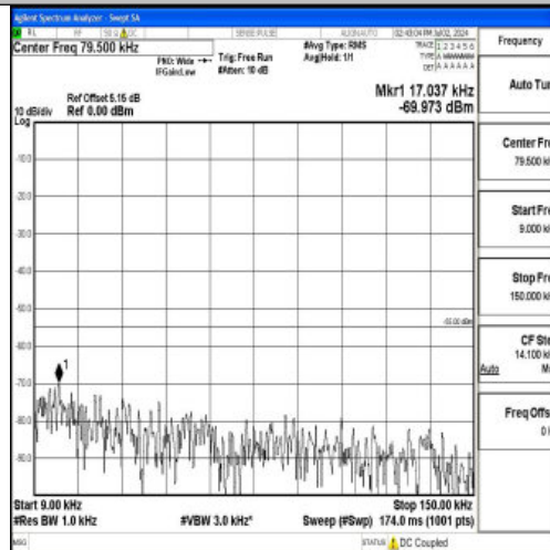
Band7_5MHz_16QAM_21425_1RB#0_0.009~0.15_0.009~0.15
