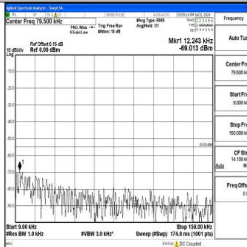
Band7_10MHz_QPSK_21100_1RB#0_0.009~0.15_0.009~0.15
