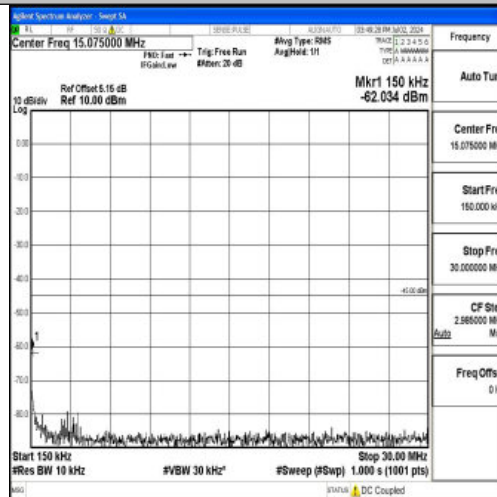
Band7_20MHz_QPSK_20850_1RB#0_0.15~30_0.15~30
