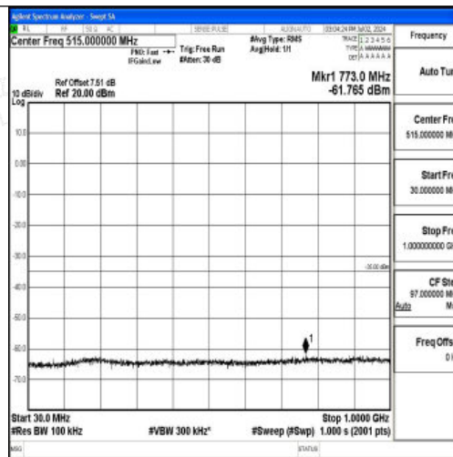
Band7_10MHz_QPSK_20800_1RB#0_30~1000_30~1000
