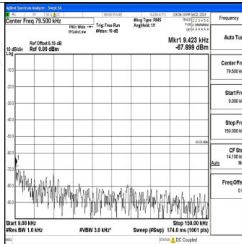
Band7_10MHz_QPSK_21400_1RB#0_0.009~0.15_0.009~0.15
