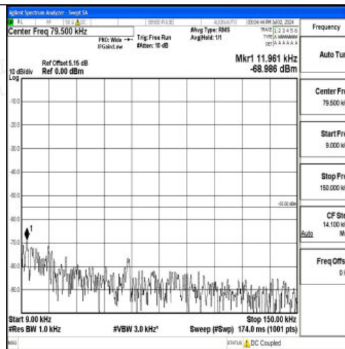
Band7_10MHz_16QAM_20800_1RB#0_0.009~0.15_0.009~0.15
