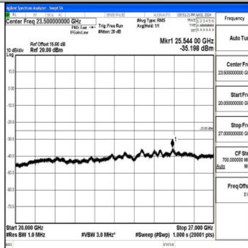
Band7_20MHz_16QAM_21100_1RB#0_20000~27000_20000~27000
