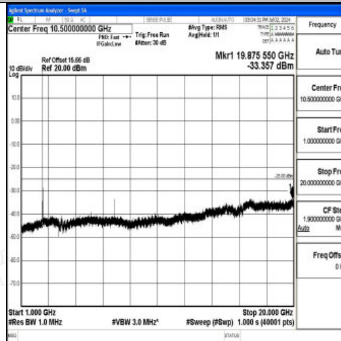
Band7_10MHz_QPSK_20800_1RB#0_1000~20000_1000~20000
