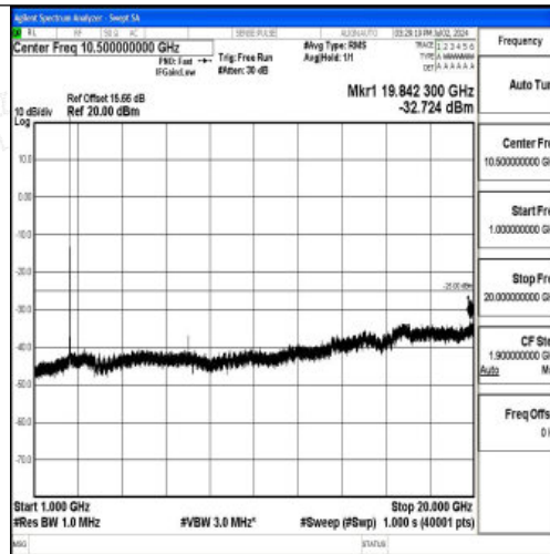
Band7_15MHz_QPSK_21375_1RB#0_1000~20000_1000~20000
