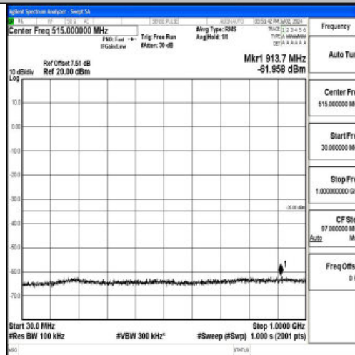
Band7_20MHz_QPSK_21350_1RB#0_30~1000_30~1000
