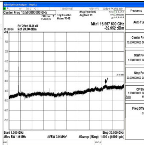
Band7_20MHz_QPSK_21350_1RB#0_1000~20000_1000~20000
