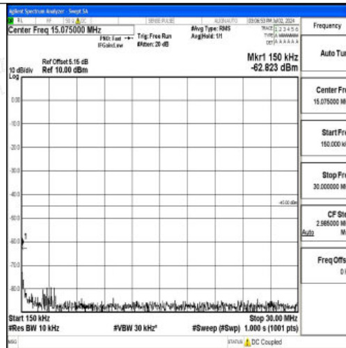
Band7_10MHz_16QAM_21400_1RB#0_0.15~30_0.15~30
