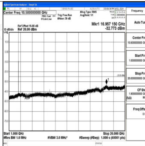
Band7_10MHz_QPSK_21400_1RB#0_1000~20000_1000~20000
