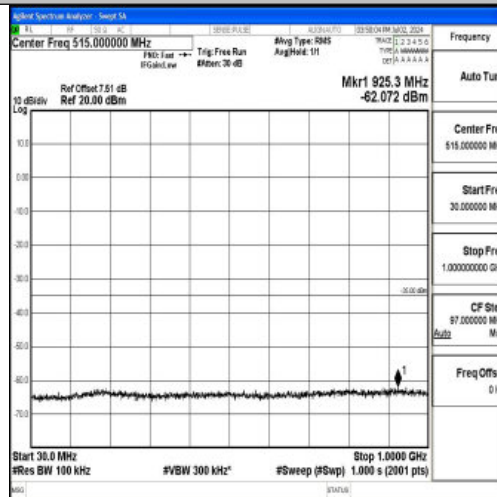
Band7_20MHz_16QAM_20850_1RB#0_30~1000_30~1000
