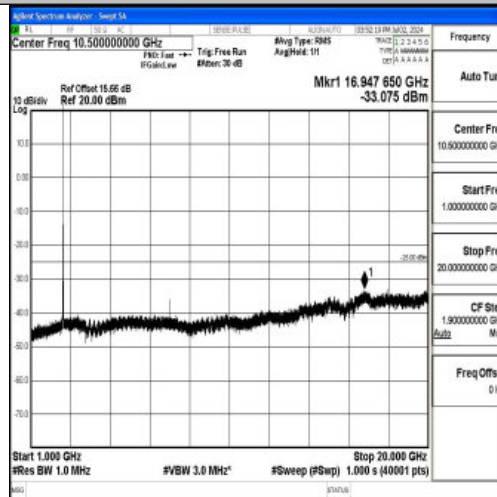
Band7_20MHz_16QAM_21350_1RB#0_1000~20000_1000~20000
