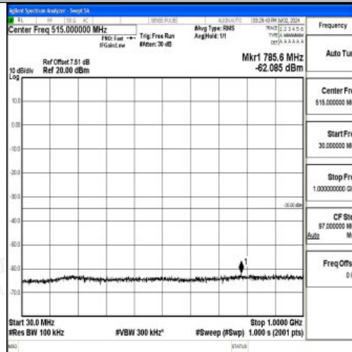
Band7_15MHz_16QAM_21375_1RB#0_30~1000_30~1000
