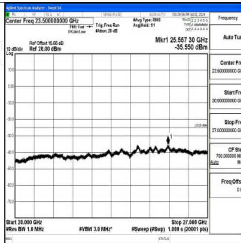
Band7_15MHz_16QAM_21375_1RB#0_20000~27000_20000~27000
