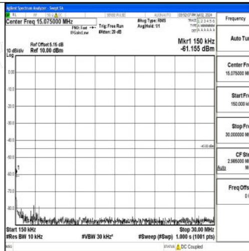
Band7_20MHz_16QAM_21350_1RB#0_0.15~30_0.15~30
