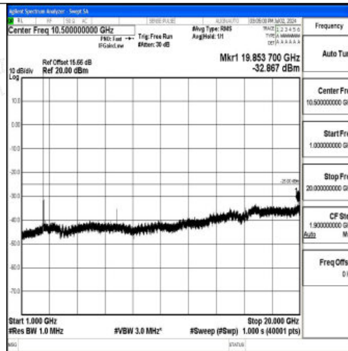
Band7_10MHz_16QAM_20800_1RB#0_1000~20000_1000~20000
