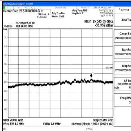
Band7_20MHz_QPSK_21350_1RB#0_20000~27000_20000~27000
