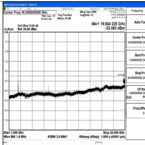
Band7_15MHz_16QAM_20825_1RB#0_1000~20000_1000~20000
