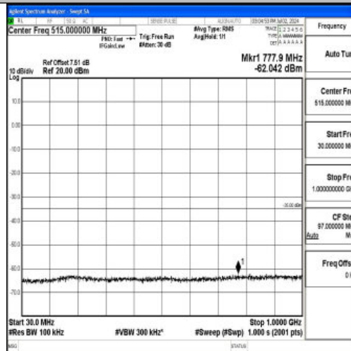
Band7_10MHz_16QAM_20800_1RB#0_30~1000_30~1000
