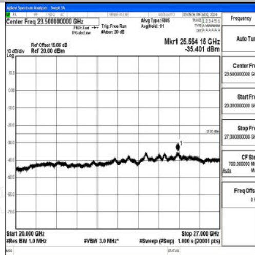
Band7_10MHz_16QAM_20800_1RB#0_20000~27000_20000~27000
