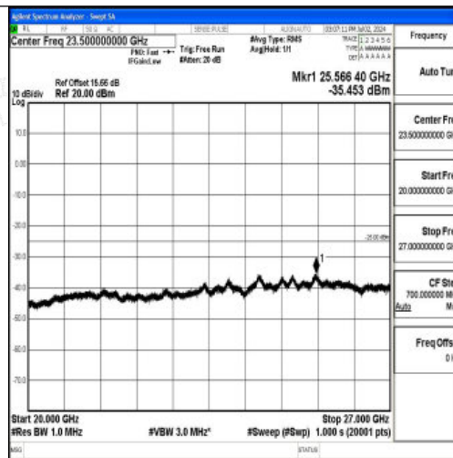
Band7_10MHz_16QAM_21400_1RB#0_20000~27000_20000~27000
