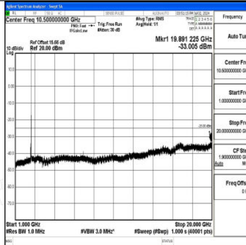
Band7_20MHz_16QAM_21100_1RB#0_1000~20000_1000~20000
