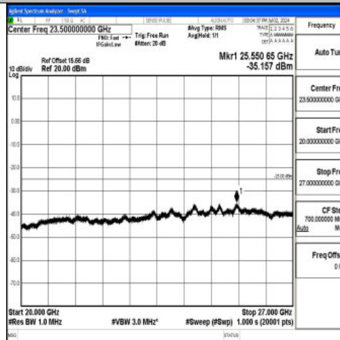
Band7_10MHz_QPSK_20800_1RB#0_20000~27000_20000~27000
