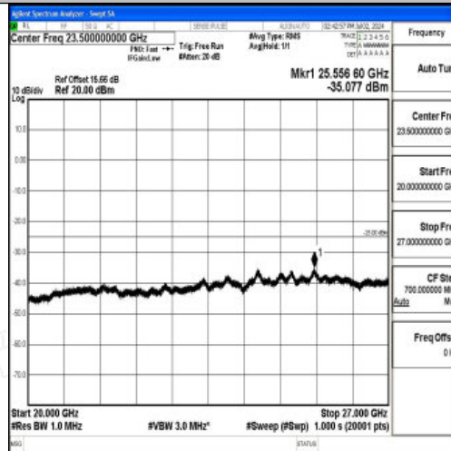
Band7_5MHz_QPSK_21425_1RB#0_20000~27000_20000~27000
