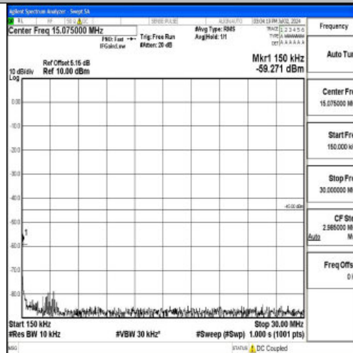
Band7_10MHz_QPSK_20800_1RB#0_0.15~30_0.15~30
