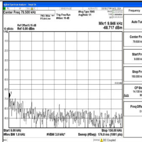
Band7_20MHz_QPSK_21100_1RB#0_0.009~0.15_0.009~0.15
