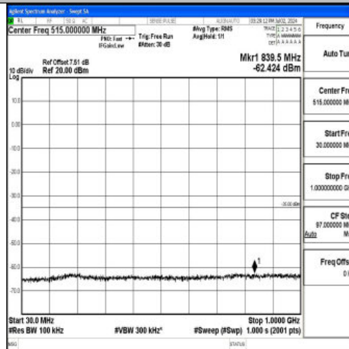
Band7_15MHz_QPSK_21375_1RB#0_30~1000_30~1000
