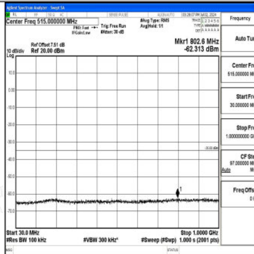
Band7_15MHz_QPSK_21100_1RB#0_30~1000_30~1000
