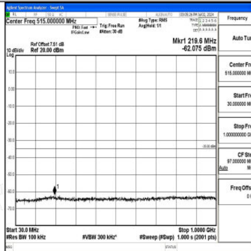
Band7_10MHz_QPSK_21100_1RB#0_30~1000_30~1000
