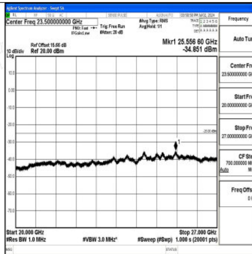
Band7_20MHz_QPSK_21100_1RB#0_20000~27000_20000~27000
