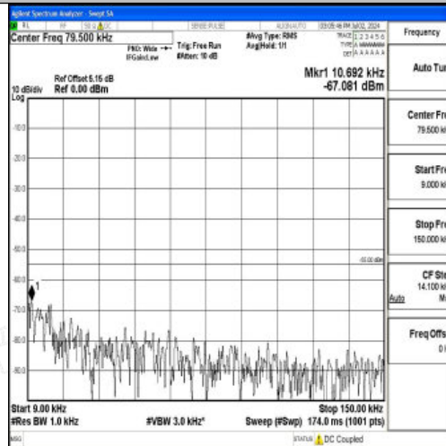
Band7_10MHz_16QAM_21100_1RB#0_0.009~0.15_0.009~0.15
