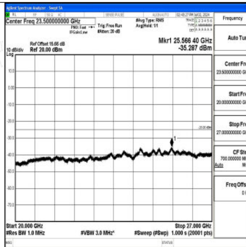
Band7_5MHz_16QAM_21425_1RB#0_20000~27000_20000~27000
