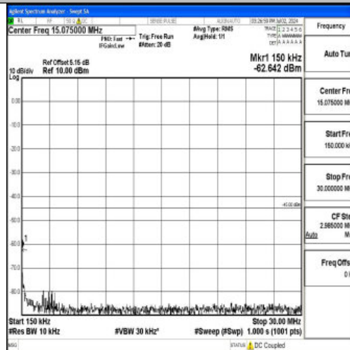
Band7_15MHz_QPSK_20825_1RB#0_0.15~30_0.15~30
