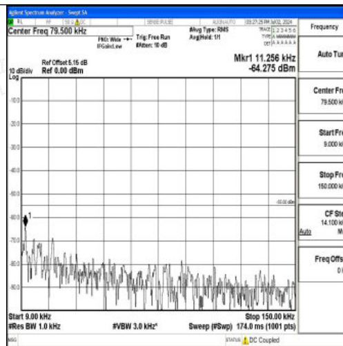
Band7_15MHz_16QAM_20825_1RB#0_0.009~0.15_0.009~0.15
