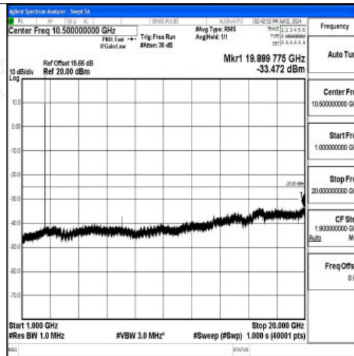
Band7_5MHz_QPSK_21425_1RB#0_1000~20000_1000~20000
