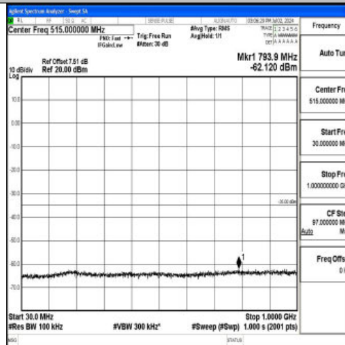
Band7_10MHz_QPSK_21400_1RB#0_30~1000_30~1000
