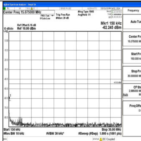
Band7_20MHz_16QAM_21100_1RB#0_0.15~30_0.15~30
