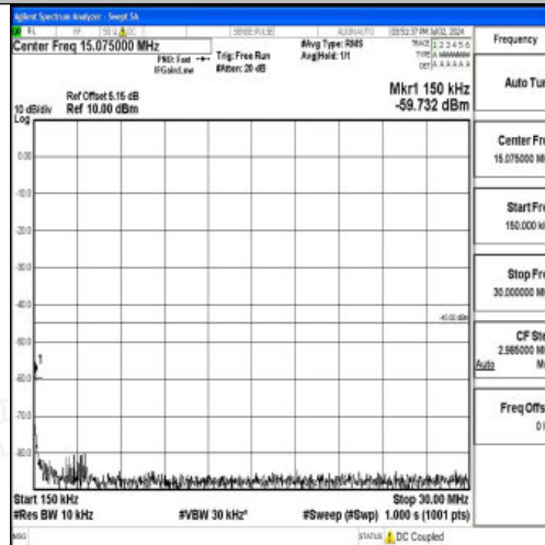
Band7_20MHz_QPSK_21350_1RB#0_0.15~30_0.15~30
