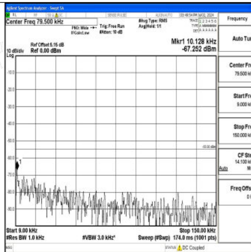
Band7_20MHz_16QAM_20850_1RB#0_0.009~0.15_0.009~0.15
