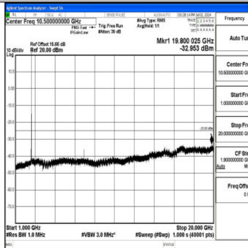
Band7_15MHz_QPSK_21100_1RB#0_1000~20000_1000~20000
