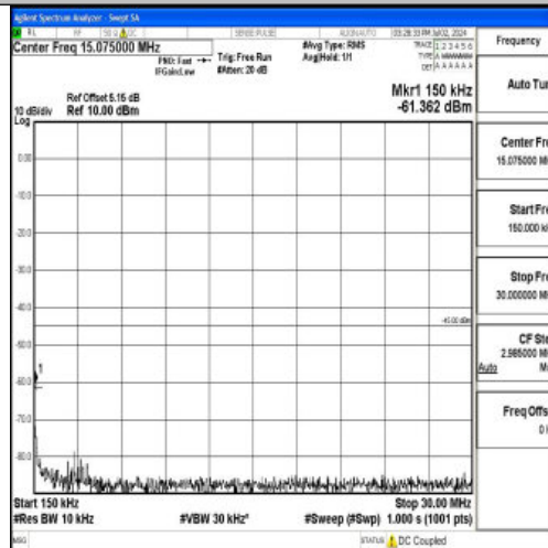
Band7_15MHz_16QAM_21100_1RB#0_0.15~30_0.15~30
