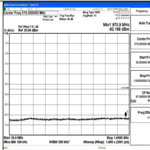
Band7_15MHz_16QAM_20825_1RB#0_30~1000_30~1000
