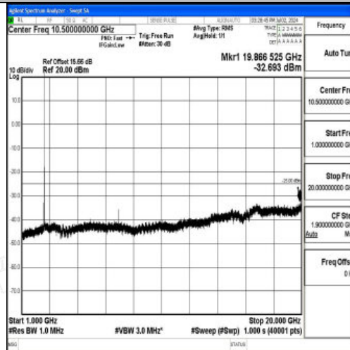
Band7_15MHz_16QAM_21100_1RB#0_1000~20000_1000~20000
