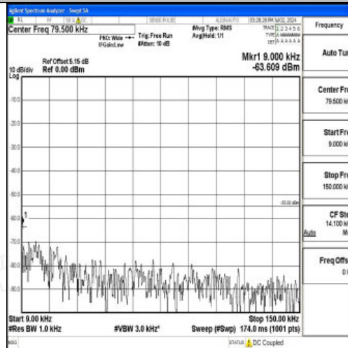
Band7_15MHz_16QAM_21100_1RB#0_0.009~0.15_0.009~0.15
