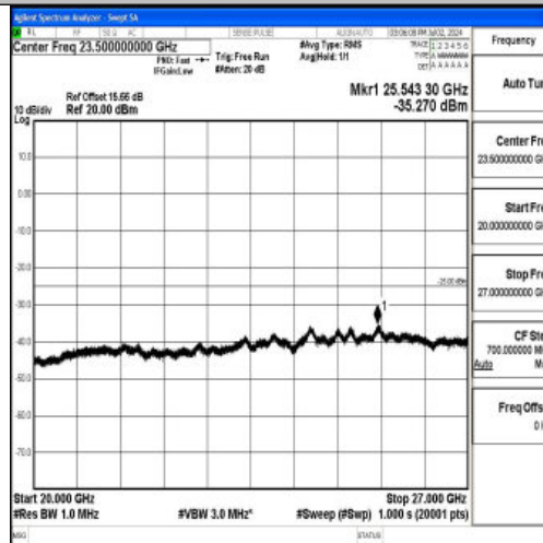
Band7_10MHz_16QAM_21100_1RB#0_20000~27000_20000~27000
