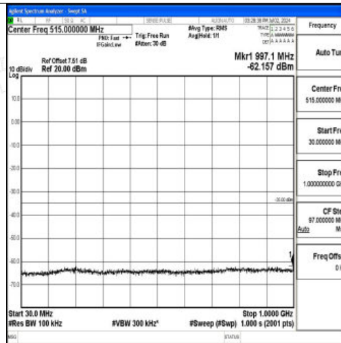
Band7_15MHz_16QAM_21100_1RB#0_30~1000_30~1000
