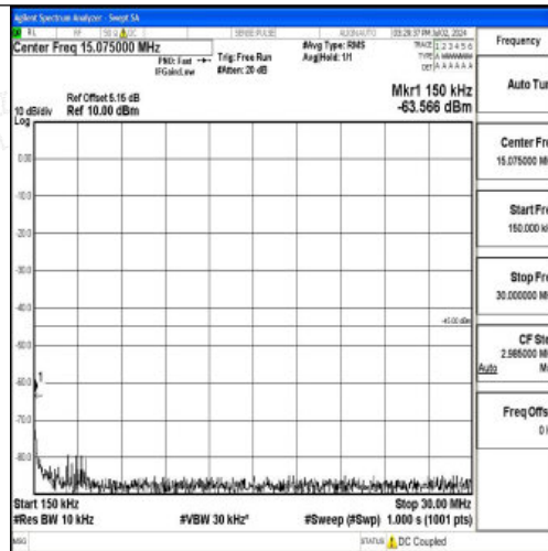
Band7_15MHz_16QAM_21375_1RB#0_0.15~30_0.15~30
