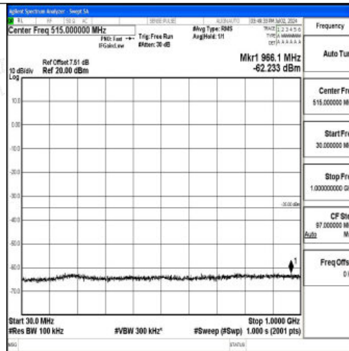
Band7_20MHz_QPSK_20850_1RB#0_30~1000_30~1000
