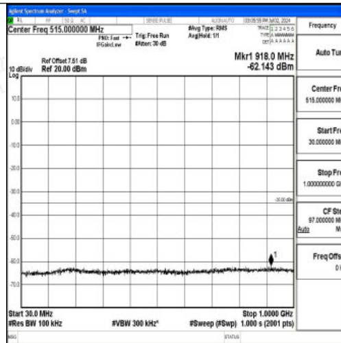
Band7_10MHz_16QAM_21100_1RB#0_30~1000_30~1000
