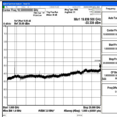
Band7_10MHz_QPSK_21100_1RB#0_1000~20000_1000~20000
