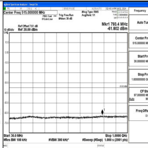
Band7_5MHz_16QAM_21425_1RB#0_30~1000_30~1000
