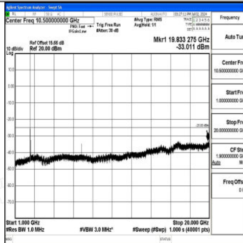
Band7_15MHz_QPSK_20825_1RB#0_1000~20000_1000~20000
