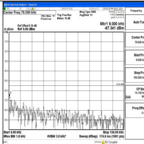
Band7_20MHz_16QAM_21350_1RB#0_0.009~0.15_0.009~0.15
