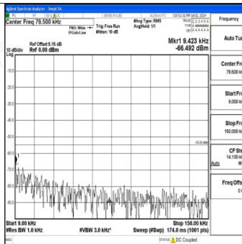
Band7_20MHz_QPSK_21350_1RB#0_0.009~0.15_0.009~0.15
