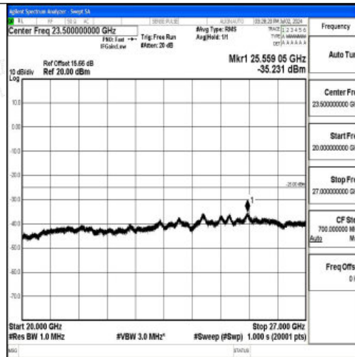
Band7_15MHz_QPSK_21100_1RB#0_20000~27000_20000~27000
