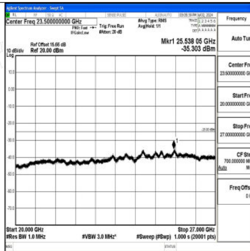
Band7_10MHz_QPSK_21100_1RB#0_20000~27000_20000~27000
