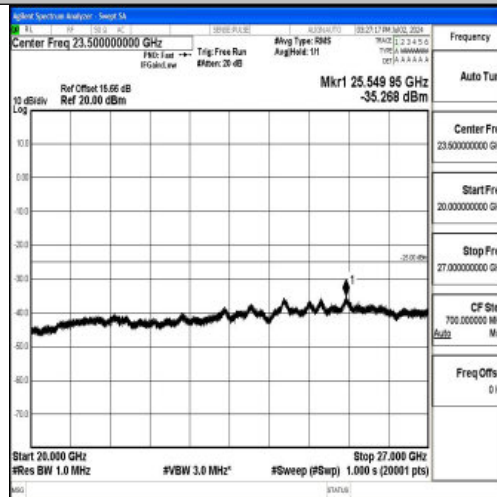
Band7_15MHz_QPSK_20825_1RB#0_20000~27000_20000~27000
