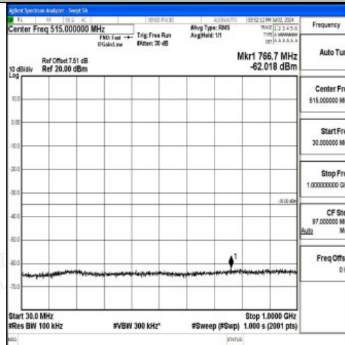
Band7_20MHz_16QAM_21350_1RB#0_30~1000_30~1000
