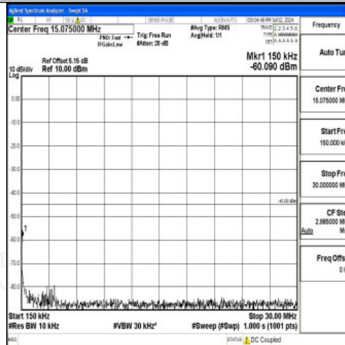
Band7_10MHz_16QAM_20800_1RB#0_0.15~30_0.15~30
