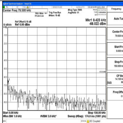
Band7_15MHz_QPSK_20825_1RB#0_0.009~0.15_0.009~0.15
