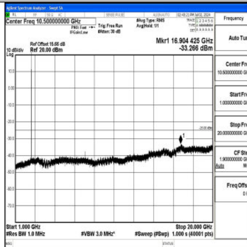
Band7_5MHz_16QAM_21425_1RB#0_1000~20000_1000~20000
