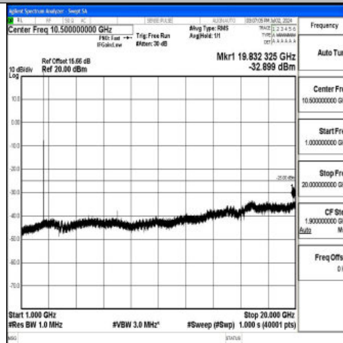
Band7_10MHz_16QAM_21400_1RB#0_1000~20000_1000~20000
