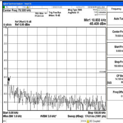
Band7_20MHz_16QAM_21100_1RB#0_0.009~0.15_0.009~0.15
