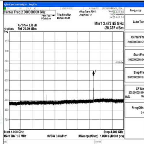
Band5_5MHz_QPSK_20425_1RB#0_1000~3000_1000~3000
