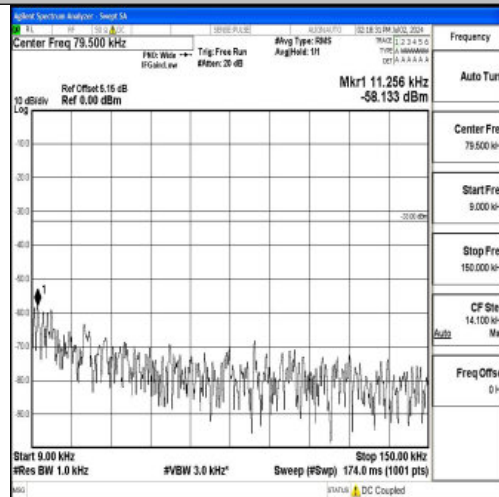
Band5_10MHz_QPSK_20525_1RB#0_0.009~0.15_0.009~0.15
