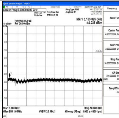
Band5_1.4MHz_QPSK_20643_1RB#0_3000~10000_3000~10000
