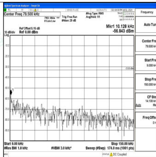
Band5_10MHz_16QAM_20450_1RB#0_0.009~0.15_0.009~0.15
