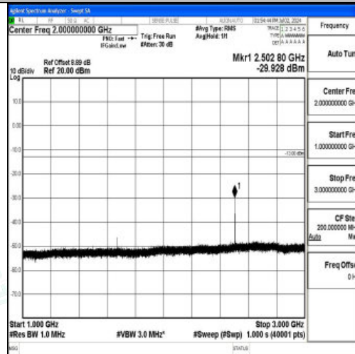
Band5_5MHz_16QAM_20525_1RB#0_1000~3000_1000~3000
