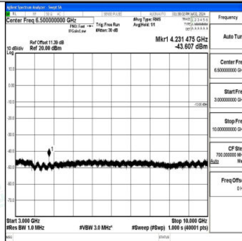
Band5_3MHz_QPSK_20635_1RB#0_3000~10000_3000~10000
