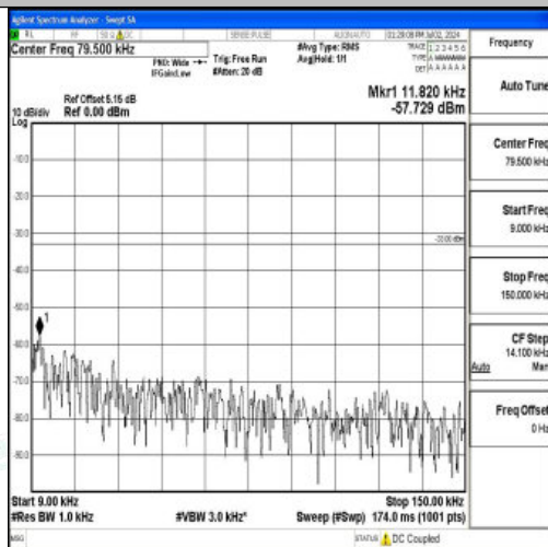
Band5_3MHz_16QAM_20525_1RB#0_0.009~0.15_0.009~0.15
