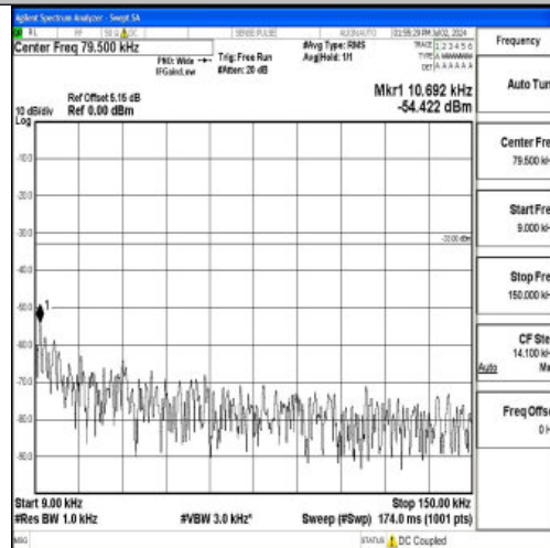
Band5_5MHz_16QAM_20625_1RB#0_0.009~0.15_0.009~0.15
