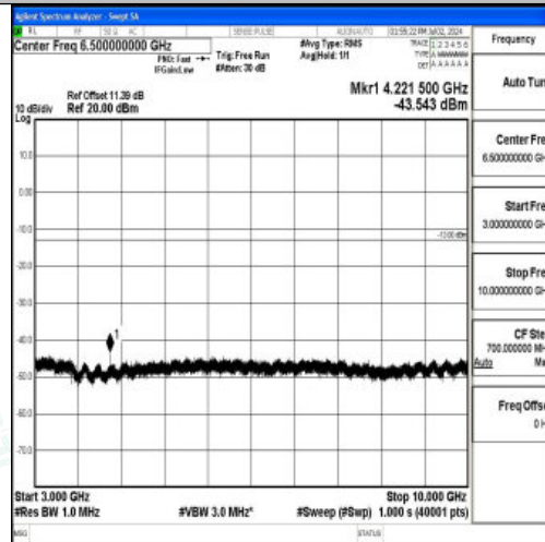
Band5_5MHz_QPSK_20625_1RB#0_3000~10000_3000~10000
