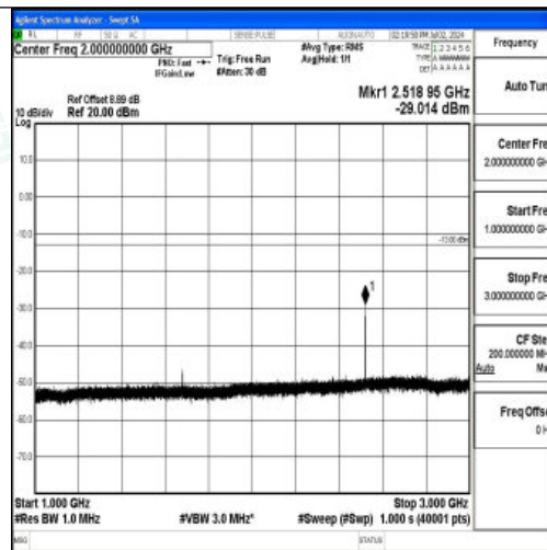
Band5_10MHz_QPSK_20600_1RB#0_1000~3000_1000~3000
