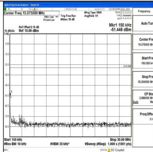
Band5_5MHz_QPSK_20425_1RB#0_0.15~30_0.15~30
