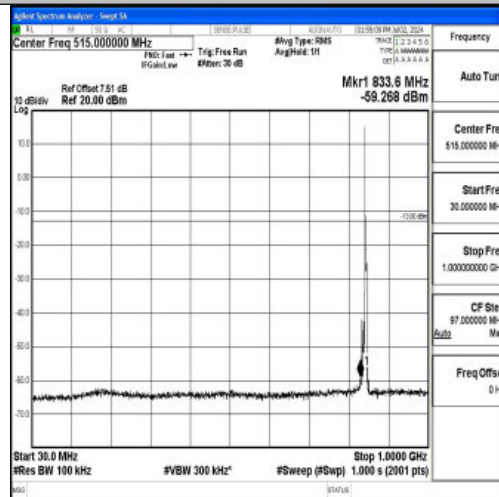
Band5_5MHz_QPSK_20625_1RB#0_30~1000_30~1000
