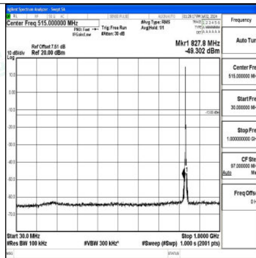
Band5_3MHz_16QAM_20525_1RB#0_30~1000_30~1000
