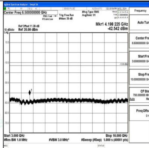
Band5_10MHz_QPSK_20600_1RB#0_3000~10000_3000~10000
