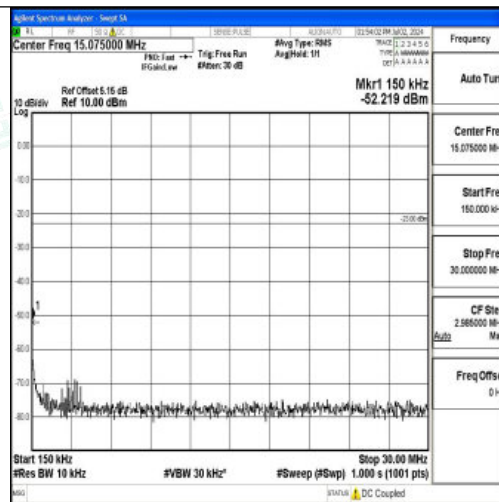
Band5_5MHz_QPSK_20525_1RB#0_0.15~30_0.15~30
