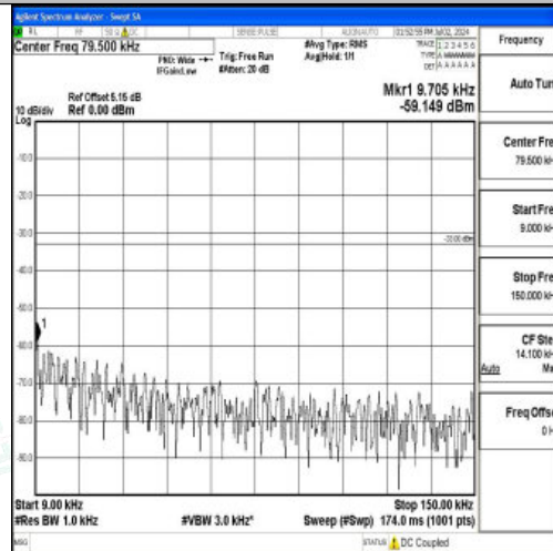
Band5_5MHz_QPSK_20425_1RB#0_0.009~0.15_0.009~0.15
