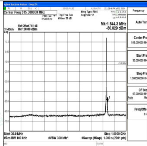
Band5_3MHz_QPSK_20525_1RB#0_30~1000_30~1000
