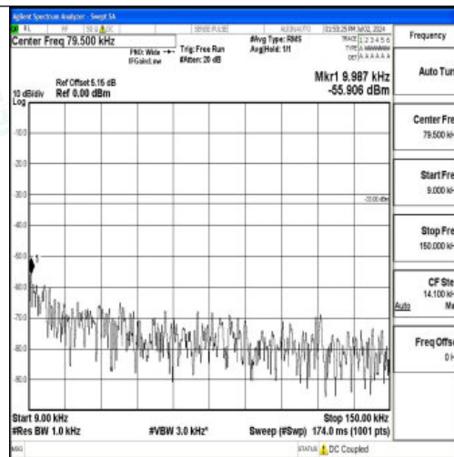
Band5_5MHz_16QAM_20425_1RB#0_0.009~0.15_0.009~0.15
