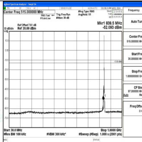
Band5_3MHz_16QAM_20635_1RB#0_30~1000_30~1000
