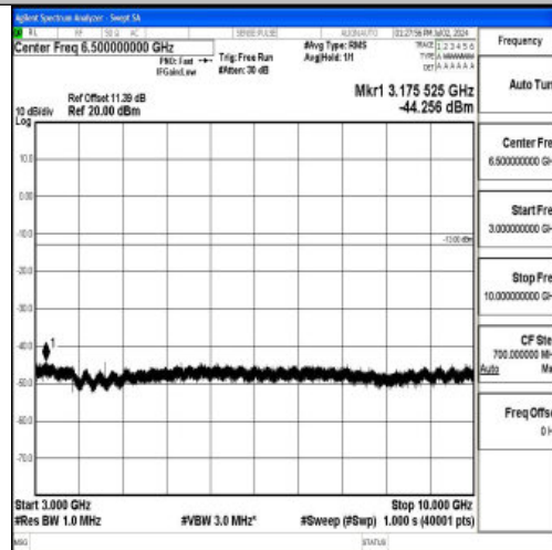
Band5_3MHz_QPSK_20415_1RB#0_3000~10000_3000~10000
