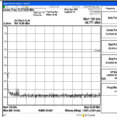
Band5_5MHz_QPSK_20625_1RB#0_0.15~30_0.15~30
