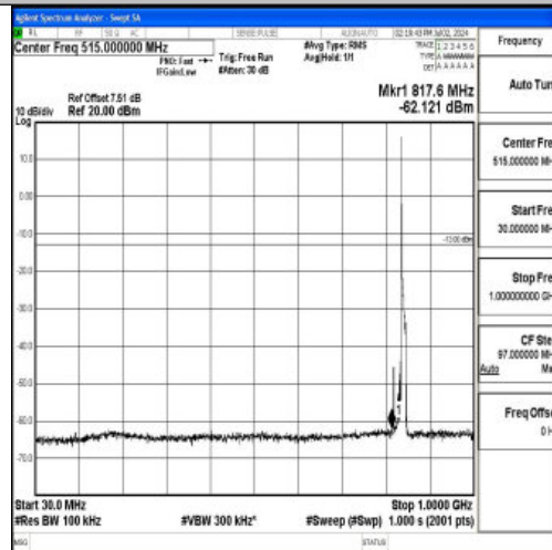
Band5_10MHz_QPSK_20600_1RB#0_30~1000_30~1000
