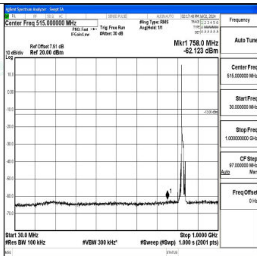
Band5_10MHz_QPSK_20450_1RB#0_30~1000_30~1000
