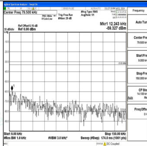
Band5_3MHz_QPSK_20415_1RB#0_0.009~0.15_0.009~0.15
