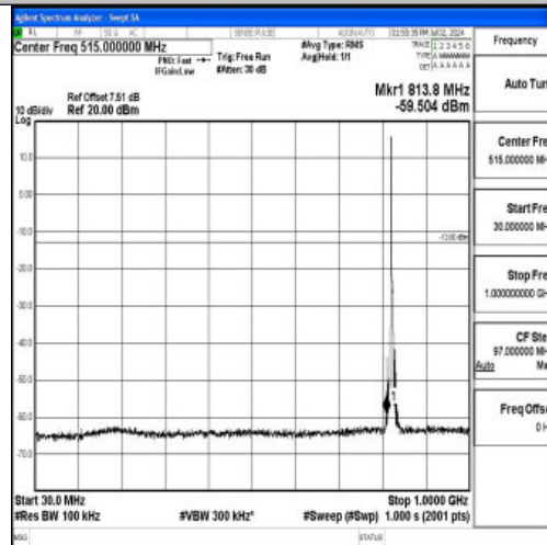
Band5_5MHz_16QAM_20425_1RB#0_30~1000_30~1000
