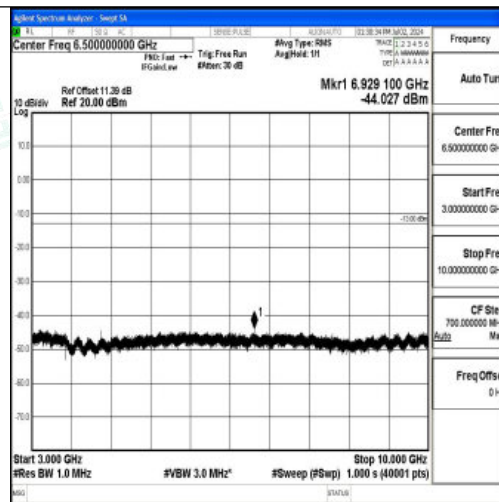
Band5_3MHz_16QAM_20635_1RB#0_3000~10000_3000~10000
