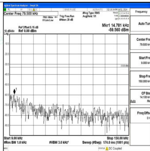
Band5_10MHz_QPSK_20600_1RB#0_0.009~0.15_0.009~0.15
