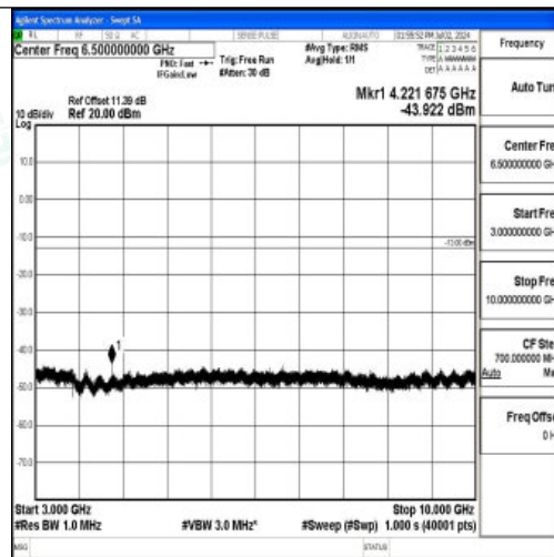
Band5_5MHz_16QAM_20625_1RB#0_3000~10000_3000~10000
