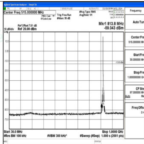
Band5_5MHz_QPSK_20425_1RB#0_30~1000_30~1000
