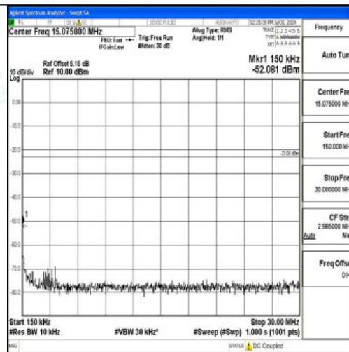
Band5_10MHz_16QAM_20600_1RB#0_0.15~30_0.15~30
