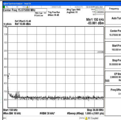
Band5_10MHz_QPSK_20600_1RB#0_0.15~30_0.15~30
