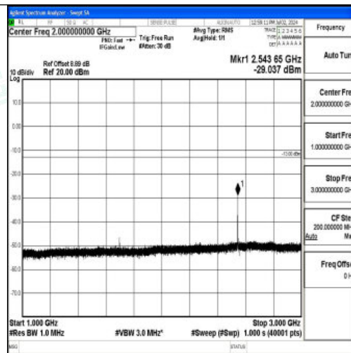
Band5_1.4MHz_QPSK_20643_1RB#0_1000~3000_1000~3000
