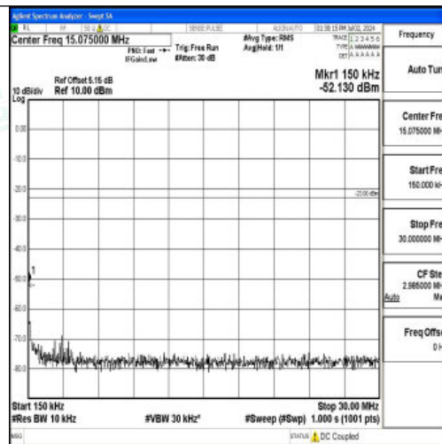
Band5_3MHz_16QAM_20635_1RB#0_0.15~30_0.15~30
