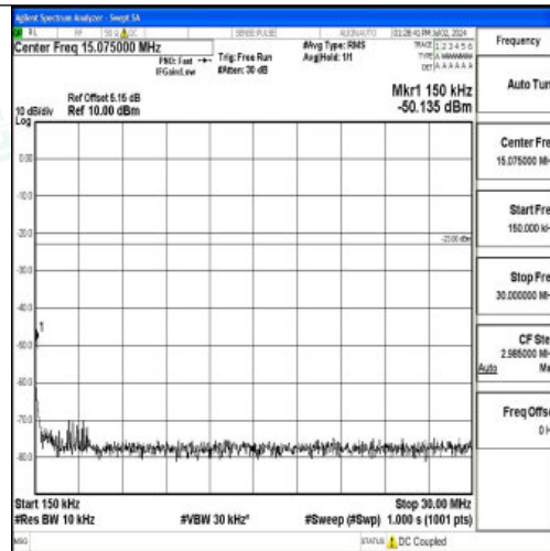
Band5_3MHz_QPSK_20525_1RB#0_0.15~30_0.15~30
