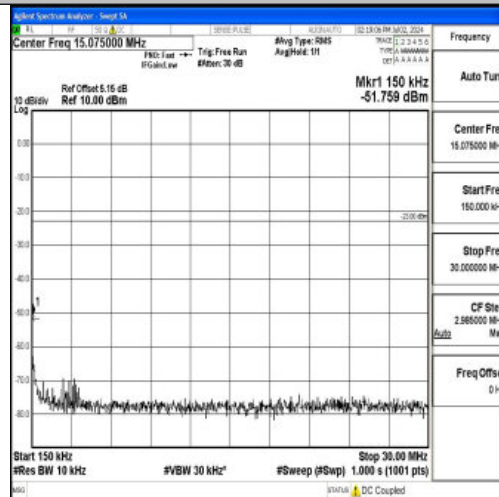
Band5_10MHz_16QAM_20525_1RB#0_0.15~30_0.15~30
