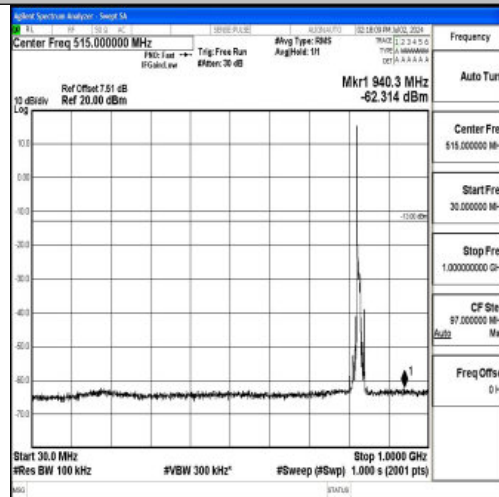
Band5_10MHz_16QAM_20450_1RB#0_30~1000_30~1000
