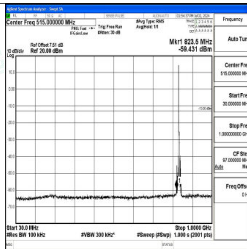
Band5_5MHz_16QAM_20525_1RB#0_30~1000_30~1000
