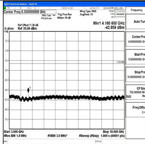
Band5_10MHz_16QAM_20525_1RB#0_3000~10000_3000~10000
