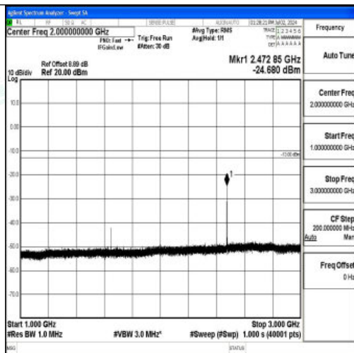
Band5_3MHz_16QAM_20415_1RB#0_1000~3000_1000~3000
