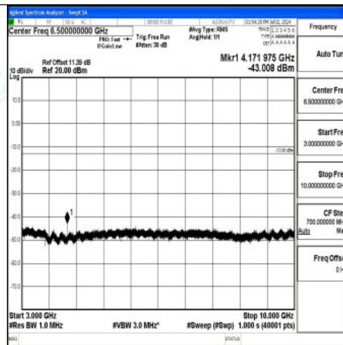
Band5_5MHz_QPSK_20525_1RB#0_3000~10000_3000~10000
