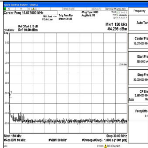
Band5_5MHz_16QAM_20525_1RB#0_0.15~30_0.15~30
