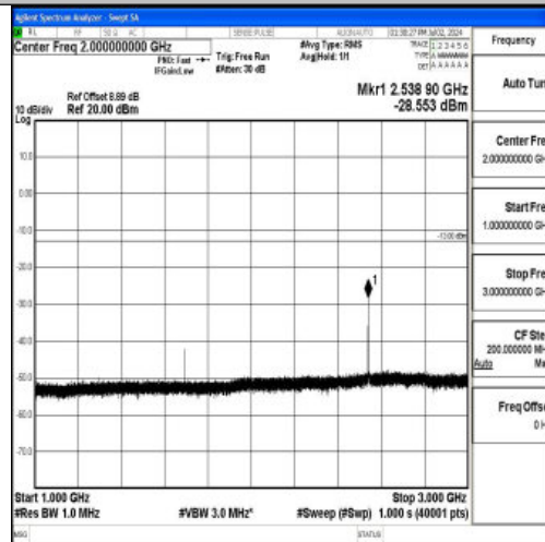
Band5_3MHz_16QAM_20635_1RB#0_1000~3000_1000~3000
