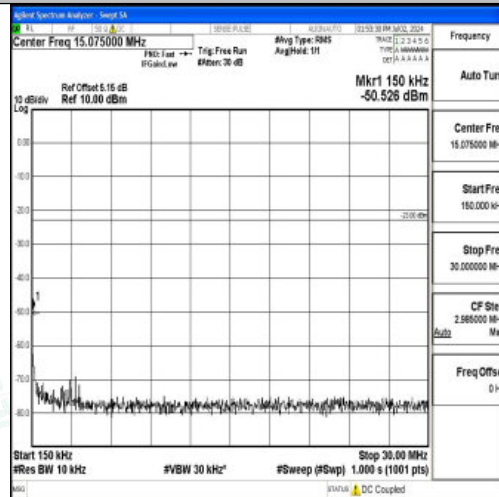
Band5_5MHz_16QAM_20425_1RB#0_0.15~30_0.15~30
