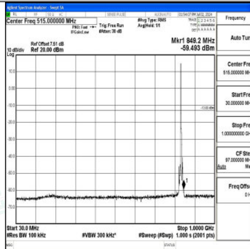
Band5_5MHz_QPSK_20525_1RB#0_30~1000_30~1000
