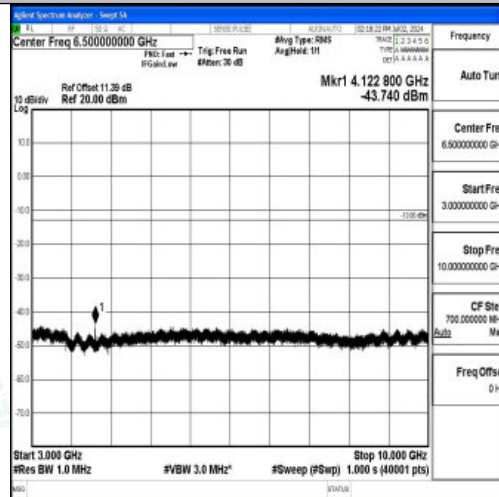
Band5_10MHz_16QAM_20450_1RB#0_3000~10000_3000~10000
