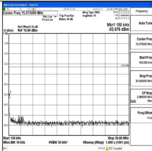
Band5_3MHz_16QAM_20525_1RB#0_0.15~30_0.15~30
