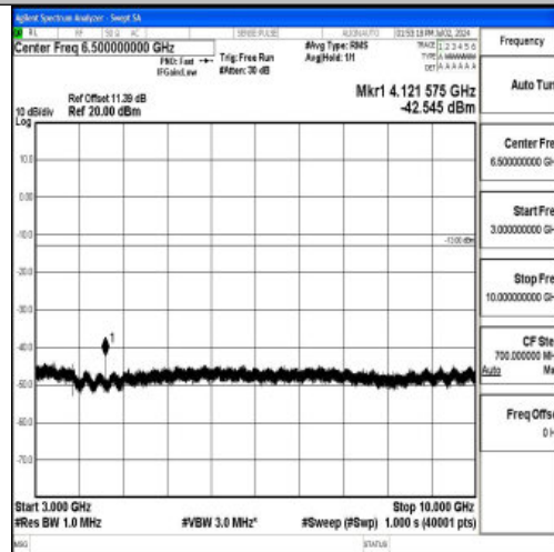
Band5_5MHz_QPSK_20425_1RB#0_3000~10000_3000~10000
