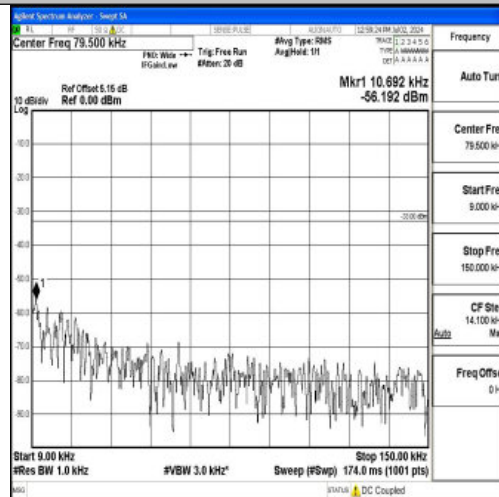
Band5_1.4MHz_16QAM_20643_1RB#0_0.009~0.15_0.009~0.15
