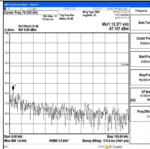
Band5_5MHz_16QAM_20525_1RB#0_0.009~0.15_0.009~0.15
