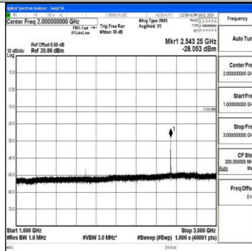
Band5_1.4MHz_16QAM_20643_1RB#0_1000~3000_1000~3000
