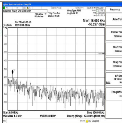
Band5_3MHz_QPSK_20635_1RB#0_0.009~0.15_0.009~0.15
