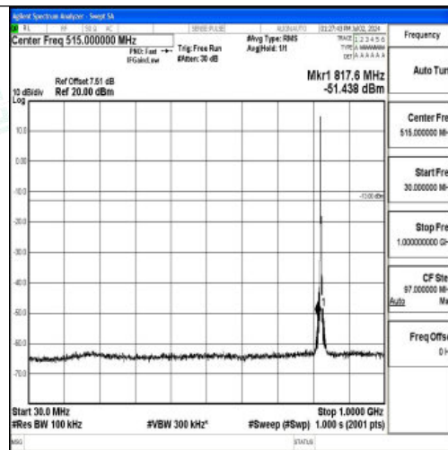
Band5_3MHz_QPSK_20415_1RB#0_30~1000_30~1000
