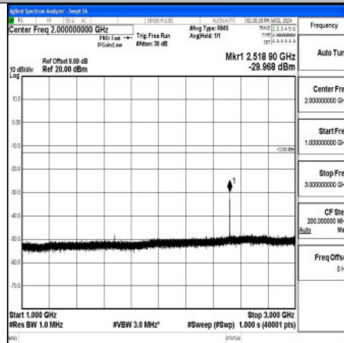
Band5_10MHz_16QAM_20600_1RB#0_1000~3000_1000~3000
