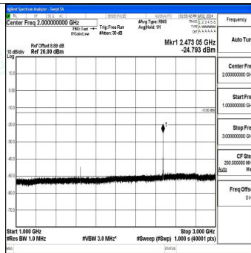
Band5_5MHz_16QAM_20425_1RB#0_1000~3000_1000~3000
