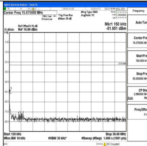
Band5_10MHz_QPSK_20450_1RB#0_0.15~30_0.15~30
