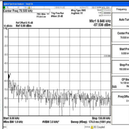
Band5_10MHz_QPSK_20450_1RB#0_0.009~0.15_0.009~0.15
