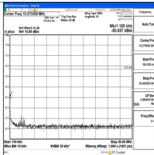
Band5_1.4MHz_16QAM_20643_1RB#0_0.15~30_0.15~30
