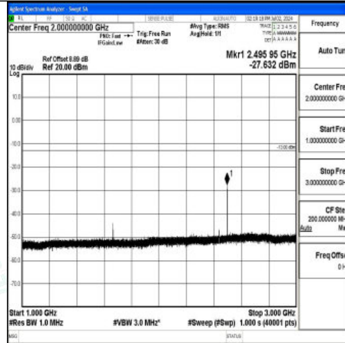
Band5_10MHz_16QAM_20525_1RB#0_1000~3000_1000~3000
