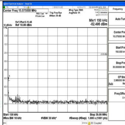
Band5_10MHz_16QAM_20450_1RB#0_0.15~30_0.15~30
