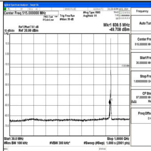
Band5_3MHz_QPSK_20635_1RB#0_30~1000_30~1000
