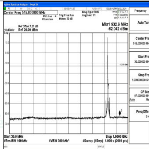
Band5_10MHz_QPSK_20525_1RB#0_30~1000_30~1000
