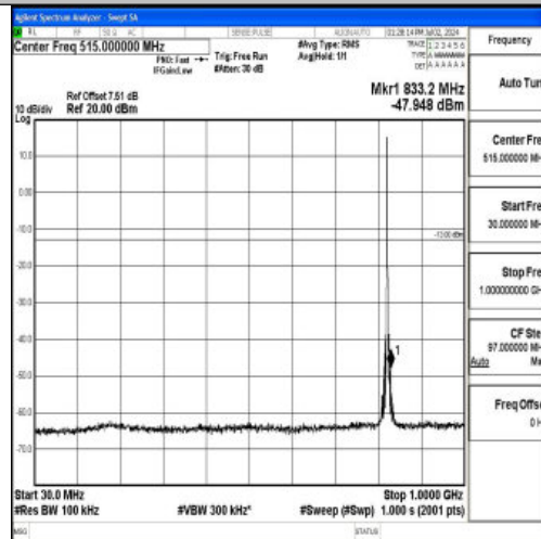
Band5_3MHz_16QAM_20415_1RB#0_30~1000_30~1000
