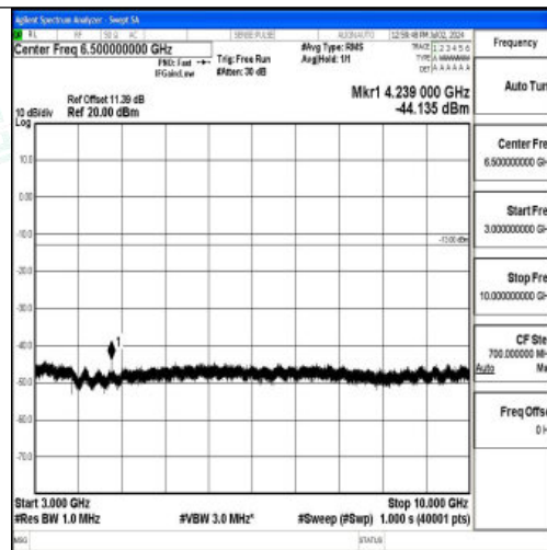
Band5_1.4MHz_16QAM_20643_1RB#0_3000~10000_3000~10000
