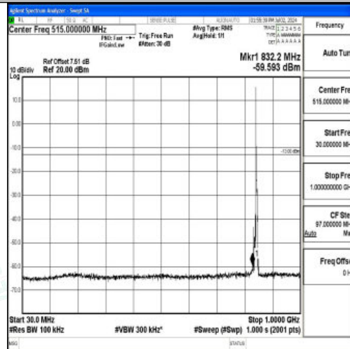
Band5_5MHz_16QAM_20625_1RB#0_30~1000_30~1000
