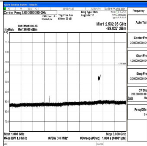
Band5_5MHz_16QAM_20625_1RB#0_1000~3000_1000~3000
