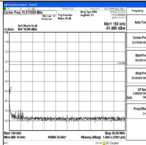
Band5_3MHz_QPSK_20415_1RB#0_0.15~30_0.15~30
