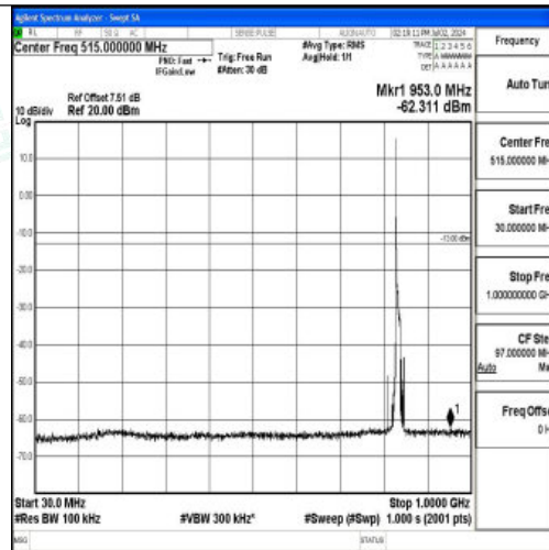
Band5_10MHz_16QAM_20525_1RB#0_30~1000_30~1000
