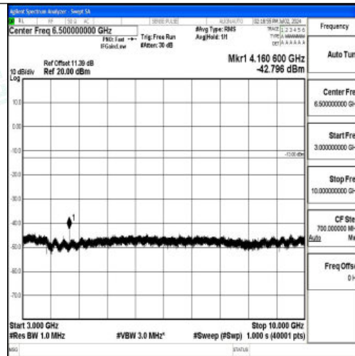
Band5_10MHz_QPSK_20525_1RB#0_3000~10000_3000~10000
