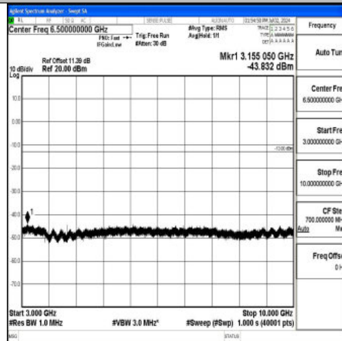
Band5_5MHz_16QAM_20525_1RB#0_3000~10000_3000~10000
