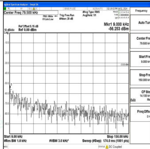
Band5_10MHz_16QAM_20525_1RB#0_0.009~0.15_0.009~0.15
