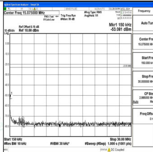
Band5_3MHz_16QAM_20415_1RB#0_0.15~30_0.15~30
