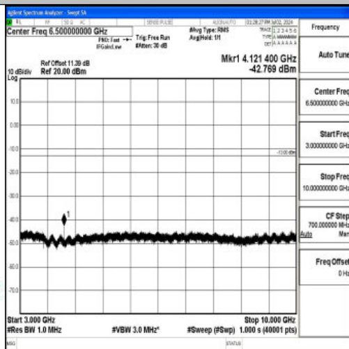
Band5_3MHz_16QAM_20415_1RB#0_3000~10000_3000~10000
