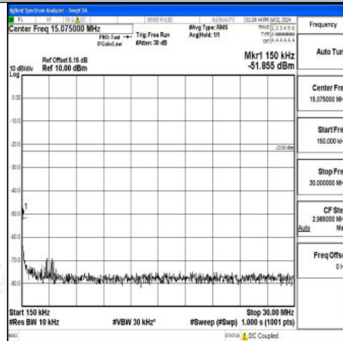
Band5_3MHz_QPSK_20635_1RB#0_0.15~30_0.15~30
