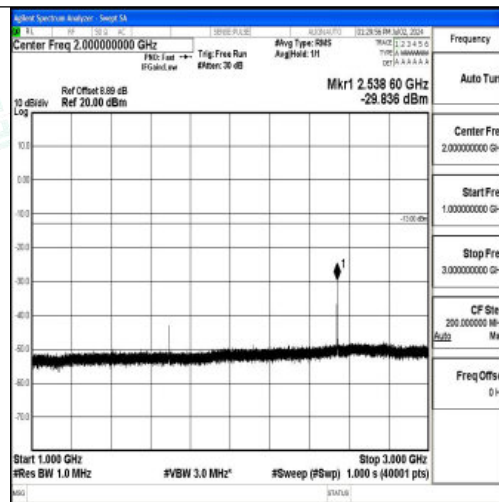
Band5_3MHz_QPSK_20635_1RB#0_1000~3000_1000~3000
