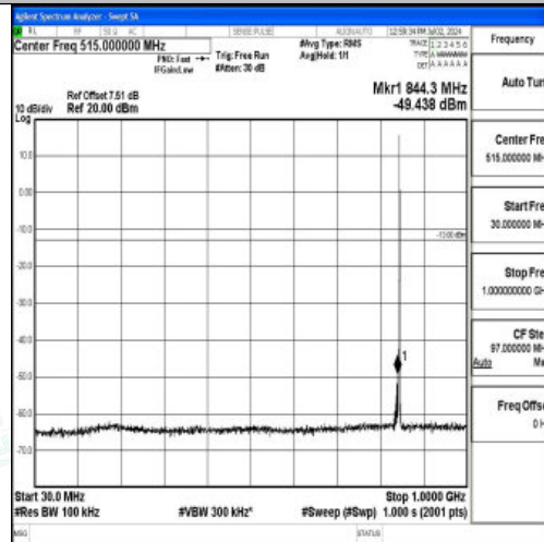
Band5_1.4MHz_16QAM_20643_1RB#0_30~1000_30~1000
