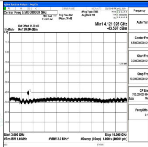
Band5_5MHz_16QAM_20425_1RB#0_3000~10000_3000~10000
