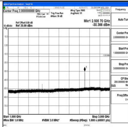
Band5_3MHz_QPSK_20525_1RB#0_1000~3000_1000~3000
