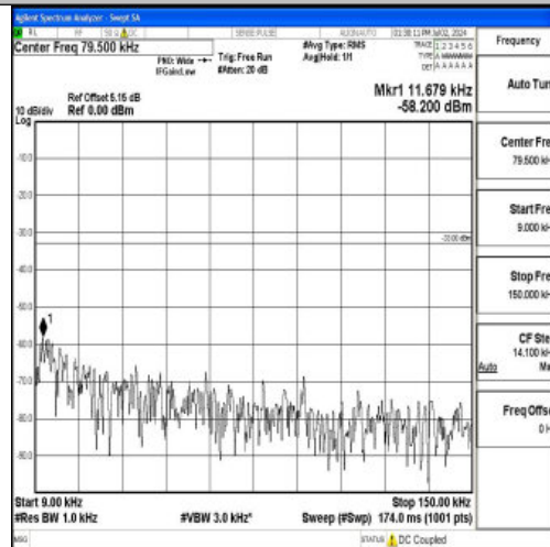
Band5_3MHz_16QAM_20635_1RB#0_0.009~0.15_0.009~0.15
