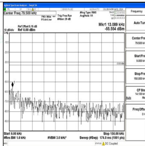
Band5_3MHz_16QAM_20415_1RB#0_0.009~0.15_0.009~0.15
