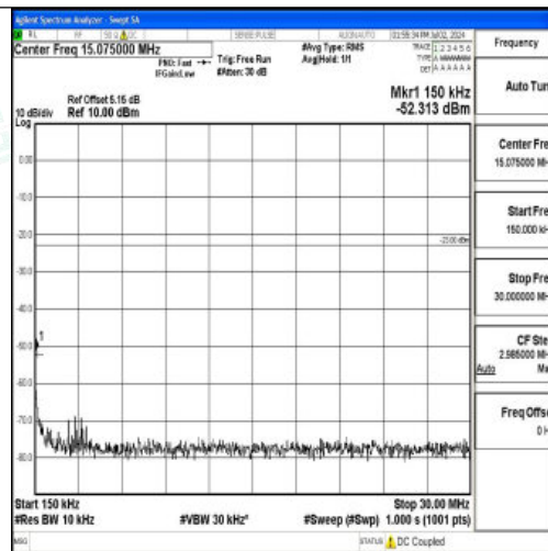
Band5_5MHz_16QAM_20625_1RB#0_0.15~30_0.15~30
