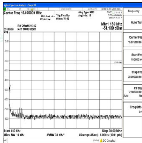
Band5_10MHz_QPSK_20525_1RB#0_0.15~30_0.15~30
