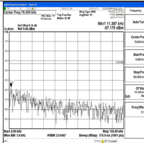
Band5_5MHz_QPSK_20525_1RB#0_0.009~0.15_0.009~0.15
