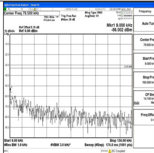
Band5_10MHz_16QAM_20600_1RB#0_0.009~0.15_0.009~0.15
