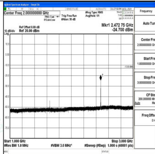
Band5_3MHz_QPSK_20415_1RB#0_1000~3000_1000~3000
