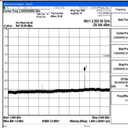
Band5_5MHz_QPSK_20525_1RB#0_1000~3000_1000~3000
