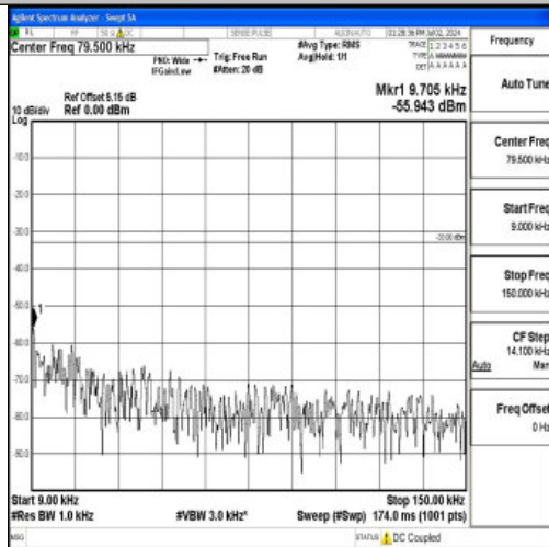
Band5_3MHz_QPSK_20525_1RB#0_0.009~0.15_0.009~0.15
