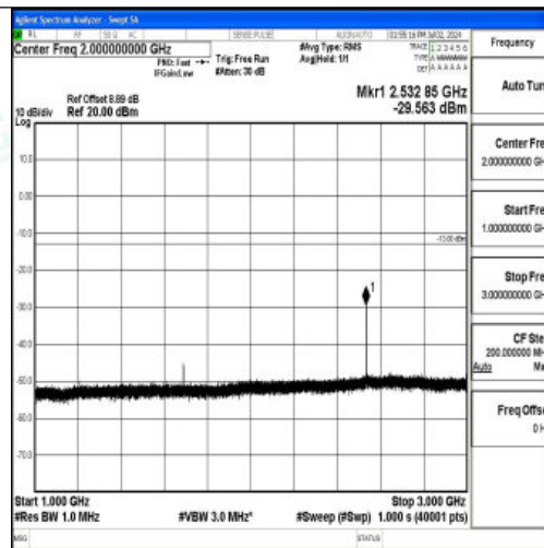
Band5_5MHz_QPSK_20625_1RB#0_1000~3000_1000~3000
