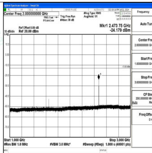
Band5_10MHz_16QAM_20450_1RB#0_1000~3000_1000~3000
