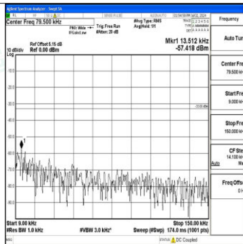
Band5_5MHz_QPSK_20625_1RB#0_0.009~0.15_0.009~0.15
