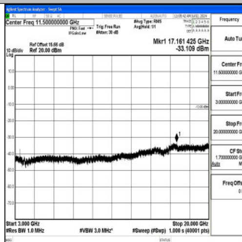
Band4_3MHz_QPSK_20175_1RB#0_3000~20000_3000~20000
