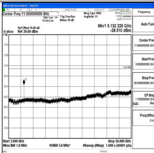
Band4_15MHz_QPSK_20025_1RB#0_3000~20000_3000~20000
