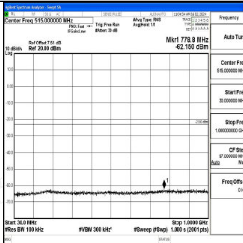
Band4_3MHz_16QAM_19965_1RB#0_30~1000_30~1000
