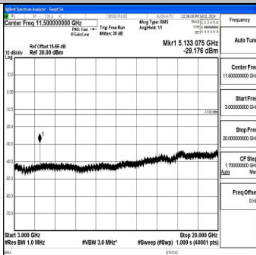
Band4_20MHz_QPSK_20050_1RB#0_3000~20000_3000~20000
