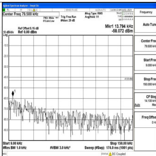
Band4_3MHz_QPSK_19965_1RB#0_0.009~0.15_0.009~0.15
