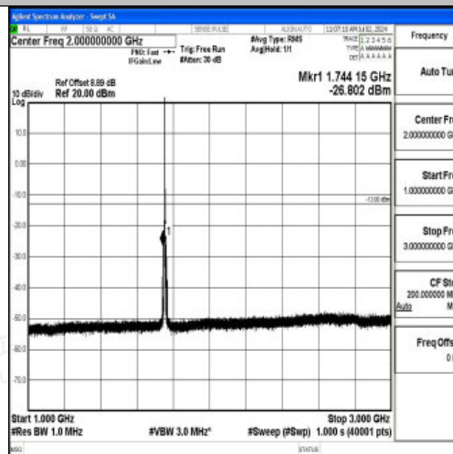
Band4_3MHz_16QAM_20385_1RB#0_1000~3000_1000~3000
