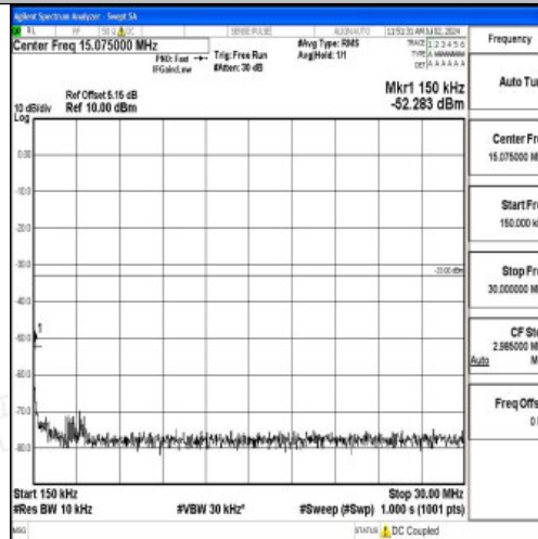
Band4_10MHz_QPSK_20000_1RB#0_0.15~30_0.15~30
