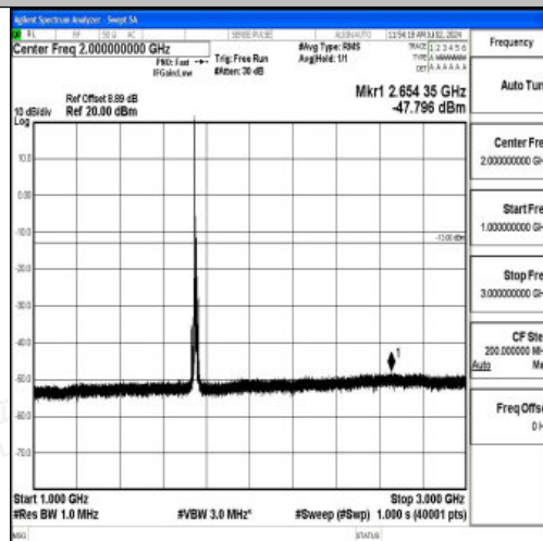
Band4_10MHz_16QAM_20350_1RB#0_1000~3000_1000~3000
