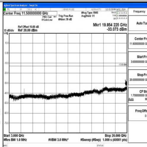
Band4_15MHz_16QAM_20175_1RB#0_3000~20000_3000~20000
