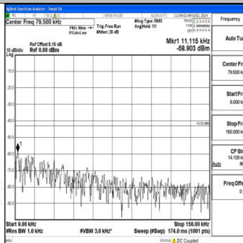
Band4_10MHz_16QAM_20350_1RB#0_0.009~0.15_0.009~0.15
