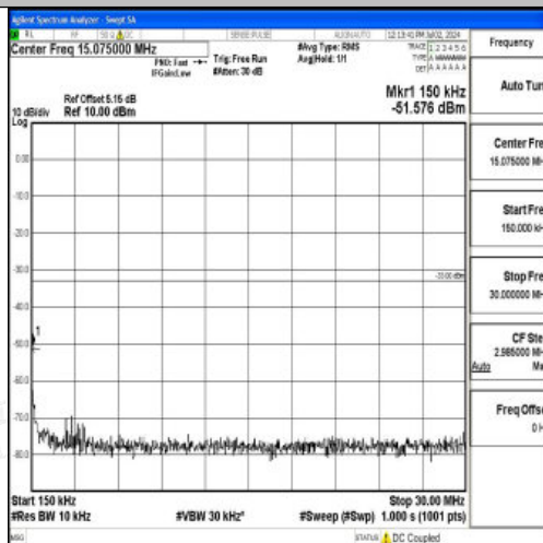
Band4_15MHz_QPSK_20025_1RB#0_0.15~30_0.15~30
