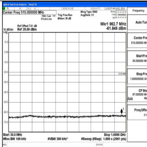
Band4_10MHz_16QAM_20000_1RB#0_30~1000_30~1000
