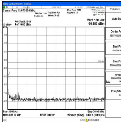
Band4_15MHz_QPSK_20325_1RB#0_0.15~30_0.15~30
