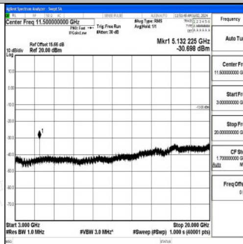
Band4_10MHz_QPSK_20000_1RB#0_3000~20000_3000~20000
