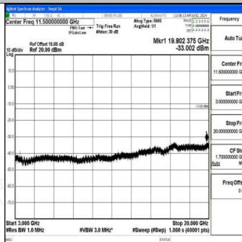
Band4_3MHz_16QAM_20175_1RB#0_3000~20000_3000~20000
