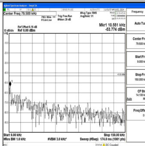
Band4_10MHz_16QAM_20000_1RB#0_0.009~0.15_0.009~0.15
