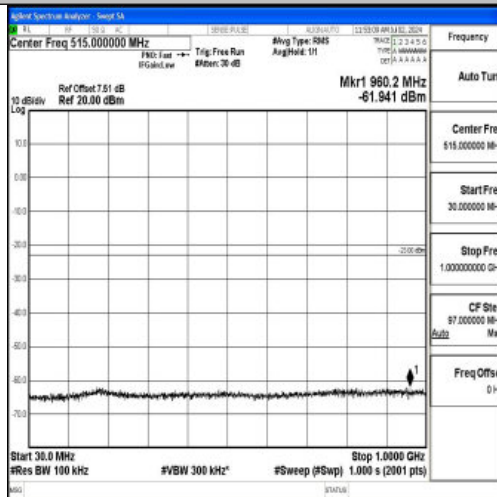
Band4_10MHz_16QAM_20175_1RB#0_30~1000_30~1000
