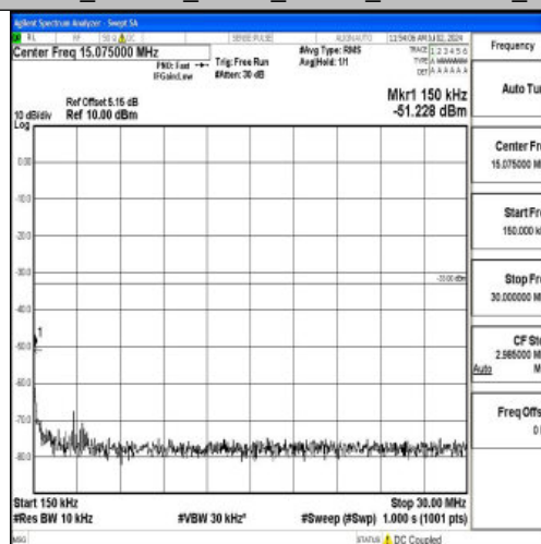
Band4_10MHz_16QAM_20350_1RB#0_0.15~30_0.15~30
