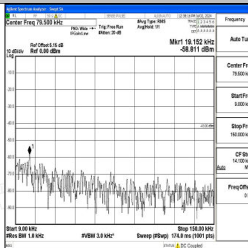
Band4_20MHz_16QAM_20300_1RB#0_0.009~0.15_0.009~0.15
