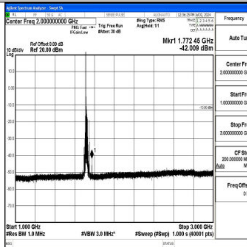
Band4_20MHz_16QAM_20050_1RB#0_1000~3000_1000~3000
