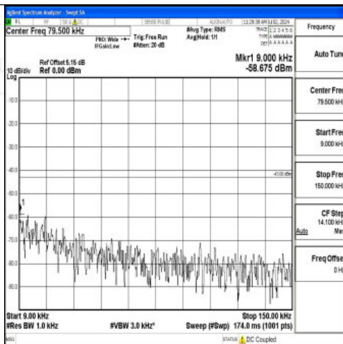
Band4_5MHz_16QAM_20175_1RB#0_0.009~0.15_0.009~0.15
