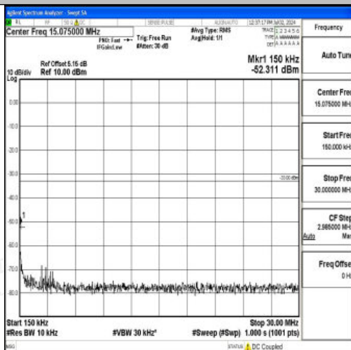
Band4_20MHz_16QAM_20175_1RB#0_0.15~30_0.15~30
