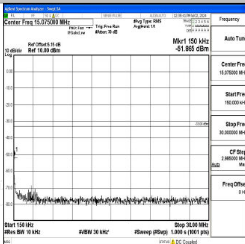
Band4_20MHz_QPSK_20050_1RB#0_0.15~30_0.15~30
