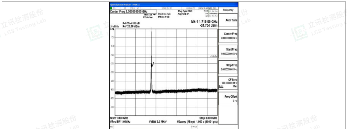
Band4_3MHz_QPSK_19965_1RB#0_1000~3000_1000~3000
