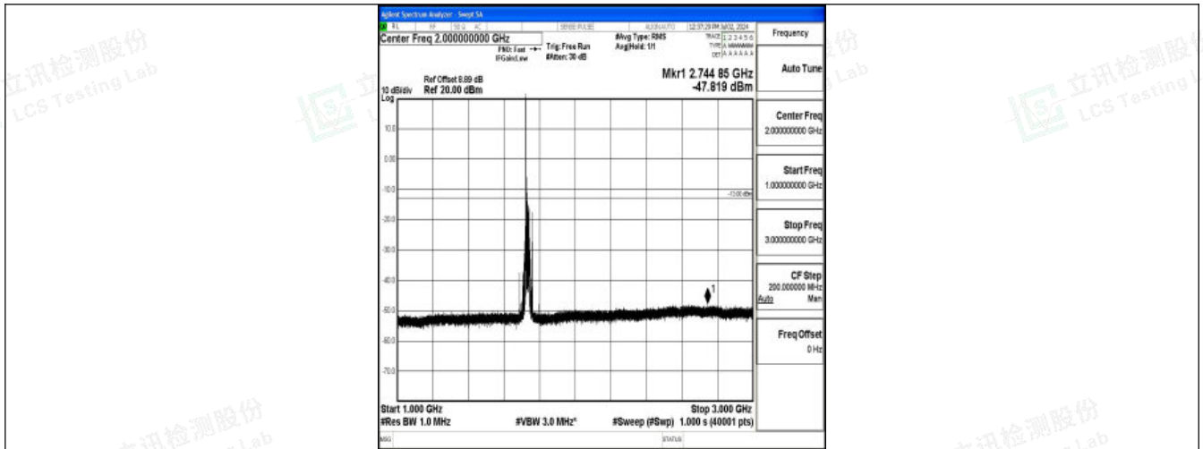
Band4_20MHz_16QAM_20175_1RB#0_1000~3000_1000~3000
