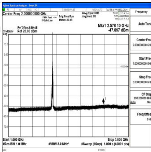
Band4_10MHz_16QAM_20175_1RB#0_1000~3000_1000~3000
