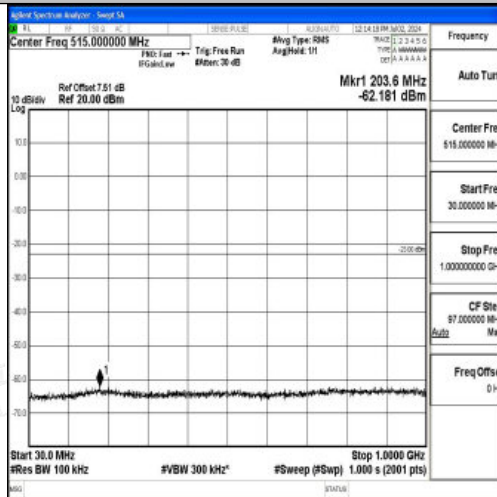
Band4_15MHz_16QAM_20025_1RB#0_30~1000_30~1000
