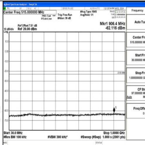
Band4_15MHz_QPSK_20325_1RB#0_30~1000_30~1000
