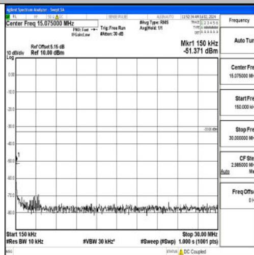
Band4_10MHz_QPSK_20175_1RB#0_0.15~30_0.15~30
