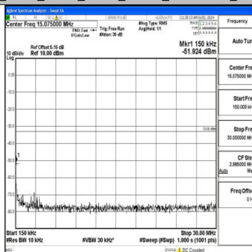
Band4_5MHz_QPSK_20175_1RB#0_0.15~30_0.15~30
