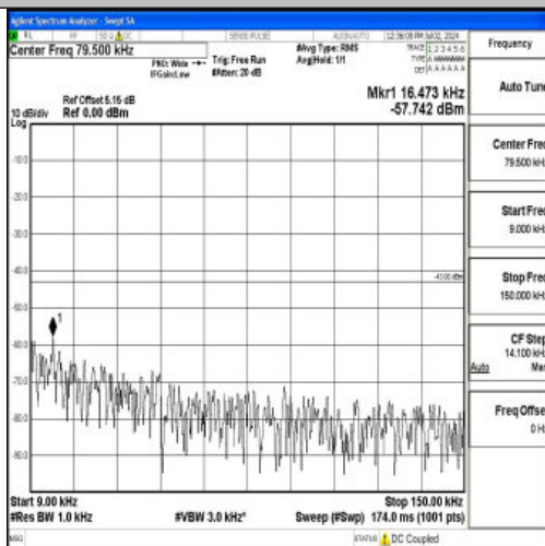
Band4_20MHz_16QAM_20050_1RB#0_0.009~0.15_0.009~0.15
