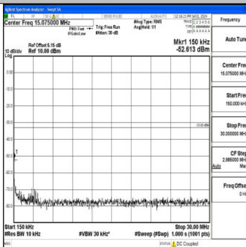
Band4_15MHz_16QAM_20325_1RB#0_0.15~30_0.15~30
