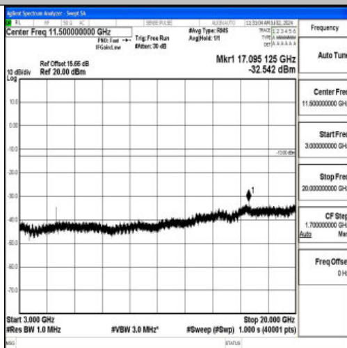
Band4_5MHz_16QAM_20375_1RB#0_3000~20000_3000~20000
