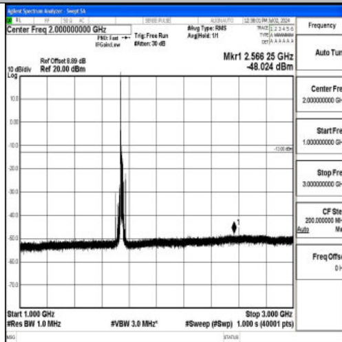
Band4_20MHz_QPSK_20300_1RB#0_1000~3000_1000~3000
