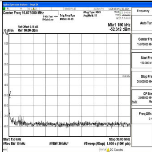
Band4_5MHz_QPSK_19975_1RB#0_0.15~30_0.15~30
