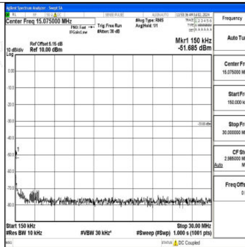
Band4_10MHz_QPSK_20350_1RB#0_0.15~30_0.15~30
