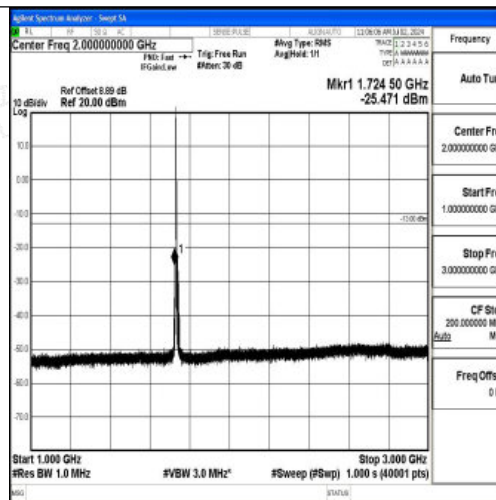
Band4_3MHz_16QAM_20175_1RB#0_1000~3000_1000~3000
