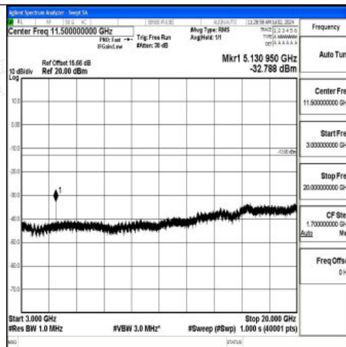
Band4_5MHz_16QAM_19975_1RB#0_3000~20000_3000~20000
