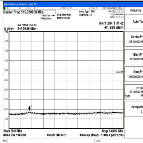
Band4_10MHz_QPSK_20350_1RB#0_30~1000_30~1000
