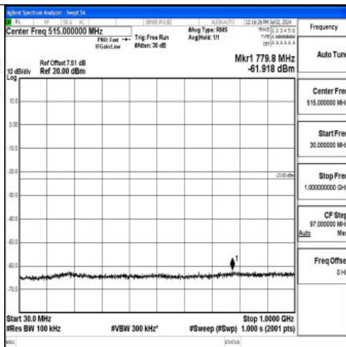
Band4_15MHz_16QAM_20325_1RB#0_30~1000_30~1000
