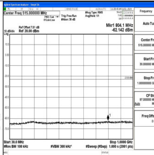
Band4_5MHz_16QAM_19975_1RB#0_30~1000_30~1000
