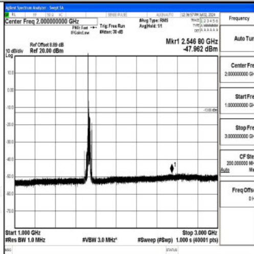
Band4_20MHz_QPSK_20175_1RB#0_1000~3000_1000~3000
