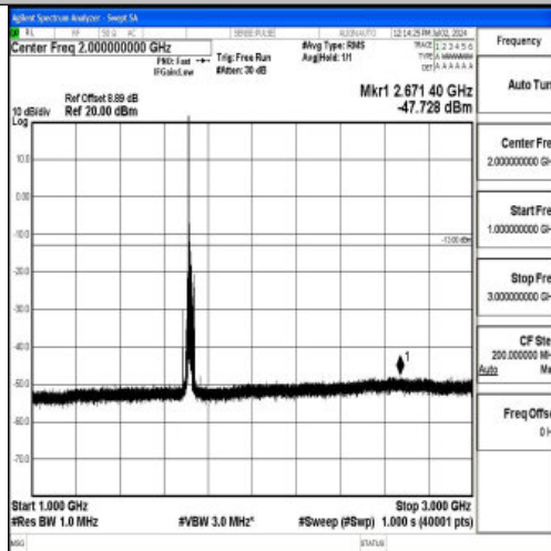
Band4_15MHz_16QAM_20025_1RB#0_1000~3000_1000~3000
