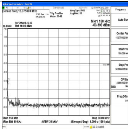
Band4_20MHz_QPSK_20300_1RB#0_0.15~30_0.15~30
