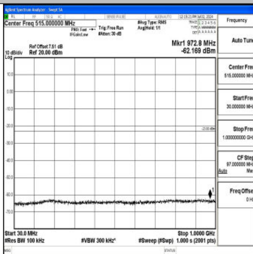
Band4_15MHz_16QAM_20175_1RB#0_30~1000_30~1000
