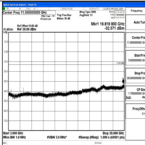
Band4_5MHz_QPSK_20175_1RB#0_3000~20000_3000~20000
