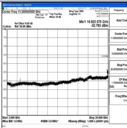
Band4_20MHz_16QAM_20300_1RB#0_3000~20000_3000~20000
