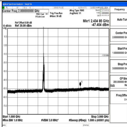
Band4_10MHz_16QAM_20000_1RB#0_1000~3000_1000~3000
