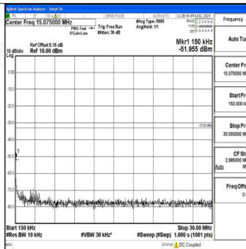
Band4_5MHz_16QAM_19975_1RB#0_0.15~30_0.15~30
