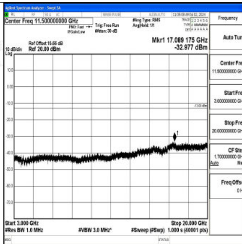
Band4_3MHz_16QAM_19965_1RB#0_3000~20000_3000~20000
