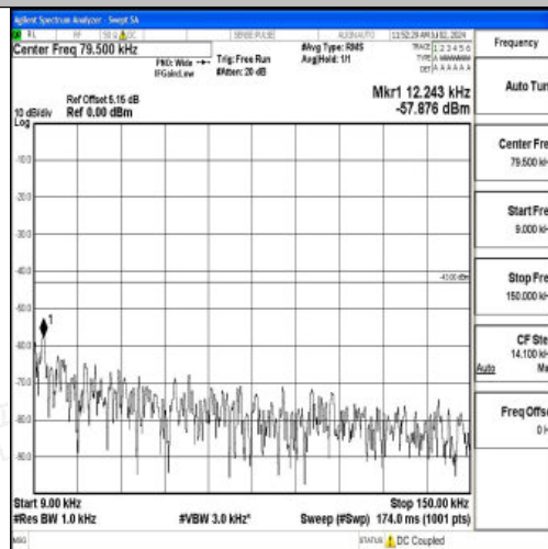
Band4_10MHz_QPSK_20175_1RB#0_0.009~0.15_0.009~0.15
