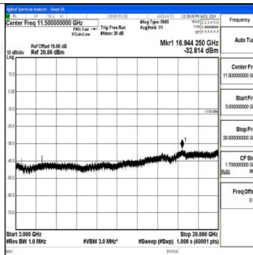
Band4_20MHz_QPSK_20300_1RB#0_3000~20000_3000~20000
