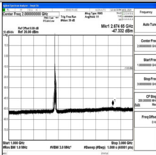
Band4_15MHz_16QAM_20325_1RB#0_1000~3000_1000~3000
