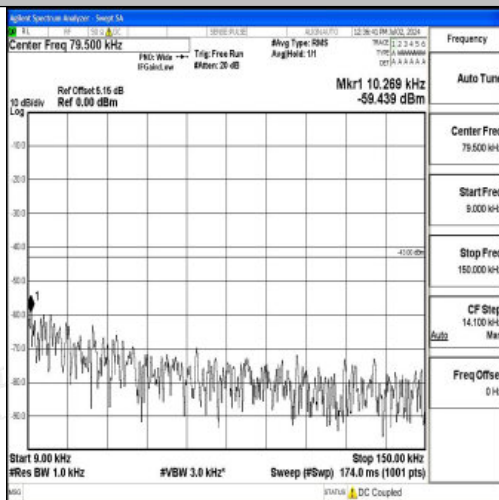
Band4_20MHz_QPSK_20175_1RB#0_0.009~0.15_0.009~0.15
