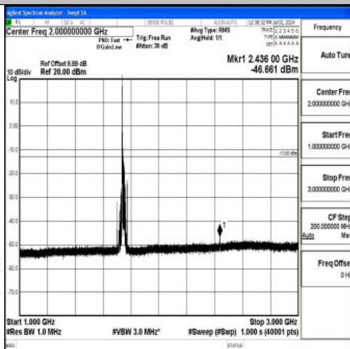
Band4_20MHz_16QAM_20300_1RB#0_1000~3000_1000~3000
