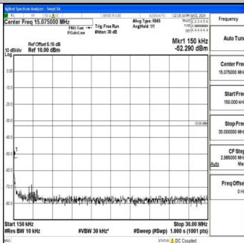
Band4_15MHz_16QAM_20175_1RB#0_0.15~30_0.15~30
