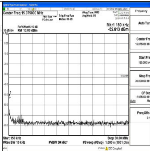
Band4_10MHz_16QAM_20000_1RB#0_0.15~30_0.15~30
