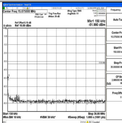
Band4_20MHz_16QAM_20300_1RB#0_0.15~30_0.15~30
