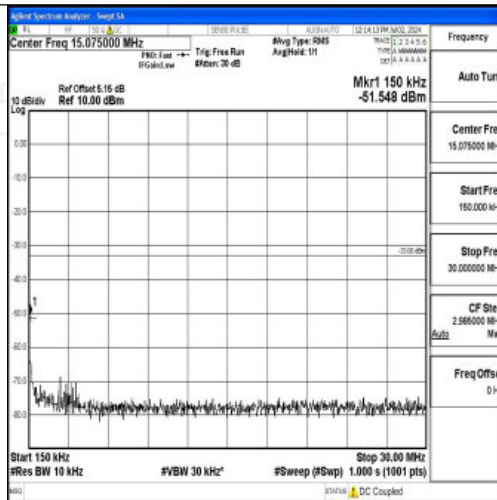
Band4_15MHz_16QAM_20025_1RB#0_0.15~30_0.15~30
