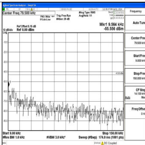
Band4_20MHz_QPSK_20050_1RB#0_0.009~0.15_0.009~0.15
