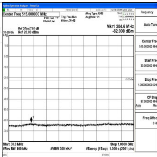
Band4_20MHz_16QAM_20300_1RB#0_30~1000_30~1000
