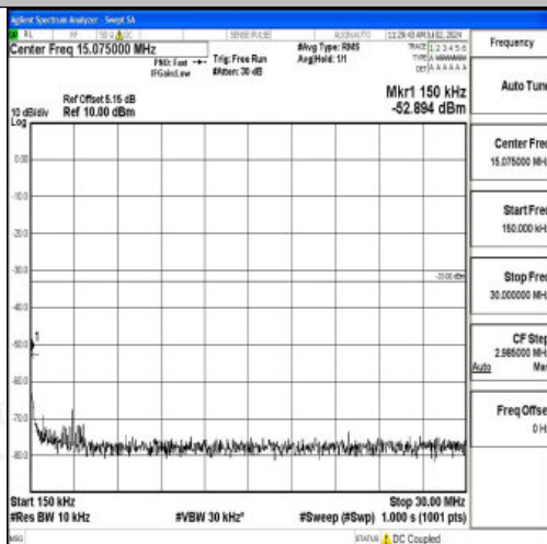
Band4_5MHz_16QAM_20175_1RB#0_0.15~30_0.15~30
