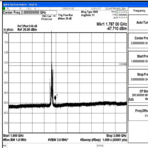
Band4_15MHz_QPSK_20175_1RB#0_1000~3000_1000~3000
