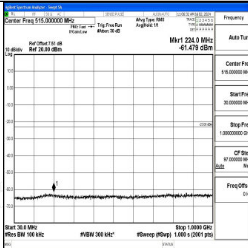
Band4_3MHz_QPSK_20385_1RB#0_30~1000_30~1000
