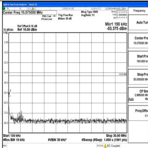
Band4_10MHz_16QAM_20175_1RB#0_0.15~30_0.15~30
