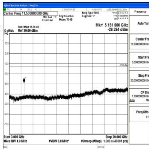
Band4_10MHz_16QAM_20000_1RB#0_3000~20000_3000~20000
