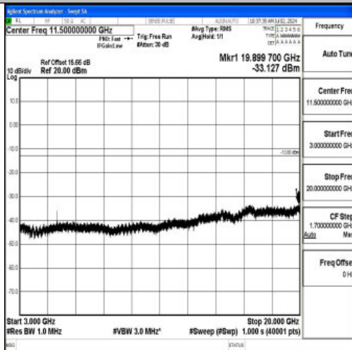
Band4_1.4MHz_16QAM_20393_1RB#0_3000~20000_3000~20000
