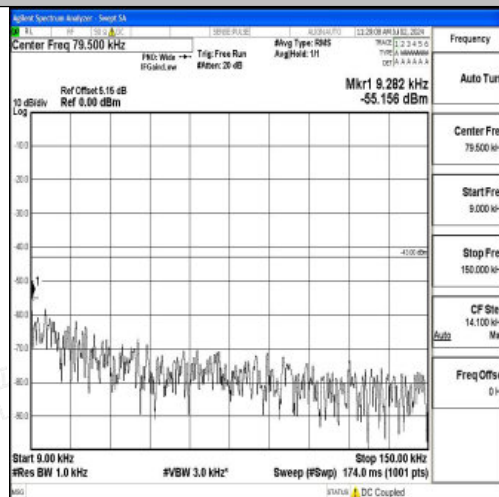
Band4_5MHz_QPSK_20175_1RB#0_0.009~0.15_0.009~0.15
