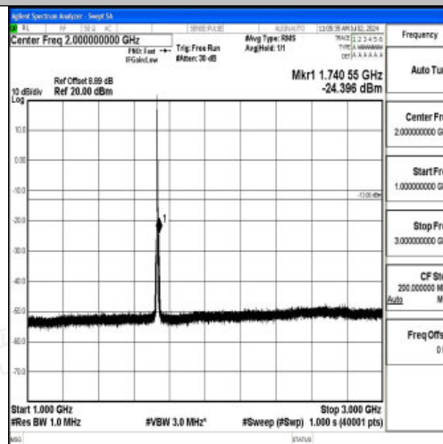
Band4_3MHz_QPSK_20175_1RB#0_1000~3000_1000~3000
