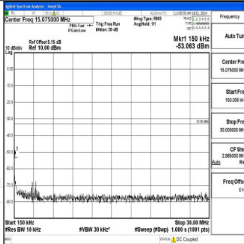
Band4_3MHz_16QAM_20175_1RB#0_0.15~30_0.15~30
