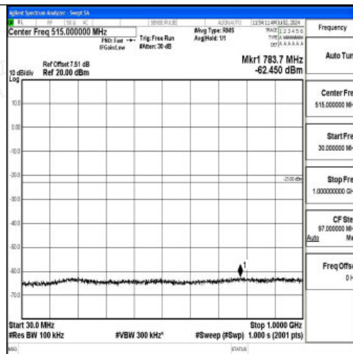
Band4_10MHz_16QAM_20350_1RB#0_30~1000_30~1000
