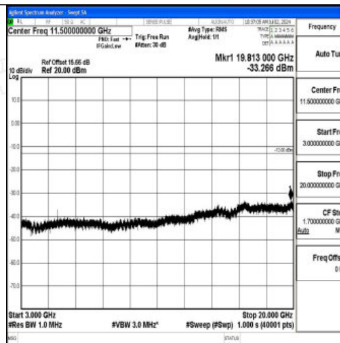
Band4_1.4MHz_QPSK_20393_1RB#0_3000~20000_3000~20000
