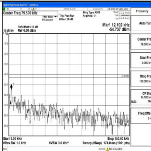
Band4_5MHz_QPSK_20375_1RB#0_0.009~0.15_0.009~0.15
