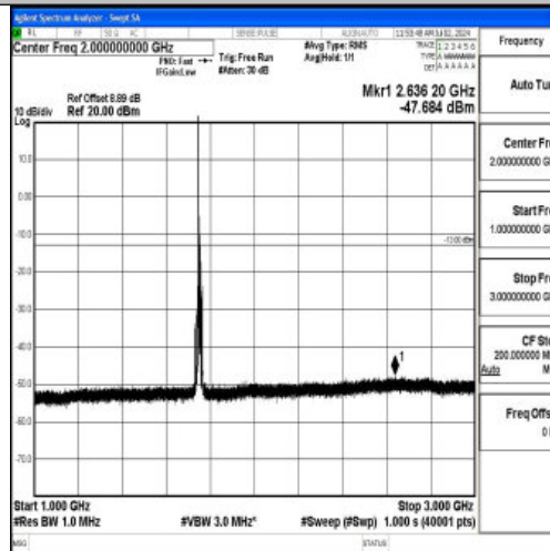
Band4_10MHz_QPSK_20350_1RB#0_1000~3000_1000~3000
