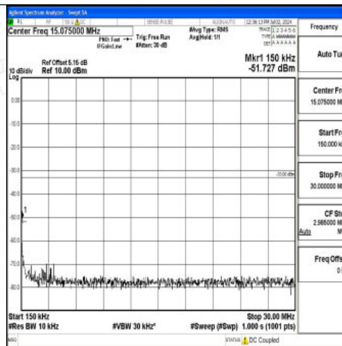
Band4_20MHz_16QAM_20050_1RB#0_0.15~30_0.15~30
