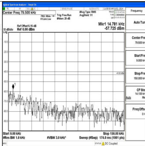
Band4_3MHz_16QAM_20175_1RB#0_0.009~0.15_0.009~0.15
