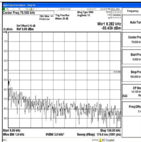
Band4_15MHz_QPSK_20025_1RB#0_0.009~0.15_0.009~0.15
