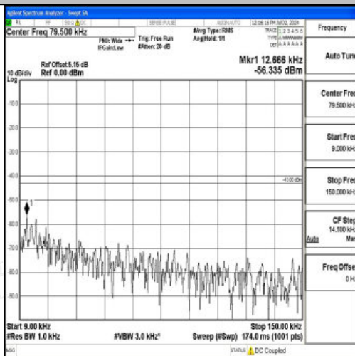
Band4_15MHz_16QAM_20325_1RB#0_0.009~0.15_0.009~0.15
