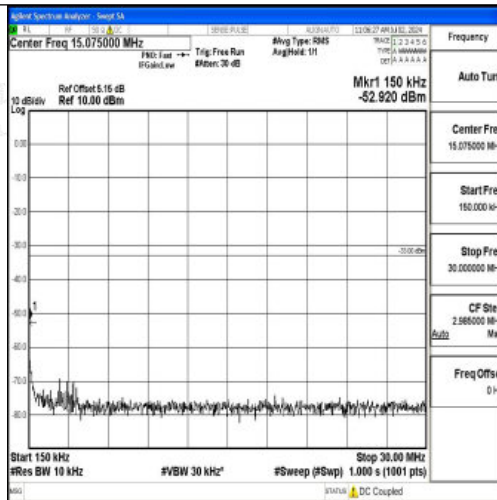
Band4_3MHz_QPSK_20385_1RB#0_0.15~30_0.15~30
