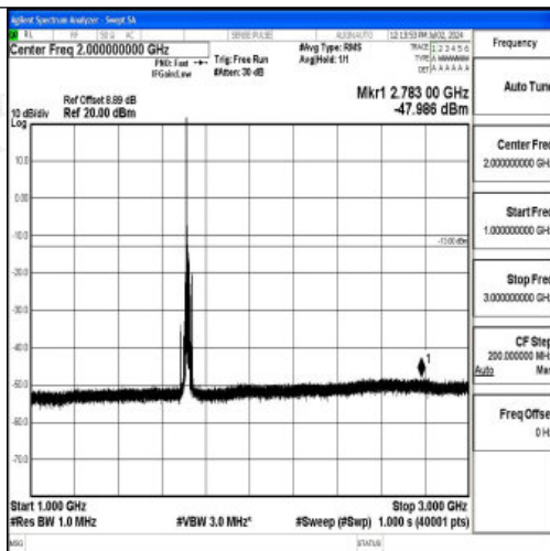
Band4_15MHz_QPSK_20025_1RB#0_1000~3000_1000~3000
