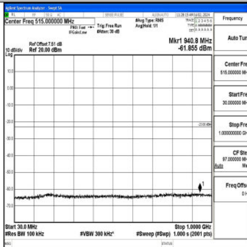
Band4_5MHz_QPSK_19975_1RB#0_30~1000_30~1000
