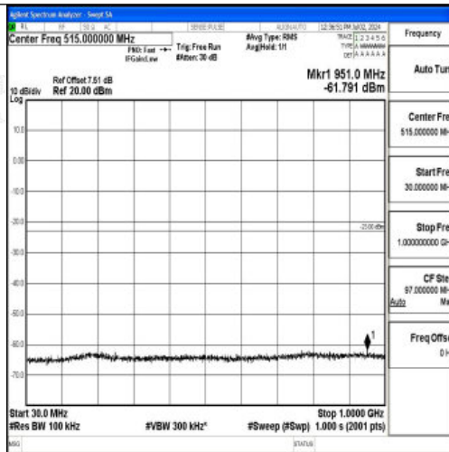
Band4_20MHz_QPSK_20175_1RB#0_30~1000_30~1000
