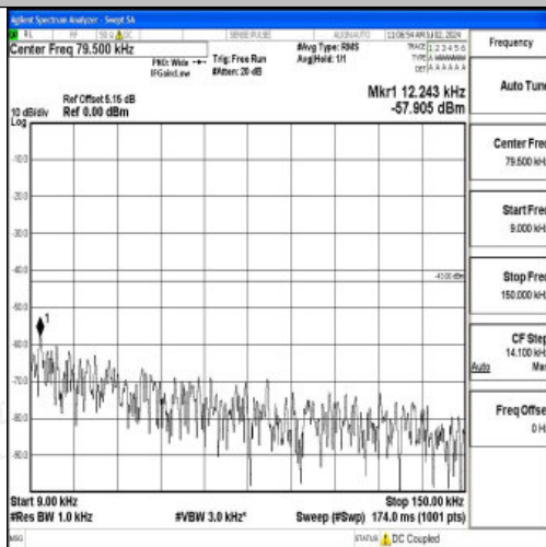
Band4_3MHz_16QAM_20385_1RB#0_0.009~0.15_0.009~0.15
