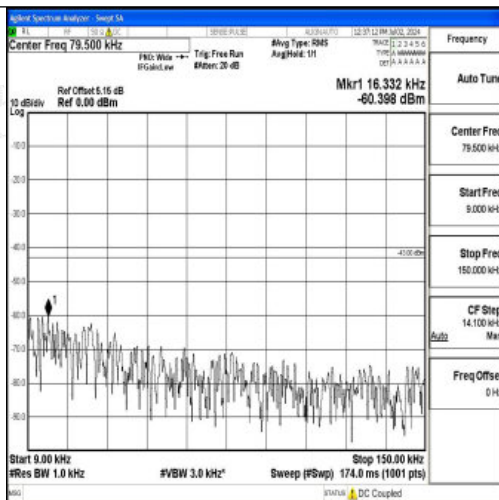
Band4_20MHz_16QAM_20175_1RB#0_0.009~0.15_0.009~0.15
