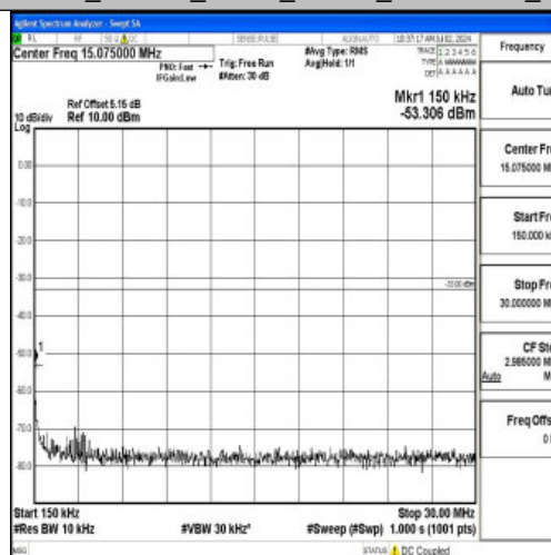
Band4_1.4MHz_16QAM_20393_1RB#0_0.15~30_0.15~30
