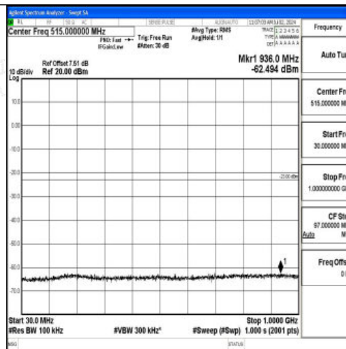
Band4_3MHz_16QAM_20385_1RB#0_30~1000_30~1000
