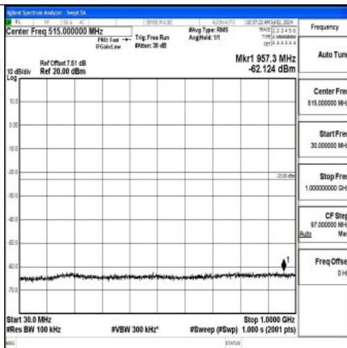
Band4_1.4MHz_16QAM_20393_1RB#0_30~1000_30~1000
