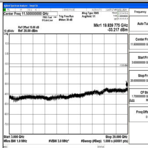
Band4_3MHz_16QAM_20385_1RB#0_3000~20000_3000~20000
