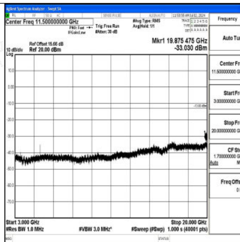
Band4_10MHz_QPSK_20350_1RB#0_3000~20000_3000~20000
