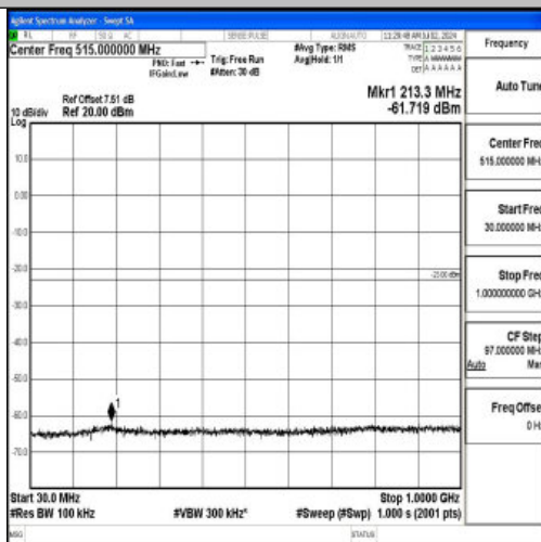
Band4_5MHz_16QAM_20175_1RB#0_30~1000_30~1000
