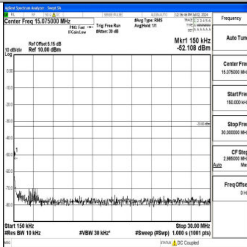
Band4_20MHz_QPSK_20175_1RB#0_0.15~30_0.15~30
