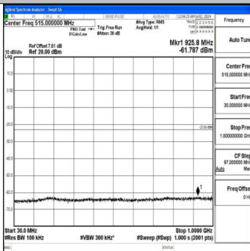
Band4_3MHz_QPSK_19965_1RB#0_30~1000_30~1000
