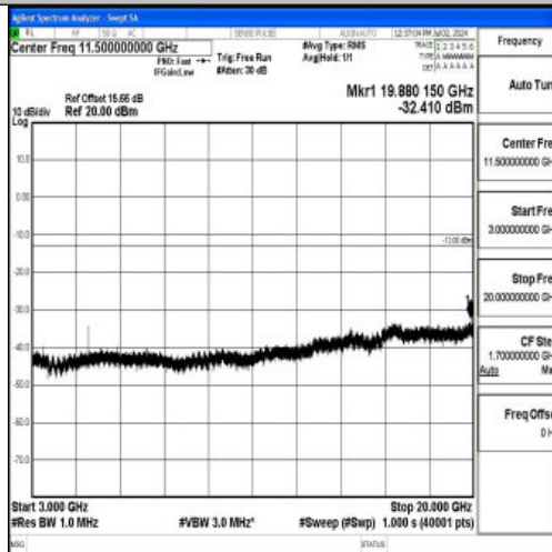
Band4_20MHz_QPSK_20175_1RB#0_3000~20000_3000~20000
