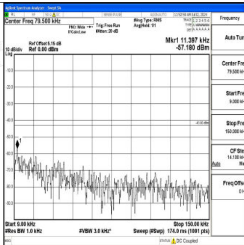
Band4_10MHz_16QAM_20175_1RB#0_0.009~0.15_0.009~0.15
