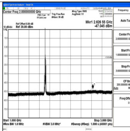
Band4_10MHz_QPSK_20000_1RB#0_1000~3000_1000~3000
