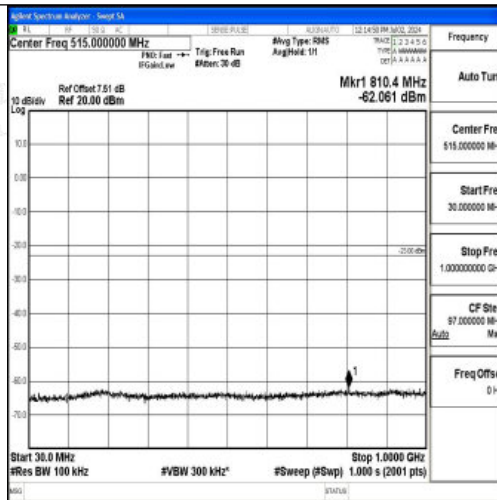
Band4_15MHz_QPSK_20175_1RB#0_30~1000_30~1000
