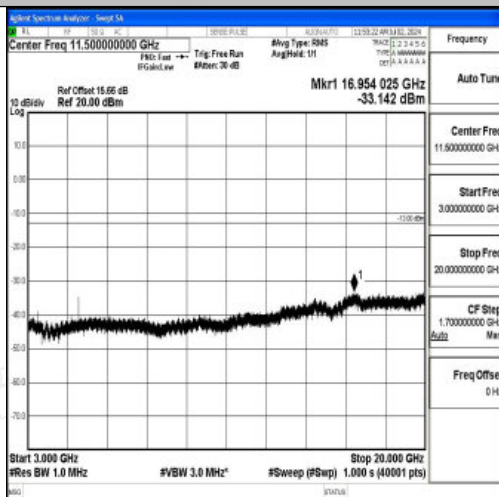
Band4_10MHz_16QAM_20175_1RB#0_3000~20000_3000~20000
