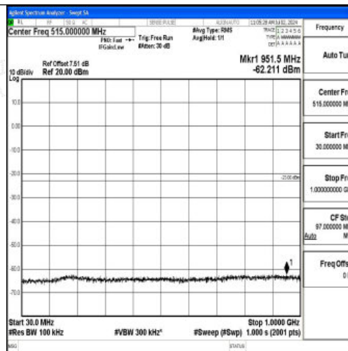
Band4_3MHz_QPSK_20175_1RB#0_30~1000_30~1000
