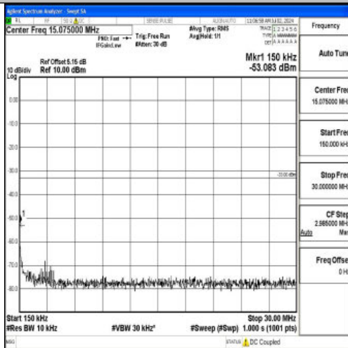
Band4_3MHz_16QAM_20385_1RB#0_0.15~30_0.15~30
