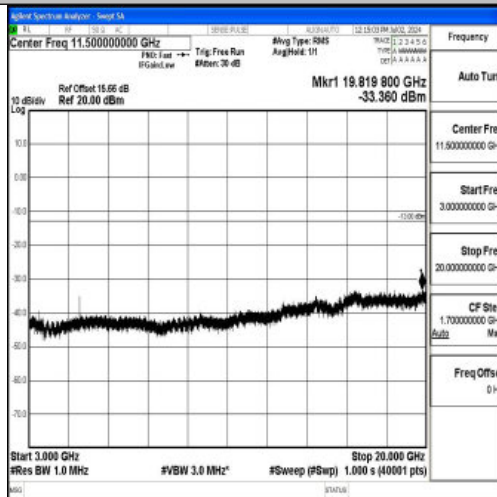
Band4_15MHz_QPSK_20175_1RB#0_3000~20000_3000~20000
