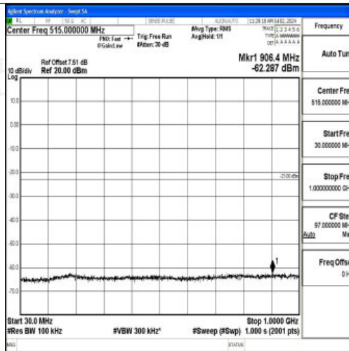
Band4_5MHz_QPSK_20175_1RB#0_30~1000_30~1000
