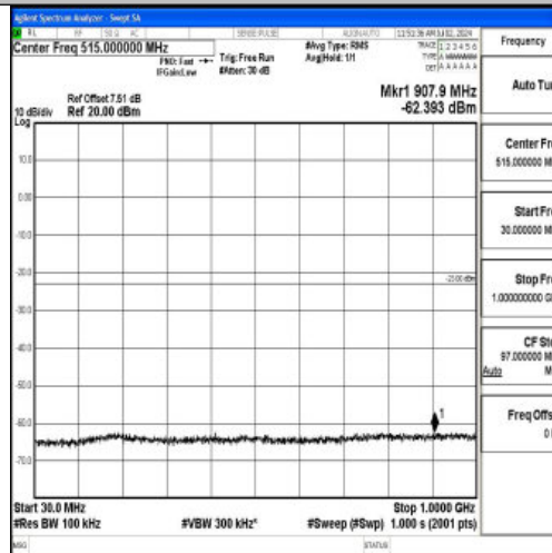
Band4_10MHz_QPSK_20000_1RB#0_30~1000_30~1000
