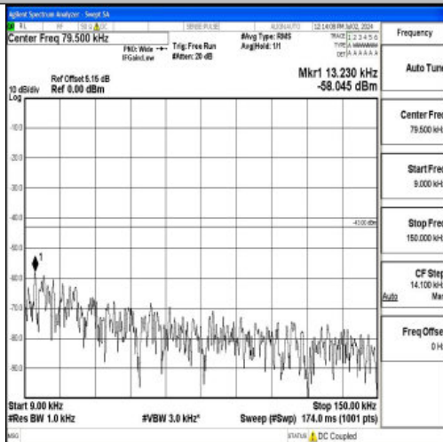
Band4_15MHz_16QAM_20025_1RB#0_0.009~0.15_0.009~0.15
