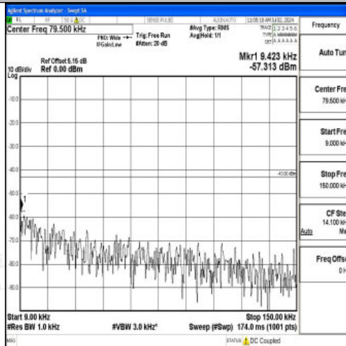
Band4_3MHz_QPSK_20175_1RB#0_0.009~0.15_0.009~0.15
