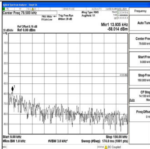
Band4_10MHz_QPSK_20350_1RB#0_0.009~0.15_0.009~0.15
