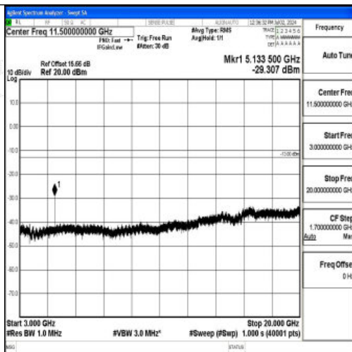
Band4_20MHz_16QAM_20050_1RB#0_3000~20000_3000~20000
