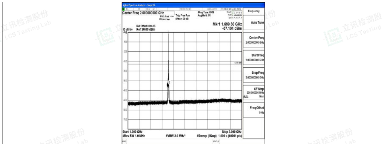
Band4_5MHz_QPSK_19975_1RB#0_1000~3000_1000~3000
