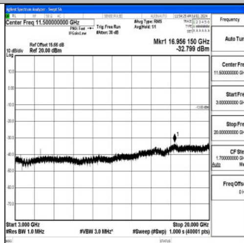
Band4_10MHz_16QAM_20350_1RB#0_3000~20000_3000~20000
