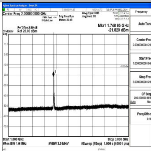
Band4_1.4MHz_16QAM_20393_1RB#0_1000~3000_1000~3000
