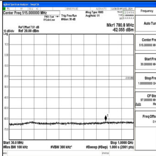
Band4_3MHz_16QAM_20175_1RB#0_30~1000_30~1000
