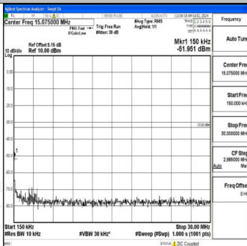
Band4_3MHz_QPSK_19965_1RB#0_0.15~30_0.15~30
