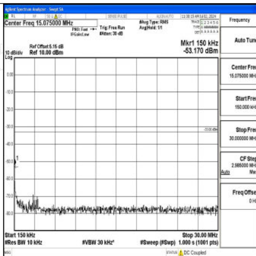
Band4_5MHz_QPSK_20375_1RB#0_0.15~30_0.15~30
