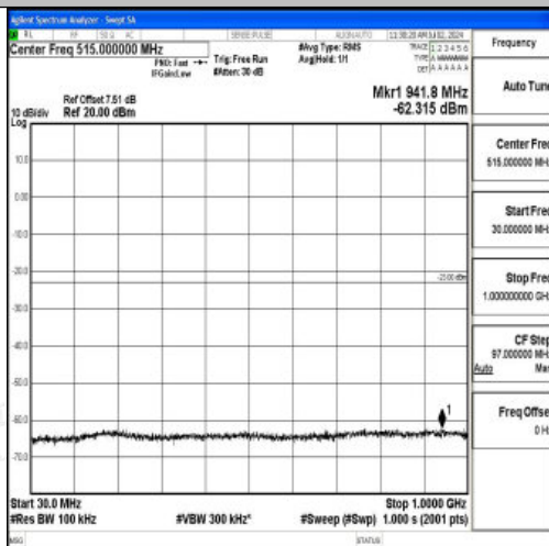
Band4_5MHz_QPSK_20375_1RB#0_30~1000_30~1000
