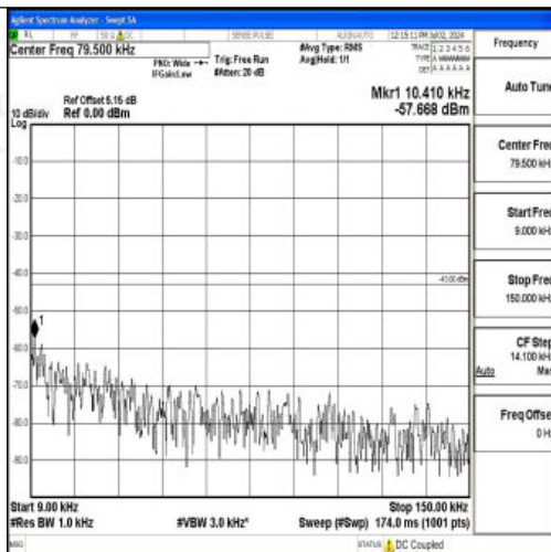
Band4_15MHz_16QAM_20175_1RB#0_0.009~0.15_0.009~0.15
