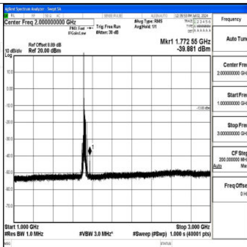
Band4_20MHz_QPSK_20050_1RB#0_1000~3000_1000~3000
