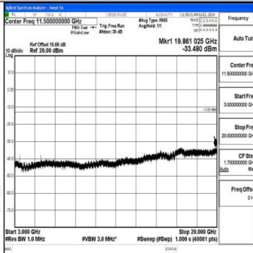
Band4_5MHz_16QAM_20175_1RB#0_3000~20000_3000~20000
