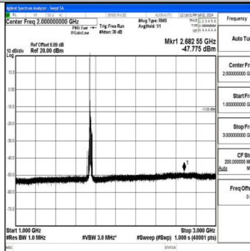
Band4_15MHz_QPSK_20325_1RB#0_1000~3000_1000~3000
