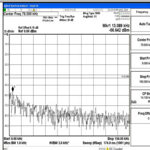
Band4_15MHz_QPSK_20325_1RB#0_0.009~0.15_0.009~0.15
