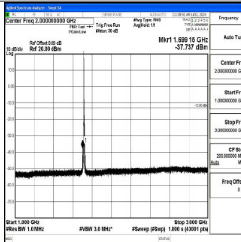
Band4_5MHz_16QAM_19975_1RB#0_1000~3000_1000~3000
