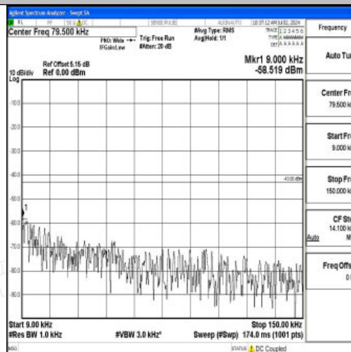
Band4_1.4MHz_16QAM_20393_1RB#0_0.009~0.15_0.009~0.15
