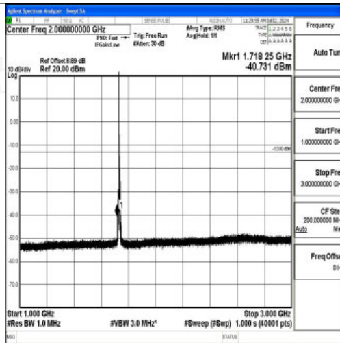
Band4_5MHz_16QAM_20175_1RB#0_1000~3000_1000~3000
