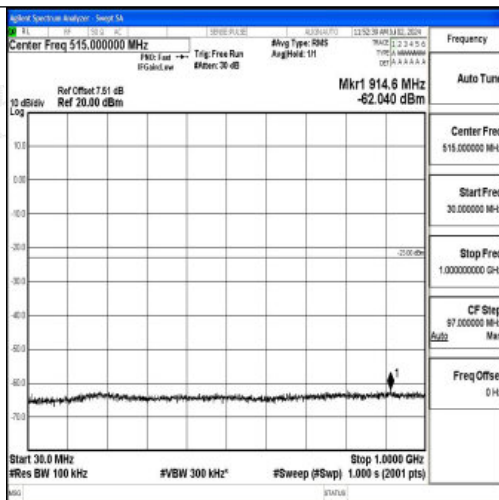
Band4_10MHz_QPSK_20175_1RB#0_30~1000_30~1000
