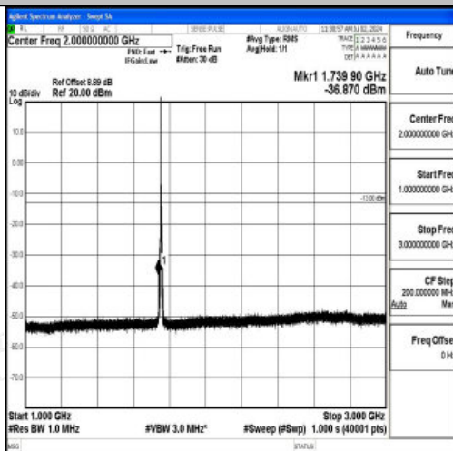
Band4_5MHz_16QAM_20375_1RB#0_1000~3000_1000~3000
