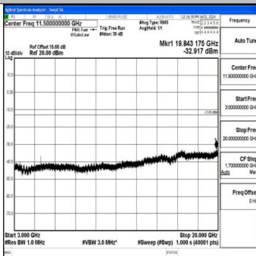
Band4_15MHz_16QAM_20325_1RB#0_3000~20000_3000~20000
