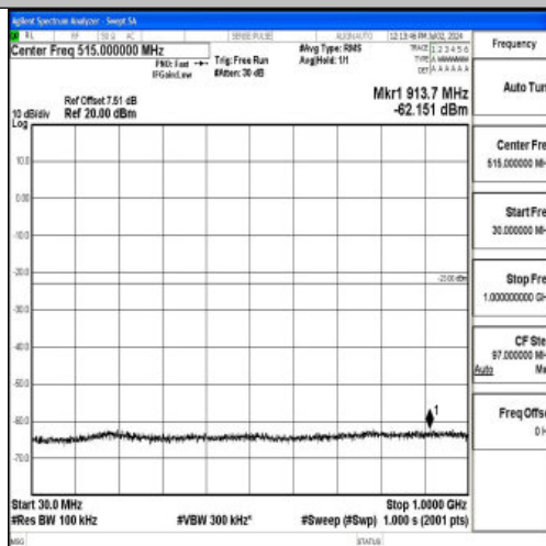
Band4_15MHz_QPSK_20025_1RB#0_30~1000_30~1000
