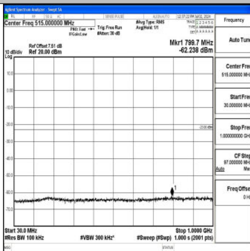
Band4_20MHz_16QAM_20175_1RB#0_30~1000_30~1000
