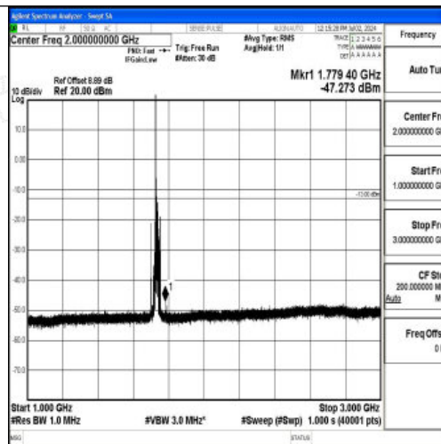
Band4_15MHz_16QAM_20175_1RB#0_1000~3000_1000~3000
