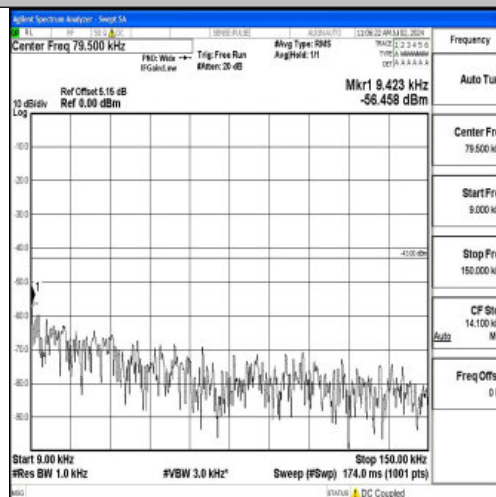
Band4_3MHz_QPSK_20385_1RB#0_0.009~0.15_0.009~0.15
