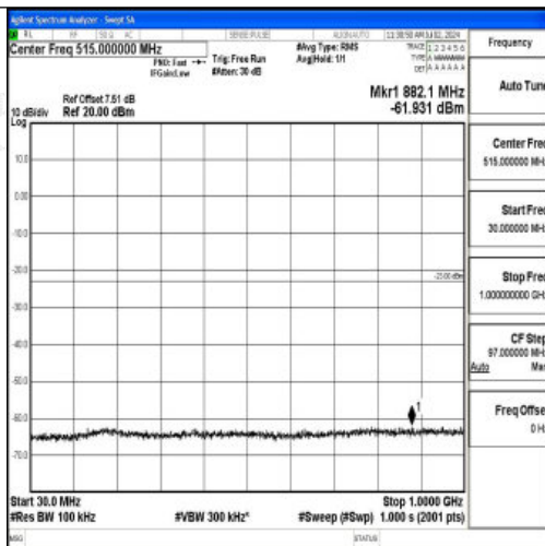
Band4_5MHz_16QAM_20375_1RB#0_30~1000_30~1000
