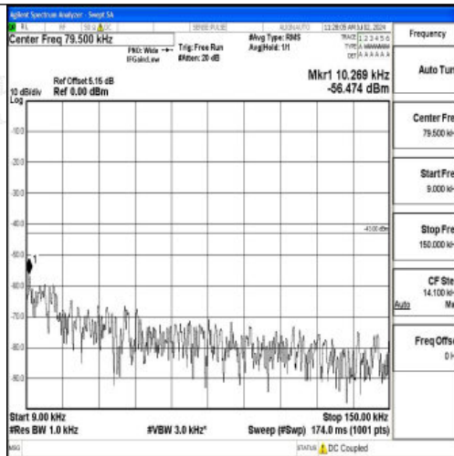
Band4_5MHz_QPSK_19975_1RB#0_0.009~0.15_0.009~0.15
