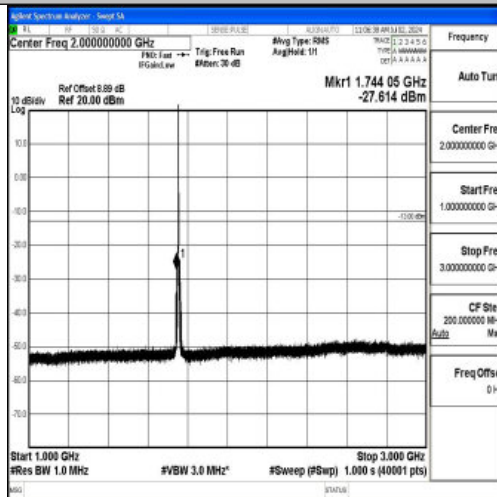
Band4_3MHz_QPSK_20385_1RB#0_1000~3000_1000~3000
