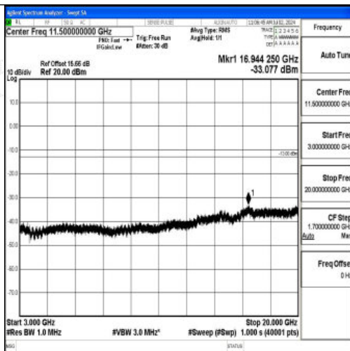
Band4_3MHz_QPSK_20385_1RB#0_3000~20000_3000~20000
