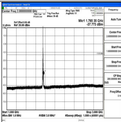
Band4_5MHz_QPSK_20375_1RB#0_1000~3000_1000~3000
