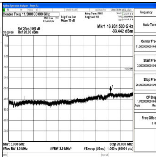
Band4_15MHz_QPSK_20325_1RB#0_3000~20000_3000~20000
