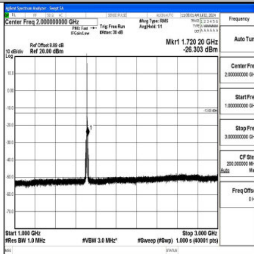
Band4_3MHz_16QAM_19965_1RB#0_1000~3000_1000~3000
