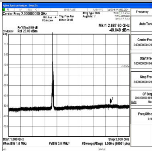
Band4_10MHz_QPSK_20175_1RB#0_1000~3000_1000~3000
