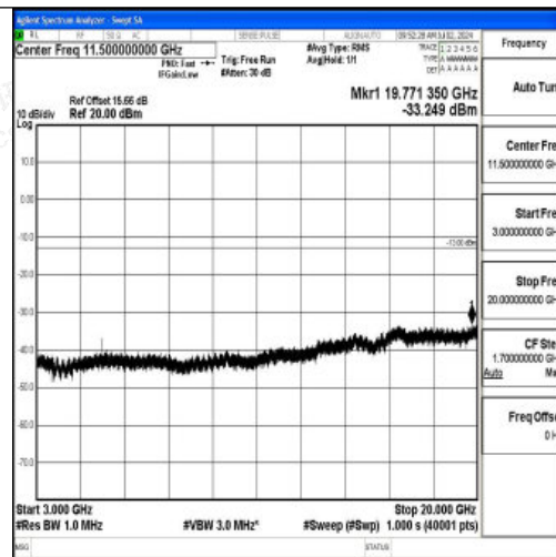
Band2_15MHz_16QAM_18675_1RB#0_3000~20000_3000~20000
