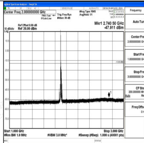
Band2_15MHz_16QAM_19125_1RB#0_1000~3000_1000~3000
