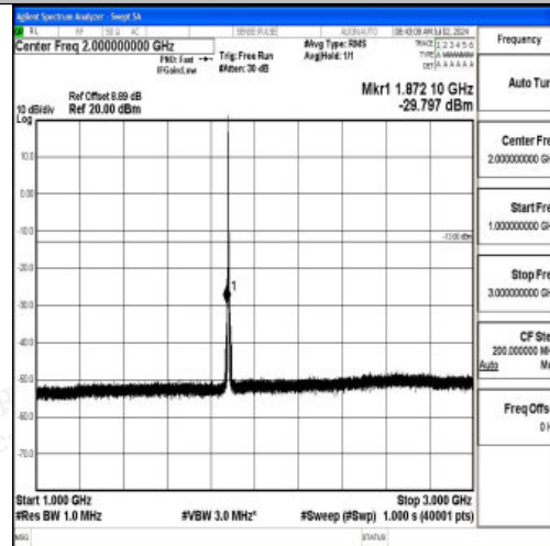
Band2_3MHz_QPSK_18900_1RB#0_1000~3000_1000~3000
