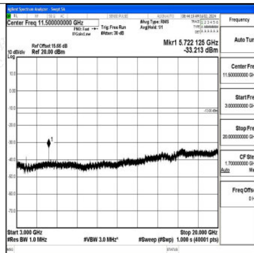
Band2_3MHz_QPSK_19185_1RB#0_3000~20000_3000~20000
