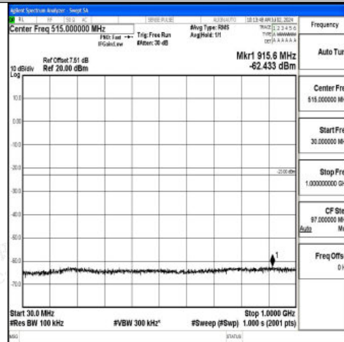
Band2_20MHz_16QAM_18700_1RB#0_30~1000_30~1000
