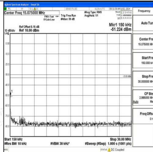
Band2_10MHz_16QAM_18900_1RB#0_0.15~30_0.15~30
