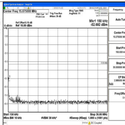
Band2_3MHz_16QAM_18615_1RB#0_0.15~30_0.15~30
