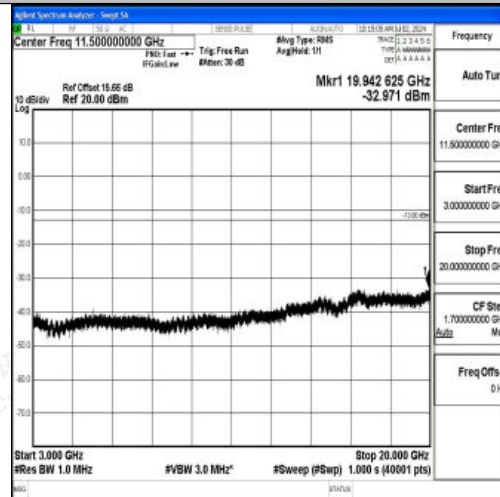
Band2_20MHz_16QAM_18900_1RB#0_3000~20000_3000~20000
