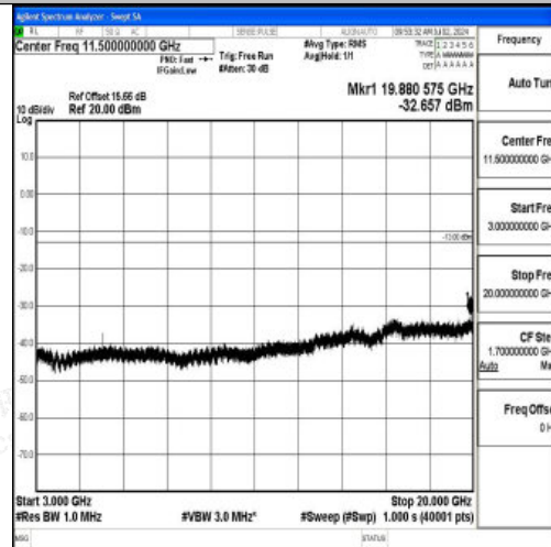
Band2_15MHz_16QAM_18900_1RB#0_3000~20000_3000~20000
