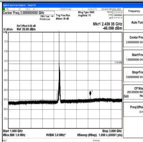
Band2_20MHz_16QAM_19100_1RB#0_1000~3000_1000~3000
