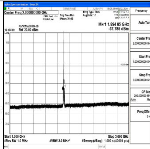
Band2_5MHz_16QAM_19175_1RB#0_1000~3000_1000~3000
