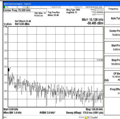
Band2_5MHz_16QAM_18625_1RB#0_0.009~0.15_0.009~0.15
