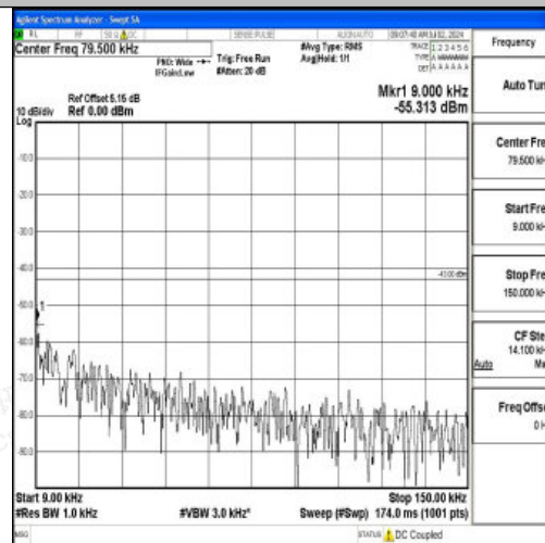
Band2_5MHz_QPSK_18900_1RB#0_0.009~0.15_0.009~0.15
