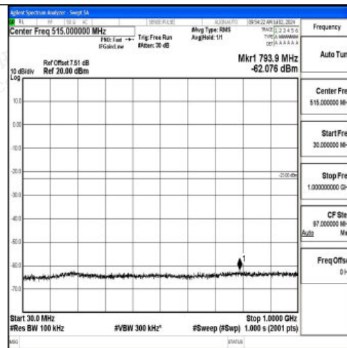
Band2_15MHz_16QAM_19125_1RB#0_30~1000_30~1000
