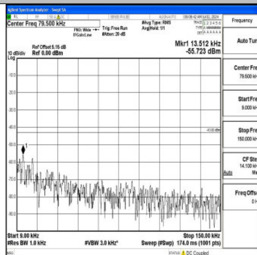
Band2_5MHz_QPSK_19175_1RB#0_0.009~0.15_0.009~0.15
