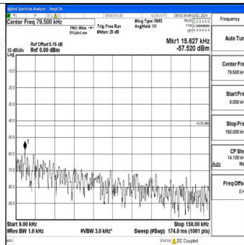
Band2_15MHz_QPSK_18675_1RB#0_0.009~0.15_0.009~0.15
