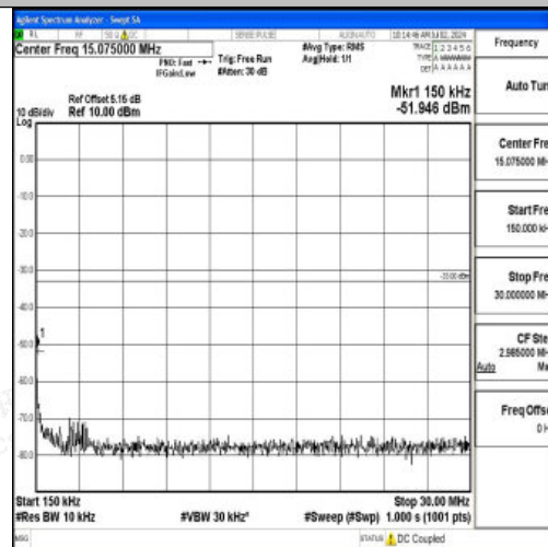
Band2_20MHz_16QAM_18900_1RB#0_0.15~30_0.15~30
