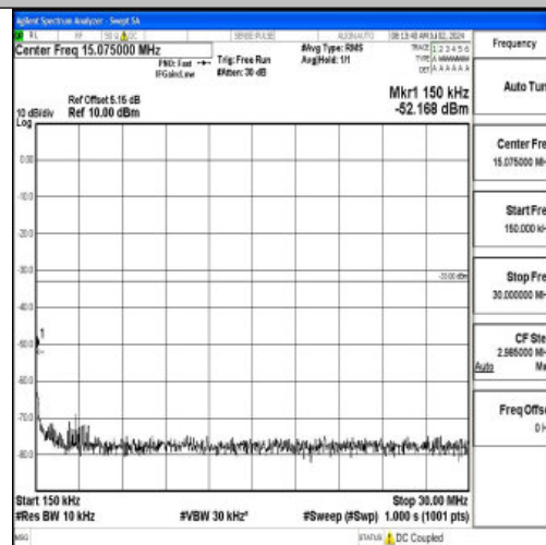
Band2_1.4MHz_16QAM_19193_1RB#0_0.15~30_0.15~30
