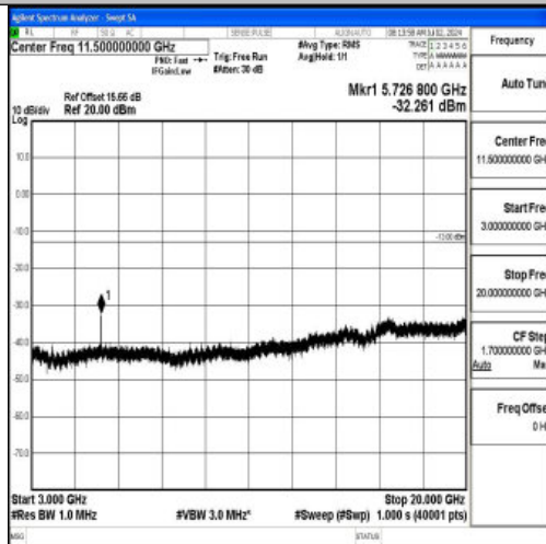
Band2_1.4MHz_16QAM_19193_1RB#0_3000~20000_3000~20000
