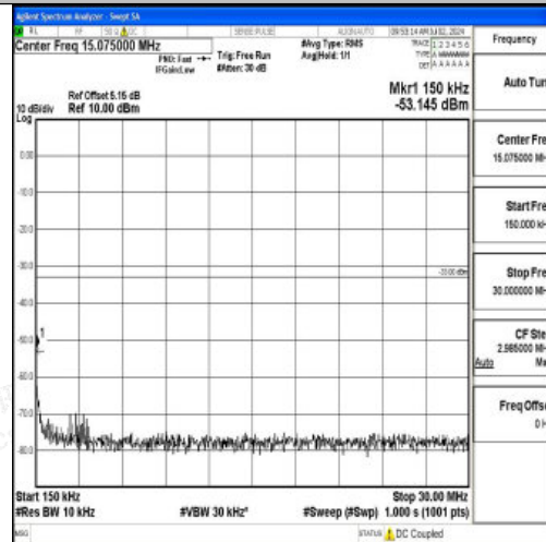
Band2_15MHz_16QAM_18900_1RB#0_0.15~30_0.15~30
