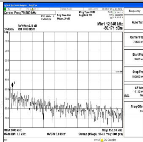
Band2_10MHz_16QAM_19150_1RB#0_0.009~0.15_0.009~0.15
