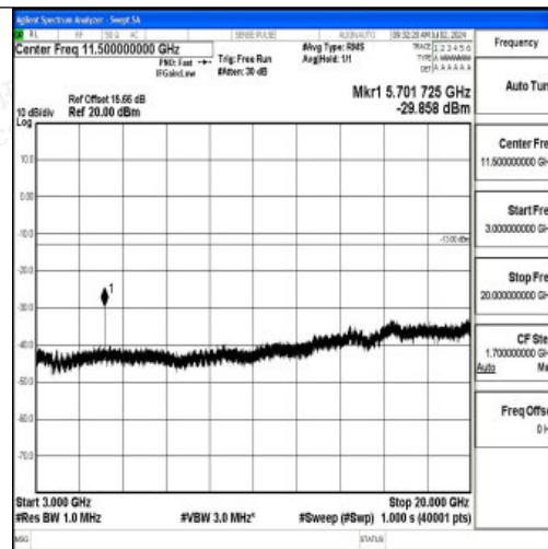
Band2_10MHz_QPSK_19150_1RB#0_3000~20000_3000~20000
