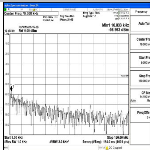
Band2_3MHz_16QAM_19185_1RB#0_0.009~0.15_0.009~0.15
