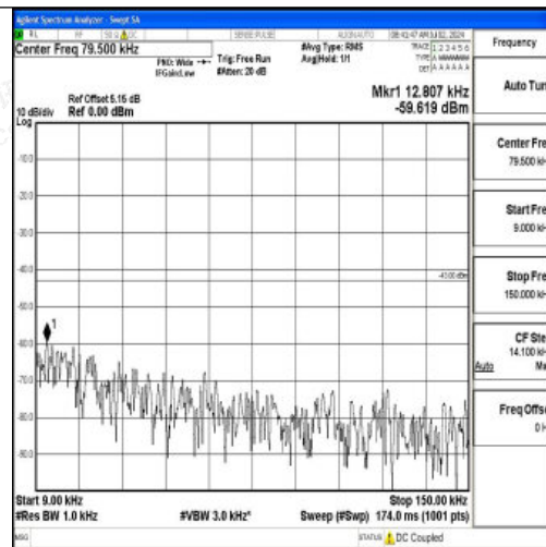
Band2_3MHz_QPSK_18615_1RB#0_0.009~0.15_0.009~0.15
