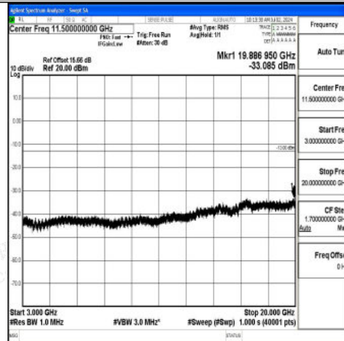
Band2_20MHz_QPSK_18700_1RB#0_3000~20000_3000~20000
