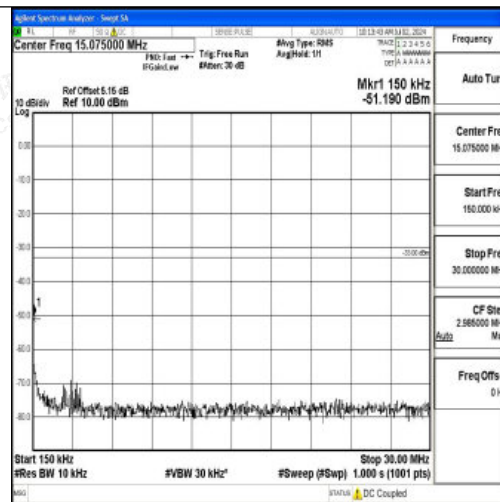
Band2_20MHz_16QAM_18700_1RB#0_0.15~30_0.15~30
