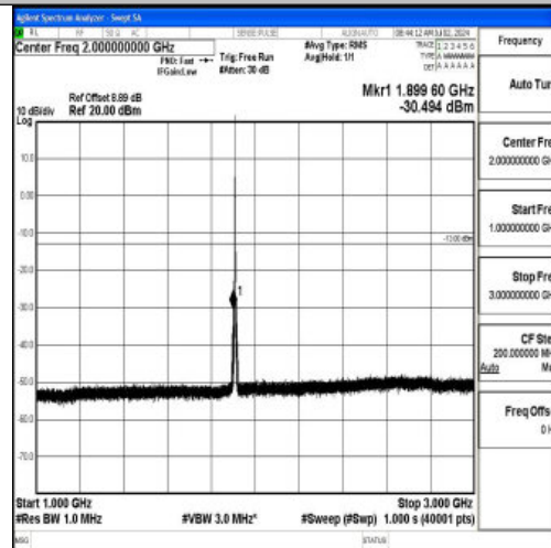
Band2_3MHz_QPSK_19185_1RB#0_1000~3000_1000~3000
