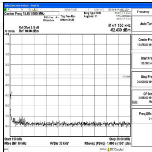
Band2_15MHz_QPSK_19125_1RB#0_0.15~30_0.15~30
