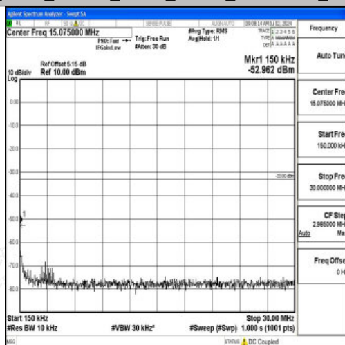
Band2_5MHz_16QAM_18900_1RB#0_0.15~30_0.15~30
