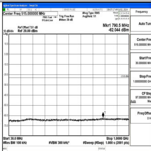
Band2_5MHz_16QAM_18625_1RB#0_30~1000_30~1000
