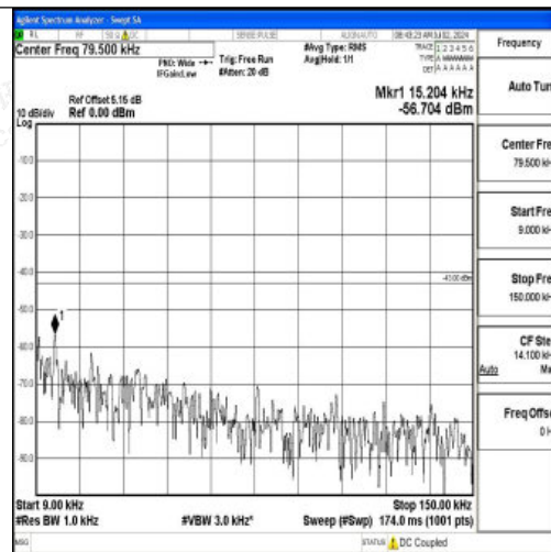
Band2_3MHz_16QAM_18900_1RB#0_0.009~0.15_0.009~0.15
