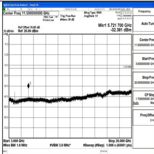
Band2_3MHz_16QAM_19185_1RB#0_3000~20000_3000~20000
