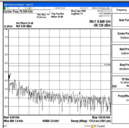
Band2_15MHz_16QAM_19125_1RB#0_0.009~0.15_0.009~0.15
