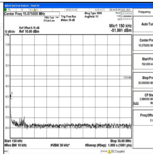
Band2_3MHz_QPSK_19185_1RB#0_0.15~30_0.15~30
