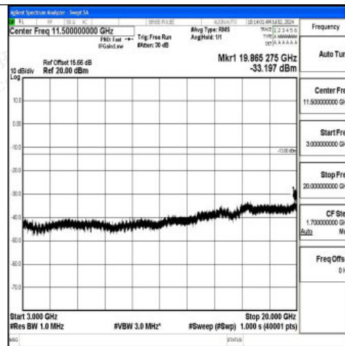
Band2_20MHz_16QAM_18700_1RB#0_3000~20000_3000~20000
