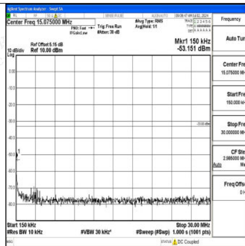
Band2_5MHz_QPSK_19175_1RB#0_0.15~30_0.15~30
