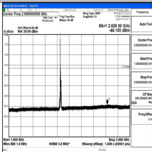
Band2_10MHz_16QAM_18650_1RB#0_1000~3000_1000~3000
