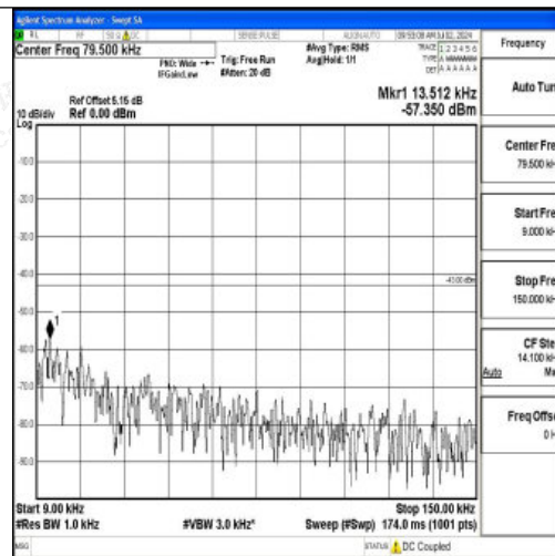
Band2_15MHz_16QAM_18900_1RB#0_0.009~0.15_0.009~0.15
