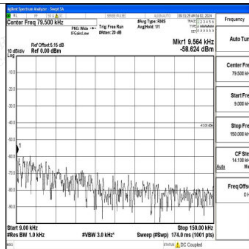
Band2_10MHz_16QAM_18900_1RB#0_0.009~0.15_0.009~0.15
