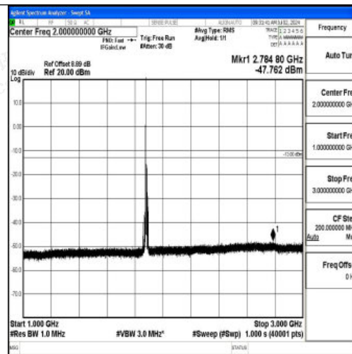
Band2_10MHz_16QAM_18900_1RB#0_1000~3000_1000~3000
