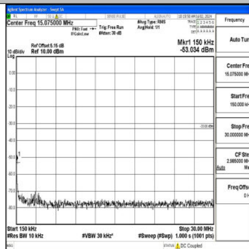
Band2_20MHz_16QAM_19100_1RB#0_0.15~30_0.15~30
