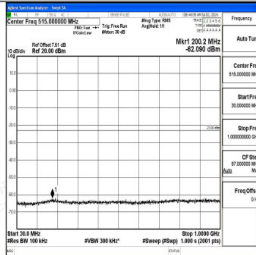
Band2_3MHz_QPSK_19185_1RB#0_30~1000_30~1000
