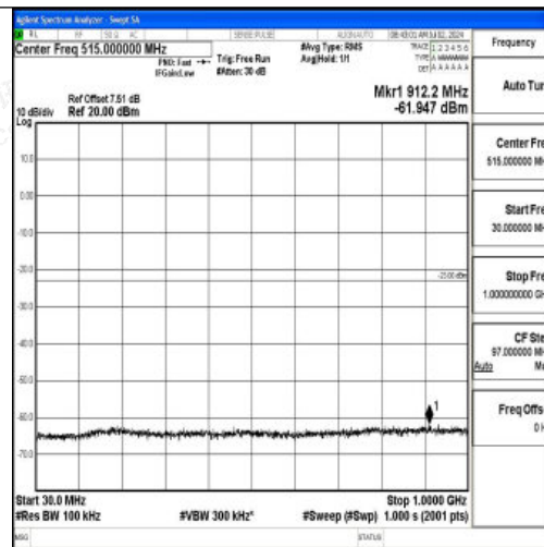
Band2_3MHz_QPSK_18900_1RB#0_30~1000_30~1000
