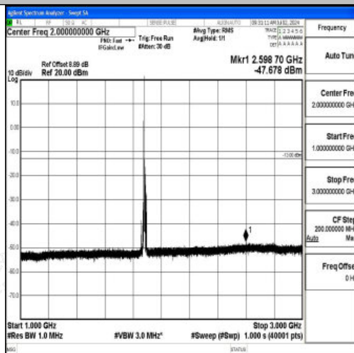
Band2_10MHz_QPSK_18900_1RB#0_1000~3000_1000~3000
