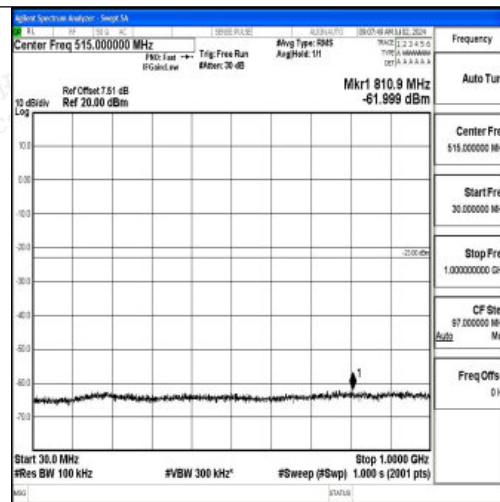
Band2_5MHz_QPSK_18900_1RB#0_30~1000_30~1000
