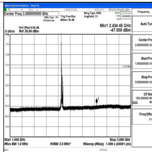
Band2_15MHz_QPSK_18675_1RB#0_1000~3000_1000~3000
