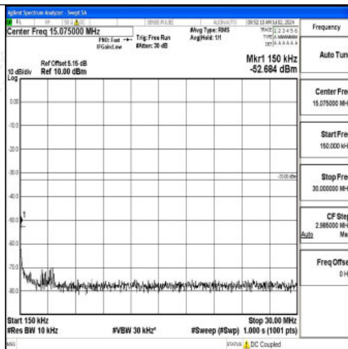
Band2_15MHz_16QAM_18675_1RB#0_0.15~30_0.15~30
