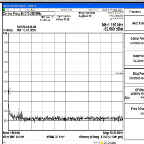
Band2_5MHz_QPSK_18625_1RB#0_0.15~30_0.15~30
