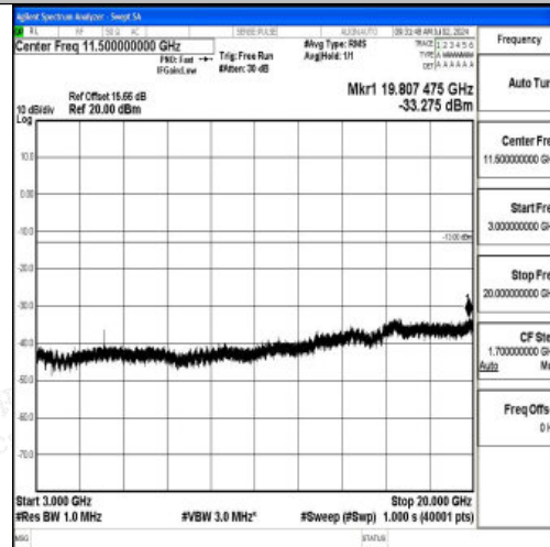
Band2_10MHz_16QAM_18900_1RB#0_3000~20000_3000~20000
