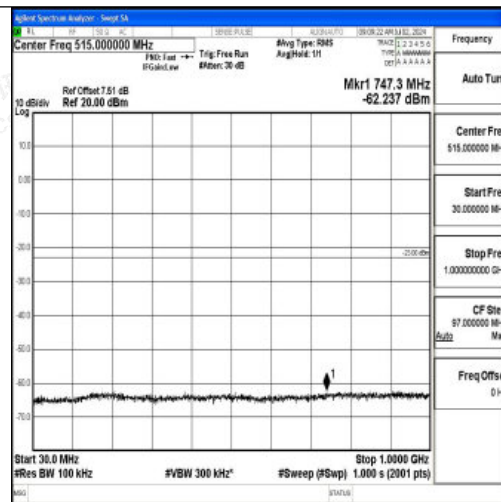
Band2_5MHz_16QAM_19175_1RB#0_30~1000_30~1000
