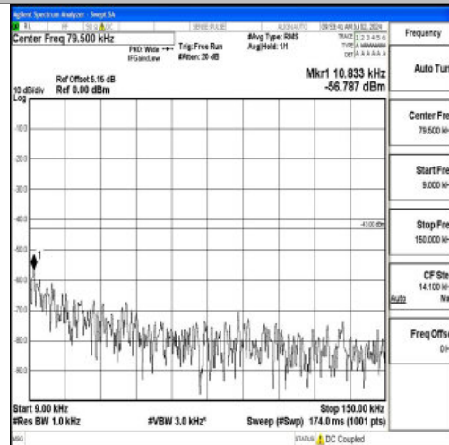
Band2_15MHz_QPSK_19125_1RB#0_0.009~0.15_0.009~0.15
