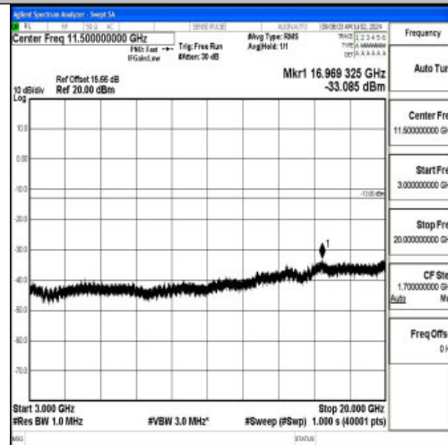
Band2_5MHz_QPSK_18900_1RB#0_3000~20000_3000~20000
