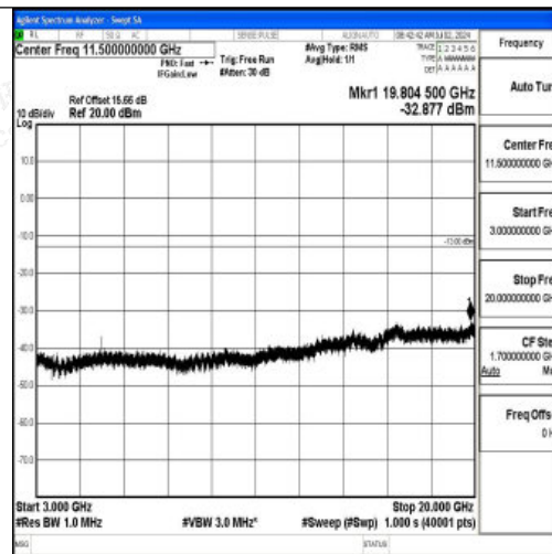
Band2_3MHz_16QAM_18615_1RB#0_3000~20000_3000~20000
