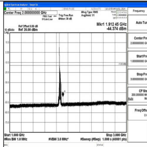
Band2_20MHz_16QAM_18700_1RB#0_1000~3000_1000~3000
