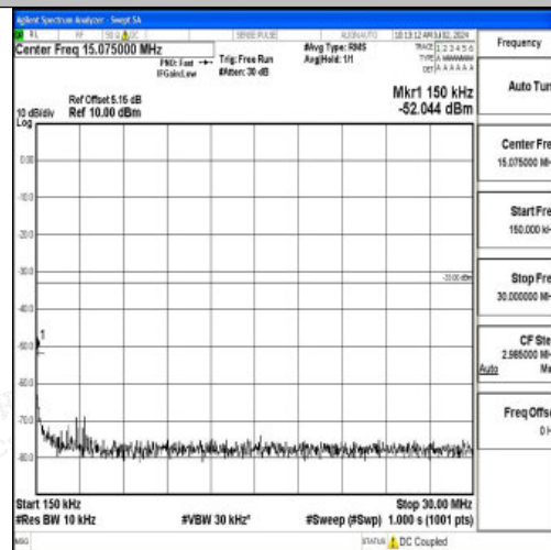
Band2_20MHz_QPSK_18700_1RB#0_0.15~30_0.15~30
