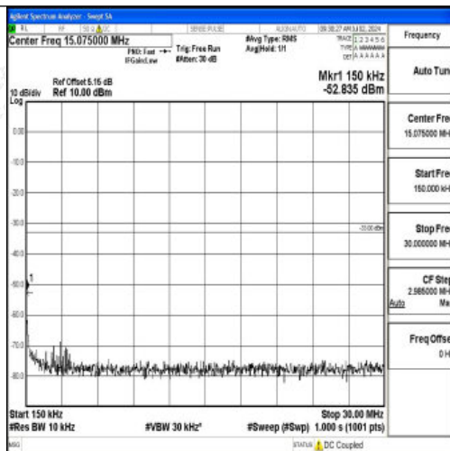
Band2_10MHz_16QAM_18650_1RB#0_0.15~30_0.15~30
