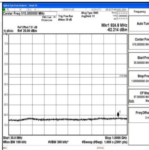
Band2_10MHz_16QAM_19150_1RB#0_30~1000_30~1000
