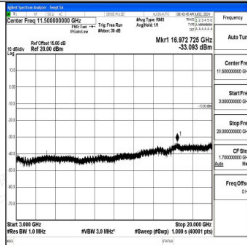
Band2_3MHz_16QAM_18900_1RB#0_3000~20000_3000~20000
