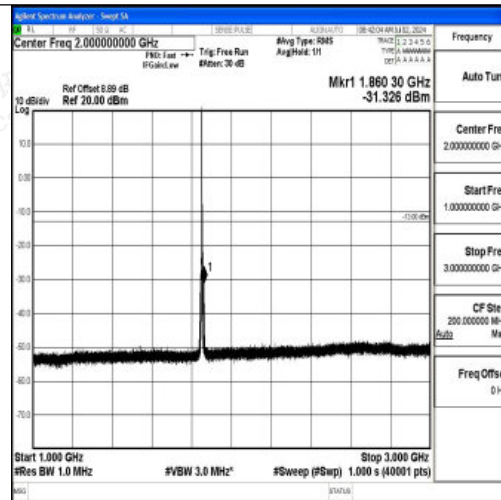
Band2_3MHz_QPSK_18615_1RB#0_1000~3000_1000~3000
