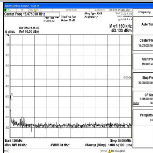
Band2_3MHz_QPSK_18900_1RB#0_0.15~30_0.15~30
