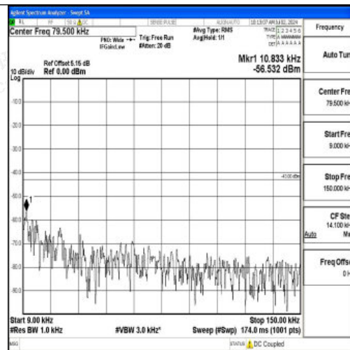
Band2_20MHz_QPSK_18700_1RB#0_0.009~0.15_0.009~0.15
