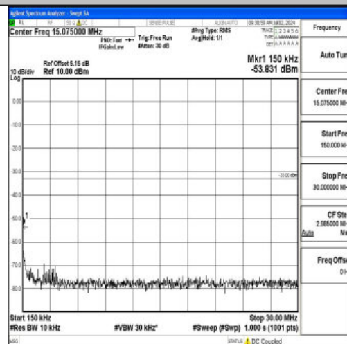
Band2_10MHz_QPSK_18900_1RB#0_0.15~30_0.15~30
