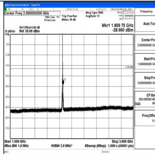
Band2_3MHz_16QAM_18615_1RB#0_1000~3000_1000~3000
