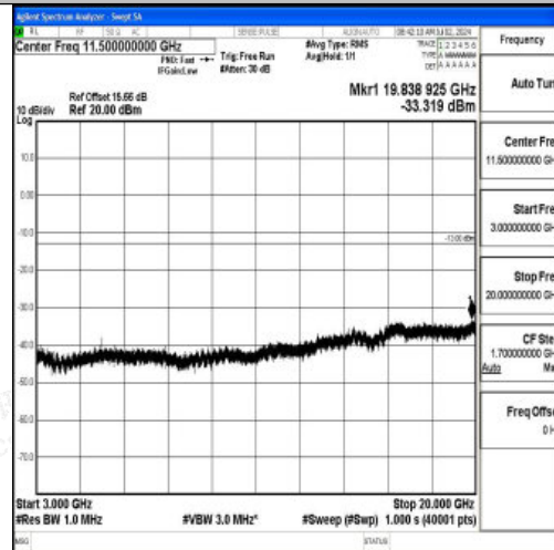
Band2_3MHz_QPSK_18615_1RB#0_3000~20000_3000~20000
