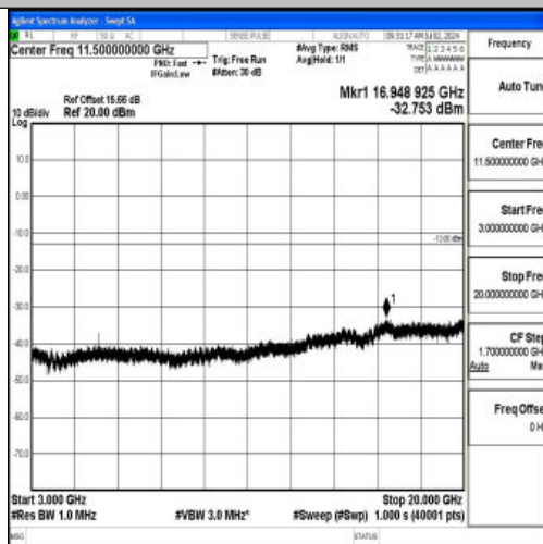
Band2_10MHz_QPSK_18900_1RB#0_3000~20000_3000~20000
