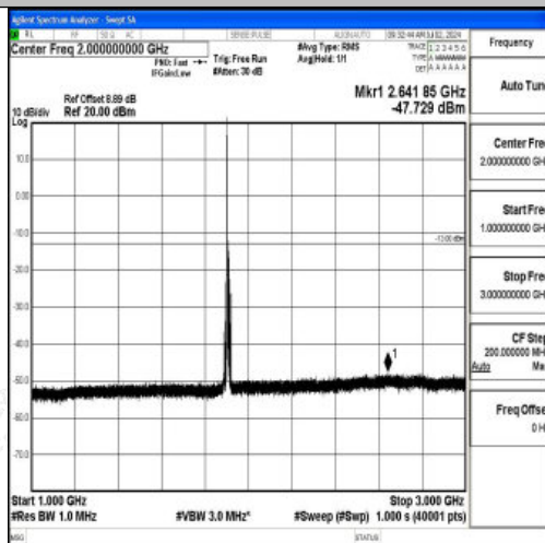
Band2_10MHz_16QAM_19150_1RB#0_1000~3000_1000~3000
