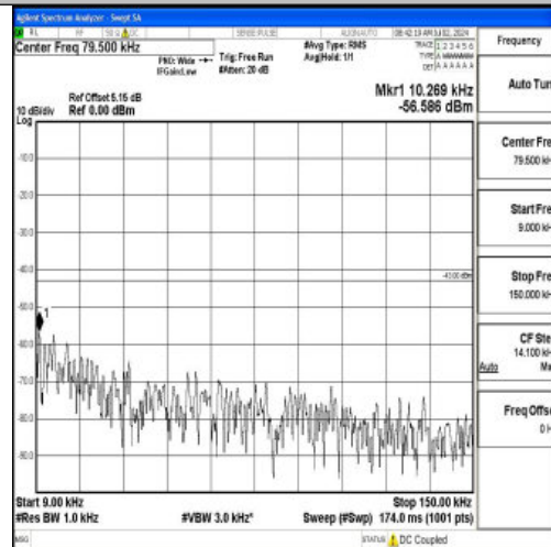
Band2_3MHz_16QAM_18615_1RB#0_0.009~0.15_0.009~0.15
