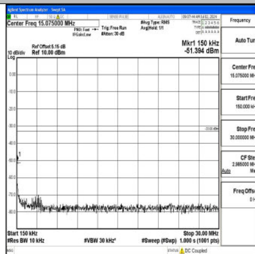
Band2_5MHz_QPSK_18900_1RB#0_0.15~30_0.15~30
