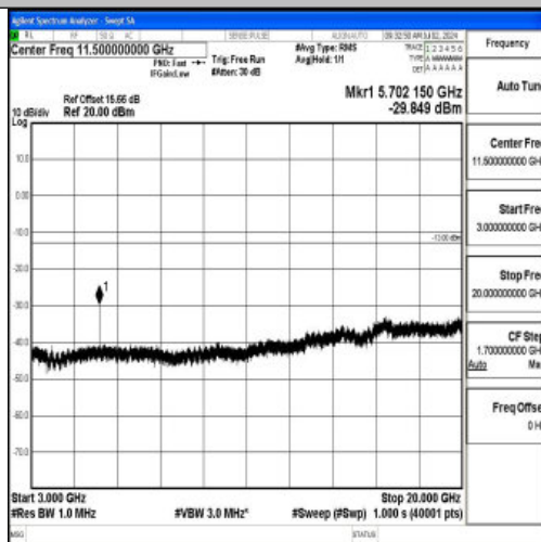
Band2_10MHz_16QAM_19150_1RB#0_3000~20000_3000~20000
