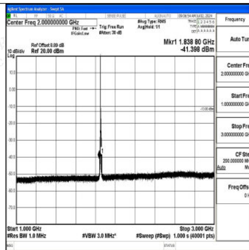
Band2_5MHz_QPSK_18625_1RB#0_1000~3000_1000~3000
