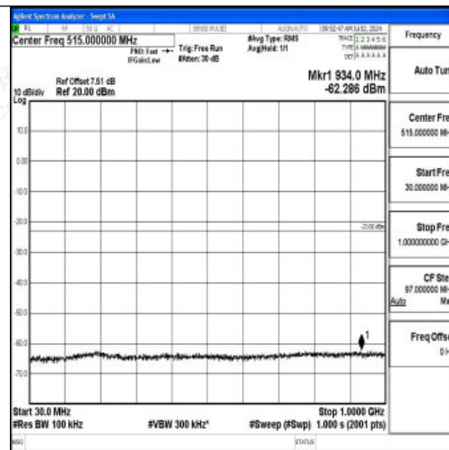
Band2_15MHz_QPSK_18900_1RB#0_30~1000_30~1000
