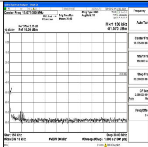
Band2_15MHz_QPSK_18900_1RB#0_0.15~30_0.15~30
