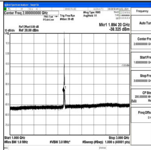
Band2_5MHz_QPSK_19175_1RB#0_1000~3000_1000~3000
