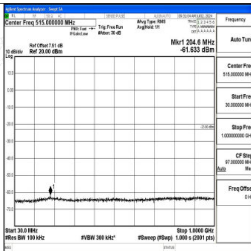
Band2_10MHz_QPSK_18900_1RB#0_30~1000_30~1000
