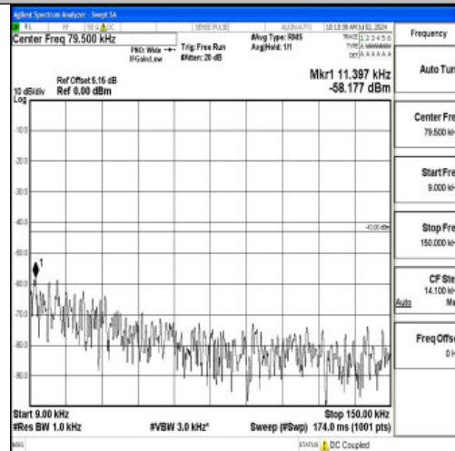
Band2_20MHz_16QAM_18700_1RB#0_0.009~0.15_0.009~0.15
