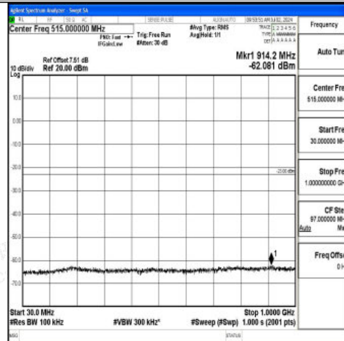
Band2_15MHz_QPSK_19125_1RB#0_30~1000_30~1000
