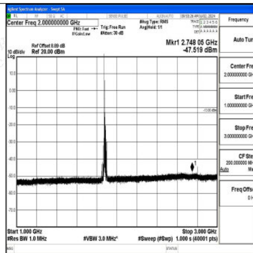
Band2_15MHz_16QAM_18900_1RB#0_1000~3000_1000~3000
