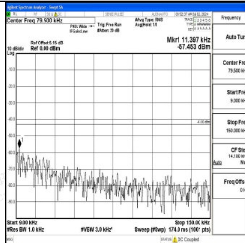
Band2_15MHz_QPSK_18900_1RB#0_0.009~0.15_0.009~0.15
