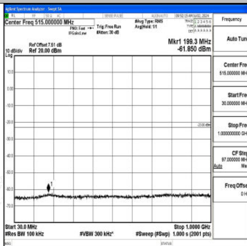
Band2_15MHz_16QAM_18675_1RB#0_30~1000_30~1000
