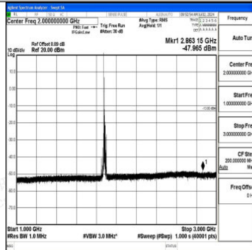
Band2_15MHz_QPSK_18900_1RB#0_1000~3000_1000~3000
