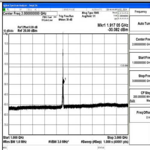
Band2_3MHz_16QAM_19185_1RB#0_1000~3000_1000~3000
