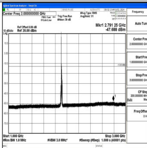
Band2_10MHz_QPSK_19150_1RB#0_1000~3000_1000~3000
