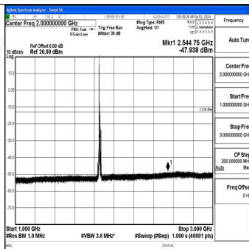
Band2_10MHz_QPSK_18650_1RB#0_1000~3000_1000~3000
