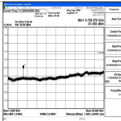
Band2_1.4MHz_QPSK_19193_1RB#0_3000~20000_3000~20000
