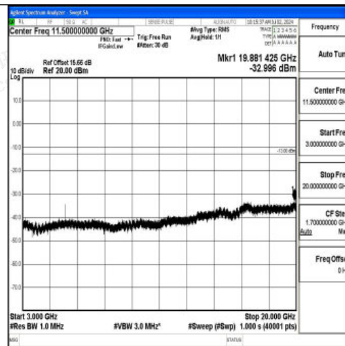
Band2_20MHz_QPSK_19100_1RB#0_3000~20000_3000~20000
