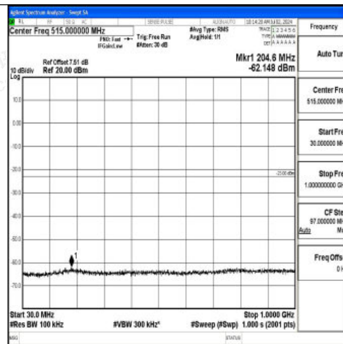
Band2_20MHz_QPSK_18900_1RB#0_30~1000_30~1000
