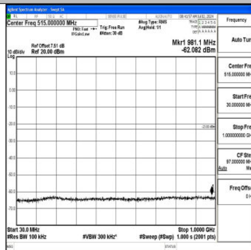
Band2_3MHz_QPSK_18615_1RB#0_30~1000_30~1000
