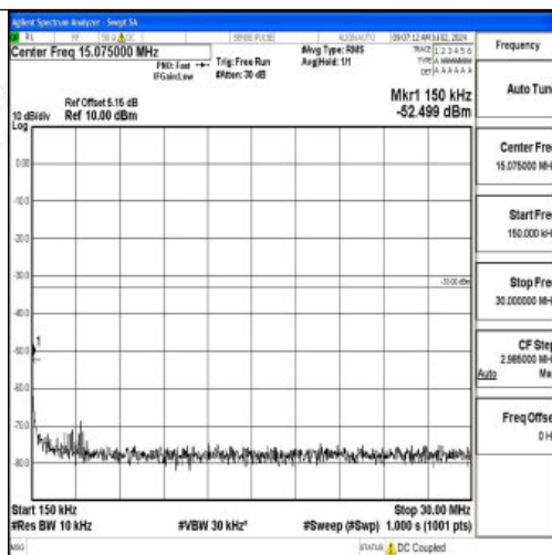
Band2_5MHz_16QAM_18625_1RB#0_0.15~30_0.15~30
