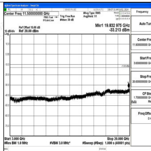
Band2_5MHz_16QAM_18625_1RB#0_3000~20000_3000~20000
