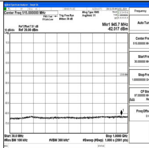
Band2_10MHz_16QAM_18900_1RB#0_30~1000_30~1000
