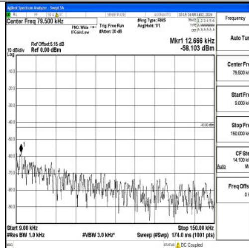
Band2_20MHz_QPSK_19100_1RB#0_0.009~0.15_0.009~0.15
