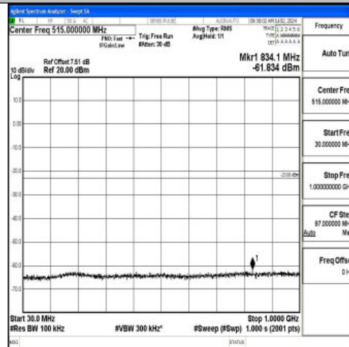
Band2_10MHz_QPSK_18650_1RB#0_30~1000_30~1000
