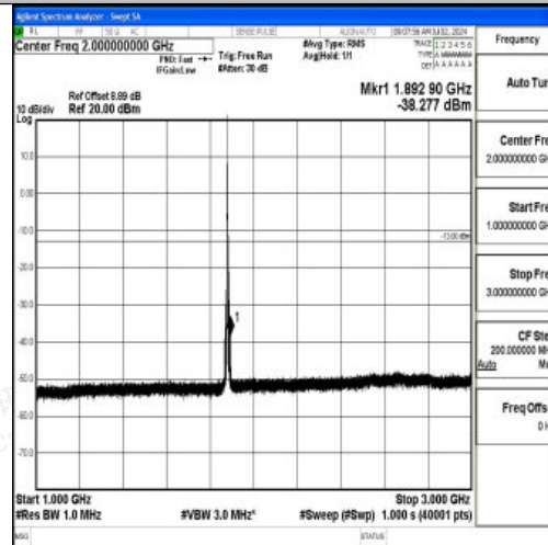
Band2_5MHz_QPSK_18900_1RB#0_1000~3000_1000~3000
