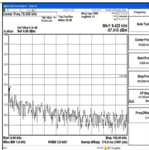
Band2_5MHz_16QAM_18900_1RB#0_0.009~0.15_0.009~0.15
