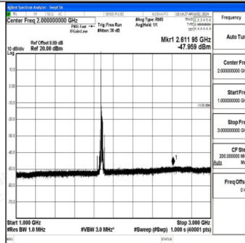
Band2_20MHz_QPSK_18900_1RB#0_1000~3000_1000~3000
