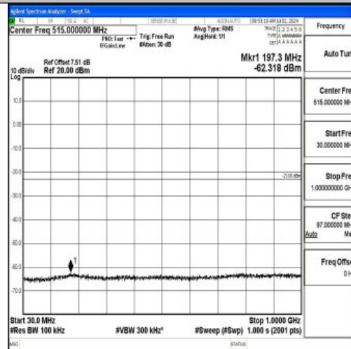
Band2_15MHz_16QAM_18900_1RB#0_30~1000_30~1000
