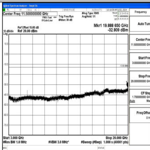
Band2_20MHz_16QAM_19100_1RB#0_3000~20000_3000~20000
