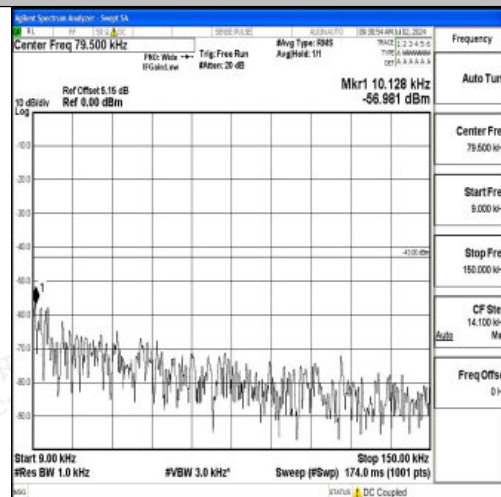
Band2_10MHz_QPSK_18900_1RB#0_0.009~0.15_0.009~0.15
