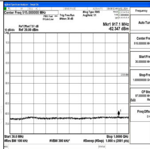
Band2_5MHz_QPSK_19175_1RB#0_30~1000_30~1000
