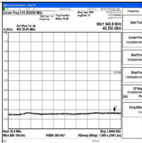
Band2_3MHz_16QAM_19185_1RB#0_30~1000_30~1000
