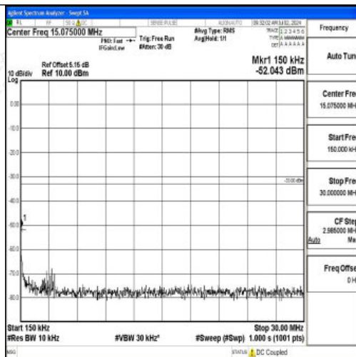
Band2_10MHz_QPSK_19150_1RB#0_0.15~30_0.15~30
