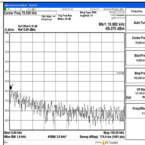
Band2_20MHz_16QAM_18900_1RB#0_0.009~0.15_0.009~0.15
