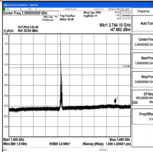
Band2_15MHz_16QAM_18675_1RB#0_1000~3000_1000~3000
