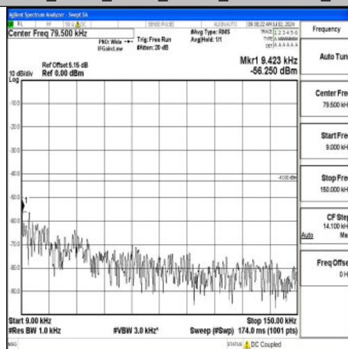
Band2_10MHz_16QAM_18650_1RB#0_0.009~0.15_0.009~0.15
