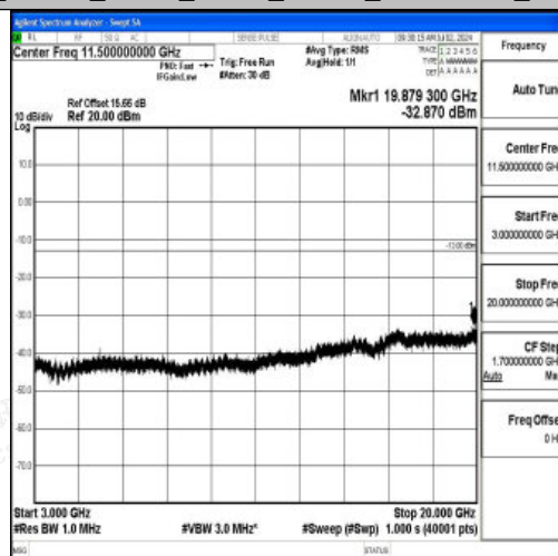
Band2_10MHz_QPSK_18650_1RB#0_3000~20000_3000~20000
