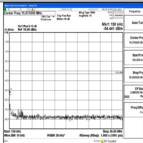
Band2_10MHz_16QAM_19150_1RB#0_0.15~30_0.15~30
