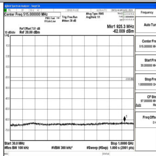
Band2_15MHz_QPSK_18675_1RB#0_30~1000_30~1000
