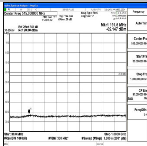
Band2_20MHz_16QAM_18900_1RB#0_30~1000_30~1000
