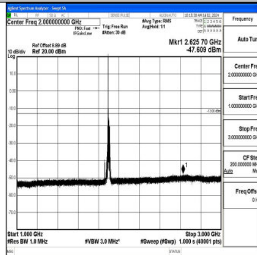
Band2_20MHz_QPSK_19100_1RB#0_1000~3000_1000~3000
