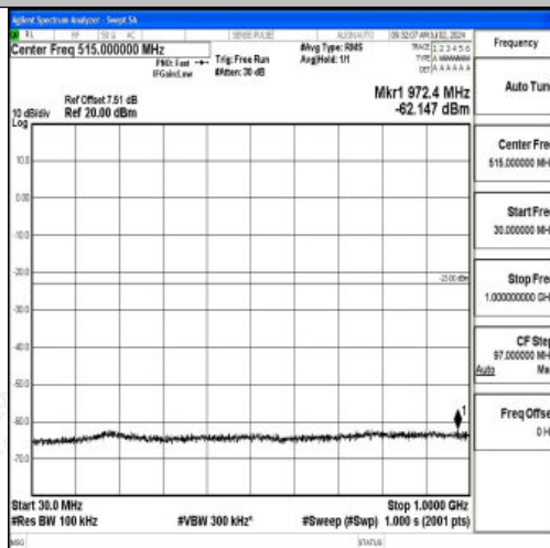
Band2_10MHz_QPSK_19150_1RB#0_30~1000_30~1000
