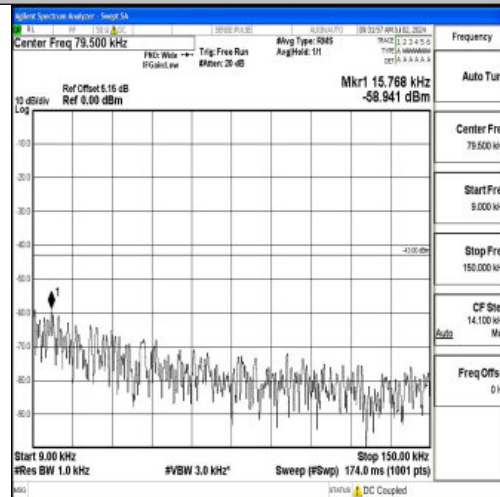
Band2_10MHz_QPSK_19150_1RB#0_0.009~0.15_0.009~0.15
