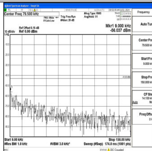
Band2_15MHz_16QAM_18675_1RB#0_0.009~0.15_0.009~0.15
