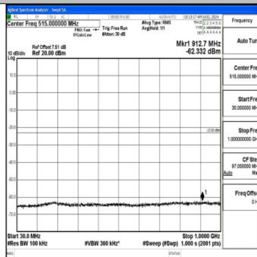
Band2_20MHz_QPSK_18700_1RB#0_30~1000_30~1000
