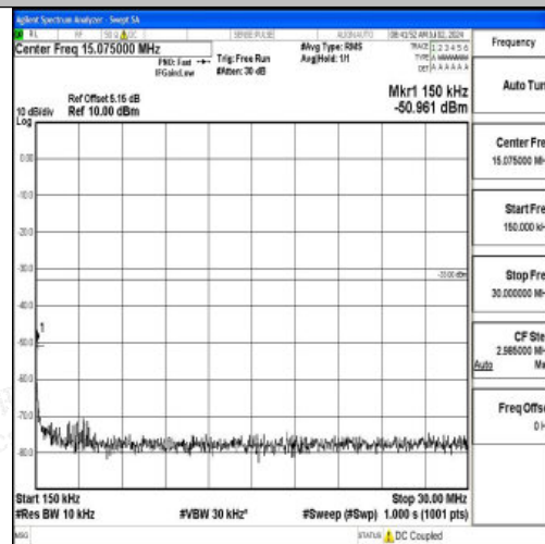
Band2_3MHz_QPSK_18615_1RB#0_0.15~30_0.15~30
