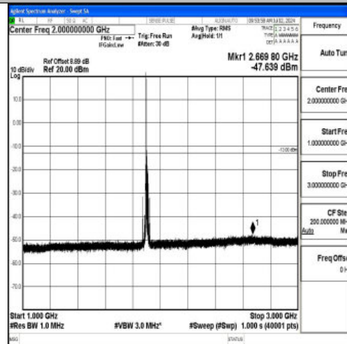
Band2_15MHz_QPSK_19125_1RB#0_1000~3000_1000~3000
