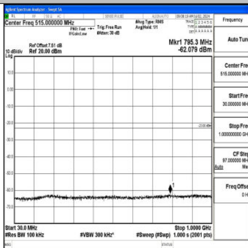
Band2_5MHz_16QAM_18900_1RB#0_30~1000_30~1000
