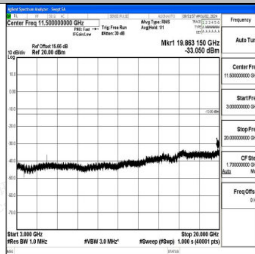
Band2_15MHz_QPSK_18675_1RB#0_3000~20000_3000~20000
