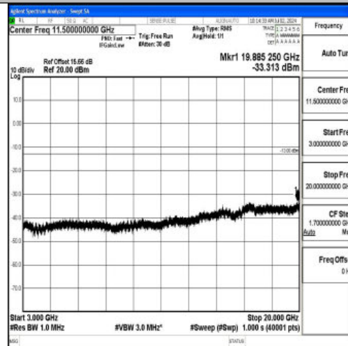
Band2_20MHz_QPSK_18900_1RB#0_3000~20000_3000~20000
