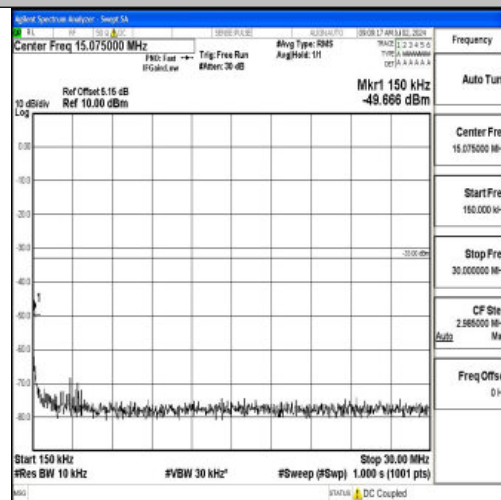
Band2_5MHz_16QAM_19175_1RB#0_0.15~30_0.15~30
