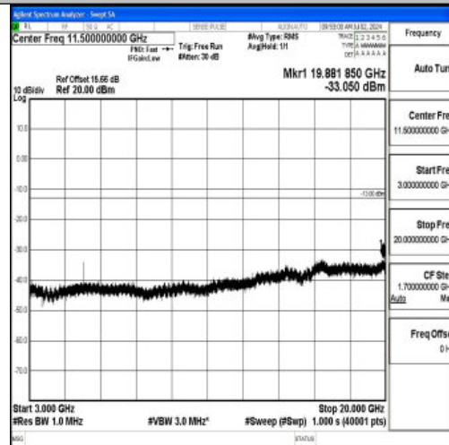
Band2_15MHz_QPSK_18900_1RB#0_3000~20000_3000~20000
