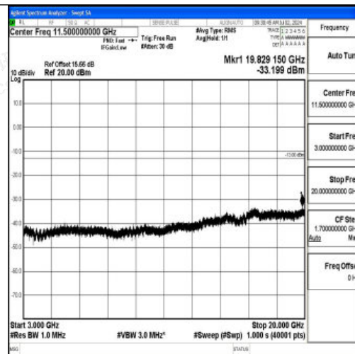
Band2_10MHz_16QAM_18650_1RB#0_3000~20000_3000~20000
