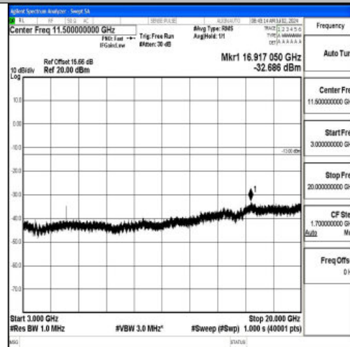
Band2_3MHz_QPSK_18900_1RB#0_3000~20000_3000~20000
