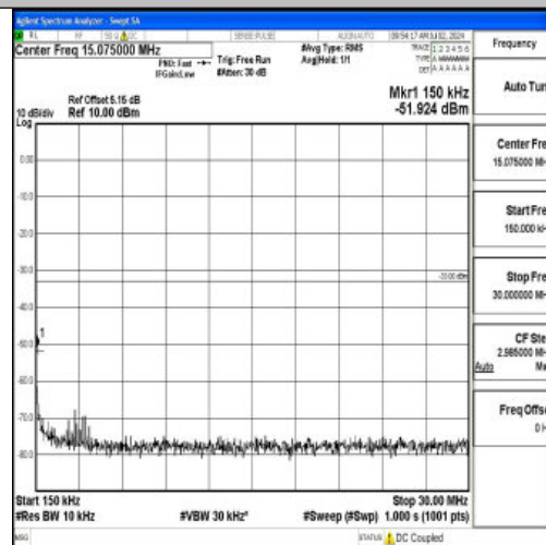
Band2_15MHz_16QAM_19125_1RB#0_0.15~30_0.15~30
