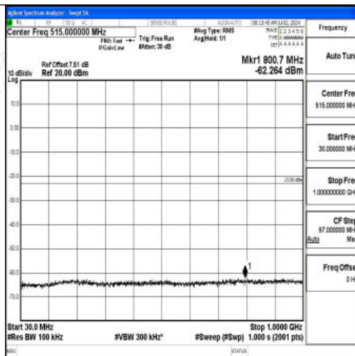
Band2_1.4MHz_16QAM_19193_1RB#0_30~1000_30~1000
