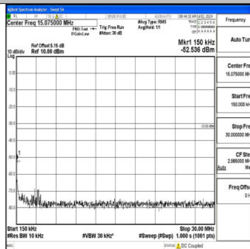
Band2_3MHz_16QAM_19185_1RB#0_0.15~30_0.15~30
