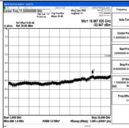
Band2_5MHz_16QAM_19175_1RB#0_3000~20000_3000~20000
