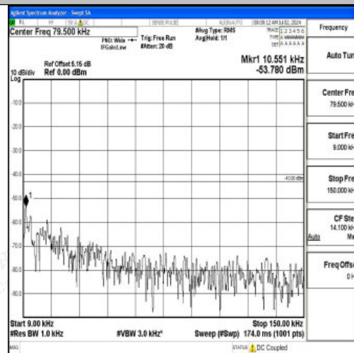
Band2_5MHz_16QAM_19175_1RB#0_0.009~0.15_0.009~0.15
