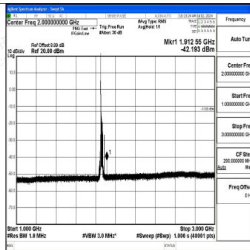
Band2_20MHz_QPSK_18700_1RB#0_1000~3000_1000~3000
