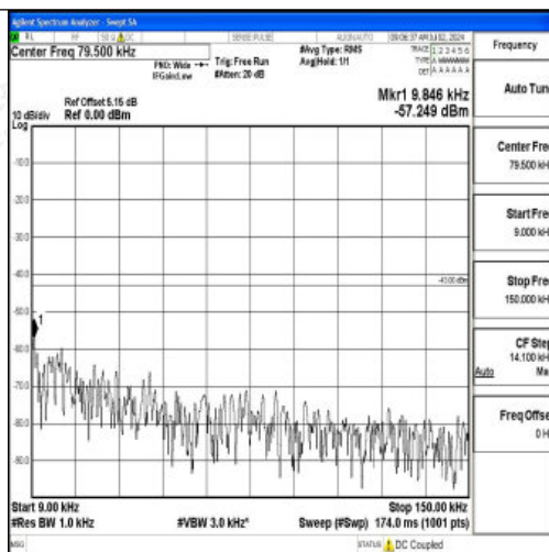
Band2_5MHz_QPSK_18625_1RB#0_0.009~0.15_0.009~0.15
