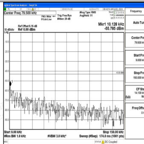
Band2_3MHz_QPSK_18900_1RB#0_0.009~0.15_0.009~0.15
