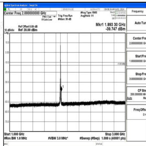
Band2_5MHz_16QAM_18900_1RB#0_1000~3000_1000~3000
