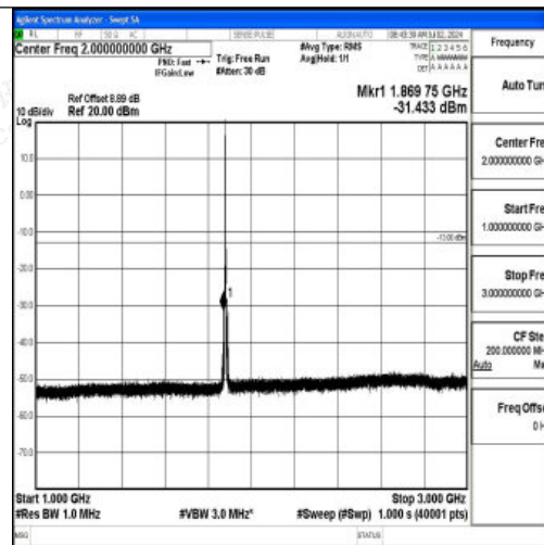
Band2_3MHz_16QAM_18900_1RB#0_1000~3000_1000~3000
