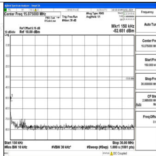
Band2_20MHz_QPSK_19100_1RB#0_0.15~30_0.15~30
