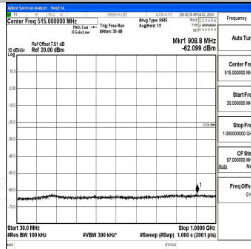
Band2_3MHz_16QAM_18615_1RB#0_30~1000_30~1000
