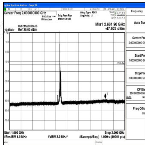
Band2_20MHz_16QAM_18900_1RB#0_1000~3000_1000~3000
