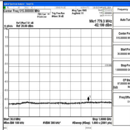
Band2_20MHz_QPSK_19100_1RB#0_30~1000_30~1000
