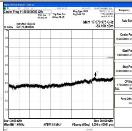
Band2_5MHz_16QAM_18900_1RB#0_3000~20000_3000~20000
