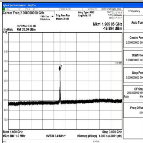
Band2_1.4MHz_16QAM_19193_1RB#0_1000~3000_1000~3000
