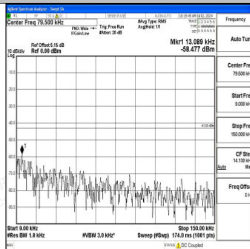
Band2_20MHz_16QAM_19100_1RB#0_0.009~0.15_0.009~0.15
