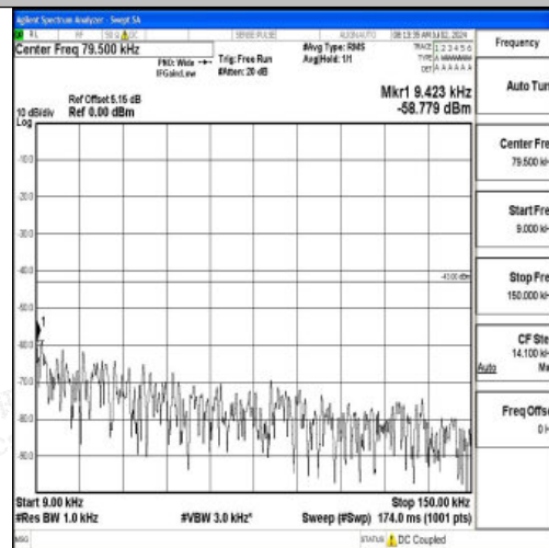
Band2_1.4MHz_16QAM_19193_1RB#0_0.009~0.15_0.009~0.15
