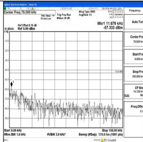
Band2_3MHz_QPSK_19185_1RB#0_0.009~0.15_0.009~0.15
