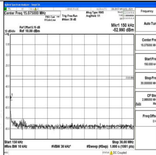
Band2_10MHz_QPSK_18650_1RB#0_0.15~30_0.15~30
