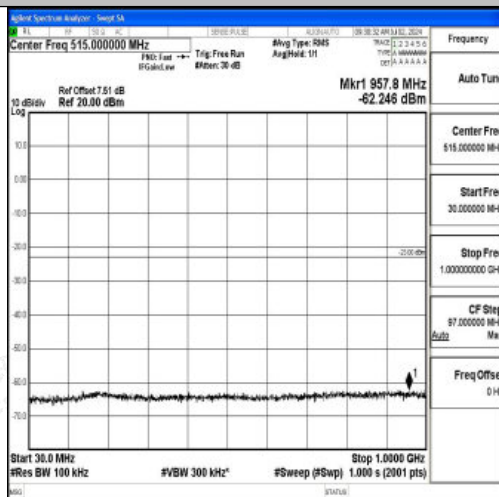
Band2_10MHz_16QAM_18650_1RB#0_30~1000_30~1000
