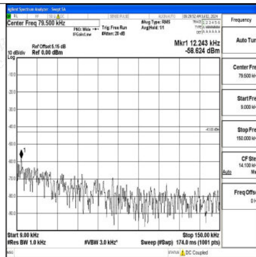
Band2_10MHz_QPSK_18650_1RB#0_0.009~0.15_0.009~0.15
