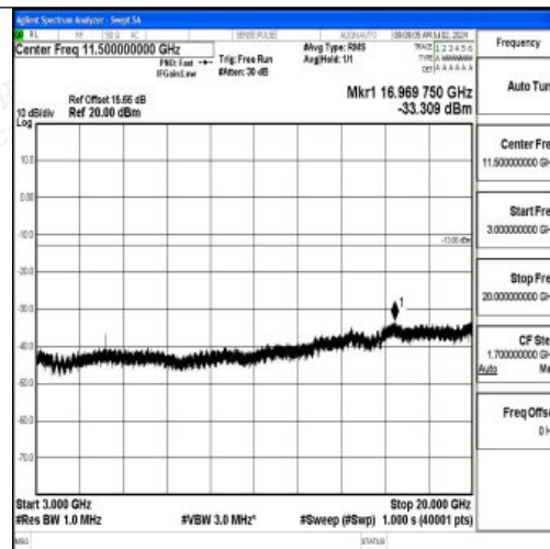
Band2_5MHz_QPSK_19175_1RB#0_3000~20000_3000~20000
