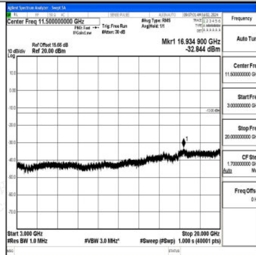
Band2_5MHz_QPSK_18625_1RB#0_3000~20000_3000~20000
