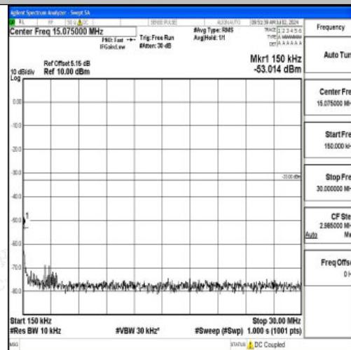
Band2_15MHz_QPSK_18675_1RB#0_0.15~30_0.15~30
