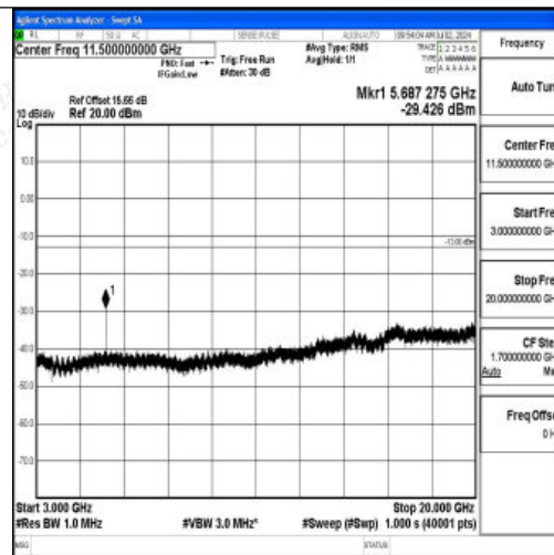
Band2_15MHz_QPSK_19125_1RB#0_3000~20000_3000~20000
