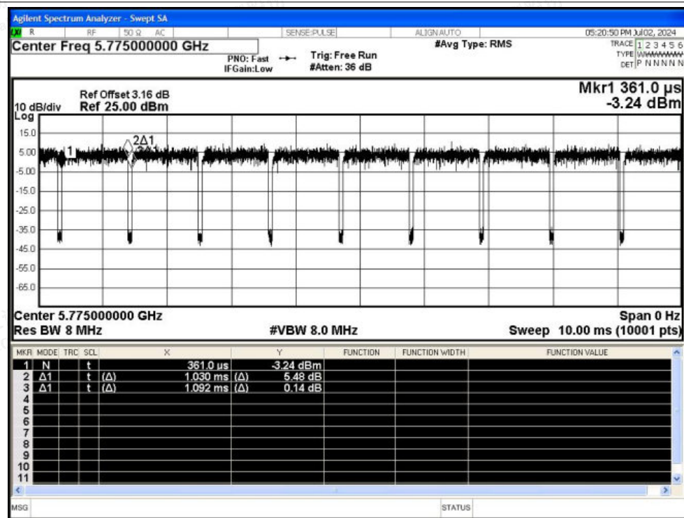
Duty Cycle HVHT ac80 5775MHz Ant1
