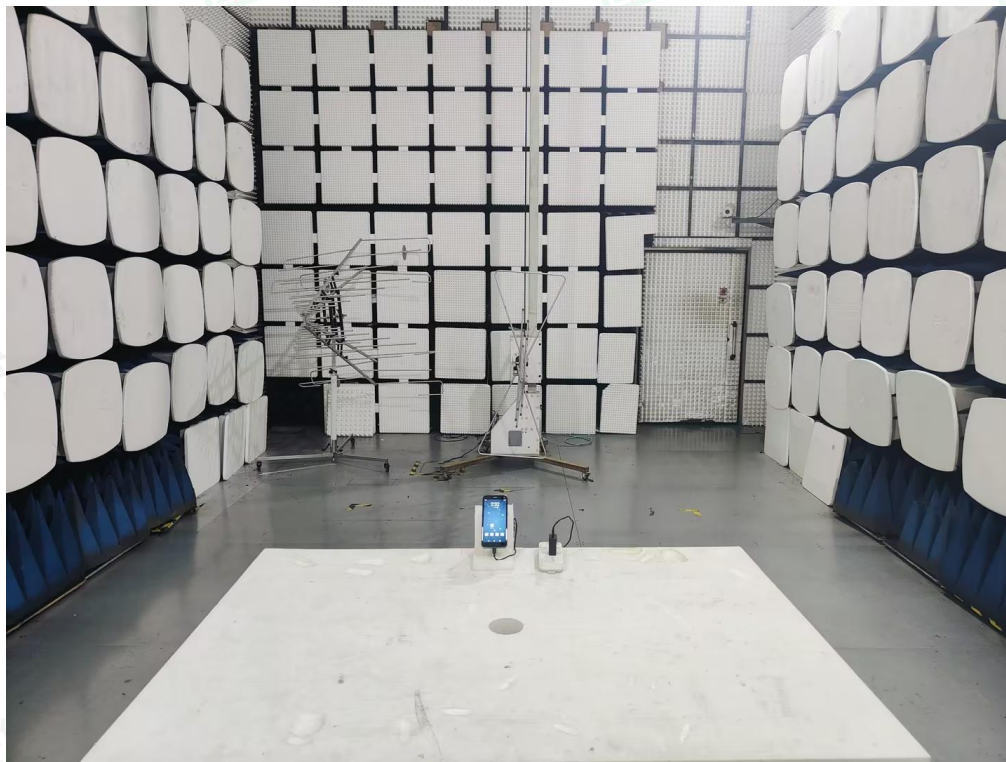
Fig. 2 (30 MHz – 1 GHz)
