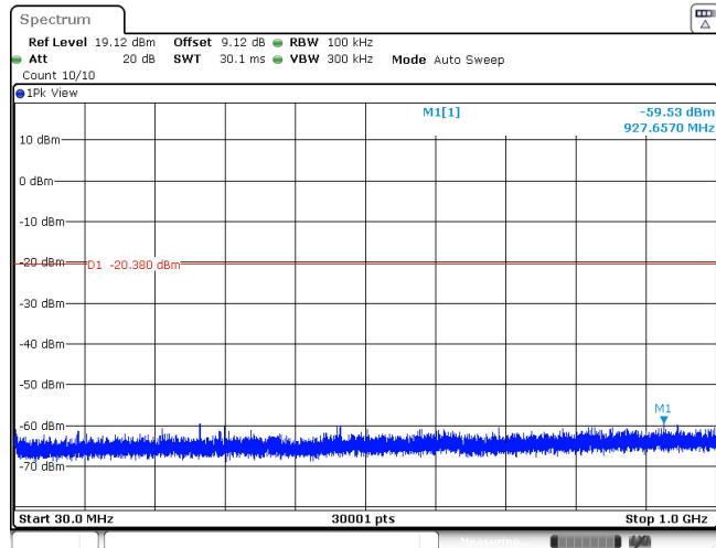
11AX20SISO_Ant1_2462_52Tone_RU39_30~1000
