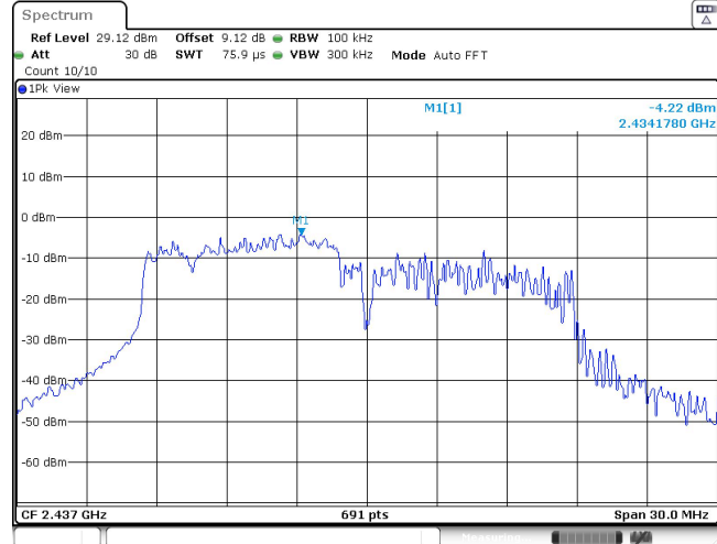
11AX20SISO_Ant1_2437_106Tone_RU53_0~Reference
