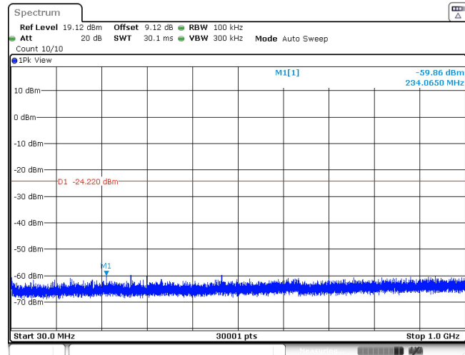
11AX20SISO_Ant1_2437_106Tone_RU53_30~1000
