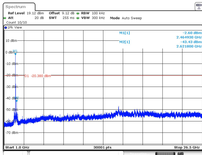
11AX20SISO_Ant1_2462_52Tone_RU39_1000~26500
