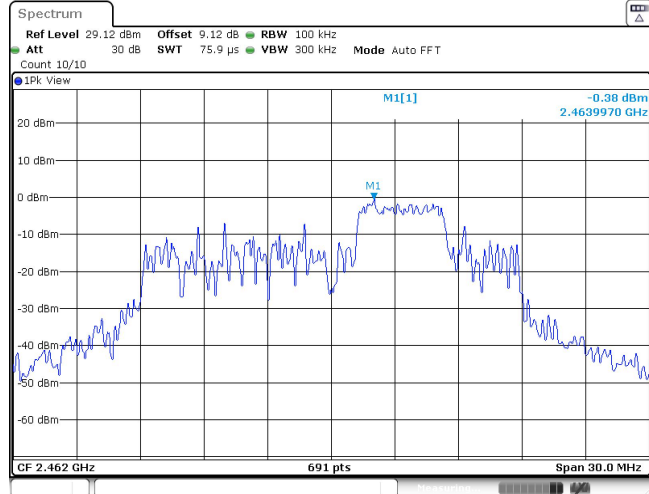
11AX20SISO_Ant1_2462_52Tone_RU39_0~Reference
