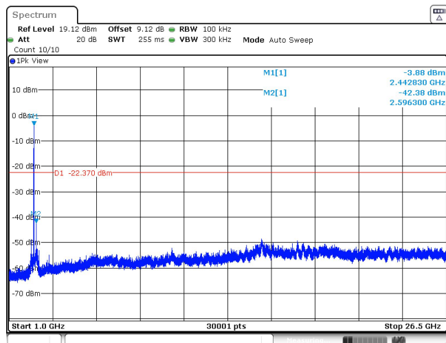
11AX20SISO_Ant1_2437_52Tone_RU40_1000~26500
