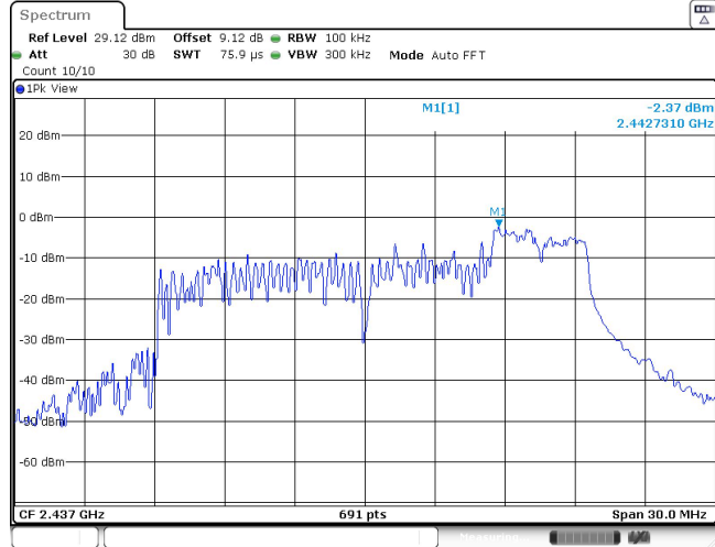
11AX20SISO_Ant1_2437_52Tone_RU40_0~Reference
