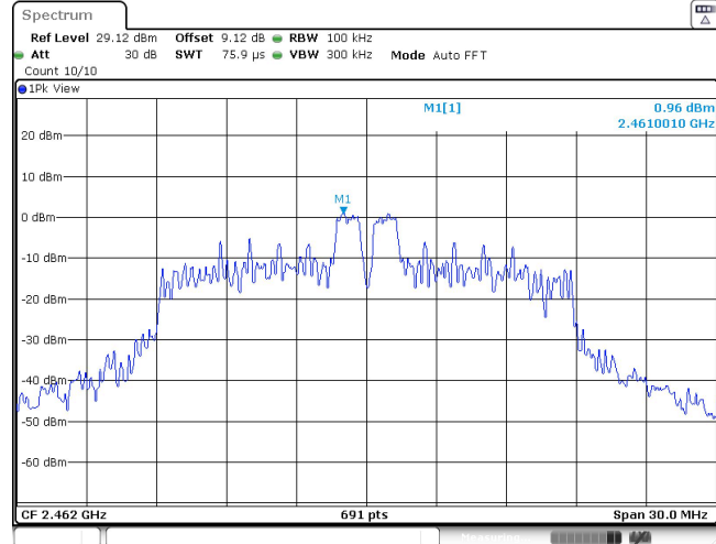
11AX20SISO_Ant1_2462_26Tone_RU4_0~Reference
