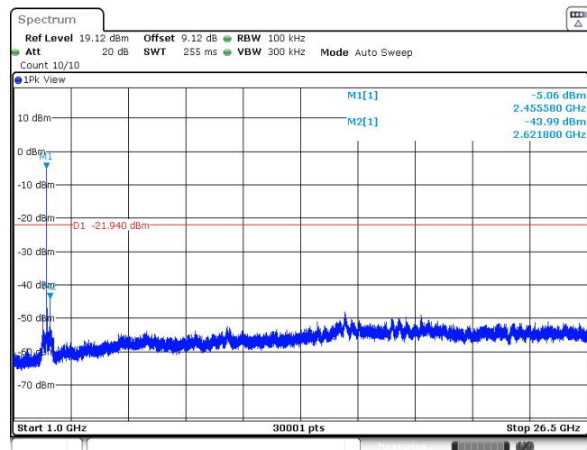
11AX20SISO_Ant1_2462_52Tone_RU37_1000~26500
