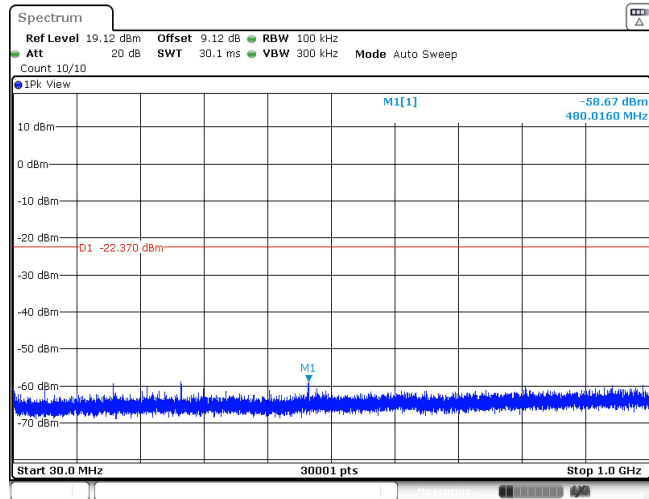
11AX20SISO_Ant1_2437_52Tone_RU40_30~1000
