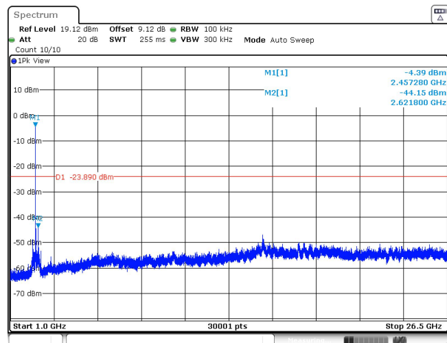
11AX20SISO_Ant1_2462_106Tone_RU53_1000~26500
