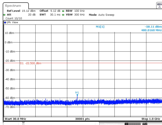
11AX20SISO_Ant1_2462_52Tone_RU40_0~Reference
