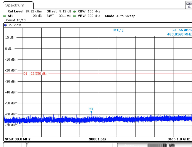
11AX20SISO_Ant1_2437_52Tone_RU37_30~1000
