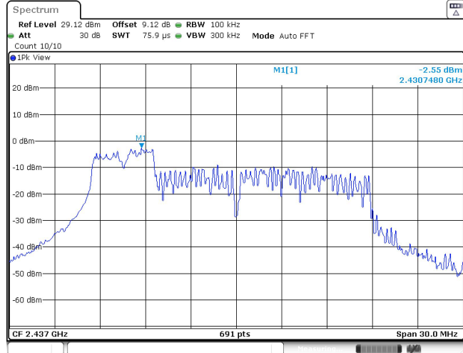
11AX20SISO_Ant1_2437_52Tone_RU37_0~Reference
