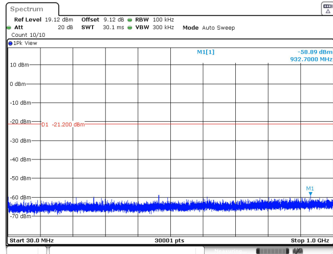
11AX20SISO_Ant1_2437_26Tone_RU8_30~1000
