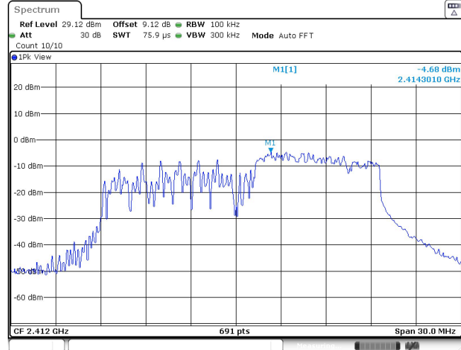
11AX20SISO_Ant1_2412_106Tone_RU54_0~Reference
