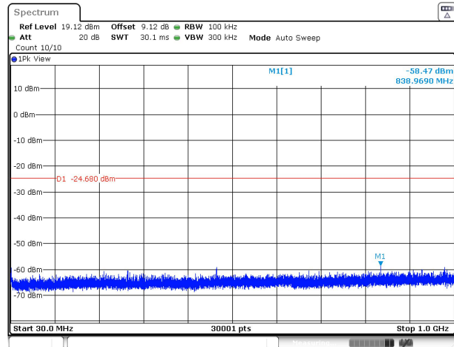
11AX20SISO_Ant1_2412_106Tone_RU54_30~1000
