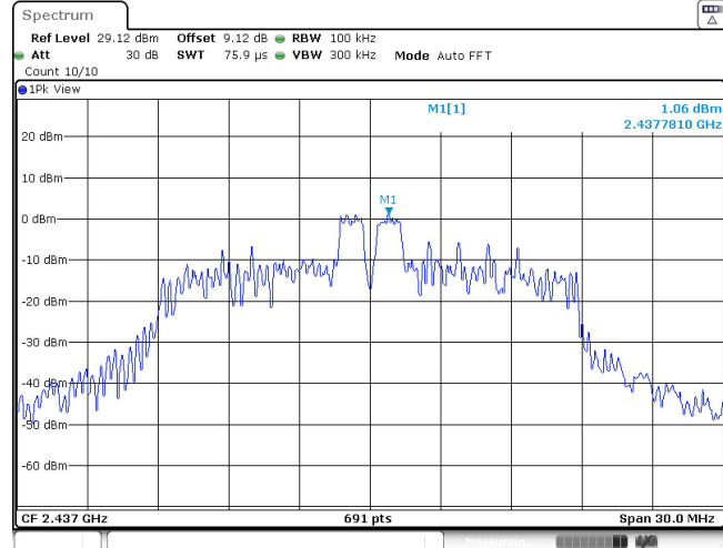
11AX20SISO_Ant1_2437_26Tone_RU4_0~Reference
