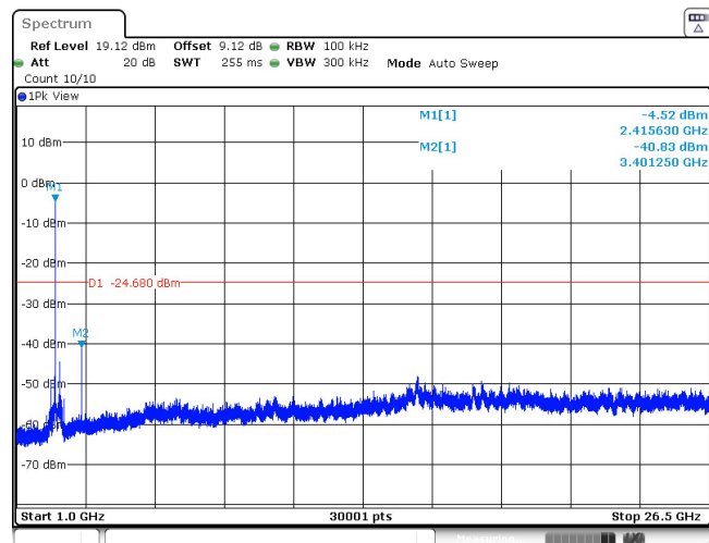
11AX20SISO_Ant1_2412_106Tone_RU54_1000~26500
