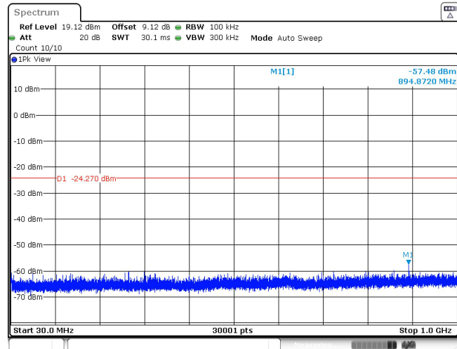
11AX20SISO_Ant1_2412_106Tone_RU53_30~1000
