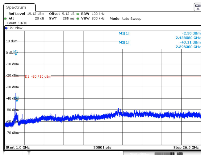
11AX20SISO_Ant1_2437_52Tone_RU39_1000~26500
