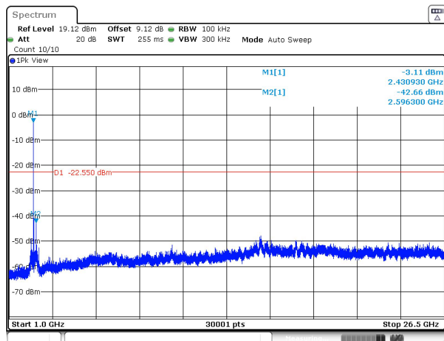
11AX20SISO_Ant1_2437_52Tone_RU37_1000~26500
