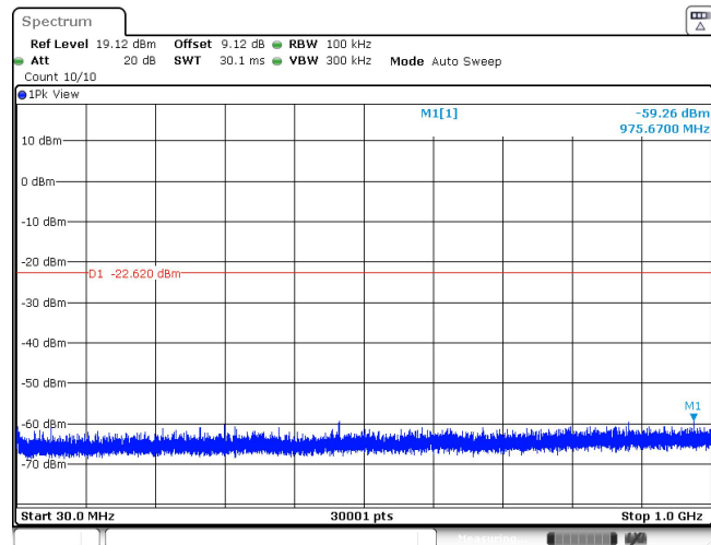
11AX20SISO_Ant1_2412_52Tone_RU40_30~1000
