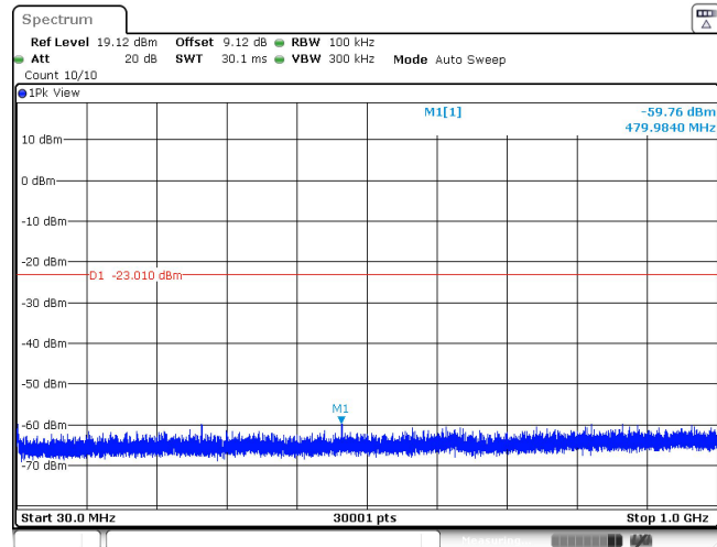
11AX20SISO_Ant1_2412_52Tone_RU37_30~1000
