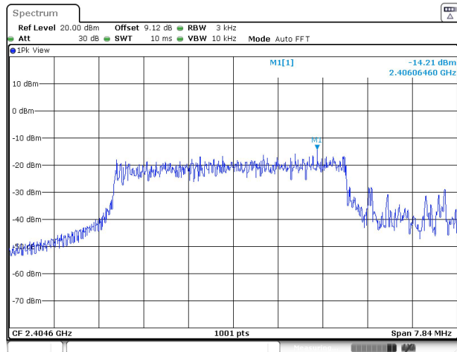
11AX20SISO_Ant1_2412_52Tone_RU37
