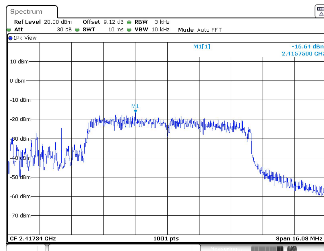
11AX20SISO_Ant1_2412_106Tone_RU53
