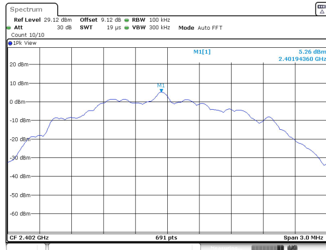
BLE_2M_Ant1_2402_0~Reference
