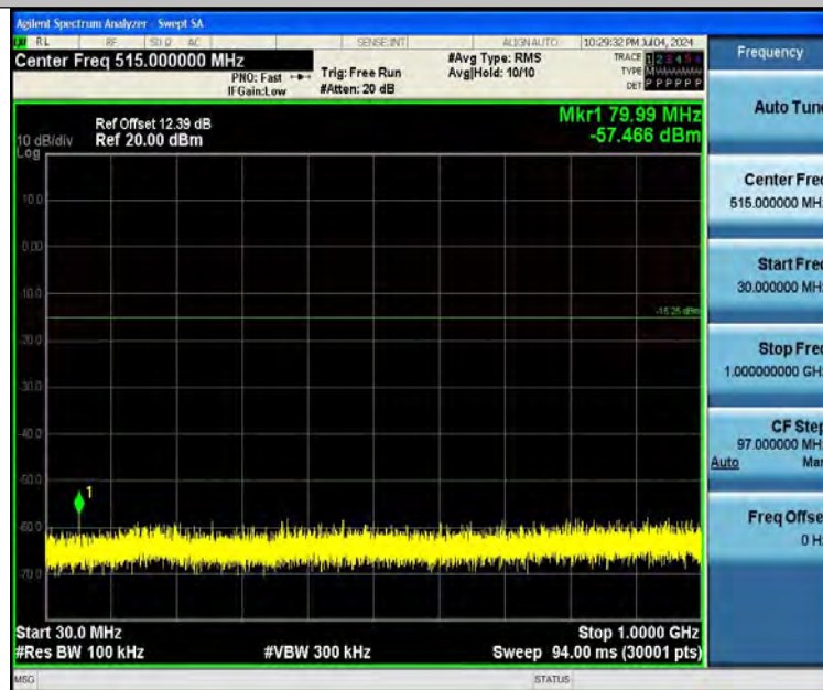
BLE_1M-Ant1-2402-30~1000-PASS
