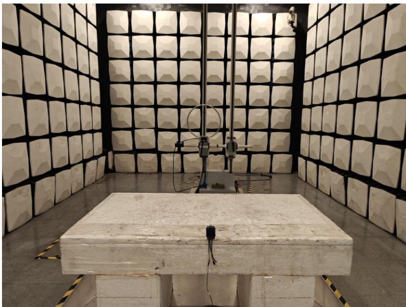
Radiated Emission View (9kHz-30MHz)
