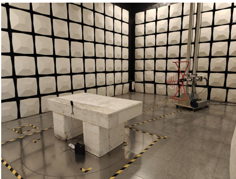
Radiated Emission View (30MHz-1GHz)
