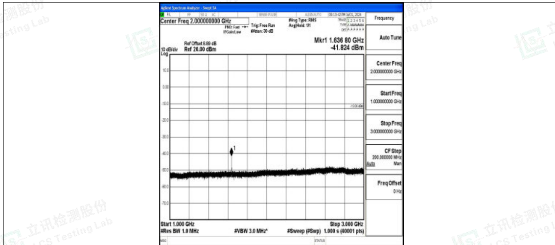
Band26_1.4MHz_QPSK_26740_1RB#0_1000~3000_1000~3000
