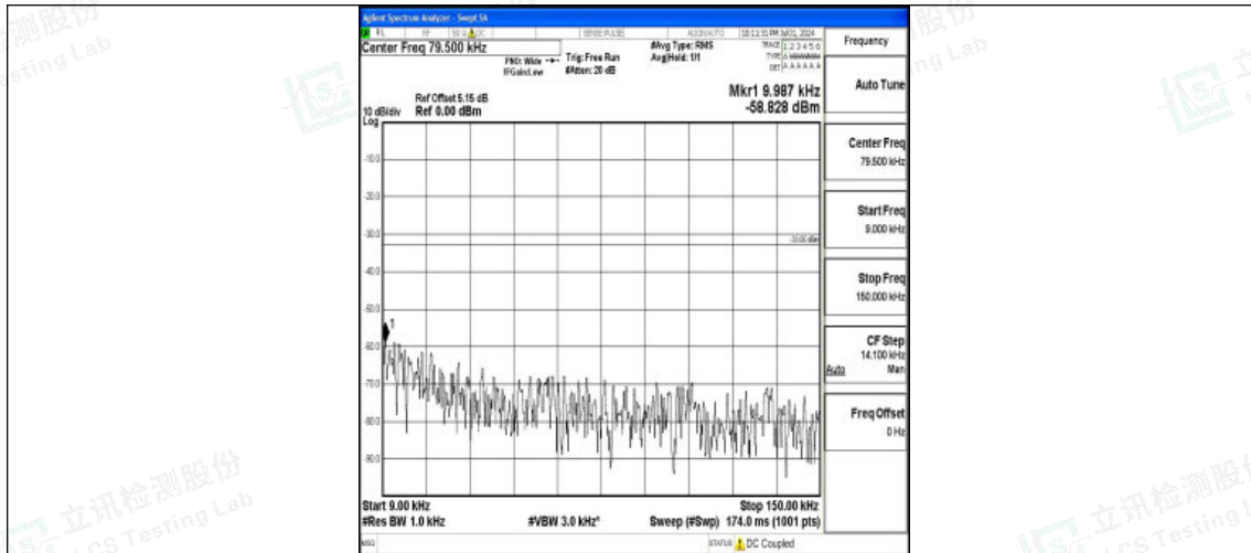
Band26_5MHz_16QAM_26765_1RB#0_0.009~0.15_0.009~0.15
