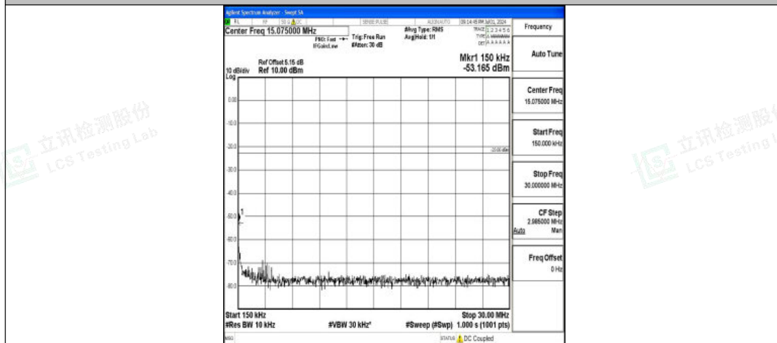
Band26_1.4MHz_QPSK_26783_1RB#0_0.15~30_0.15~30
