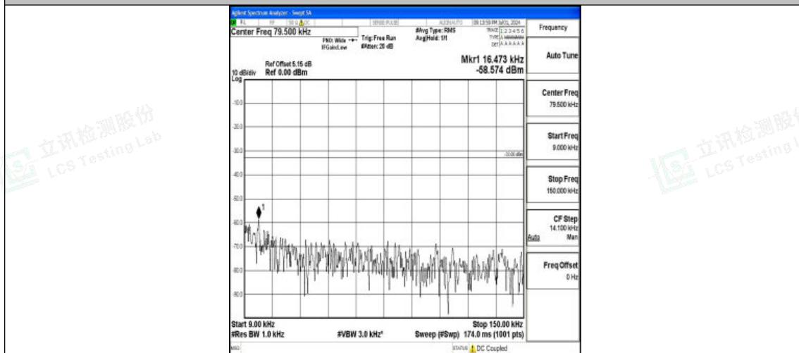
Band26_1.4MHz_16QAM_26740_1RB#0_0.009~0.15_0.009~0.15
