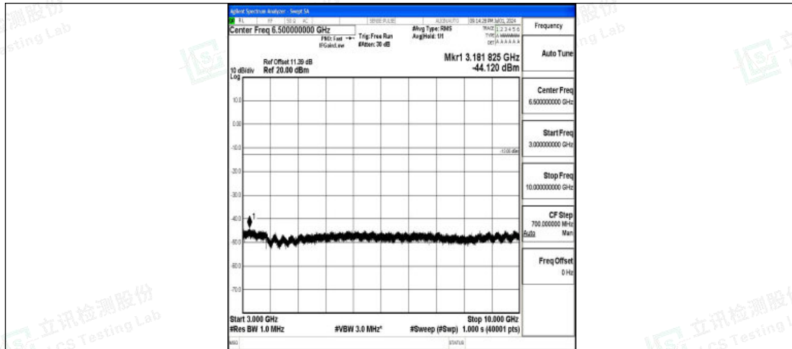
Band26_1.4MHz_16QAM_26740_1RB#0_3000~10000_3000~10000
