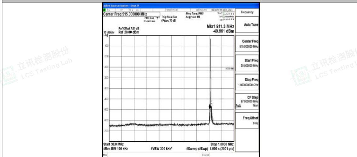
Band26_3MHz_QPSK_26740_1RB#0_30~1000_30~1000
