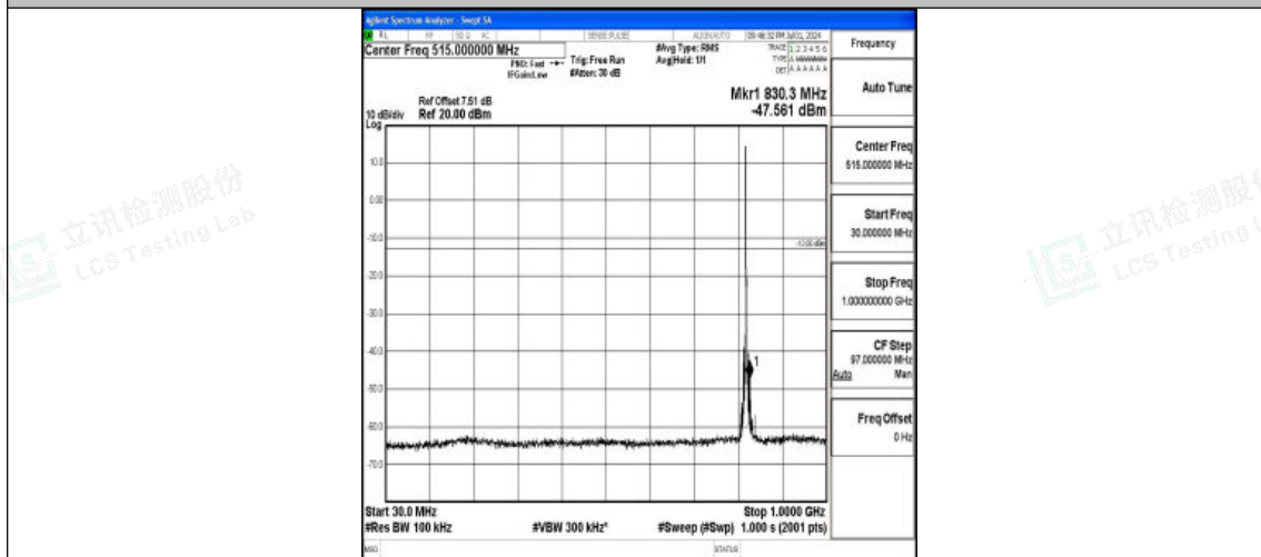
Band26_3MHz_16QAM_26775_1RB#0_30~1000_30~1000
