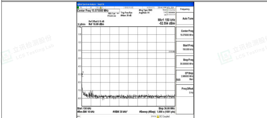
Band26_3MHz_16QAM_26705_1RB#0_0.15~30_0.15~30
