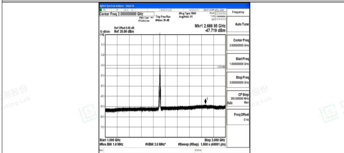
Band25_10MHz_QPSK_26640_1RB#0_1000~3000_1000~3000
