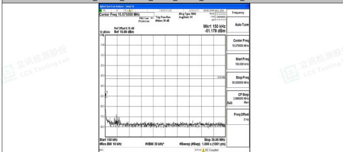
Band25_20MHz_16QAM_26140_1RB#0_0.15~30_0.15~30
