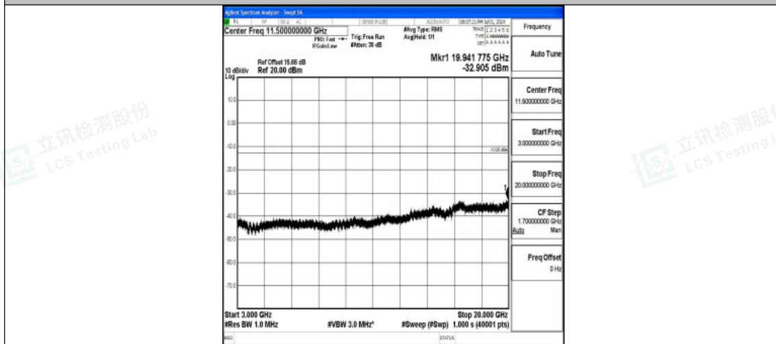
Band25_10MHz_QPSK_26640_1RB#0_3000~20000_3000~20000
