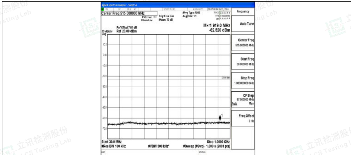
Band25_10MHz_QPSK_26640_1RB#0_30~1000_30~1000
