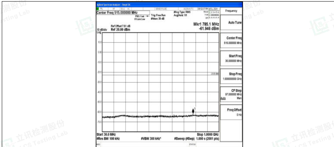
Band25_20MHz_QPSK_26590_1RB#0_30~1000_30~1000
