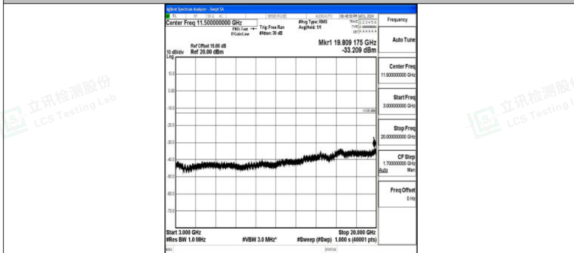
Band25_1.4MHz_16QAM_26047_1RB#0_3000~20000_3000~20000
