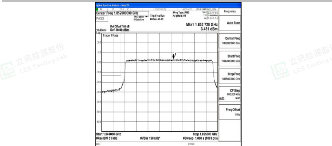
Band25_5MHz_QPSK_26065_25RB#0
