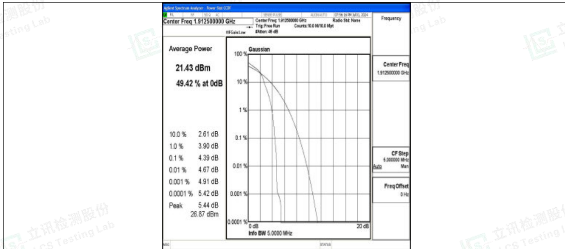
Band25-5MHz-16QAM-26665-1RB#0-PASS
