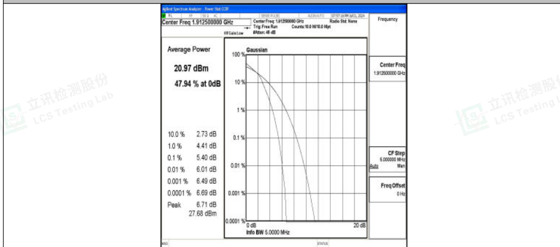
Band25-5MHz-16QAM-26665-25RB#0-PASS
