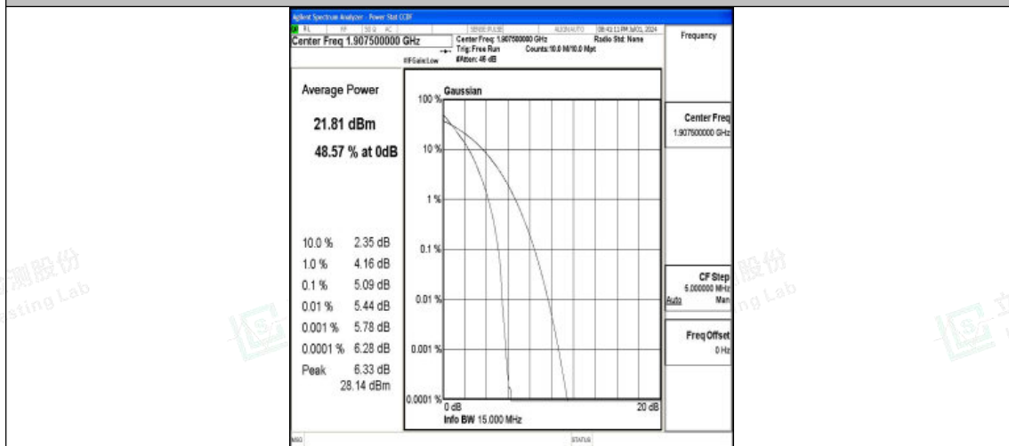
Band25-15MHz-QPSK-26615-75RB#0-PASS
