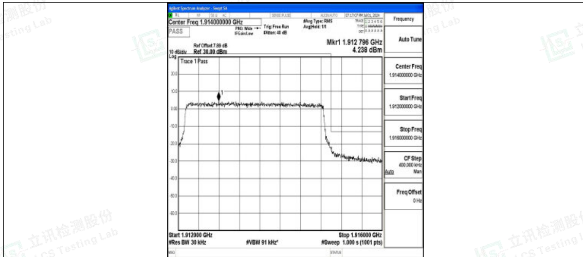
Band25_3MHz_QPSK_26675_15RB#0
