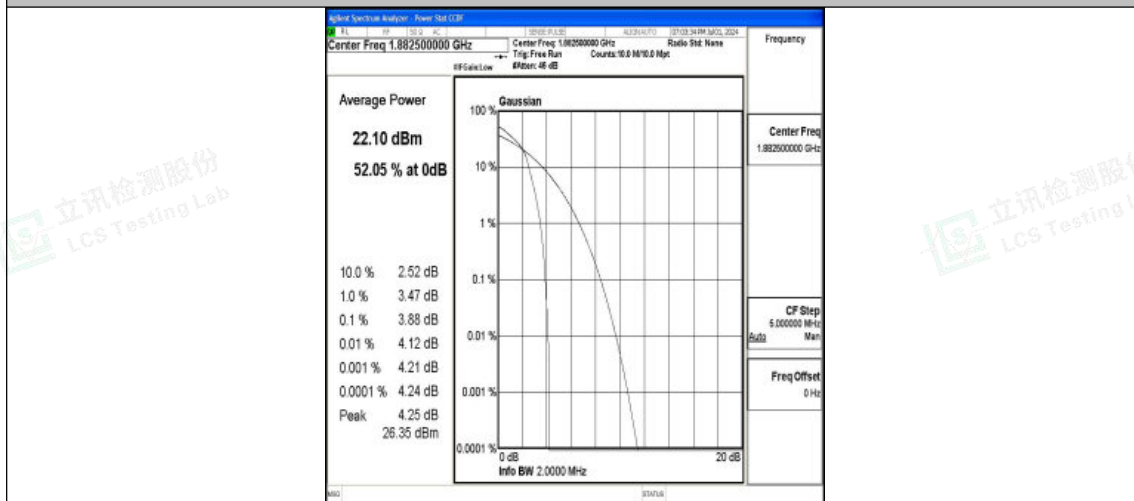
Band25-1.4MHz-16QAM-26365-1RB#0-PASS
