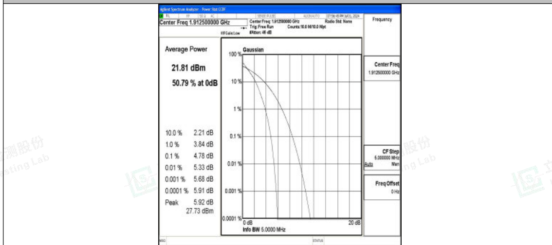
Band25-5MHz-QPSK-26665-25RB#0-PASS
