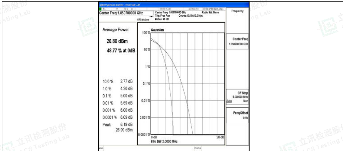
Band25-1.4MHz-16QAM-26047-6RB#0-PASS
