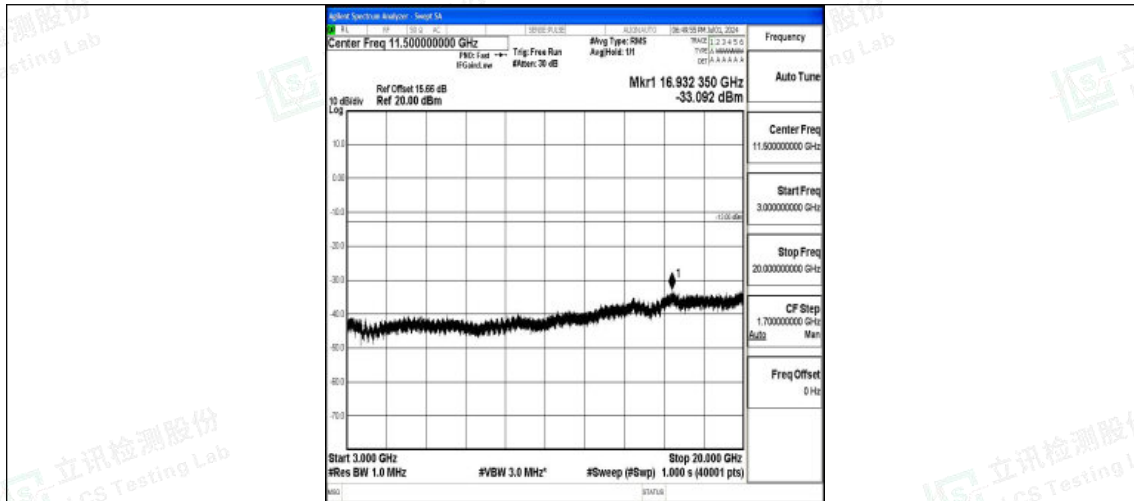
Band25_1.4MHz_16QAM_26365_1RB#0_3000~20000_3000~20000
