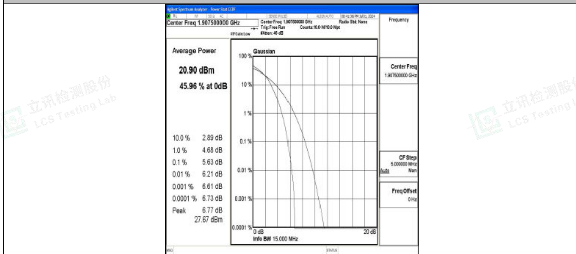
Band25-15MHz-16QAM-26615-75RB#0-PASS
