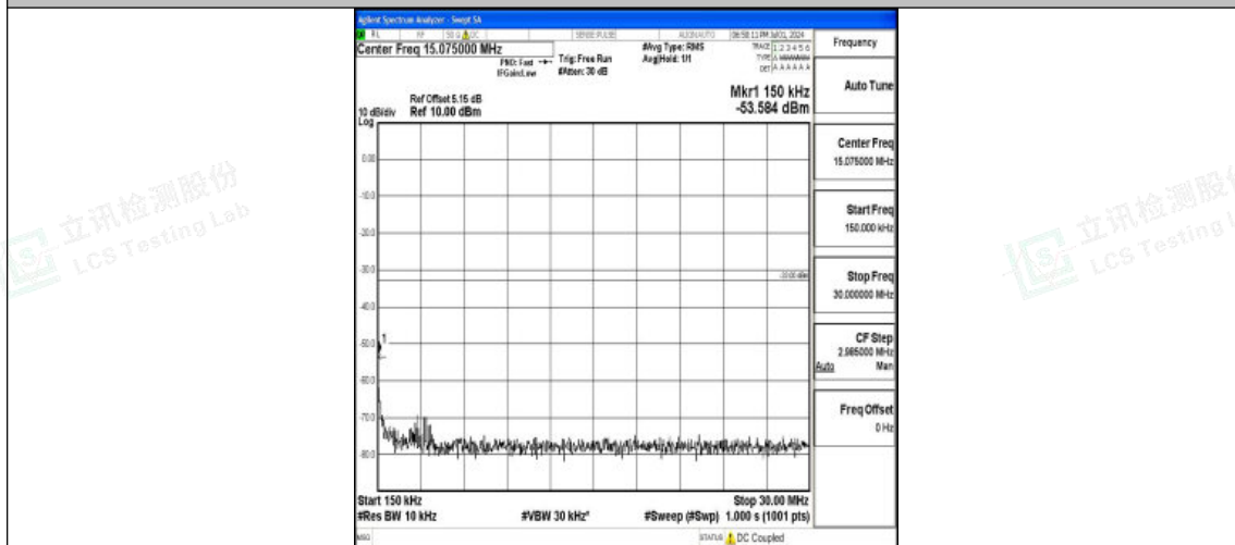
Band25_1.4MHz_QPSK_26683_1RB#0_0.15~30_0.15~30
