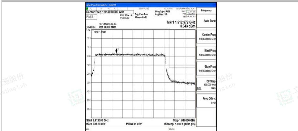
Band25_3MHz_16QAM_26675_15RB#0
