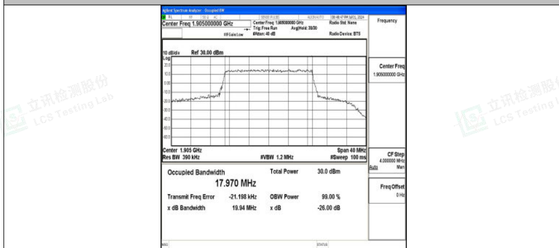
Band25-20MHz-16QAM-26590-100RB#0-PASS
