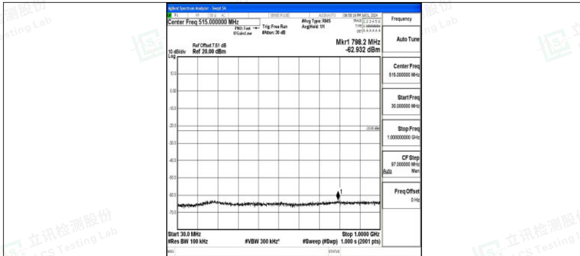
Band25_1.4MHz_QPSK_26683_1RB#0_30~1000_30~1000
