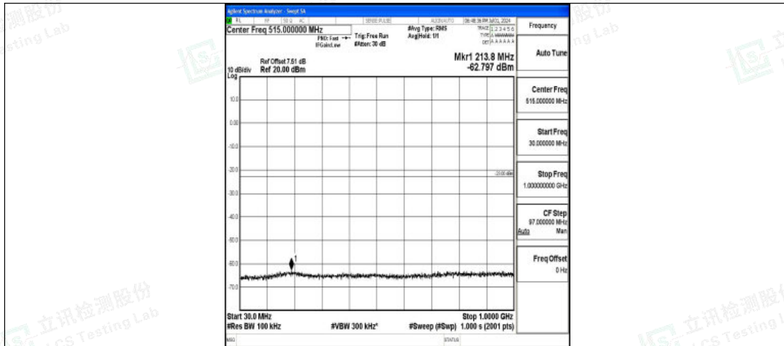
Band25_1.4MHz_16QAM_26047_1RB#0_30~1000_30~1000
