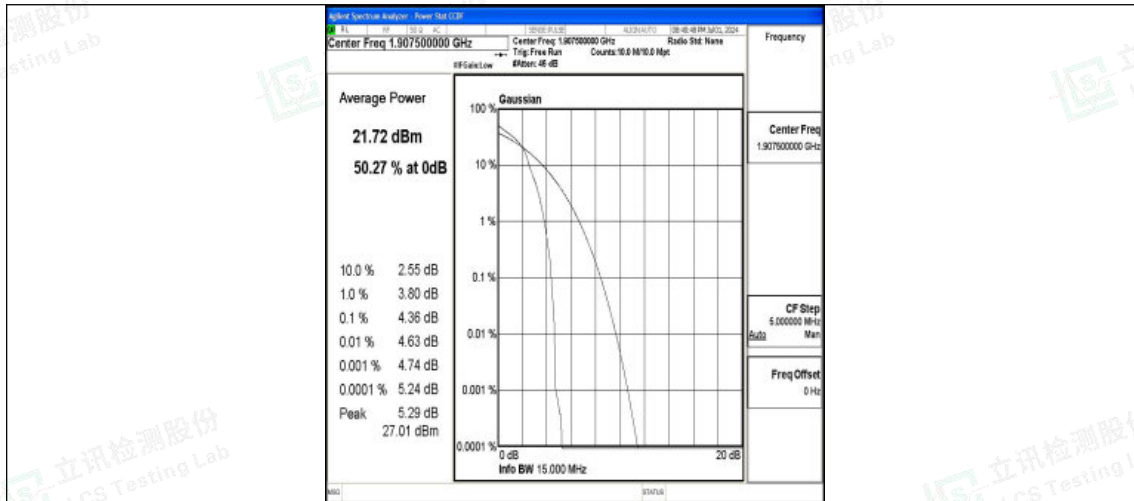
Band25-15MHz-16QAM-26615-1RB#0-PASS
