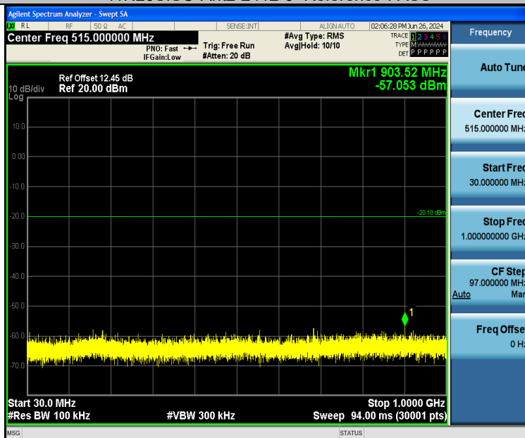
11N20SISO-Ant2-2412-30~1000-PASS
