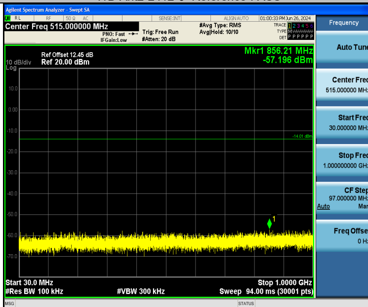
11B-Ant2-2412-30~1000-PASS
