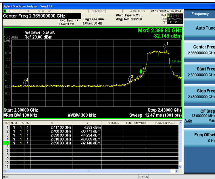
11G-Ant2-2412-PASS
