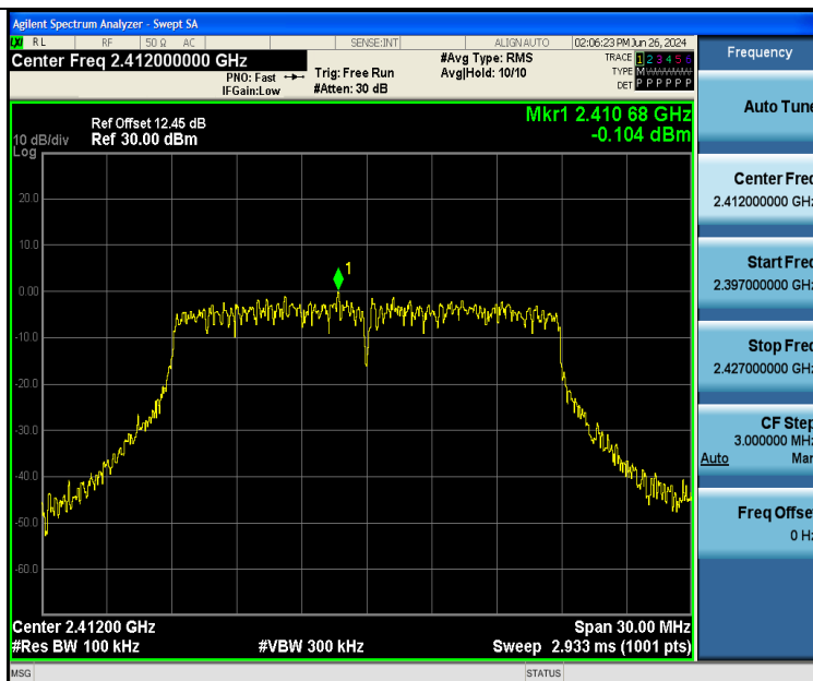
11N20SISO-Ant2-2412-0~Reference-PASS
