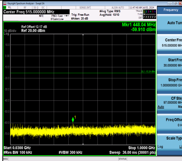
BLE_1M-Ant1-2480-30~1000-PASS
