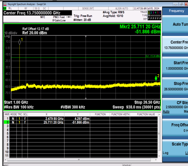
BLE_1M-Ant1-2480-1000~26500-PASS
