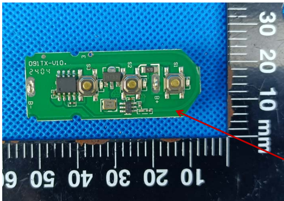
PCB Antenna
