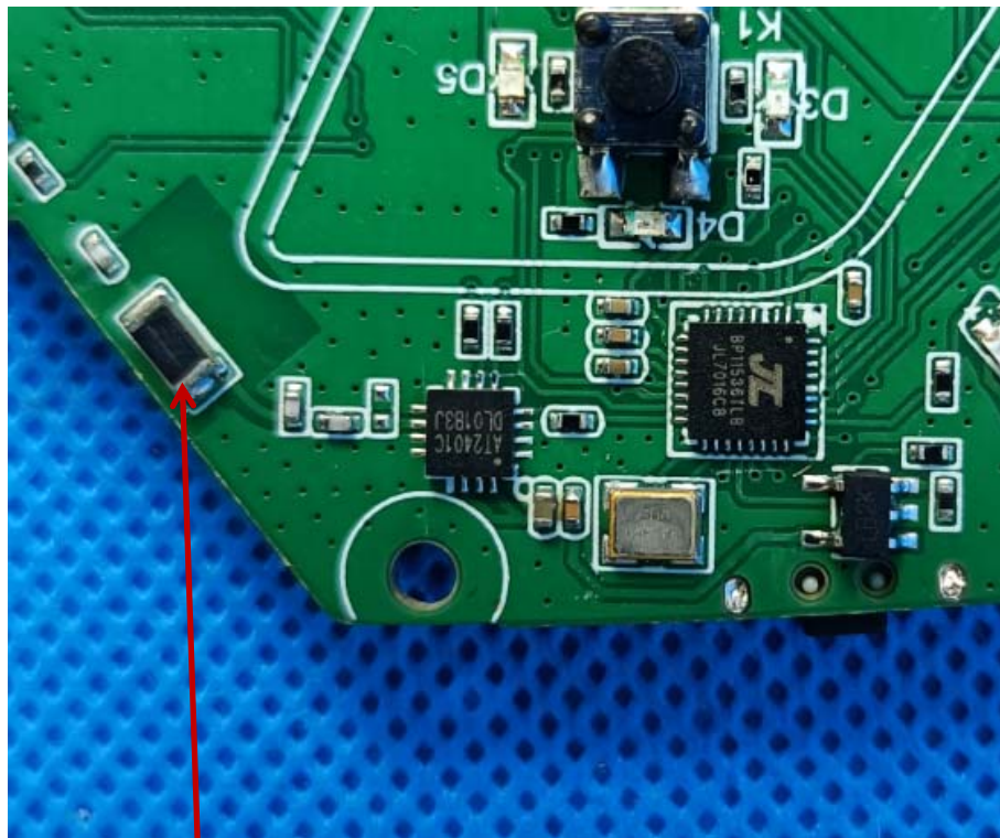
Chip ANT
