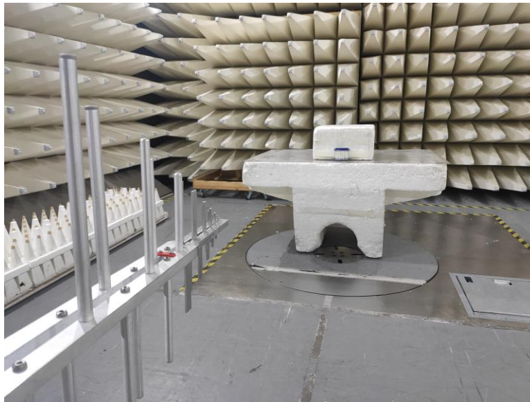
Photograph No.2 Setup for spurious emission field strength measurements in the anechoic chamber above 1000 MHz for XRT20229
