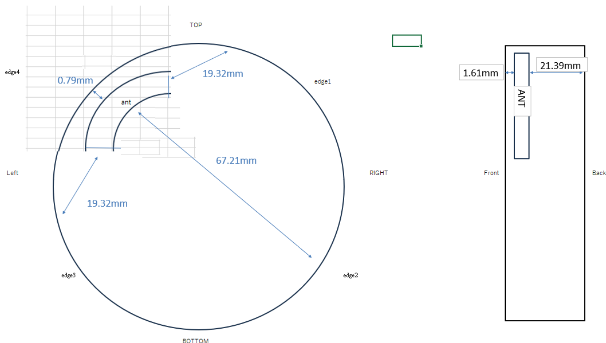
Photograph 21. Antenna position of EUT
