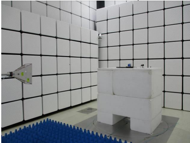
Part 15.247_BT_Radiated_Setup
