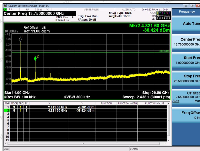
2.4G-Ant1-2411-1000~26500-PASS
