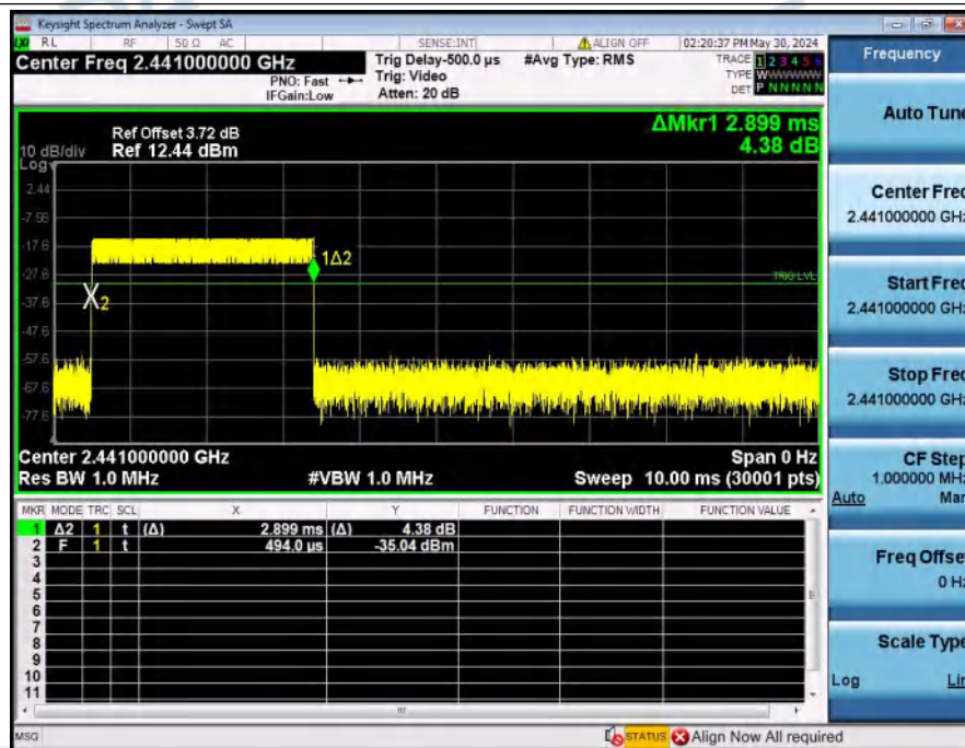
Dwell_Time_(Hopping)_NVNT_ANT1_1-DH5_2441_One_Burst_Time
