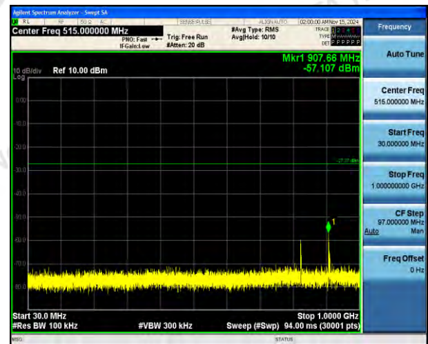
30MHz-1GHz
