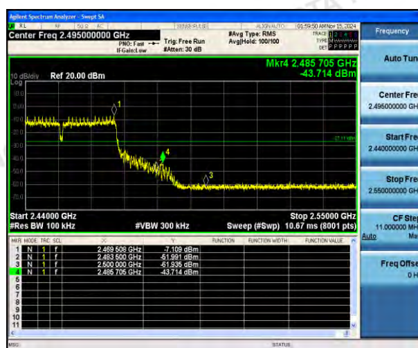
Right bandedge
