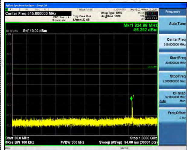
30MHz-1GHz
