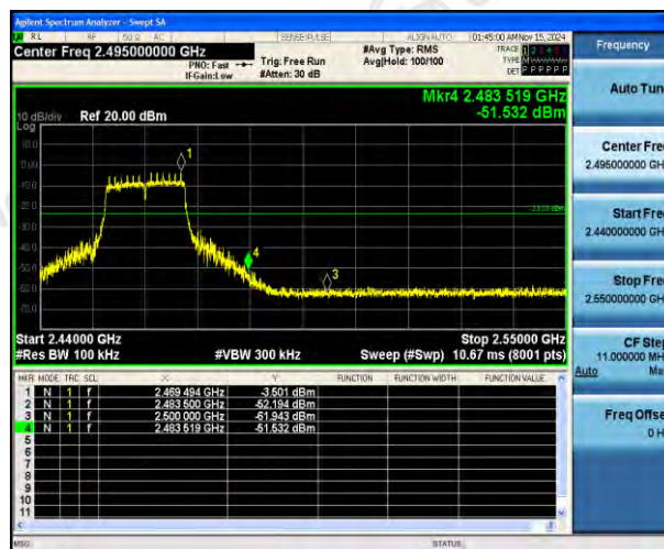
Right bandedge
