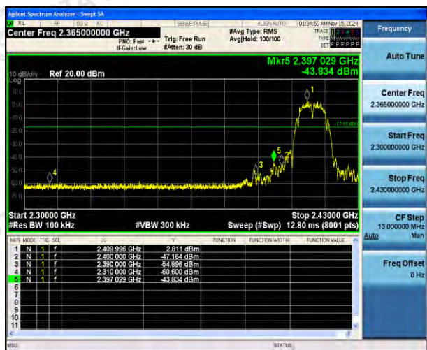
Left bandedge
