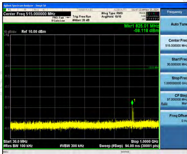
30MHz-1GHz
