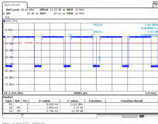
π/4DQPSK(2-DH5)_Channel 39
