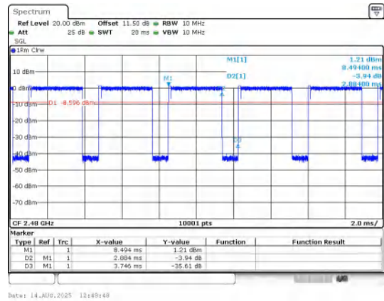
π/4DQPSK(2-DH5)_Channel 78
