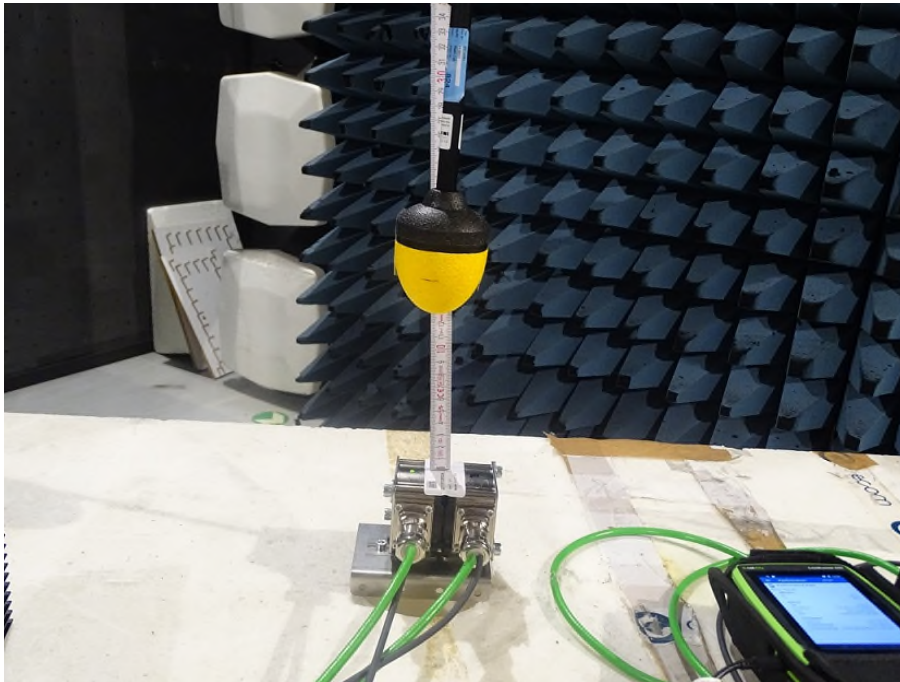
Photograph 5 : Measurement E-Field, worst case position, distance 20.0 cm
