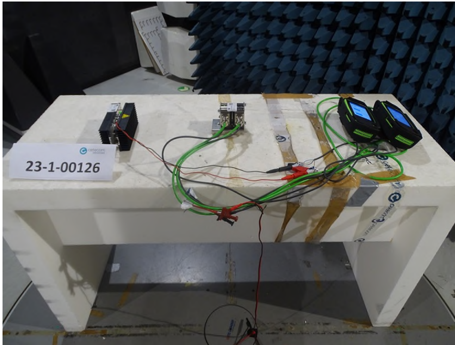
Photograph 1 : set-up
