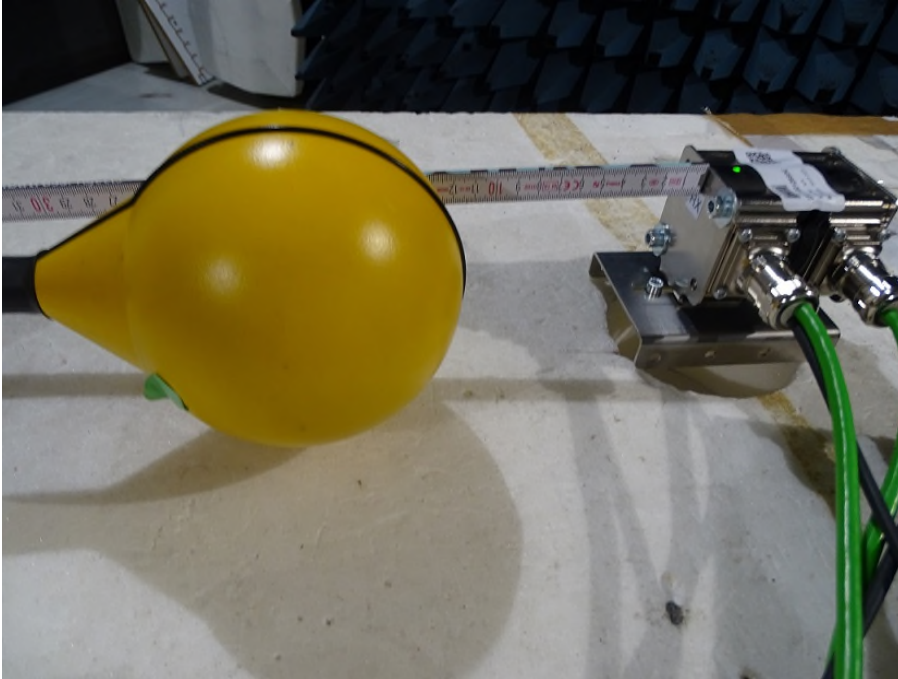
Photograph 3 : Measurement H-Field, worst case position, distance 20.0 cm
