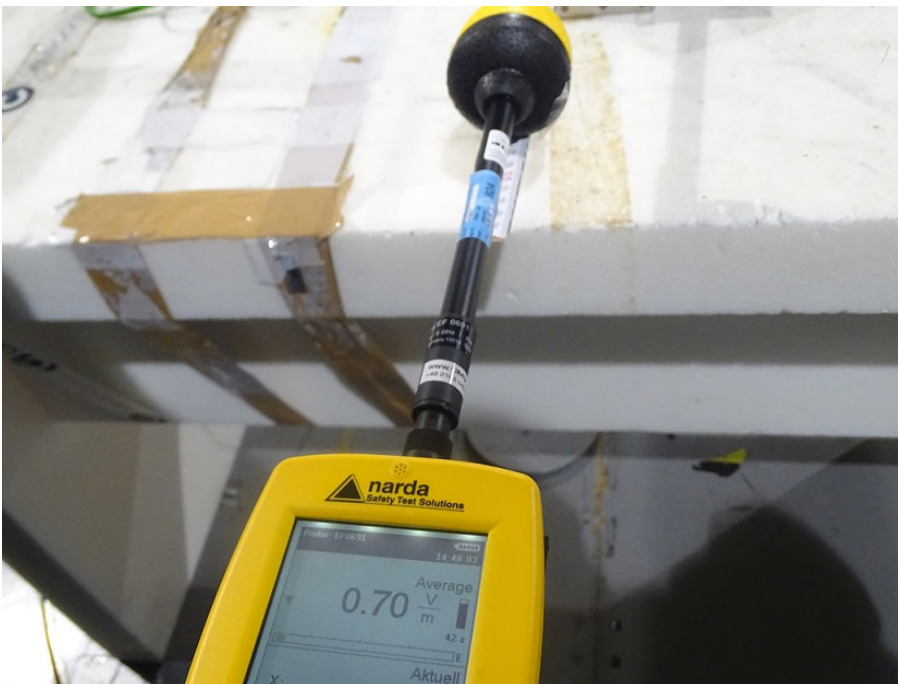
Photograph 4 : Measurement E-Field, worst case position distance 20.0 cm
