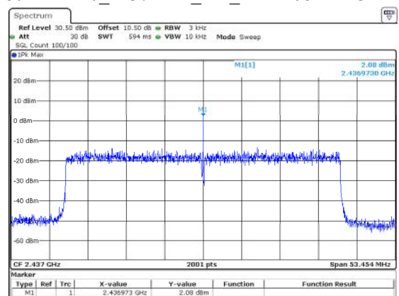
802.11ax40_2437MHz_RU_Full 2.08dBm/3kHz
