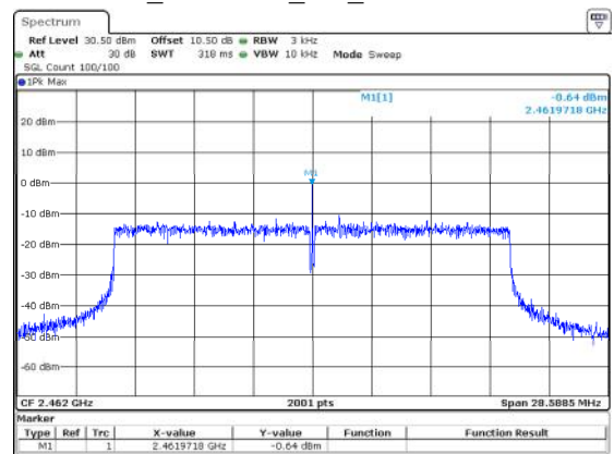
802.11ax20_2462MHz_RU_Full -0.64dBm/3kHz
