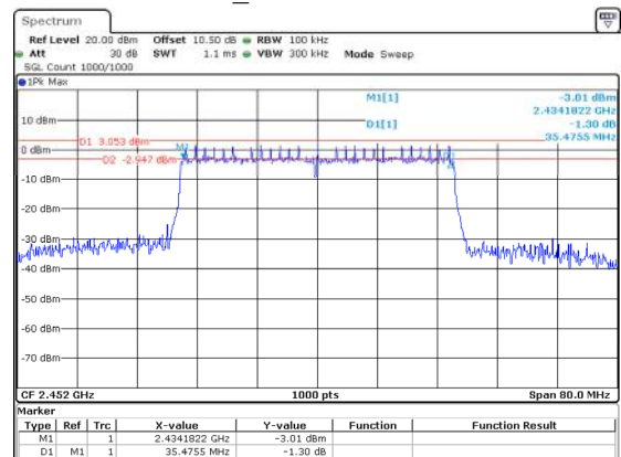
802.11n40_2452MHz 35.475MHz
