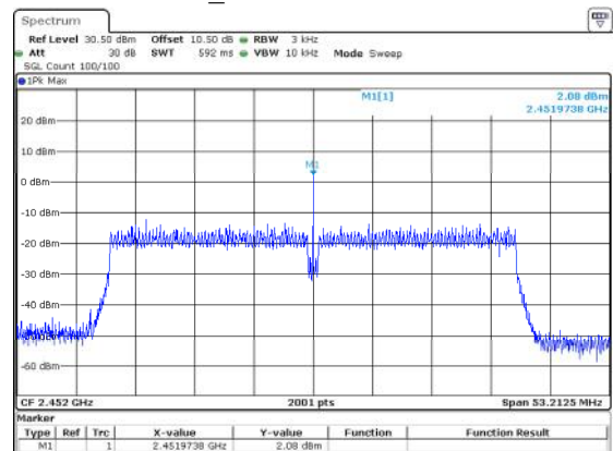
802.11n40_2452MHz 2.08dBm/3kHz
