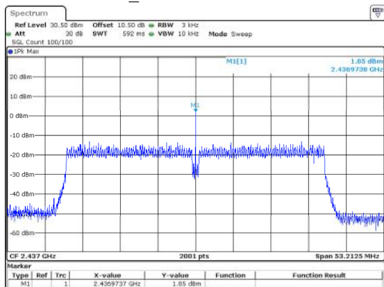
802.11n40_2437MHz 1.85dBm/3kHz
