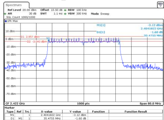
802.11n40_2422MHz 35.475MHz
