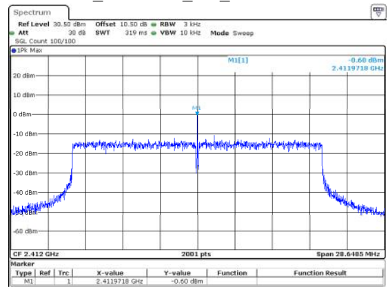
802.11ax20_2412MHz_RU_Full -0.60dBm/3kHz
