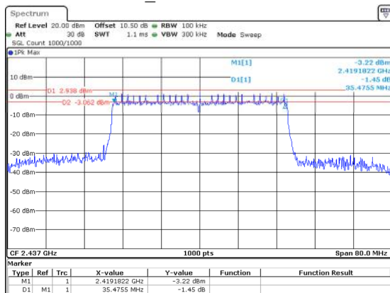
802.11n40_2437MHz 35.475MHz
