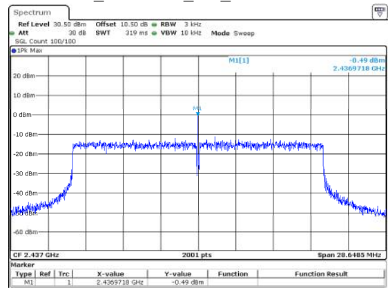
802.11ax20_2437MHz_RU_Full -0.49dBm/3kHz
