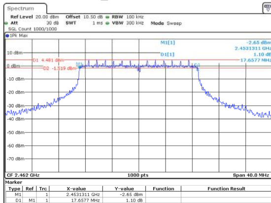
802.11n20_2462MHz 17.658MHz
