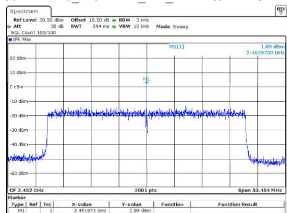
802.11ax40_2452MHz_RU_Full 1.89dBm/3kHz
