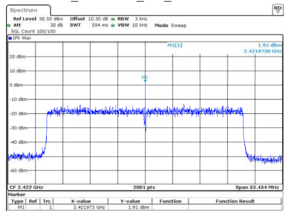
802.11ax40_2422MHz_RU_Full 1.91dBm/3kHz
