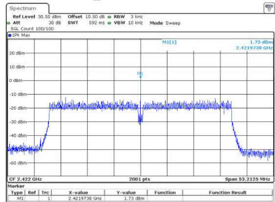
802.11n40_2422MHz 1.73dBm/3kHz
