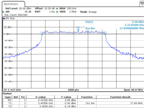
802.11n20_2412MHz 17.840MHz
