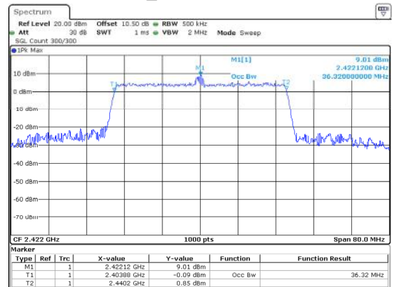
802.11n40_2422MHz 36.320MHz
