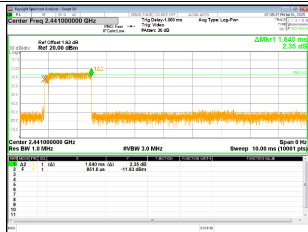
3DH5-2441MHz-One burst
