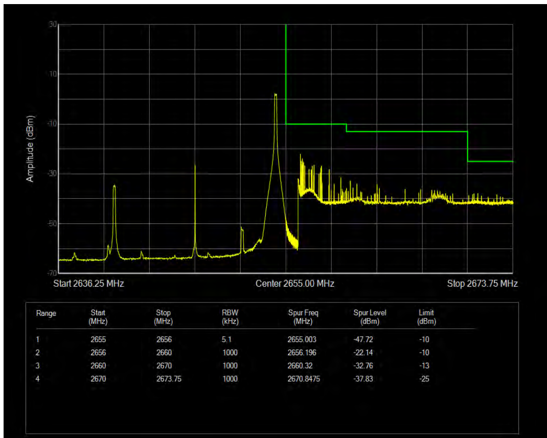
Band41a 16QAM BW=15MHz Channel=41165 RB Size=1 Position=#Max
