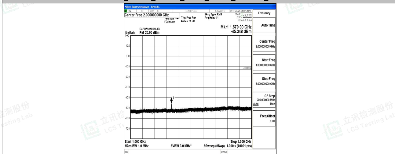
Band5_10MHz_16QAM_20600_1RB#0_1000~3000_1000~3000
