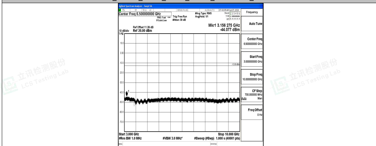
Band5_10MHz_QPSK_20525_1RB#0_3000~10000_3000~10000
