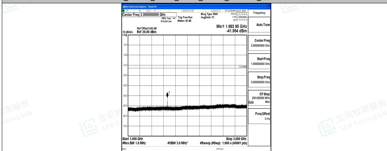
Band5_10MHz_QPSK_20525_1RB#0_1000~3000_1000~3000
