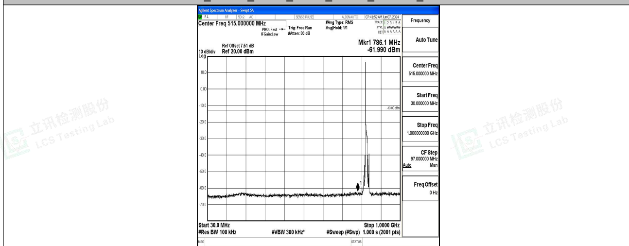
Band5_10MHz_QPSK_20450_1RB#0_30~1000_30~1000
