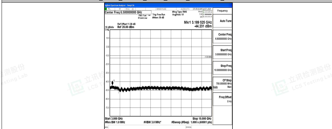
Band5_5MHz_16QAM_20525_1RB#0_3000~10000_3000~10000
