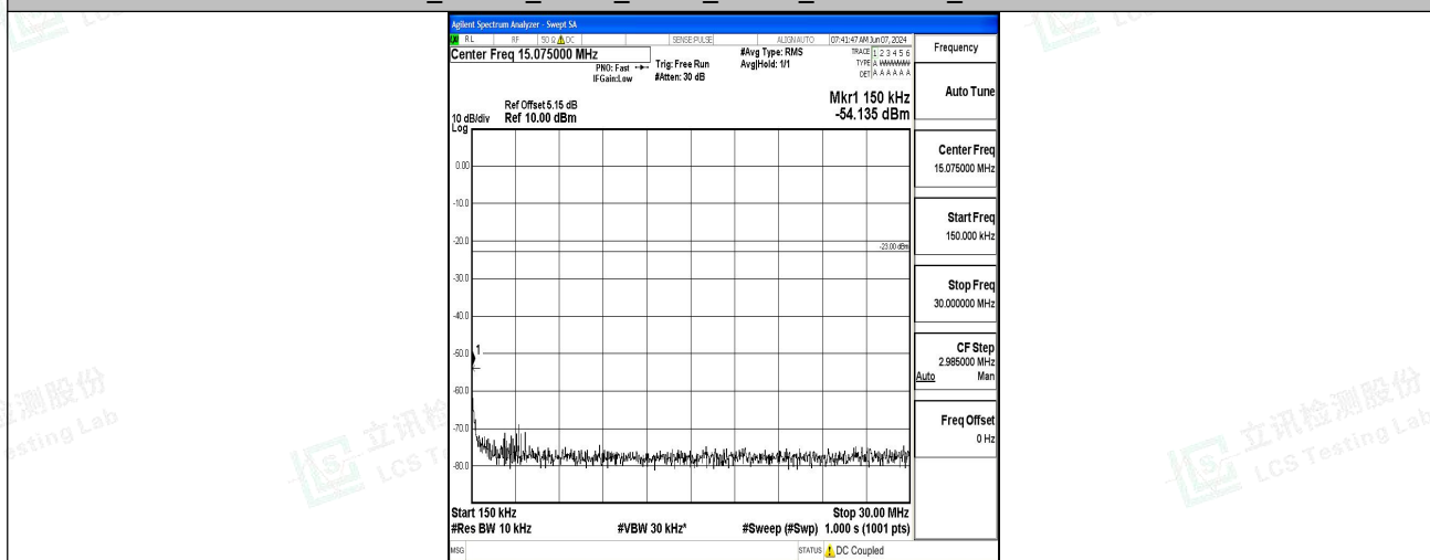
Band5_10MHz_QPSK_20450_1RB#0_0.15~30_0.15~30
