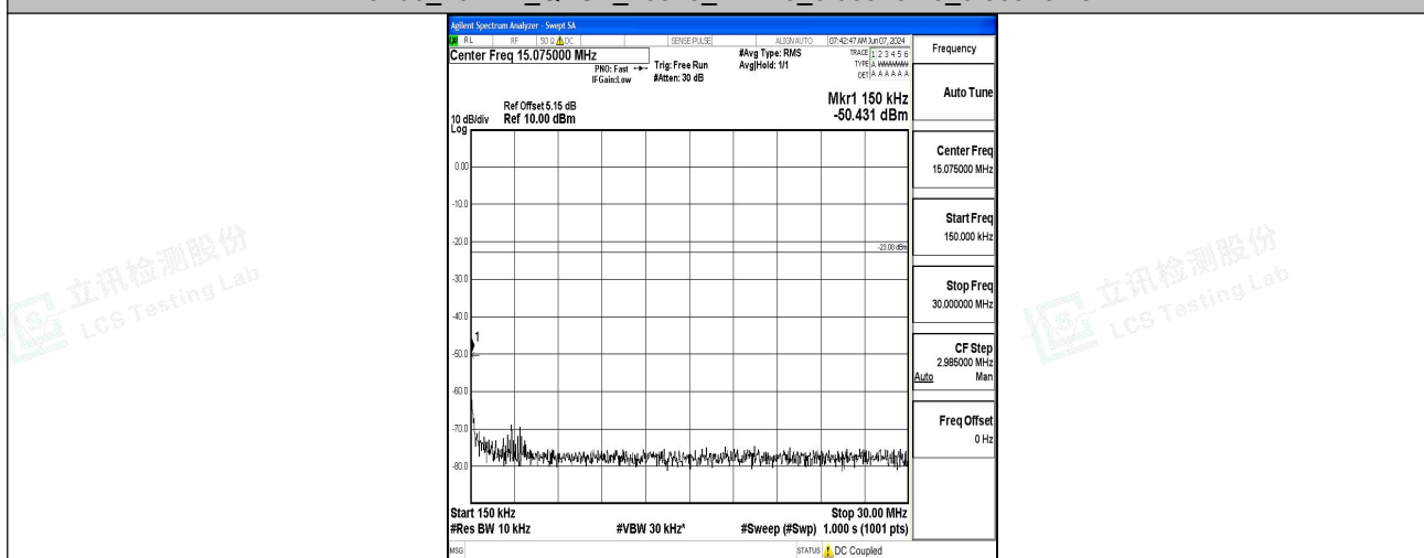
Band5_10MHz_QPSK_20525_1RB#0_0.15~30_0.15~30
